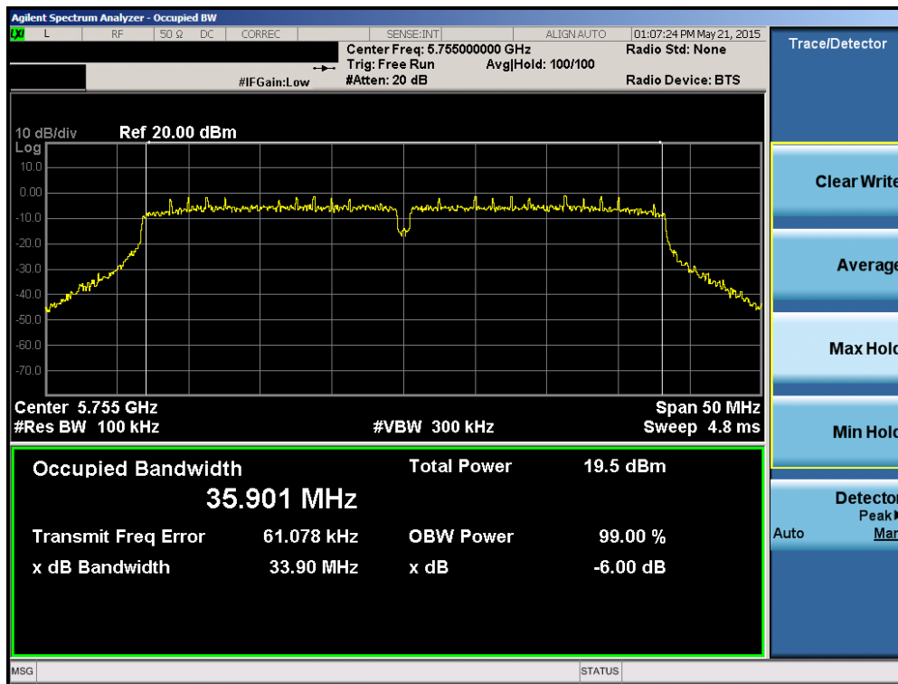
Plot 6-32. 6dB Bandwidth Plot (40MHz BW 802.11n (UNII Band 3) – Ch. 151)
