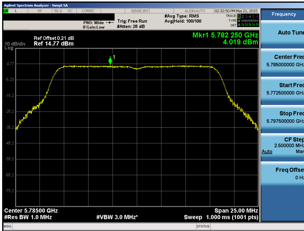
Plot 6-60. Power Spectral Density Plot (802.11a (UNII Band 3) – Ch. 157)
