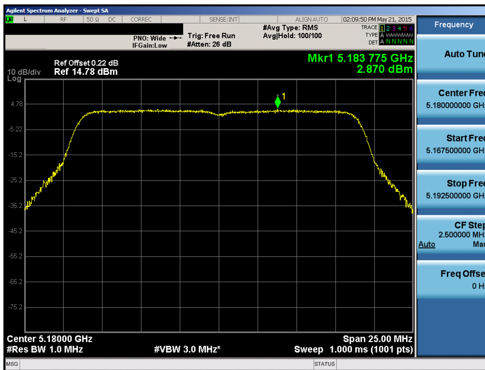
Plot 6-37. Power Spectral Density Plot (20MHz BW 802.11n (UNII Band 1) – Ch. 36)
