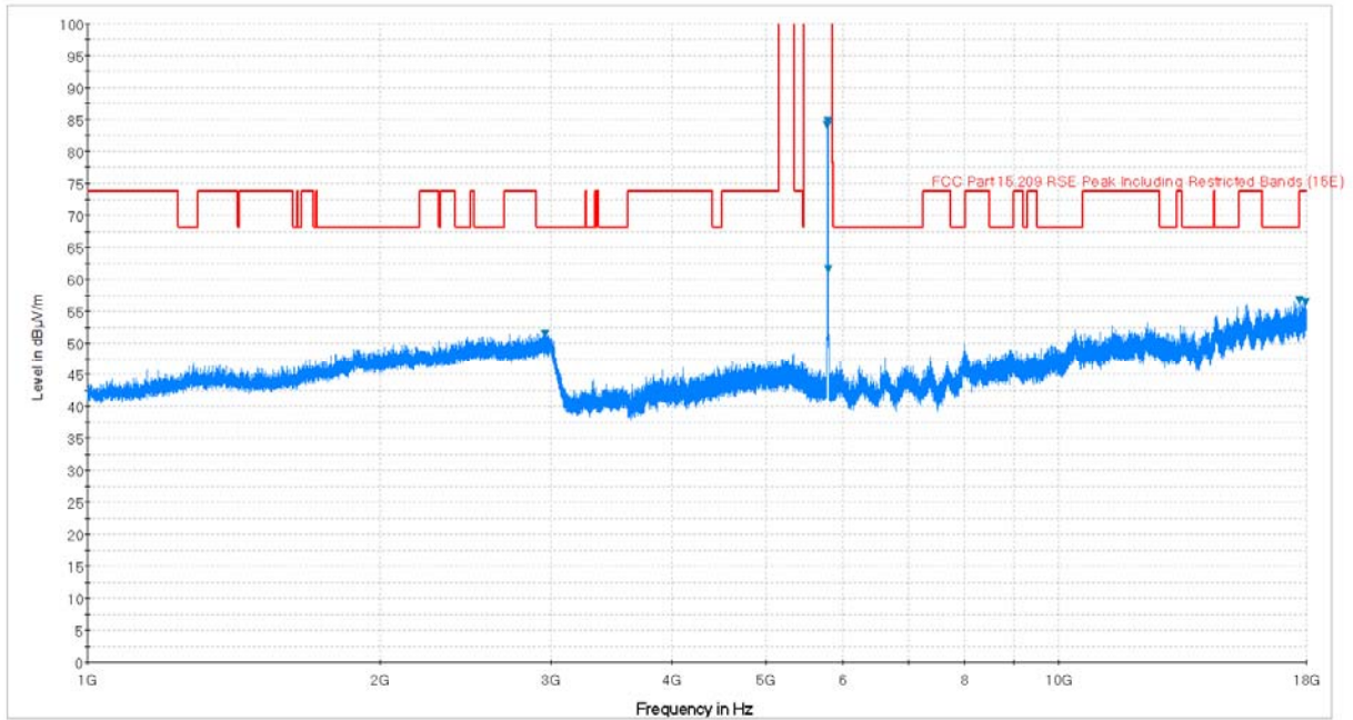
Plot 6-74. Radiated Spurious Plot above 1GHz (802.11a – U3 Ch. 157, Ant. Pol. V)
