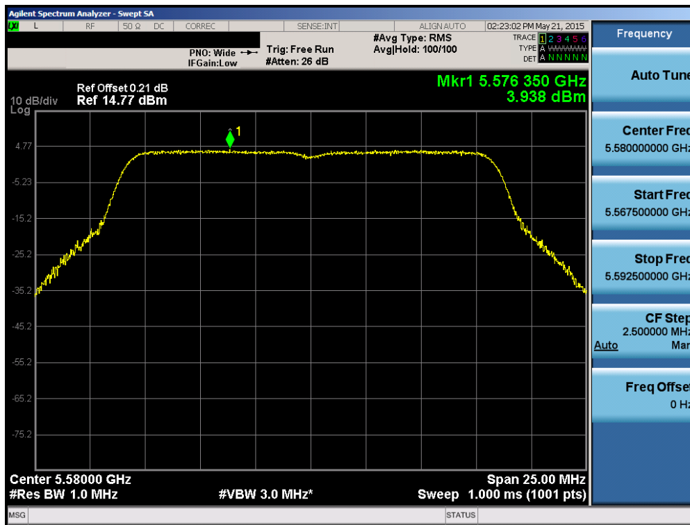
Plot 6-51. Power Spectral Density Plot (802.11a (UNII Band 2C) – Ch. 116)
