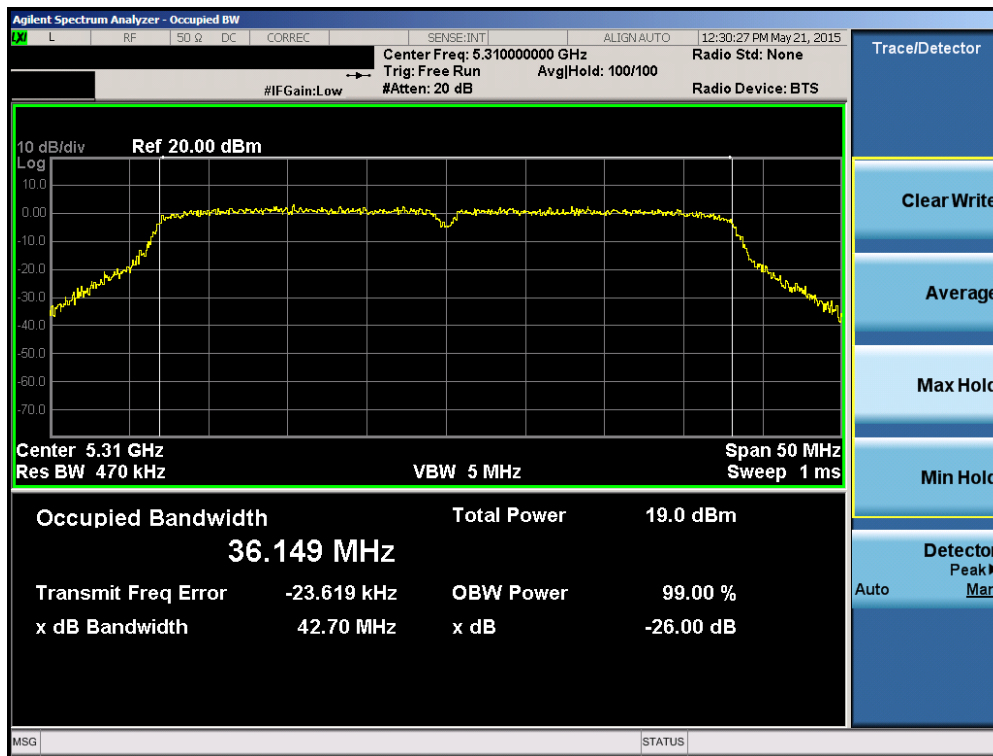
Plot 6-16. 26dB Bandwidth Plot (40MHz BW 802.11n (UNII Band 2A) – Ch. 62)
