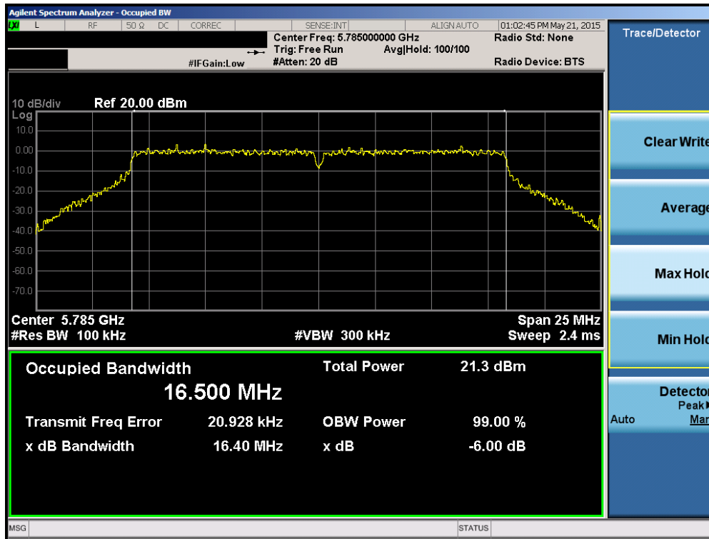
Plot 6-27. 6dB Bandwidth Plot (802.11a (UNII Band 3) – Ch. 157)
