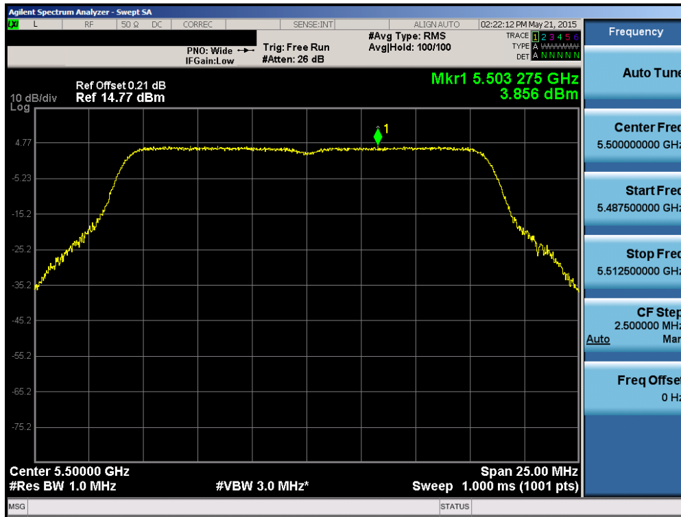
Plot 6-50. Power Spectral Density Plot (802.11a (UNII Band 2C) – Ch. 100)
