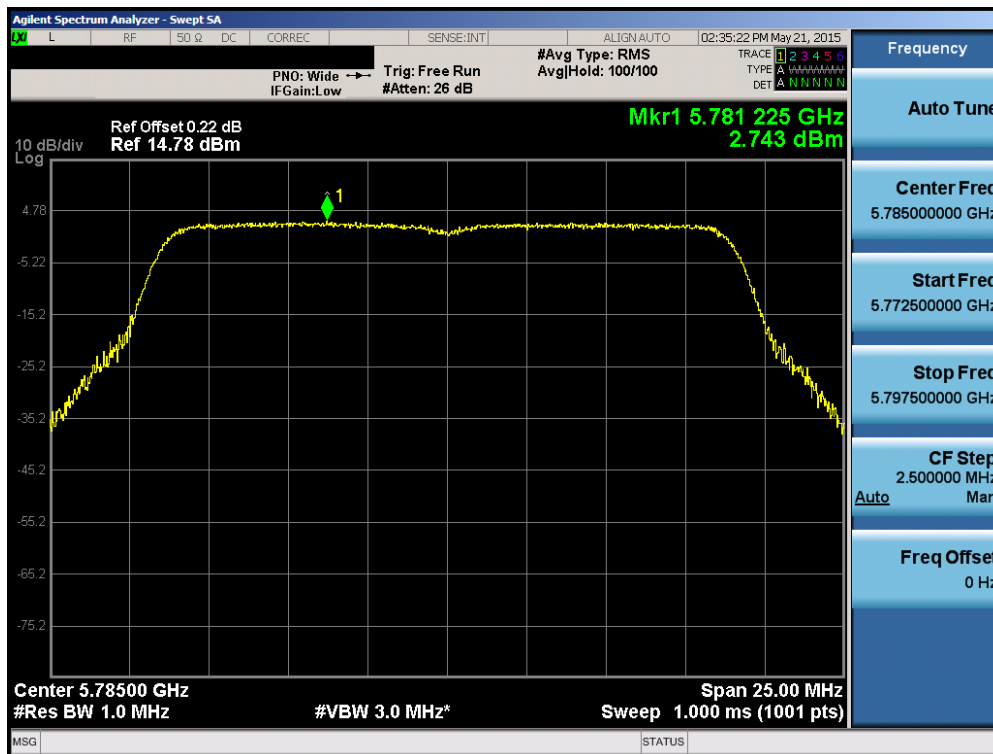
Plot 6-63. Power Spectral Density Plot (20MHz BW 802.11a/n (UNII Band 3) – Ch. 157)
