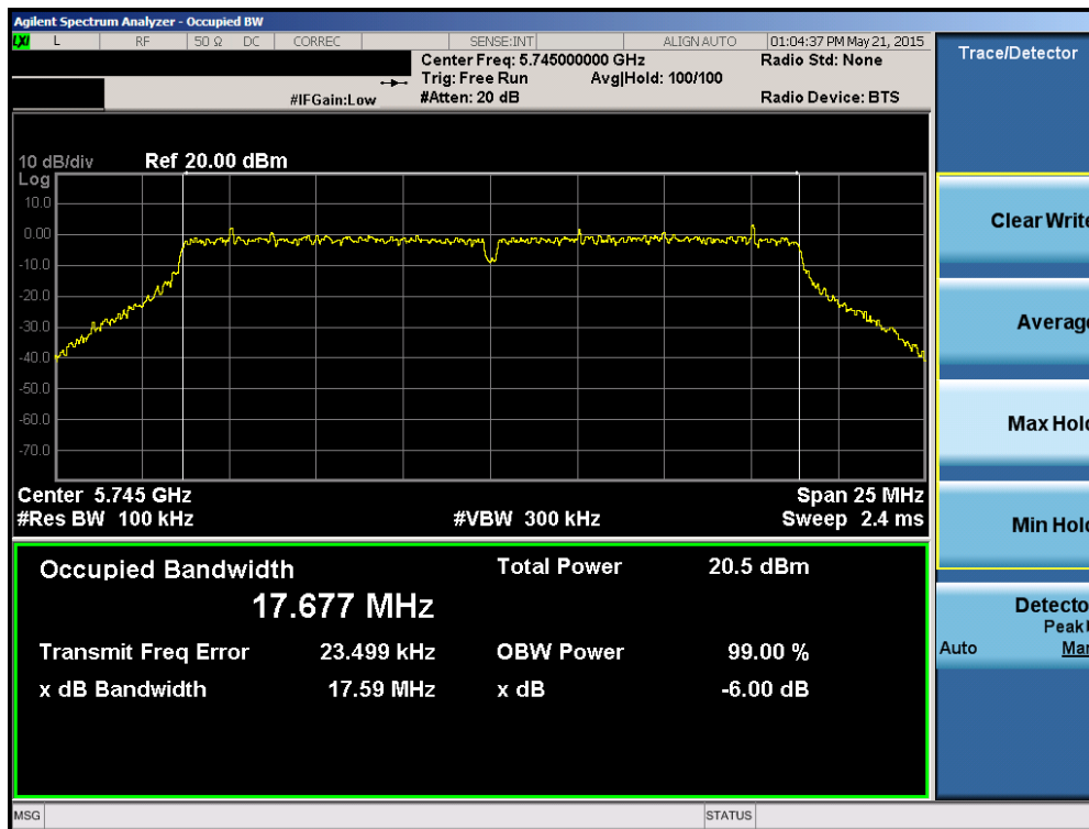
Plot 6-29. 6dB Bandwidth Plot (20MHz BW 802.11n (UNII Band 3) – Ch. 149)
