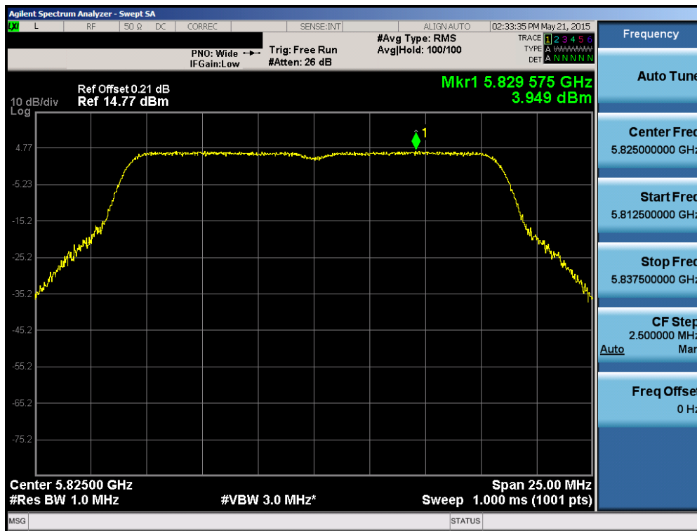
Plot 6-61. Power Spectral Density Plot (802.11a (UNII Band 3) – Ch. 165)
