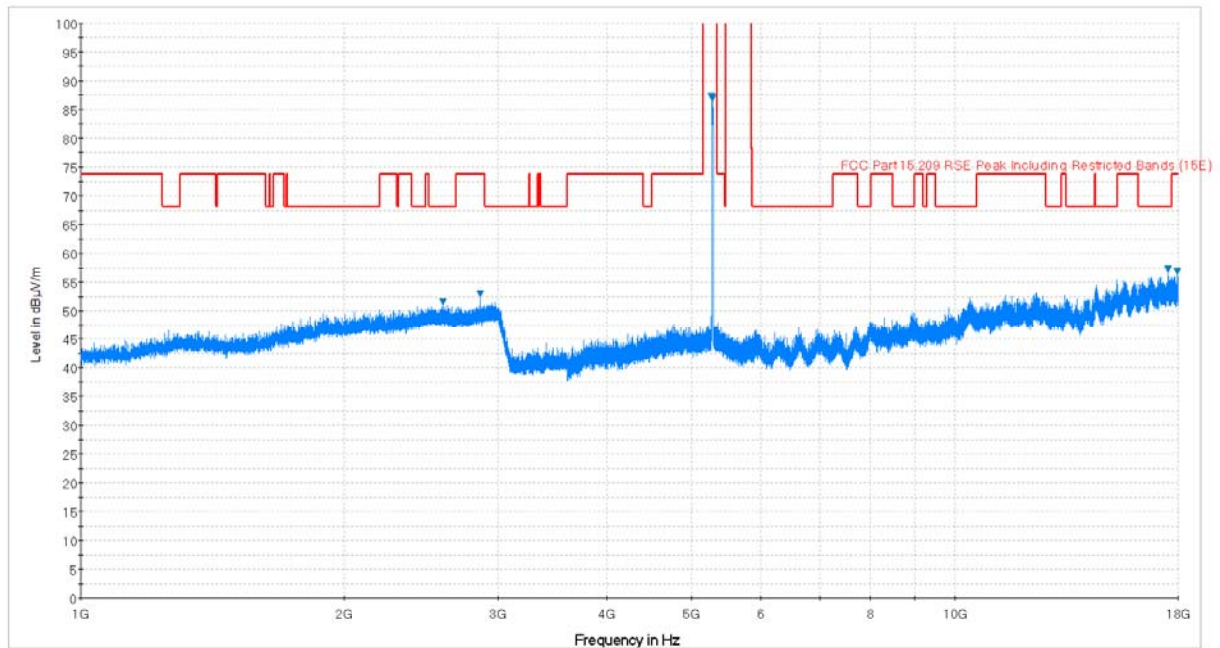
Plot 6-70. Radiated Spurious Plot above 1GHz (802.11a – U2A Ch. 56, Ant. Pol. V)
