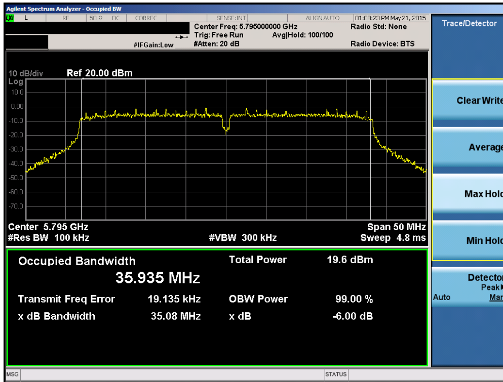
Plot 6-33. 6dB Bandwidth Plot (40MHz BW 802.11n (UNII Band 3) – Ch. 159)
