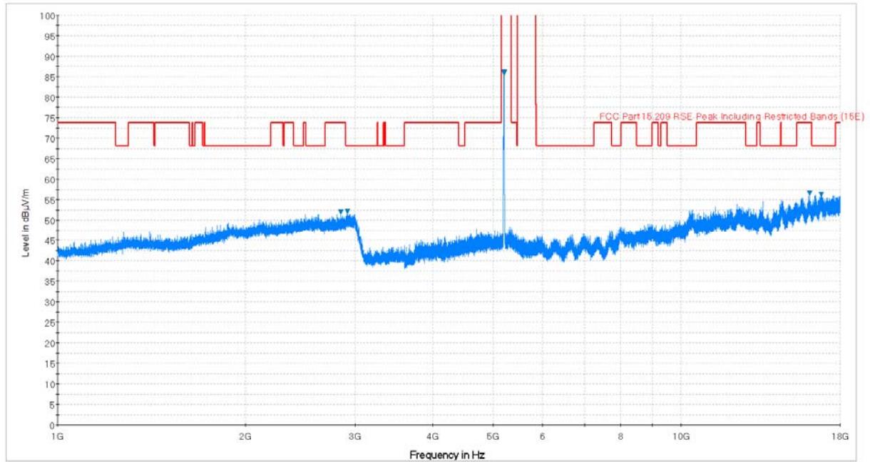
Plot 6-67. Radiated Spurious Plot above 1GHz (802.11a – U1 Ch. 40, Ant. Pol. H)
