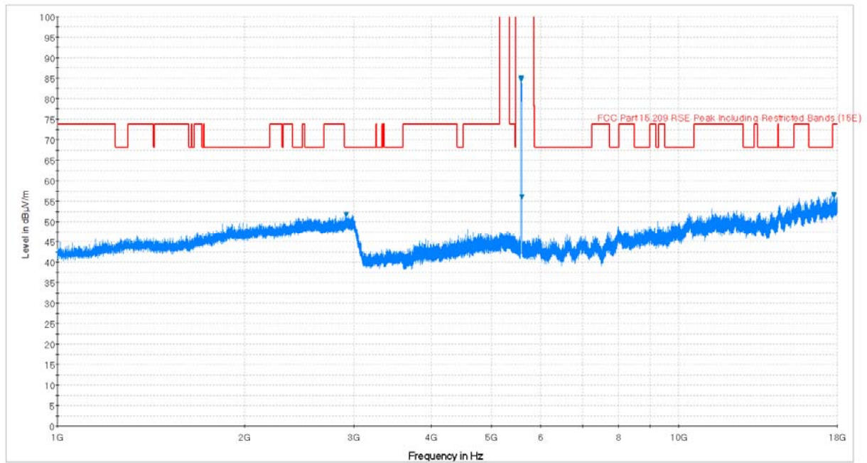
Plot 6-71. Radiated Spurious Plot above 1GHz (802.11a – U2C Ch. 116, Ant. Pol. H)
