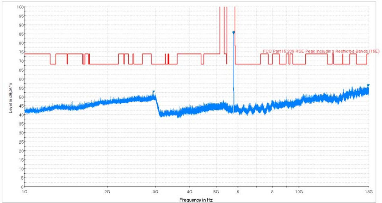
Plot 6-73. Radiated Spurious Plot above 1GHz (802.11a – U3 Ch. 157, Ant. Pol. H)
