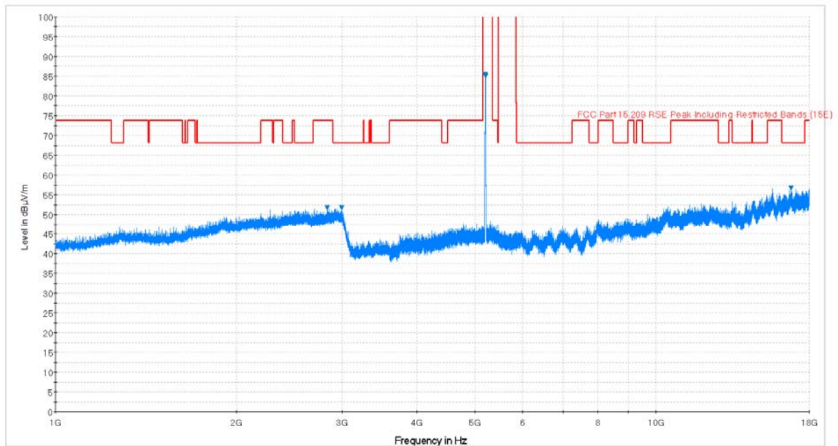
Plot 6-68. Radiated Spurious Plot above 1GHz (802.11a – U1 Ch. 40, Ant. Pol. V)
