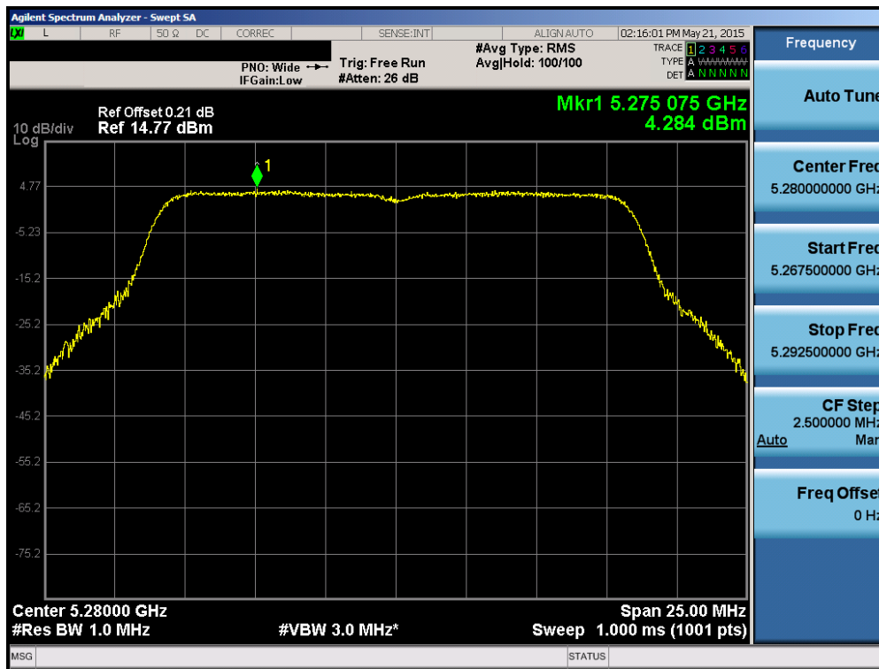
Plot 6-43. Power Spectral Density Plot (802.11a (UNII Band 2A) – Ch. 56)
