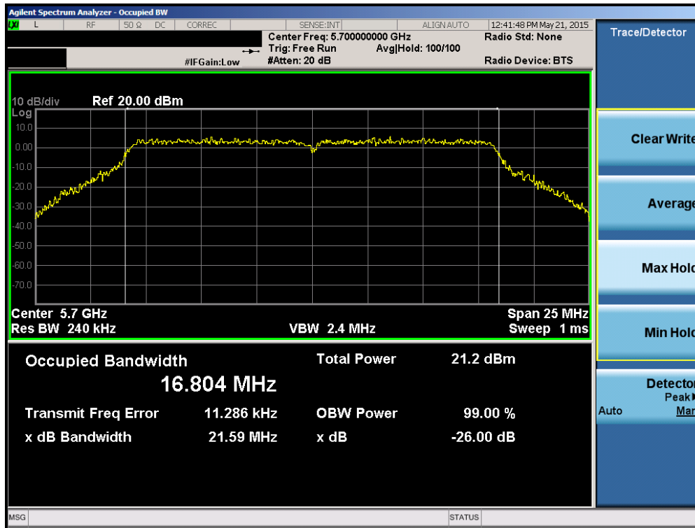
Plot 6-19. 26dB Bandwidth Plot (802.11a (UNII Band 2C) – Ch. 140)
