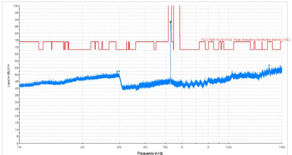
Plot 6-69. Radiated Spurious Plot above 1GHz (802.11a – U2A Ch. 56, Ant. Pol. H)
