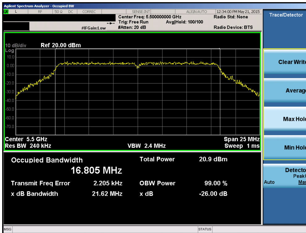
Plot 6-17. 26dB Bandwidth Plot (802.11a (UNII Band 2C) – Ch. 100)
