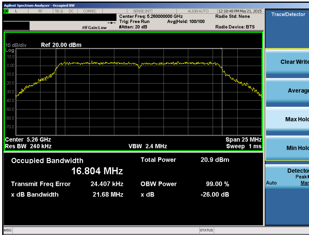
Plot 6-9. 26dB Bandwidth Plot (802.11a (UNII Band 2A) – Ch. 52)
