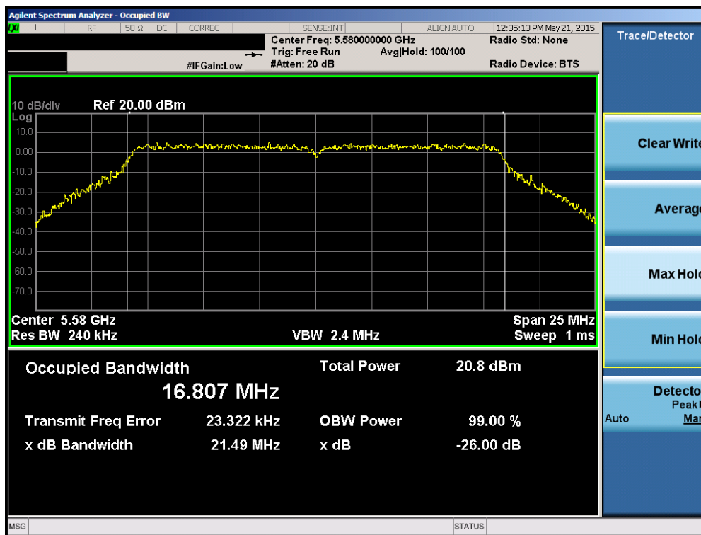
Plot 6-18. 26dB Bandwidth Plot (802.11a (UNII Band 2C) – Ch. 116)
