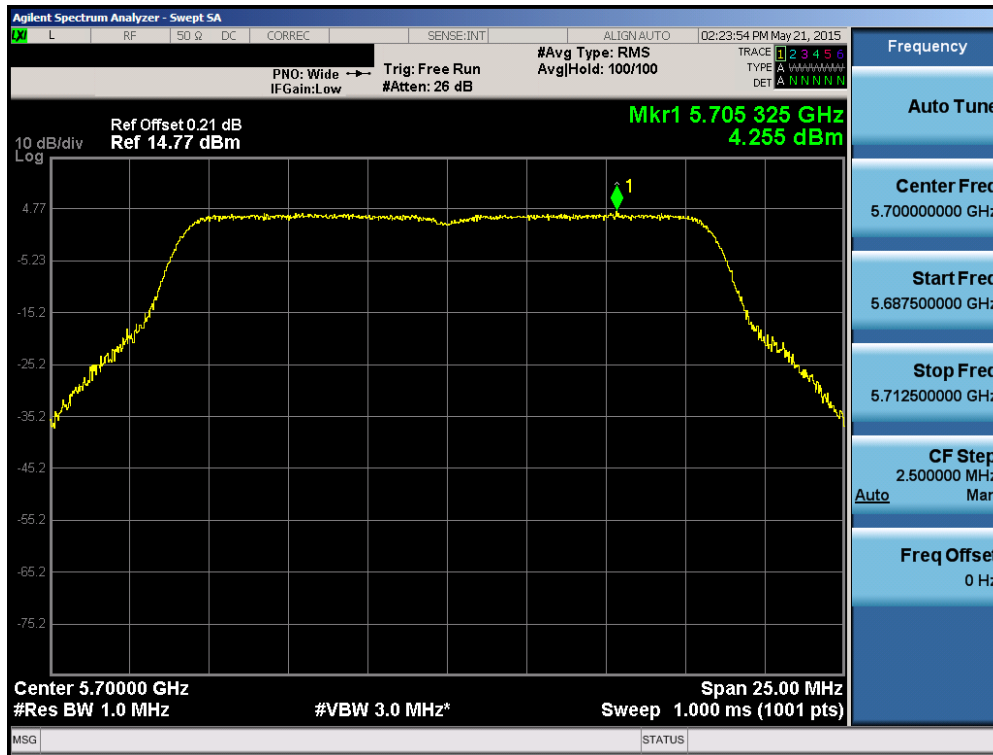
Plot 6-52. Power Spectral Density Plot (802.11a (UNII Band 2C) – Ch. 140
