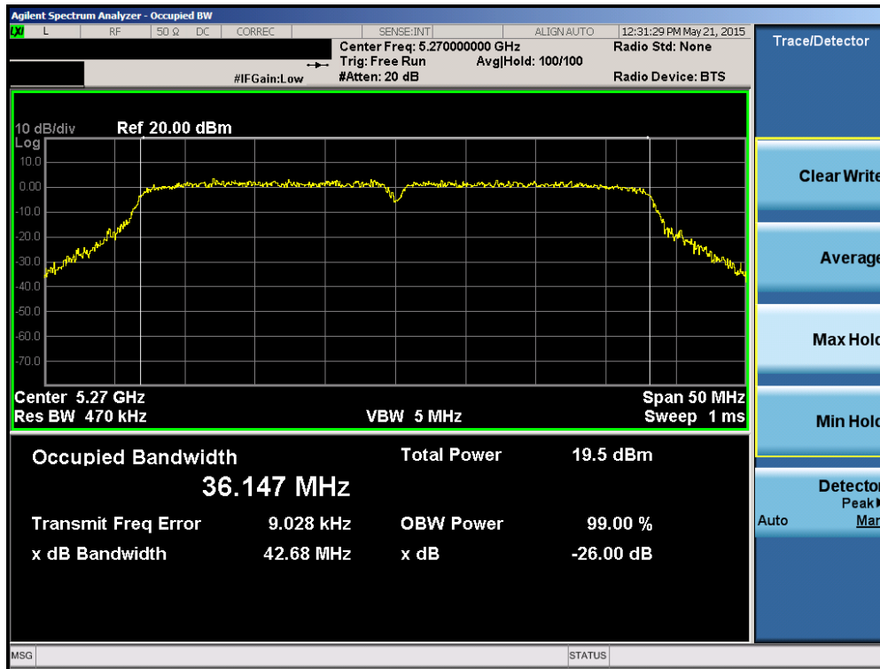
Plot 6-15. 26dB Bandwidth Plot (40MHz BW 802.11n (UNII Band 2A) – Ch. 54)
