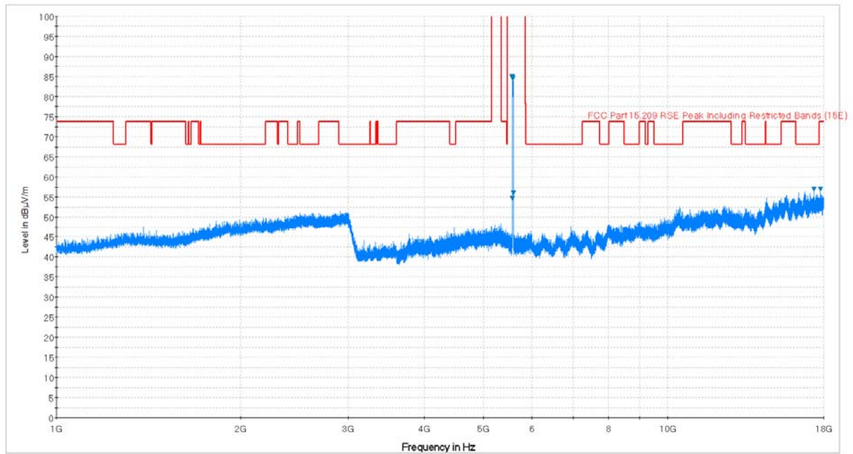
Plot 6-72. Radiated Spurious Plot above 1GHz (802.11a – U2C Ch. 116, Ant. Pol. V)
