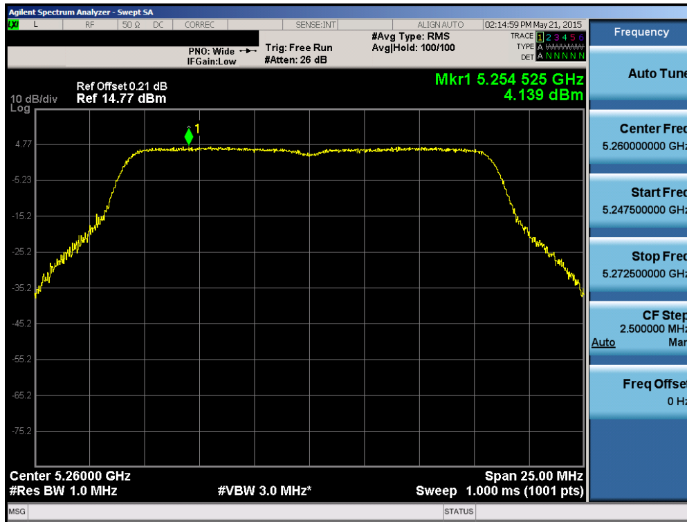
Plot 6-42. Power Spectral Density Plot (802.11a (UNII Band 2A) – Ch. 52)
