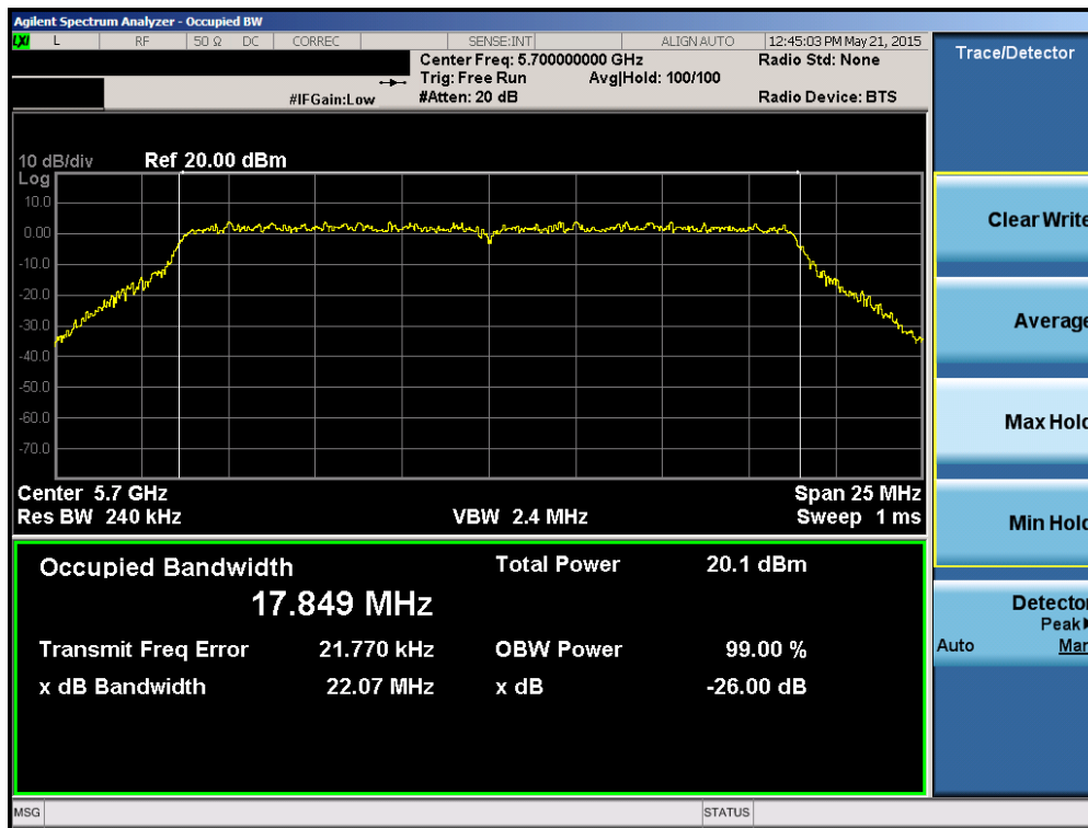
Plot 6-22. 26dB Bandwidth Plot (20MHz BW 802.11n (UNII Band 2C) – Ch. 140)
