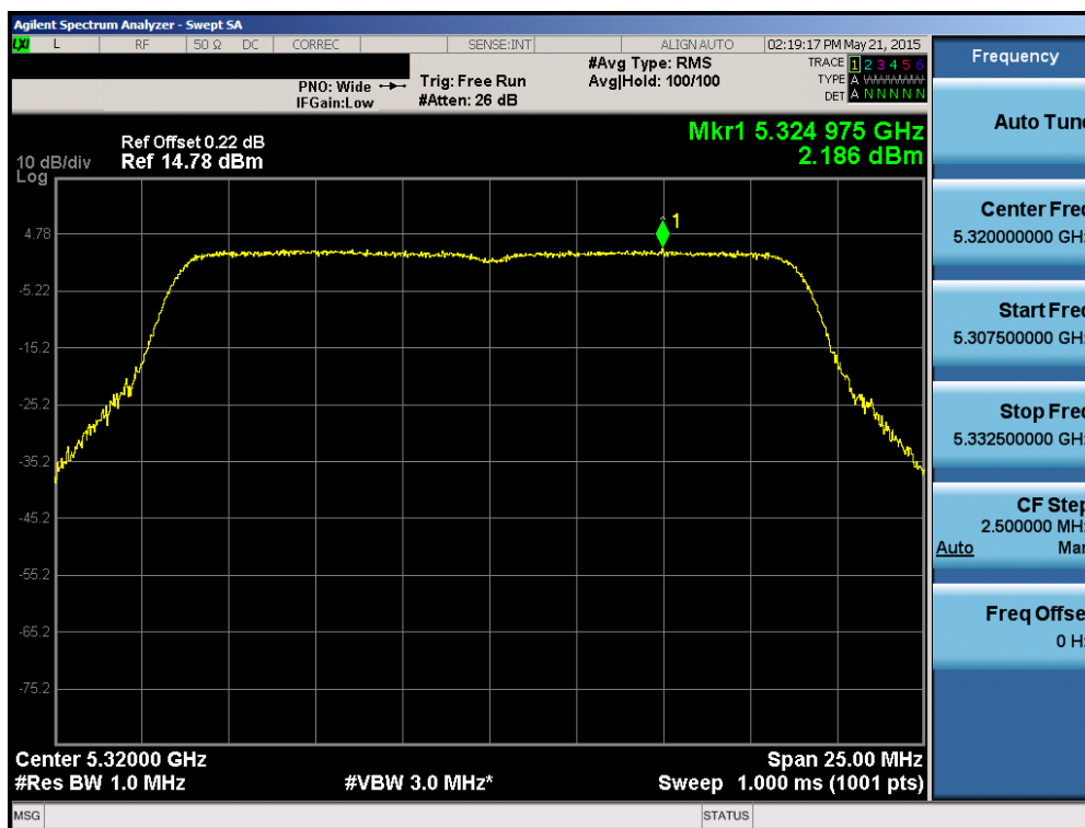
Plot 6-47. Power Spectral Density Plot (20MHz BW 802.11n (UNII Band 2A) – Ch. 64)
