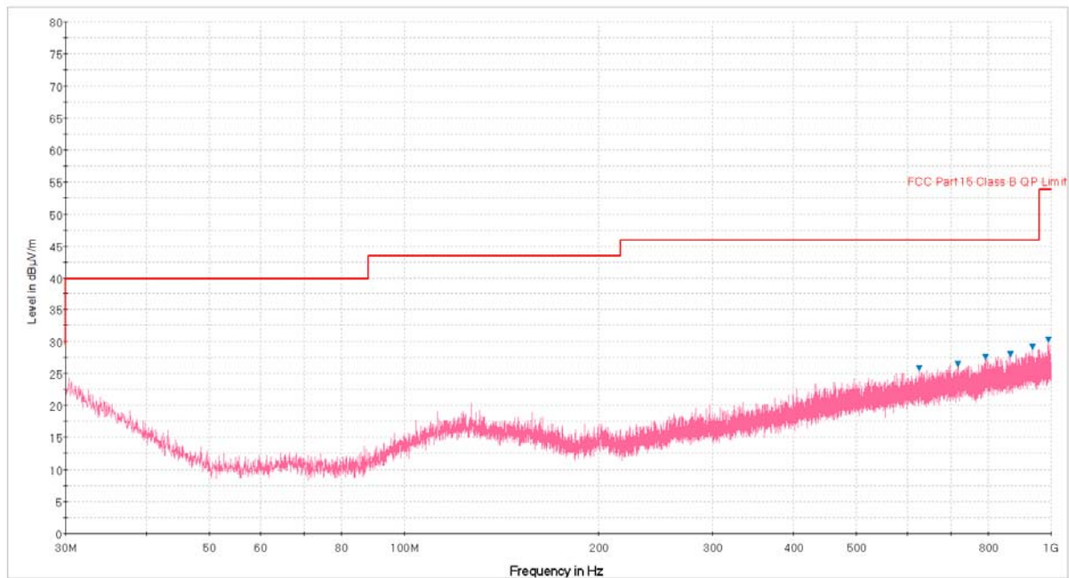
Plot 6-96. Radiated Spurious Plot below 1GHz (802.11a – U3 Ch. 157, Ant. Pol. V)
