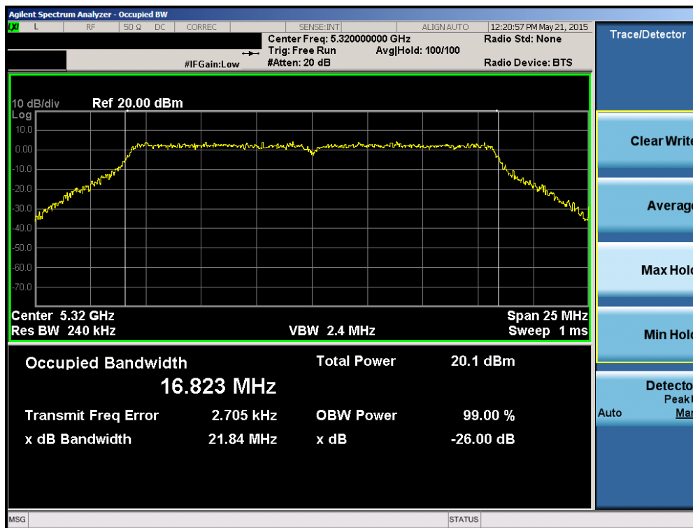
Plot 6-11. 26dB Bandwidth Plot (802.11a (UNII Band 2A) – Ch. 64)
