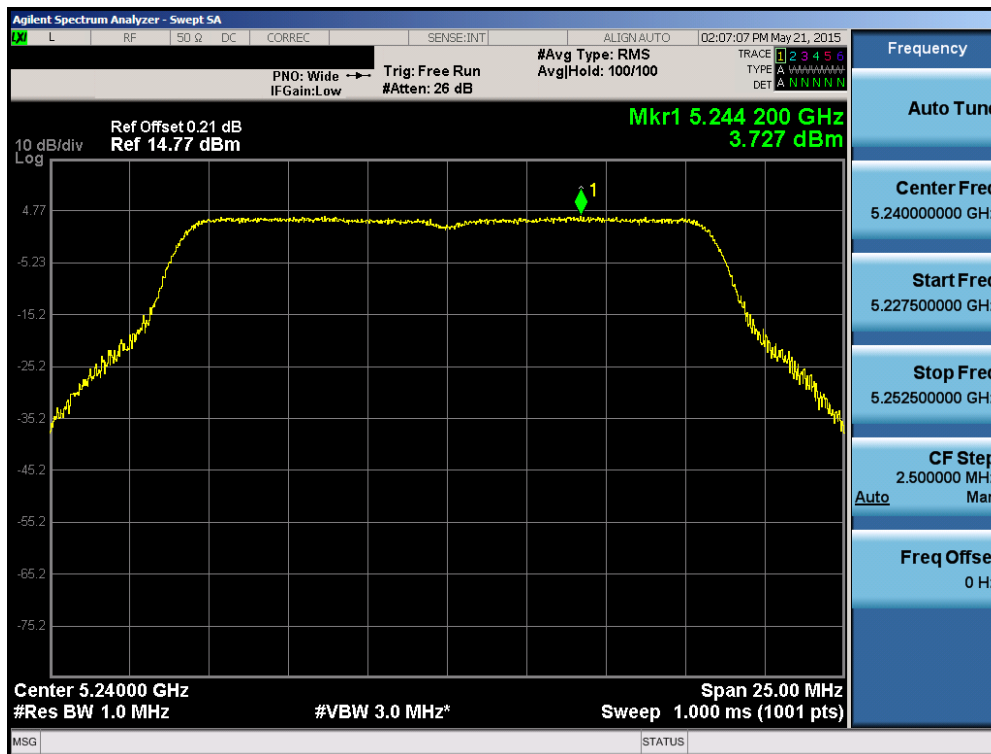
Plot 6-36. Power Spectral Density Plot (802.11a (UNII Band 1) – Ch. 48)
