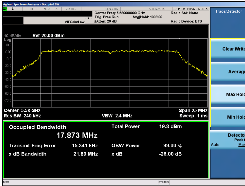
Plot 6-21. 26dB Bandwidth Plot (20MHz BW 802.11n (UNII Band 2C) – Ch. 116)
