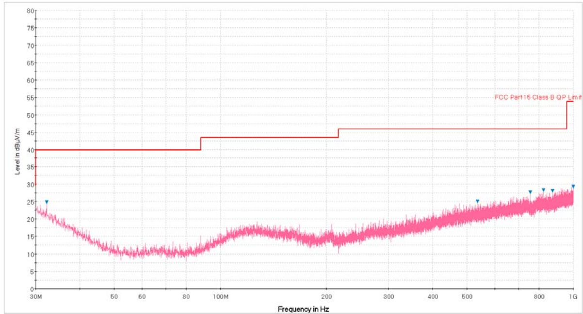
Plot 6-95. Radiated Spurious Plot below 1GHz (802.11a – U3 Ch. 157, Ant. Pol. H)
