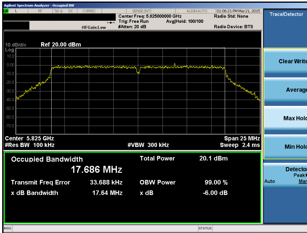
Plot 6-31. 6dB Bandwidth Plot (20MHz BW 802.11n (UNII Band 3) – Ch. 165)
