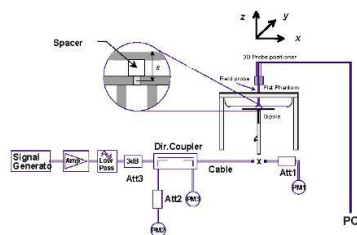
Figure 8-1 System Verification Setup Diagram
