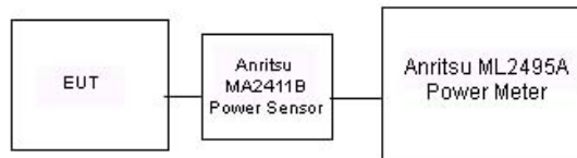
Figure 7-1 Power Measurement Setup
