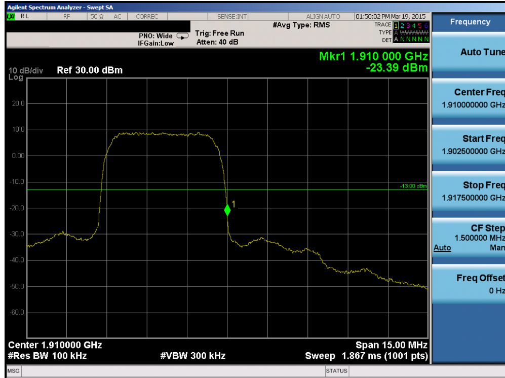
Plot 6-39. Band Edge Plot (PCS WCDMA Mode – Ch. 9538)
