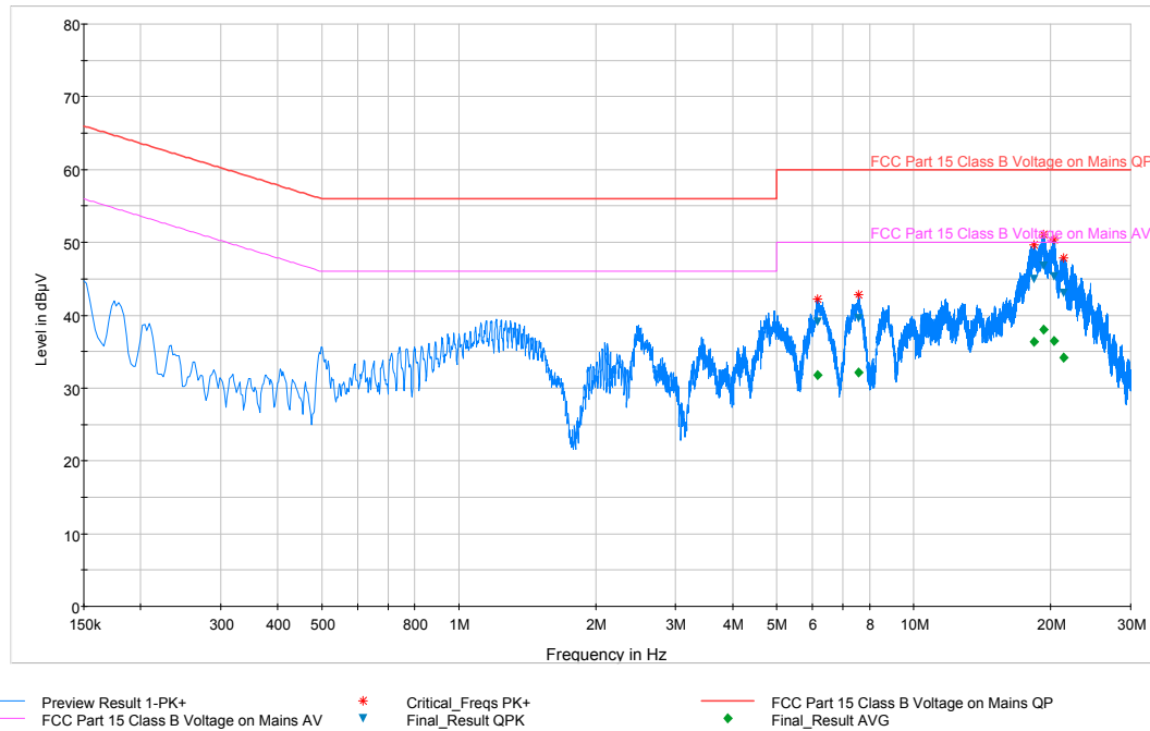
Plot 6-98. Line Conducted Plot with 802.11a UNII Band 3 (N)
