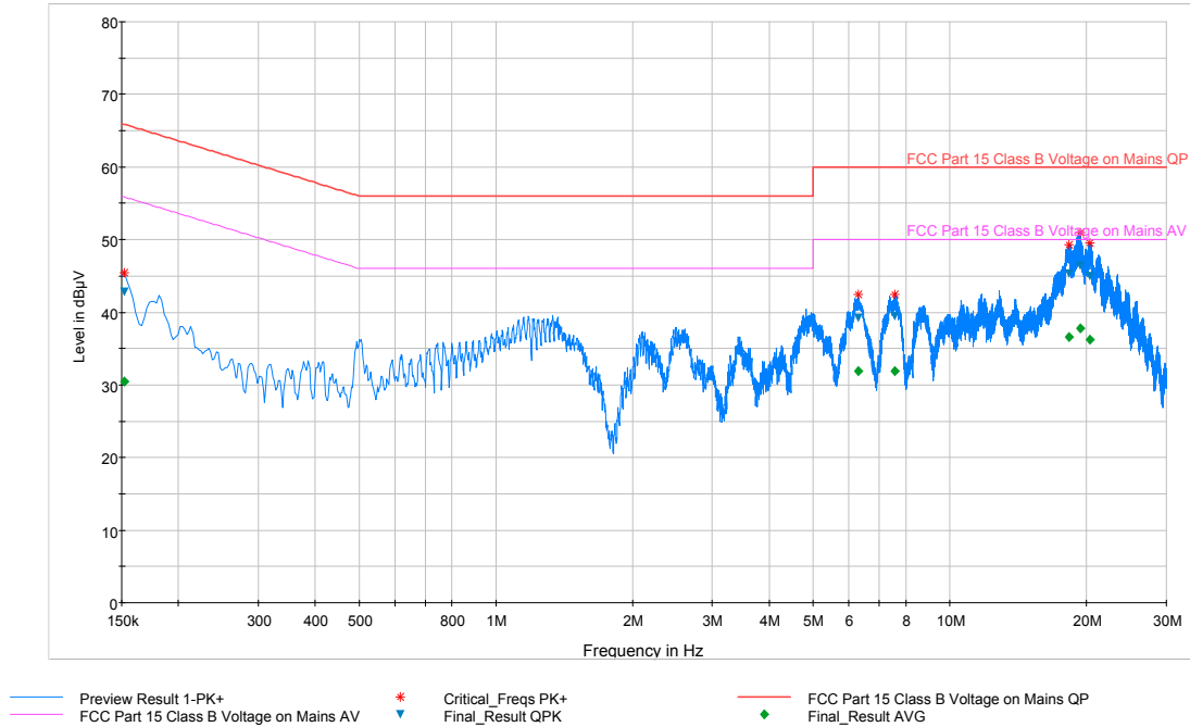
Plot 6-92. Line Conducted Plot with 802.11a UNII Band 1 (N)
