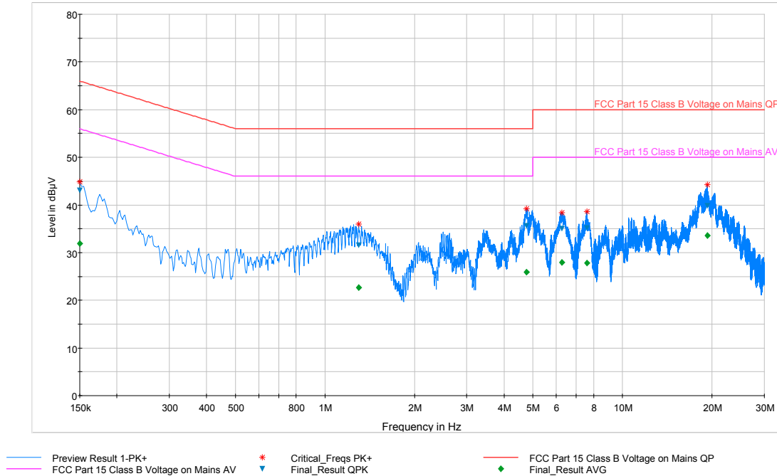
Plot 6-91. Line Conducted Plot with 802.11a UNII Band 1 (L1)
