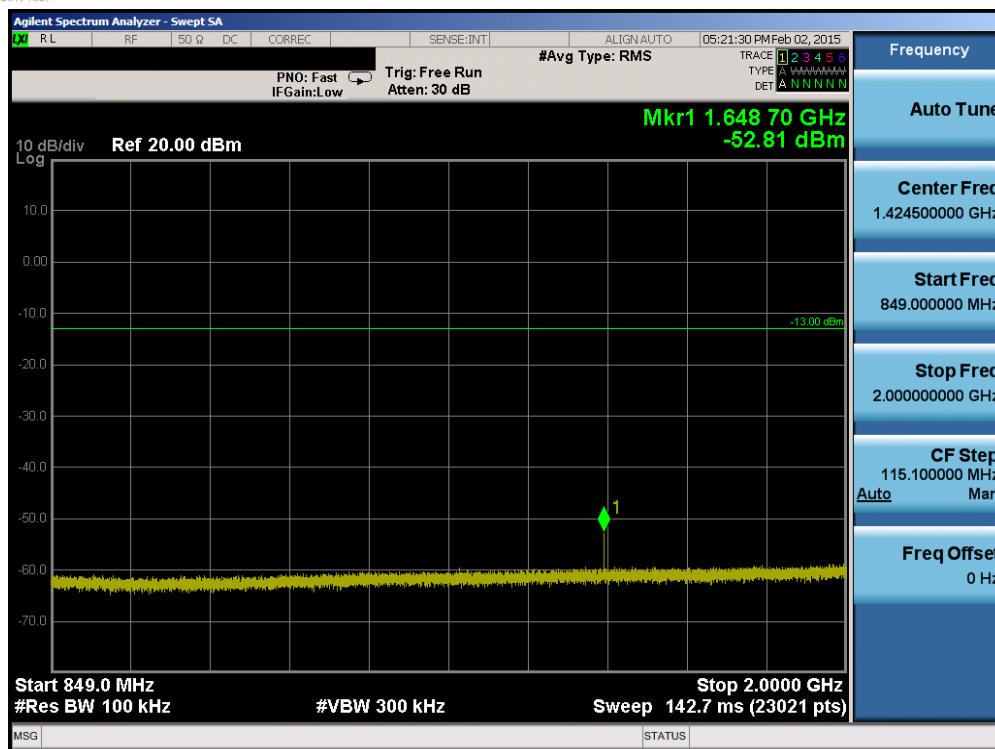
Plot 6-59. Conducted Spurious Plot (Band 5 – 5.0MHz QPSK – RB Size 1, RB Offset 0 – Low Channel)
