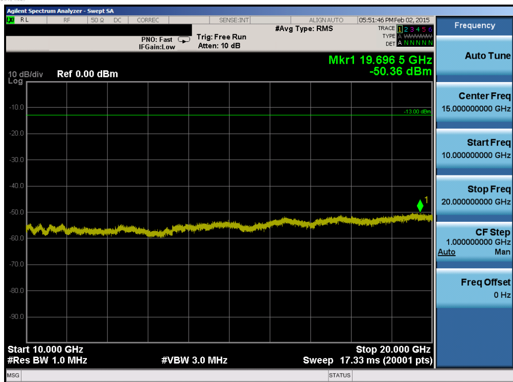
Plot 6-81. Conducted Spurious Plot (Band 25 – 5.0MHz QPSK – RB Size 1, RB Offset 0 – Mid Channel)
