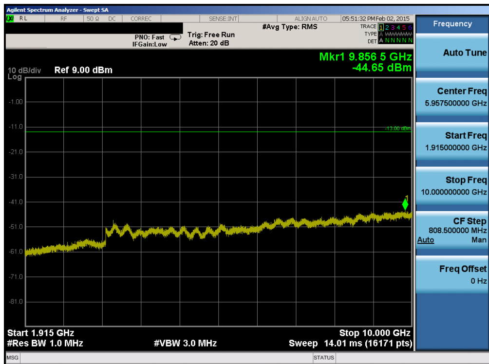
Plot 6-80. Conducted Spurious Plot (Band 25 – 5.0MHz QPSK – RB Size 1, RB Offset 0 – Mid Channel)
