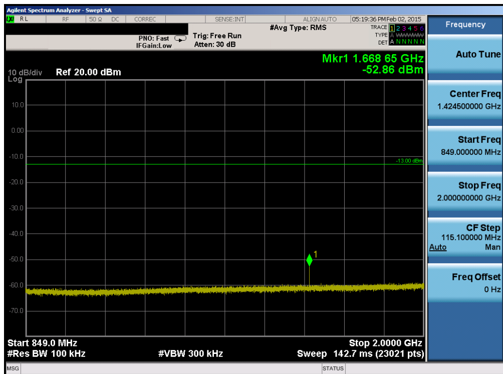
Plot 6-62. Conducted Spurious Plot (Band 5 – 5.0MHz QPSK – RB Size 1, RB Offset 0 – Mid Channel)
