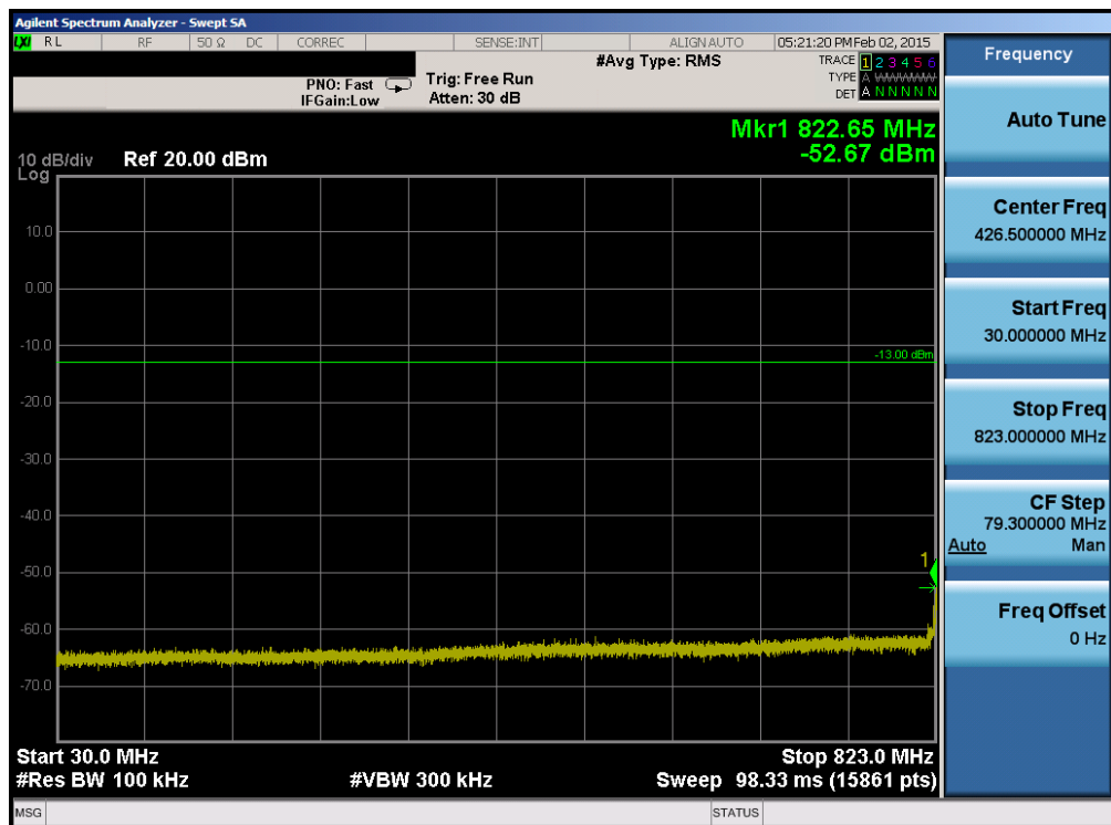
Plot 6-58. Conducted Spurious Plot (Band 5 – 5.0MHz QPSK – RB Size 1, RB Offset 0 – Low Channel)
