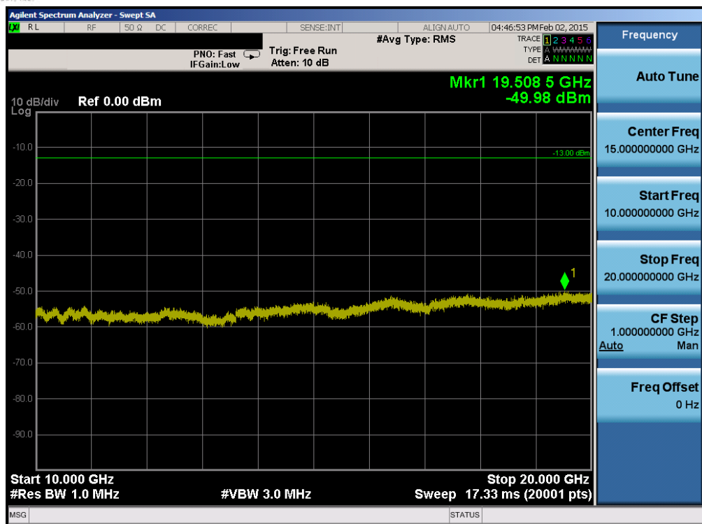
Plot 6-69. Conducted Spurious Plot (Band 4 – 5.0MHz QPSK – RB Size 1, RB Offset 0 – Low Channel)
