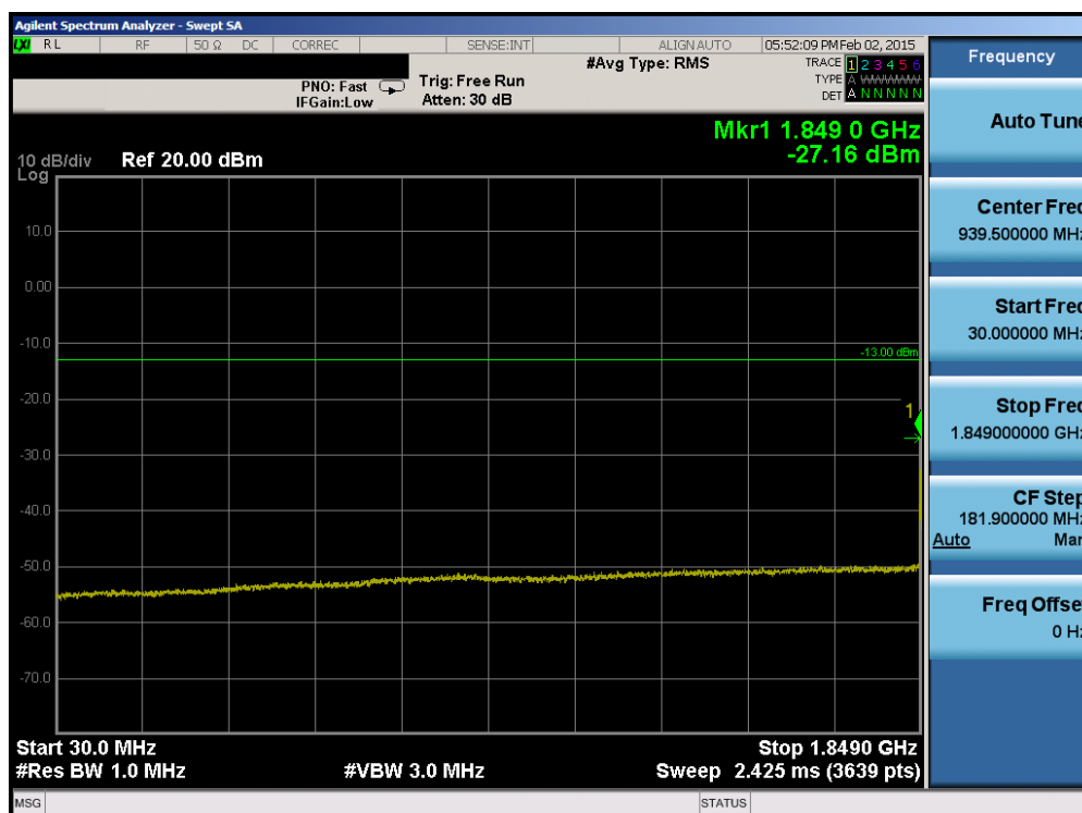
Plot 6-76. Conducted Spurious Plot (Band 25 – 5.0MHz QPSK – RB Size 1, RB Offset 0 – Low Channel)
