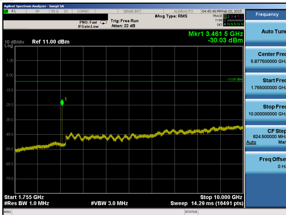
Plot 6-71. Conducted Spurious Plot (Band 4 – 5.0MHz QPSK – RB Size 1, RB Offset 0 – Mid Channel)
