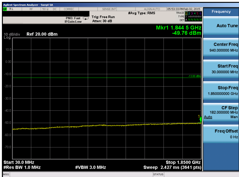
Plot 6-82. Conducted Spurious Plot (Band 25 – 5.0MHz QPSK – RB Size 1, RB Offset 0 – High Channel)
