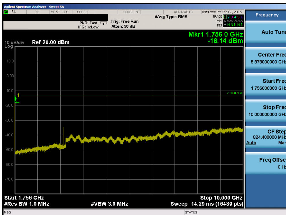
Plot 6-74. Conducted Spurious Plot (Band 4 – 5.0MHz QPSK – RB Size 1, RB Offset 0 – High Channel)
