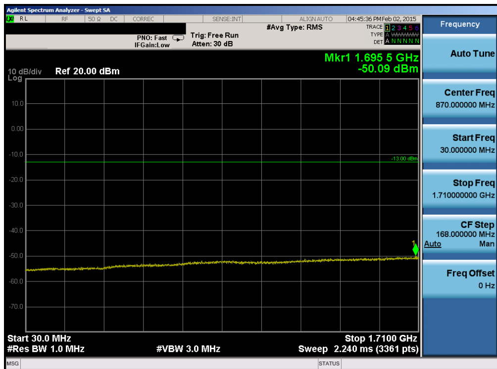
Plot 6-70. Conducted Spurious Plot (Band 4 – 5.0MHz QPSK – RB Size 1, RB Offset 0 – Mid Channel)
