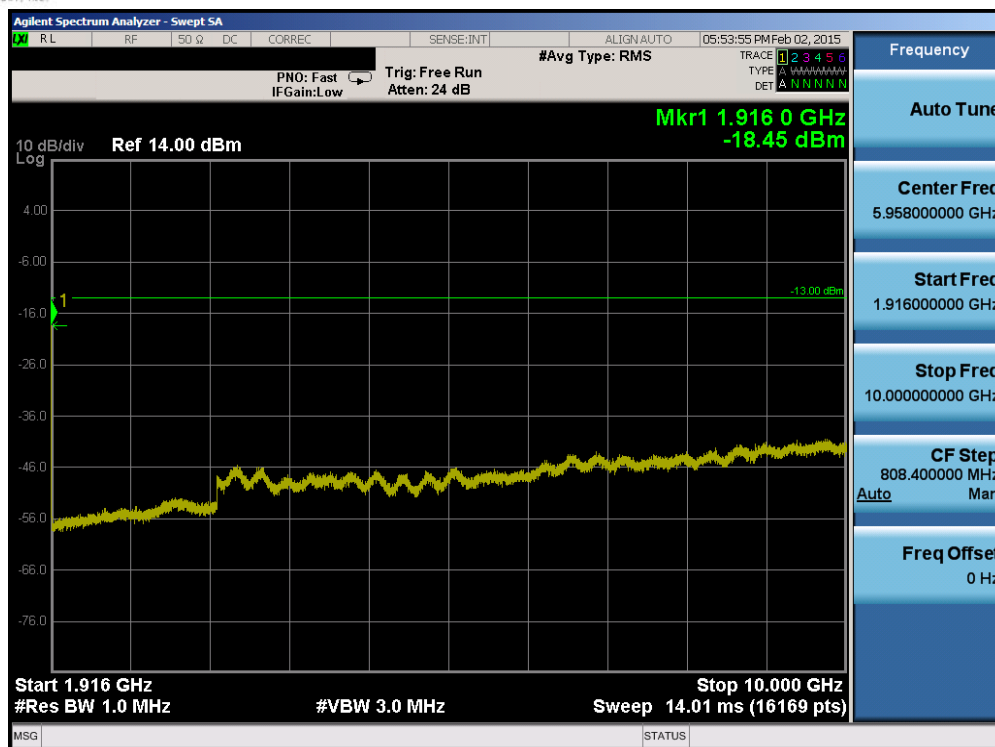
Plot 6-83. Conducted Spurious Plot (Band 25 – 5.0MHz QPSK – RB Size 1, RB Offset 0 – High Channel)
