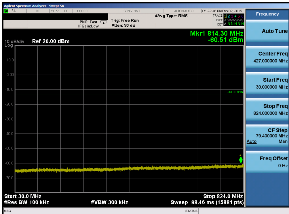
Plot 6-64. Conducted Spurious Plot (Band 5 – 5.0MHz QPSK – RB Size 1, RB Offset 0 – High Channel)
