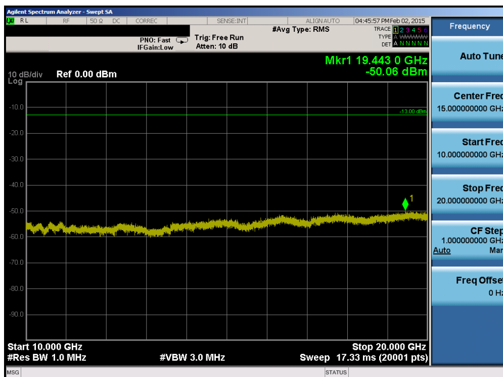
Plot 6-72. Conducted Spurious Plot (Band 4 – 5.0MHz QPSK – RB Size 1, RB Offset 0 – Mid Channel)
