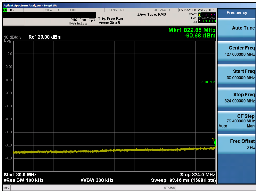
Plot 6-61. Conducted Spurious Plot (Band 5 – 5.0MHz QPSK – RB Size 1, RB Offset 0 – Mid Channel)
