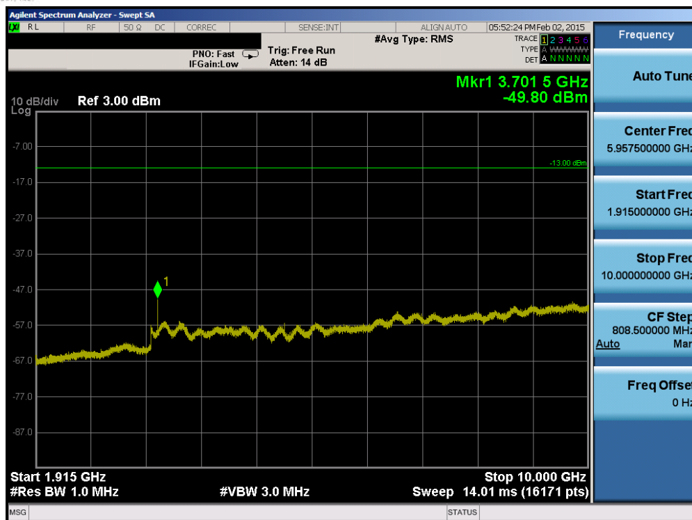
Plot 6-77. Conducted Spurious Plot (Band 25 – 5.0MHz QPSK – RB Size 1, RB Offset 0 – Low Channel)
