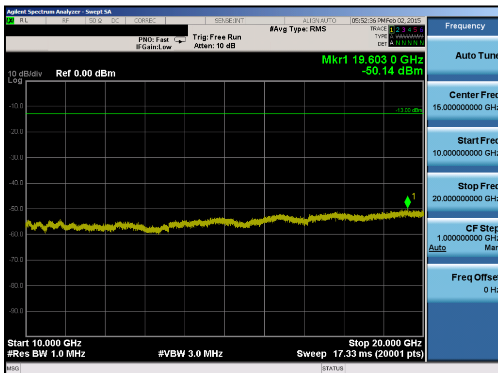
Plot 6-78. Conducted Spurious Plot (Band 25 – 5.0MHz QPSK – RB Size 1, RB Offset 0 – Low Channel)
