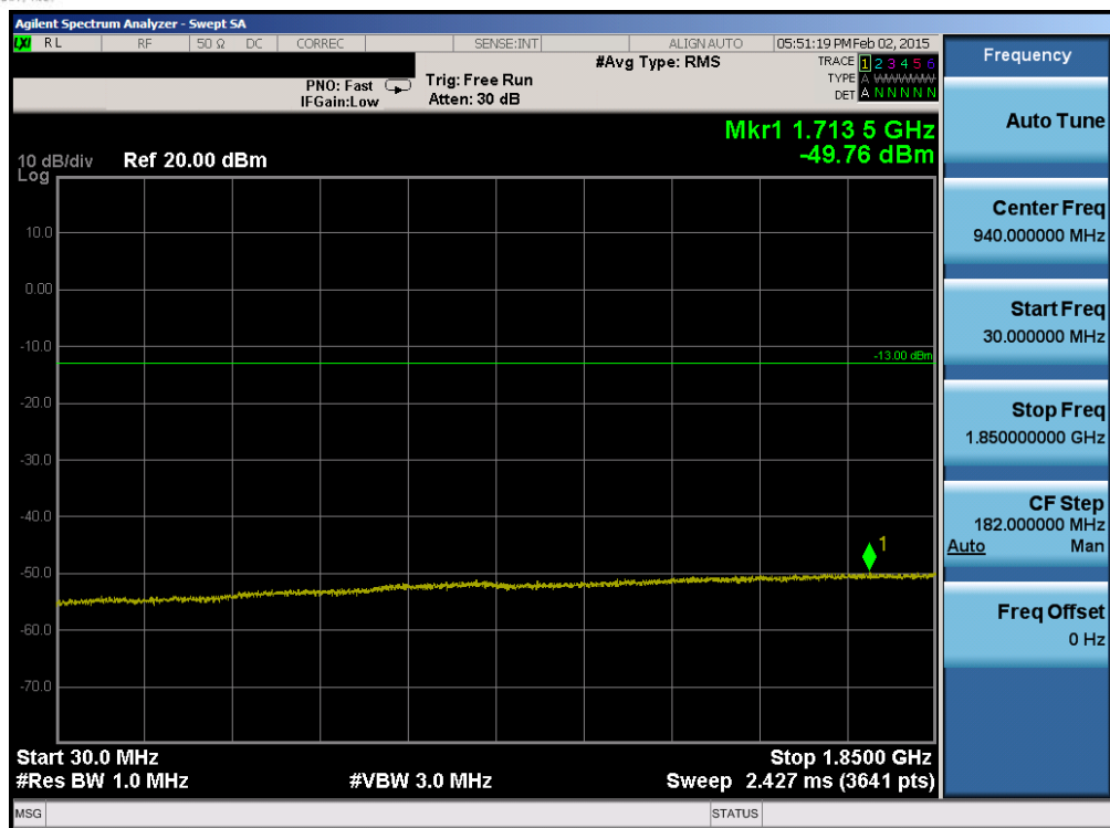
Plot 6-79. Conducted Spurious Plot (Band 25 – 5.0MHz QPSK – RB Size 1, RB Offset 0 – Mid Channel)
