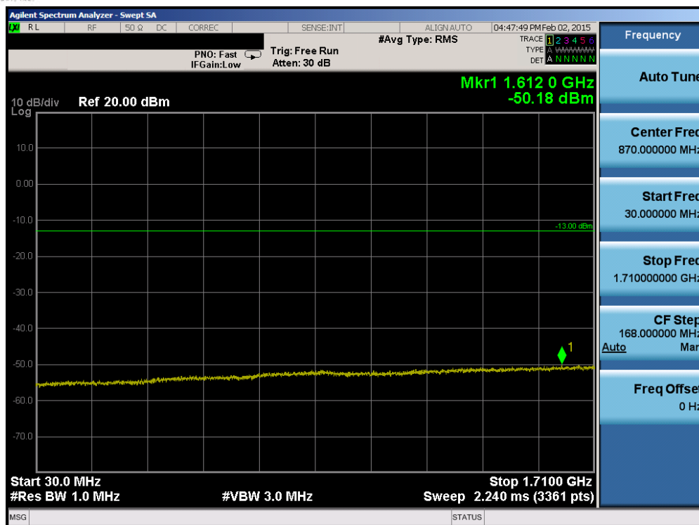
Plot 6-73. Conducted Spurious Plot (Band 4 – 5.0MHz QPSK – RB Size 1, RB Offset 0 – High Channel)
