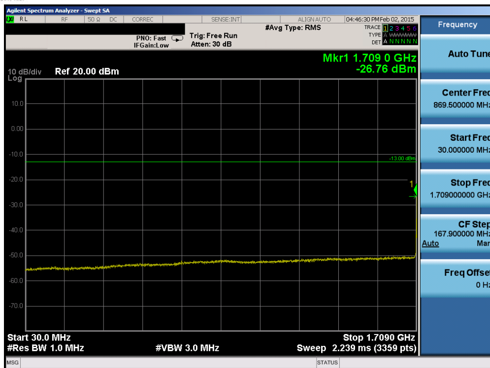
Plot 6-67. Conducted Spurious Plot (Band 4 – 5.0MHz QPSK – RB Size 1, RB Offset 0 – Low Channel)
