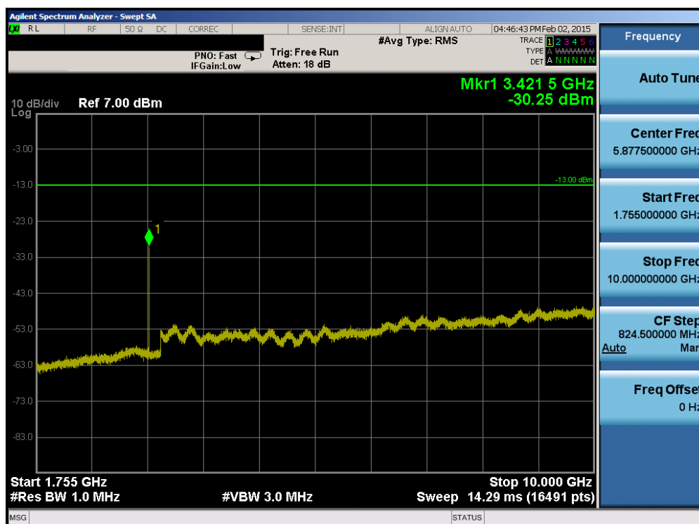
Plot 6-68. Conducted Spurious Plot (Band 4 – 5.0MHz QPSK – RB Size 1, RB Offset 0 – Low Channel)
