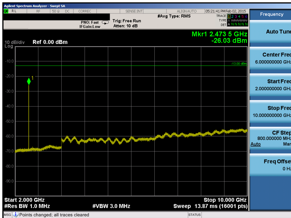
Plot 6-60. Conducted Spurious Plot (Band 5 – 5.0MHz QPSK – RB Size 1, RB Offset 0 – Low Channel)
