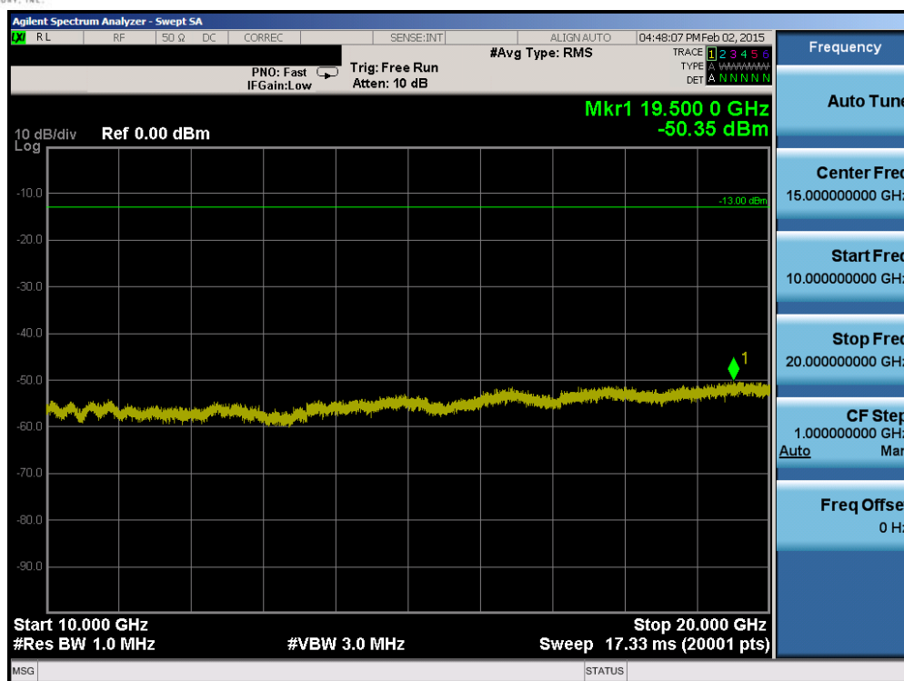
Plot 6-75. Conducted Spurious Plot (Band 4 – 5.0MHz QPSK – RB Size 1, RB Offset 0 – High Channel)
