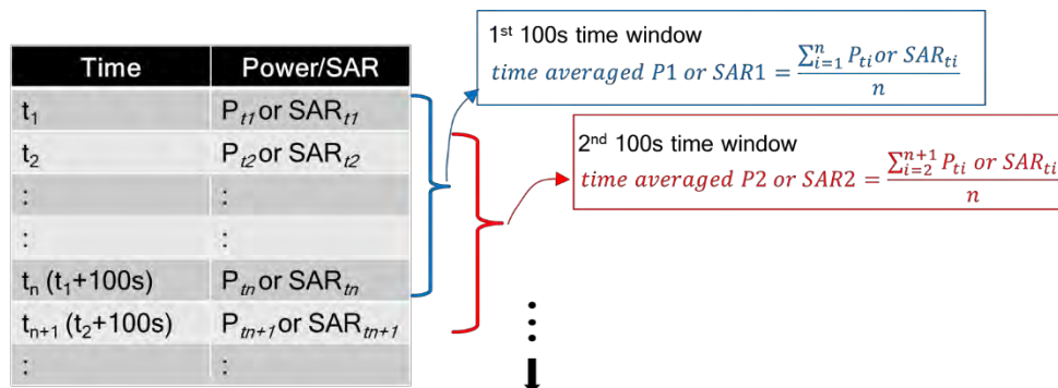
Figure 6-1: Running time averaging illustration
