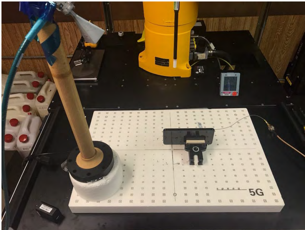
Figure 9-1 Worst-case surface of EUT positioned facing up for the mmW beam being tested
