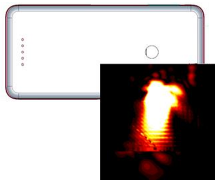
(b) Simulation(0mm)
