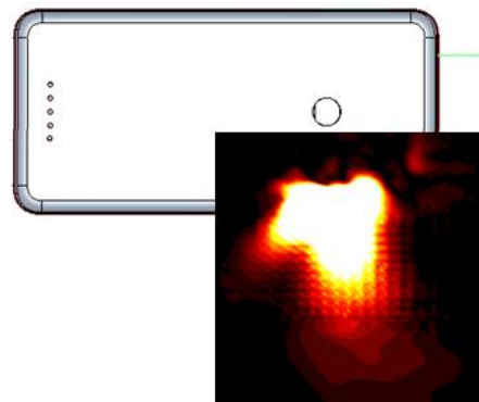
(b) Simulation(0mm)
