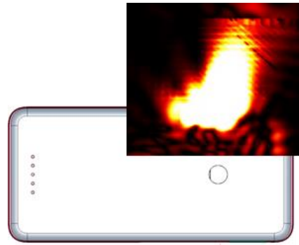
(b) Simulation(0mm)
