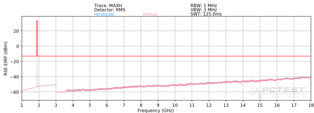
Plot 7-4. Radiated Spurious Plot above 1GHz (PCS WCDMA Mode)
