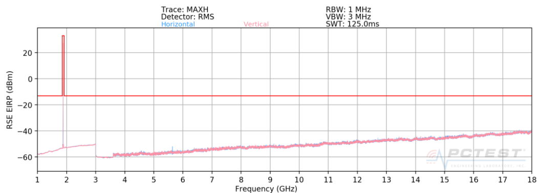
Plot 7-3. Radiated Spurious Plot above 1GHz (PCS GPRS Mode)
