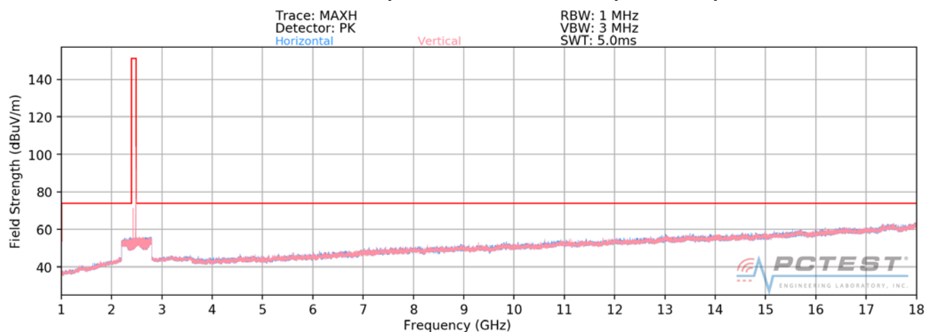
Plot 7-3. Radiated Spurious Plot above 1GHz (BT- Ch. 78)
