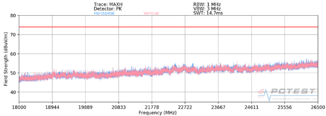
Plot 7-4. Radiated Spurious Plot above 18GHz
