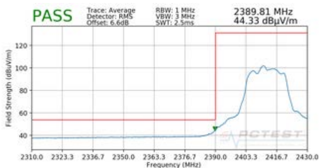
Plot 7-25. Radiated Restricted Lower Band Edge Measurement CDD (Average)
