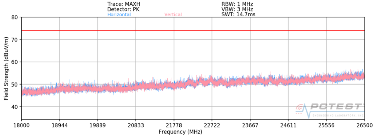
Plot 7-4. Radiated Spurious Plot above 18GHz SISO ANT1
