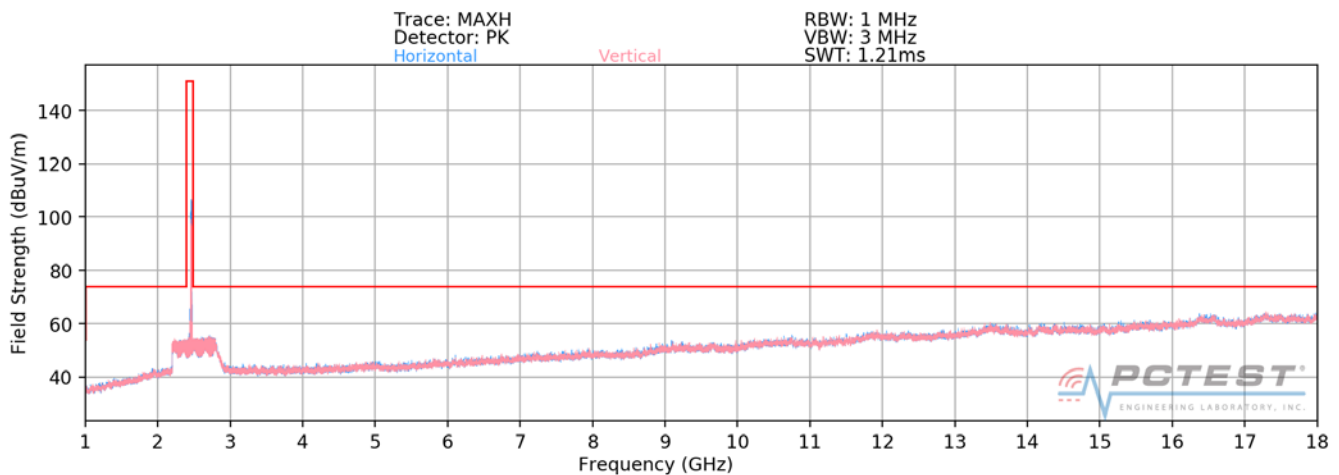
Plot 7-11. Radiated Spurious Plot above 1GHz MIMO/CDD (802.11g – Ch. 11)
