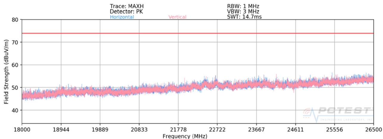
Plot 7-8. Radiated Spurious Plot above 18GHz SISO ANT2
