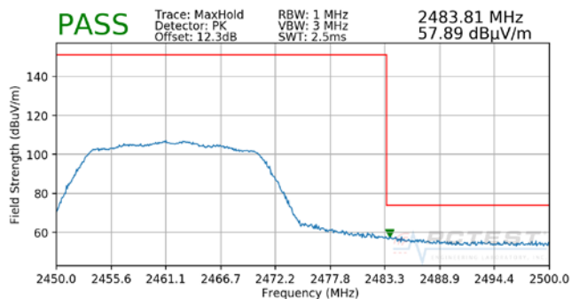
Plot 7-24. Radiated Restricted Band Edge Measurement SISO ANT2 with WCP (Peak)
