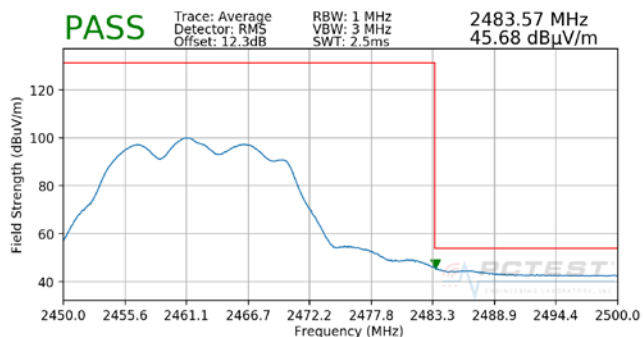
Plot 7-29. Radiated Restricted Band Edge Measurement CDD with WCP (Average)
