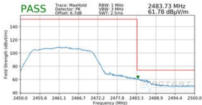
Plot 7-34. Radiated Restricted Upper Band Edge Measurement SDM (Peak)
