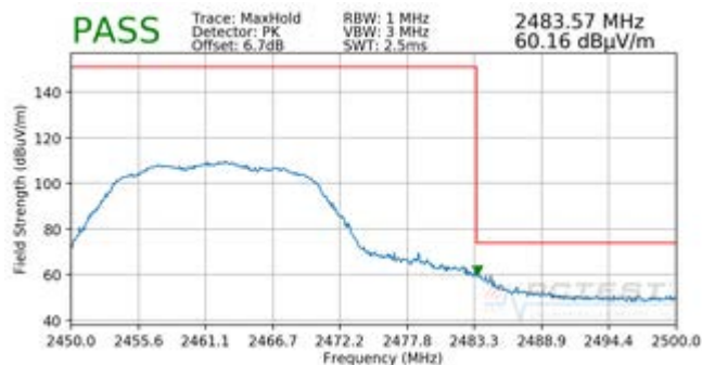
Plot 7-28. Radiated Restricted Upper Band Edge Measurement CDD (Peak)
