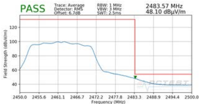
Plot 7-33. Radiated Restricted Upper Band Edge Measurement SDM (Average)
