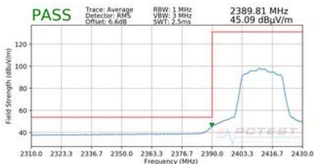
Plot 7-13. Radiated Restricted Lower Band Edge Measurement SISO ANT1 (Average)
