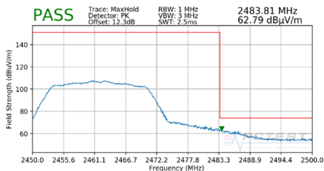
Plot 7-18. Radiated Restricted Band Edge Measurement SISO ANT1 with WCP (Peak)
