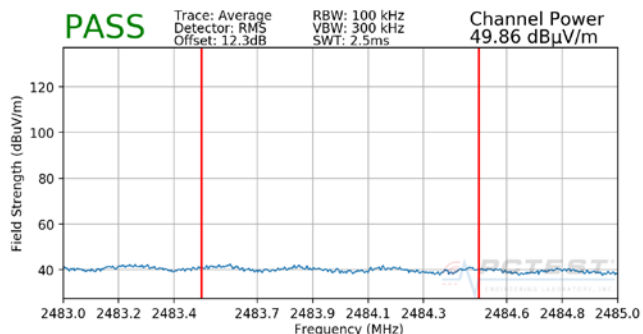
Plot 7-15. Radiated Restricted Upper Band Edge Measurement SISO ANT1 (Average)
