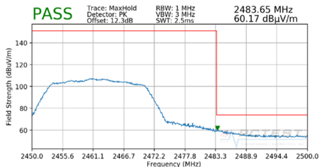
Plot 7-36. Radiated Restricted Band Edge Measurement SDM with WCP (Peak)
