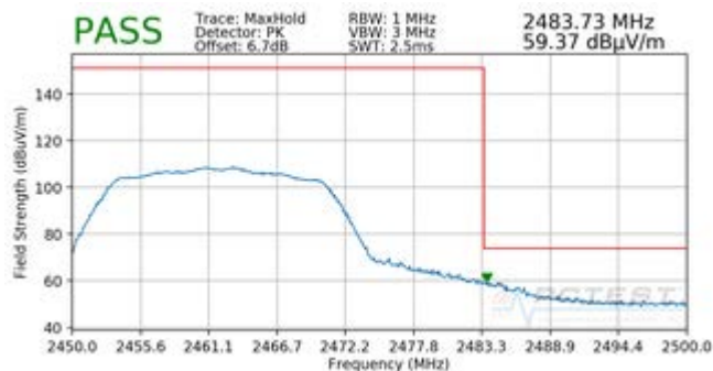
Plot 7-22. Radiated Restricted Upper Band Edge Measurement SISO ANT2 (Peak)
