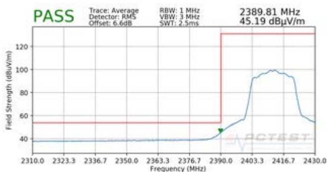
Plot 7-31. Radiated Restricted Lower Band Edge Measurement SDM (Average)
