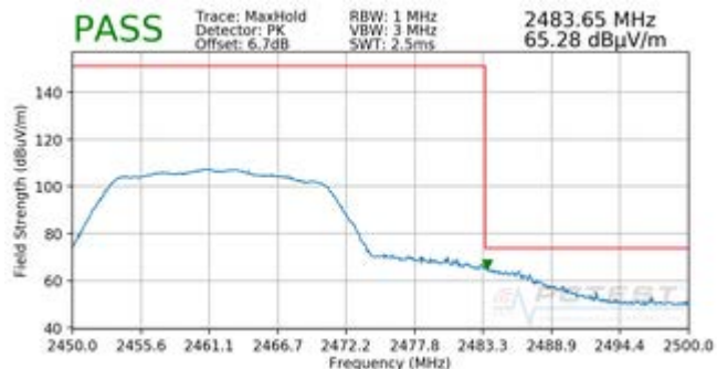
Plot 7-16. Radiated Restricted Upper Band Edge Measurement SISO ANT1 (Peak)
