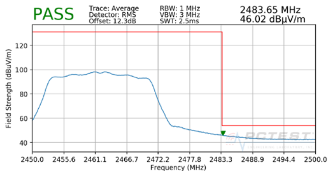
Plot 7-23. Radiated Restricted Band Edge Measurement SISO ANT2 with WCP (Average)
