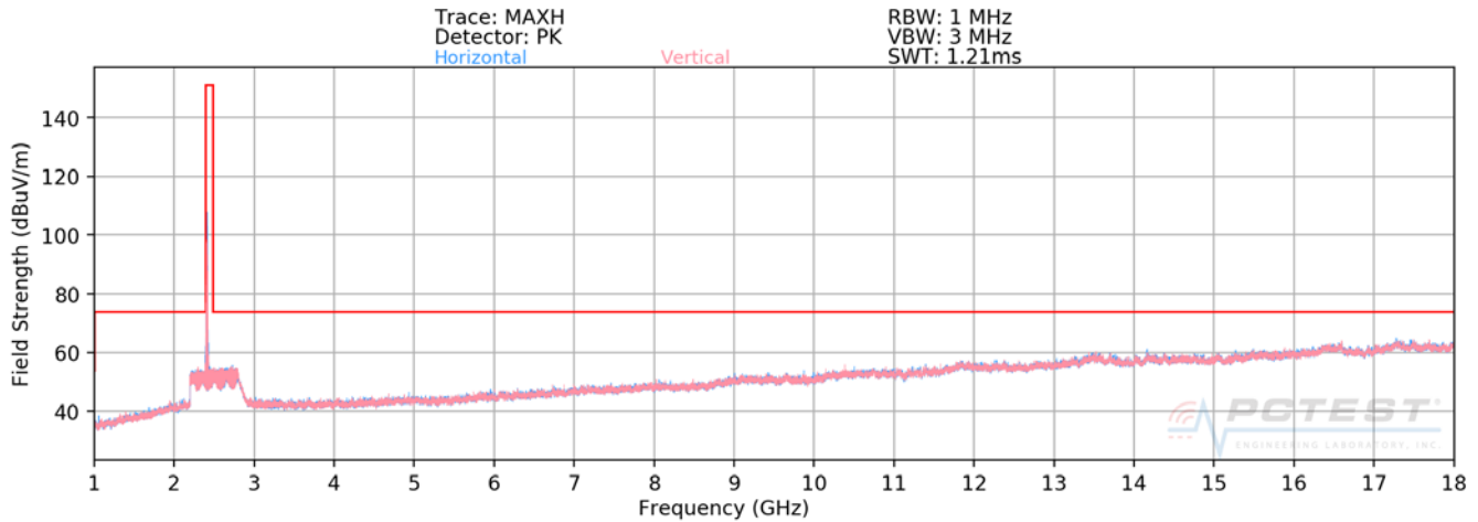
Plot 7-9. Radiated Spurious Plot above 1GHz MIMO/CDD (802.11g – Ch. 1)
