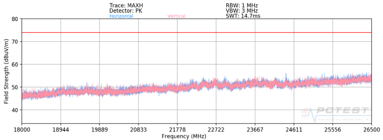
Plot 7-12. Radiated Spurious Plot above 18GHz MIMO/CDD
