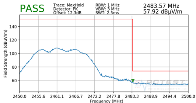
Plot 7-30. Radiated Restricted Band Edge Measurement CDD with WCP (Peak)
