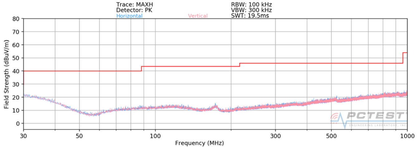
Plot 7-38. Radiated Spurious Plot below 1GHz SISO ANT2
