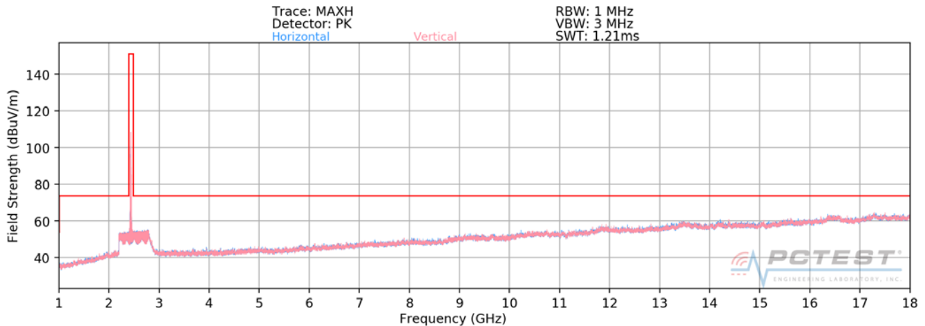
Plot 7-10. Radiated Spurious Plot above 1GHz MIMO/CDD (802.11g – Ch. 6)
