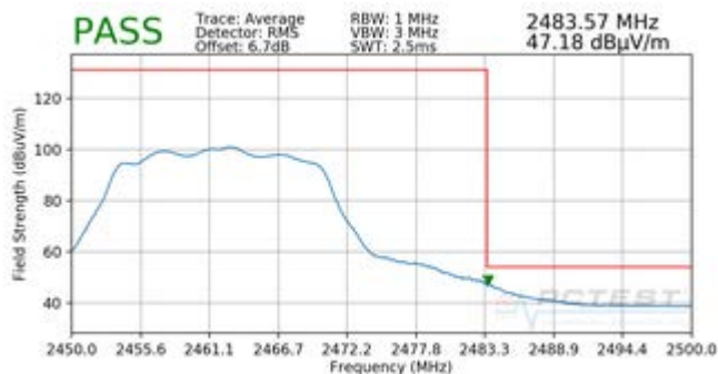
Plot 7-27. Radiated Restricted Upper Band Edge Measurement CDD (Average)
