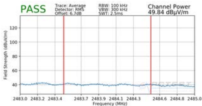
Plot 7-17. Radiated Restricted Band Edge Measurement SISO ANT1 with WCP (Average)
