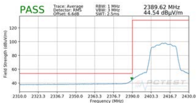
Plot 7-19. Radiated Restricted Lower Band Edge Measurement SISO ANT2 (Average)
