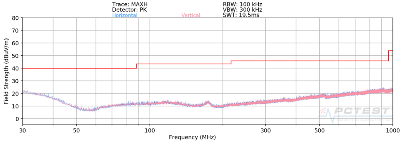
Plot 7-37. Radiated Spurious Plot below 1GHz SISO ANT1
