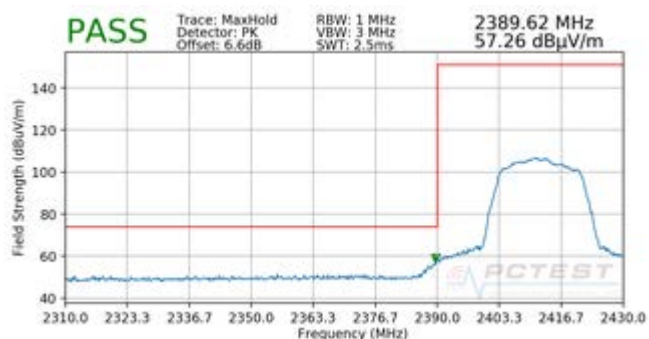
Plot 7-14. Radiated Restricted Lower Band Edge Measurement SISO ANT1 (Peak)
