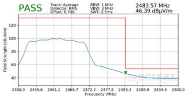
Plot 7-21. Radiated Restricted Upper Band Edge Measurement SISO ANT2 (Average)
