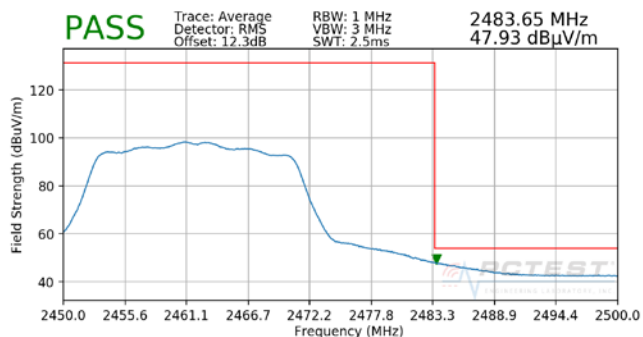
Plot 7-35. Radiated Restricted Band Edge Measurement SDM with WCP (Average)
