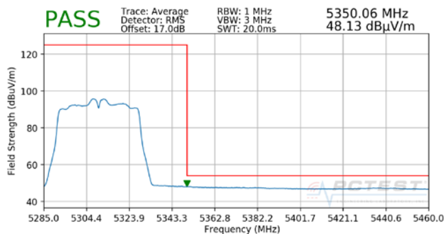
Plot 7-41. Radiated Band Edge Plot (Average – WCP)
