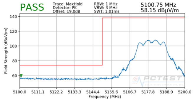
Plot 7-79. Radiated Lower Band Edge Plot MIMO (Peak – UNII Band 1)
