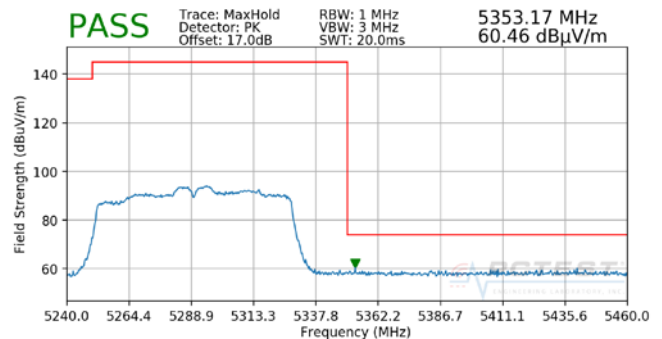
Plot 7-72. Radiated Upper Band Edge Plot SISO ANT2 (Peak – UNII Band 2A)
