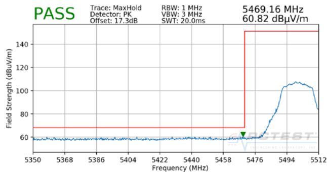
Plot 7-33. Radiated Band Edge Plot (Peak – WCP)
