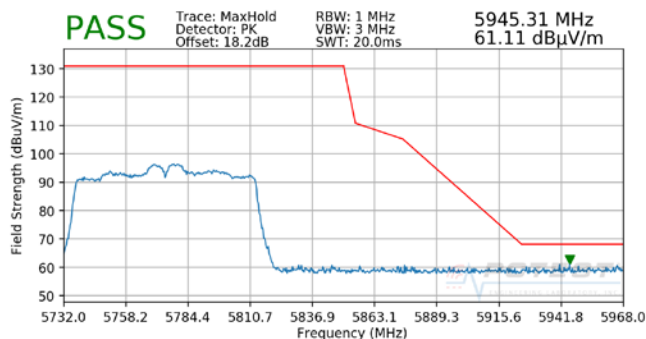
Plot 7-75. Radiated Upper Band Edge Plot SISO ANT2 (Peak – UNII Band 3)
