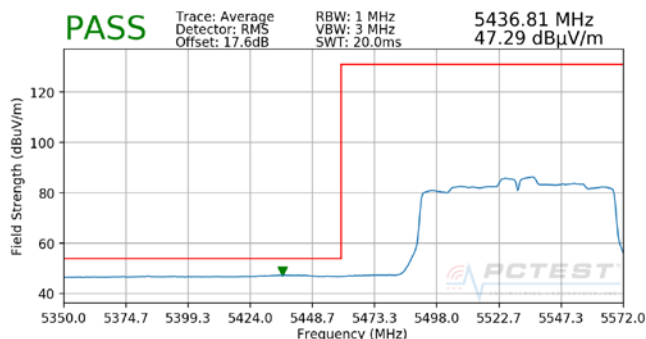
Plot 7-73. Radiated Lower Band Edge Plot SISO ANT2 (Average – UNII Band 2C)
