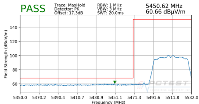
Plot 7-65. Radiated Lower Band Edge Plot SISO ANT2 (Peak - UNII Band 2C)
