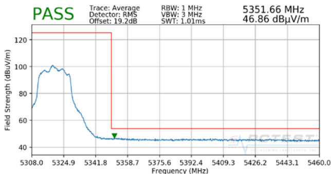
Plot 7-80. Radiated Upper Band Edge Plot MIMO (Average – UNII Band 2A)
