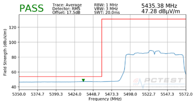
Plot 7-50. Radiated Band Edge Plot (Average – WCP)
