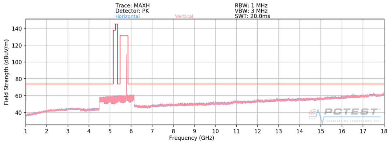
Plot 7-10. Radiated Spurious Plot above 1GHz SISO ANT2 (802.11a – U3 Ch. 157)
