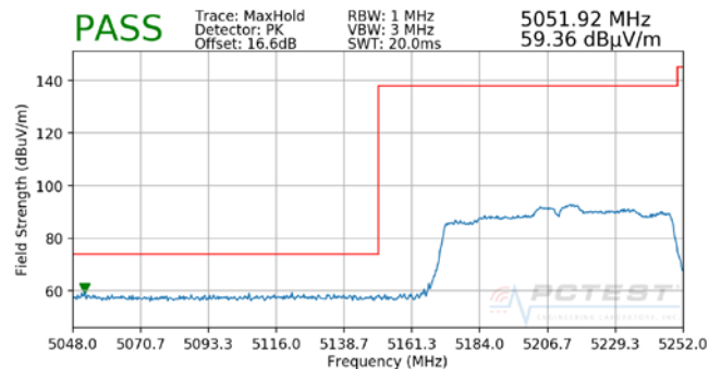
Plot 7-70. Radiated Lower Band Edge Plot SISO ANT2 (Peak – UNII Band 1)
