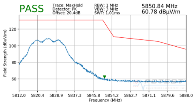
Plot 7-84. Radiated Upper Band Edge Plot MIMO (Peak – UNII Band 3)
