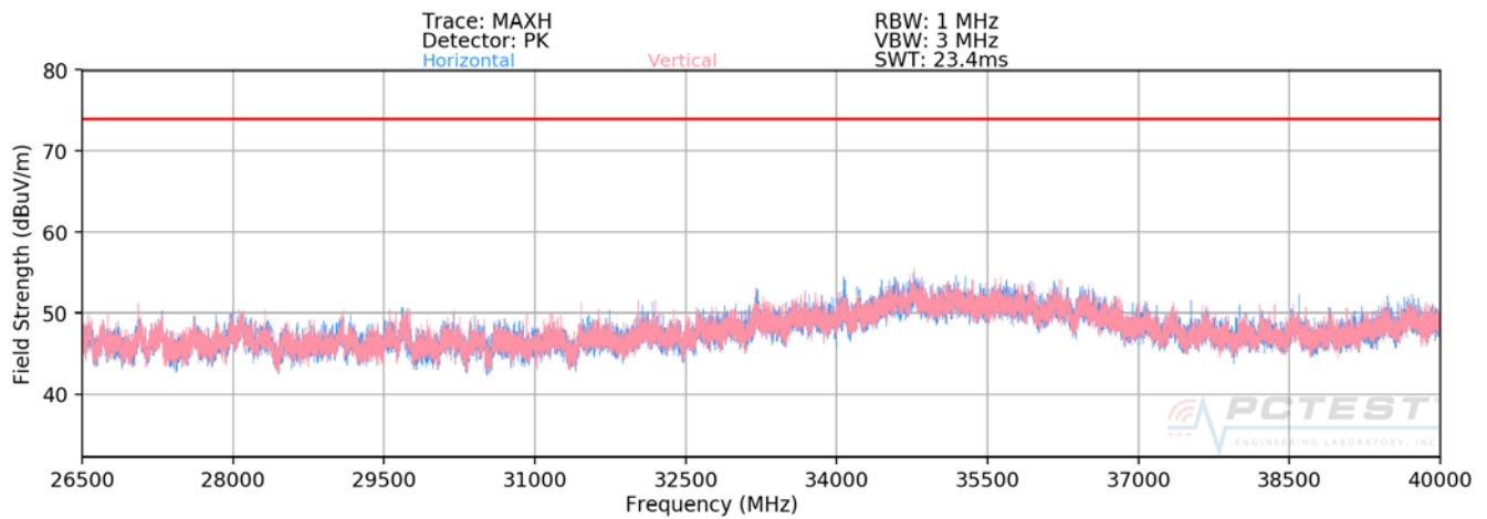
Plot 7-24. Radiated Spurious Plot above 26.5GHz (Dual Band Simult. Tx)
