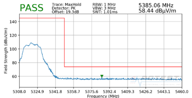
Plot 7-81. Radiated Upper Band Edge Plot MIMO (Peak – UNII Band 2A)
