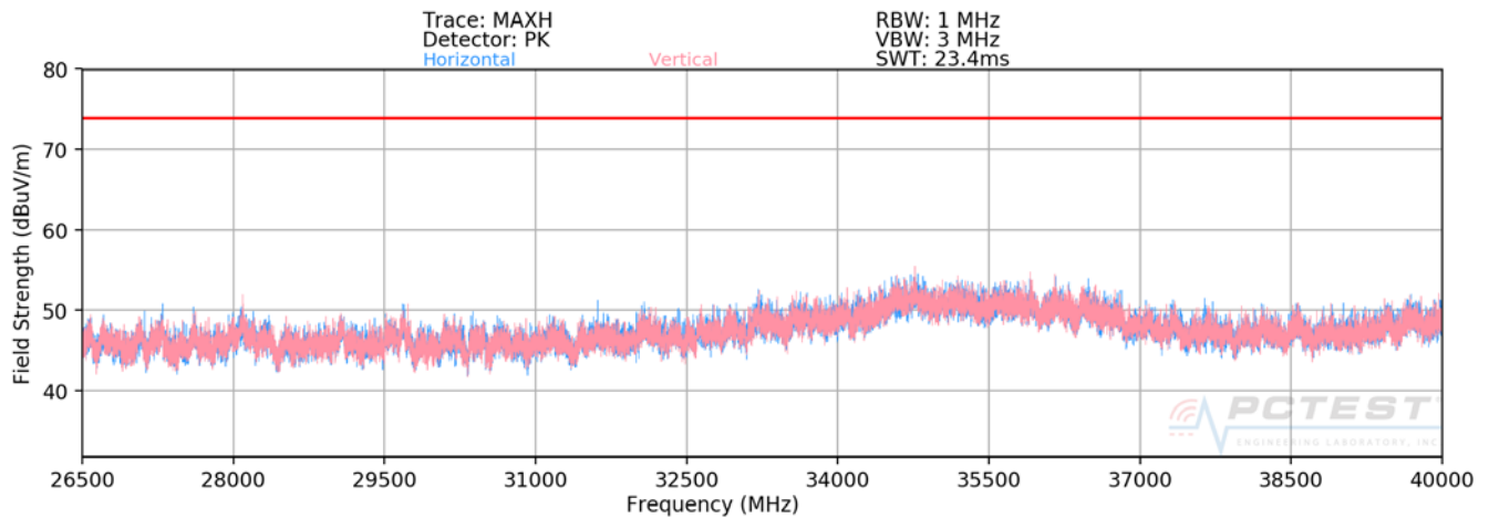
Plot 7-20. Radiated Spurious Plot 26.5GHz - 40GHz MIMO/CDD (802.11a)
