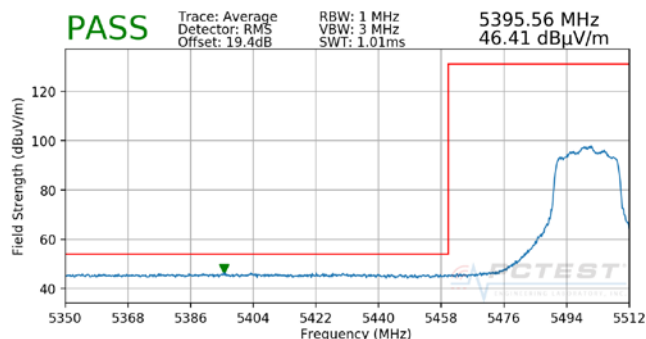
Plot 7-91. Radiated Lower Band Edge Plot MIMO (Average – UNII Band 2C)
