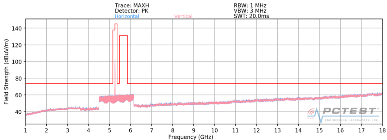
Plot 7-8. Radiated Spurious Plot above 1GHz SISO ANT2 (802.11a – U2A Ch. 56)
