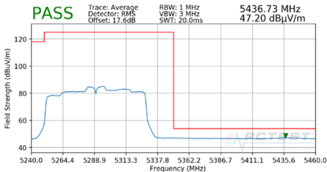
Plot 7-71. Radiated Upper Band Edge Plot SISO ANT2 (Average – UNII Band 2A)
