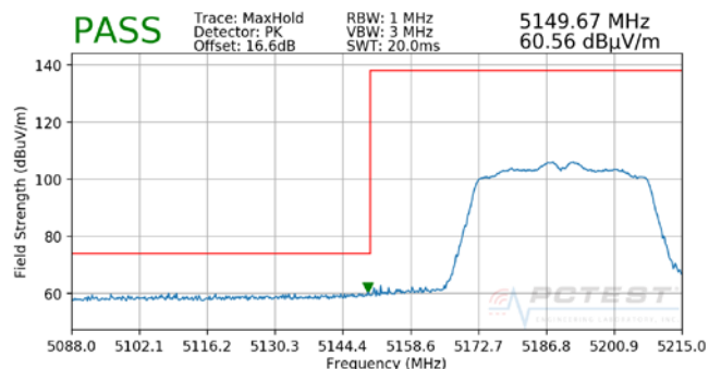
Plot 7-35. Radiated Lower Band Edge Plot (Peak – UNII Band 1)
