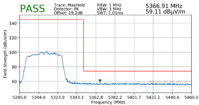
Plot 7-104. Radiated Band Edge Plot ANT (Peak – WCP)
