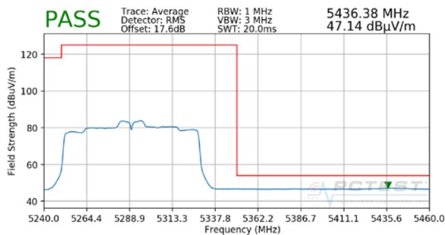
Plot 7-76. Radiated Band Edge Plot SISO ANT2 (Average – WCP)
