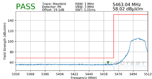
Plot 7-92. Radiated Lower Band Edge Plot MIMO (Peak – UNII Band 2C)
