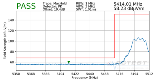
Plot 7-83. Radiated Lower Band Edge Plot MIMO (Peak – UNII Band 2C)
