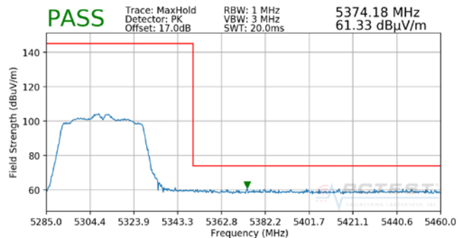
Plot 7-37. Radiated Upper Band Edge Plot (Peak – UNII Band 2A)
