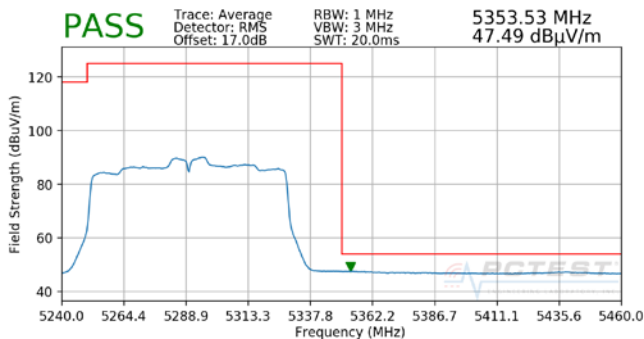
Plot 7-45. Radiated Upper Band Edge Plot (Average – UNII Band 2A)
