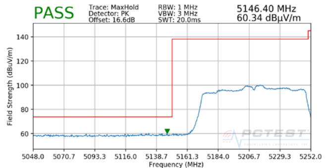
Plot 7-44. Radiated Lower Band Edge Plot (Peak – UNII Band 1)
