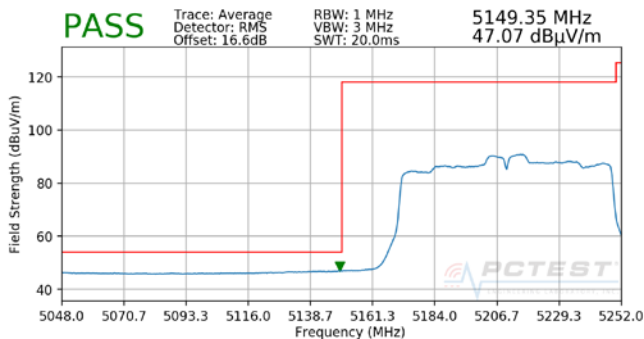
Plot 7-43. Radiated Lower Band Edge Plot (Average – UNII Band 1)
