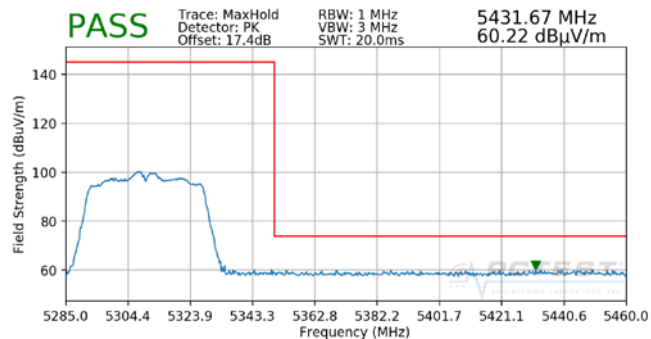
Plot 7-63. Radiated Upper Band Edge Plot SISO ANT2 (Peak – UNII Band 2A)
