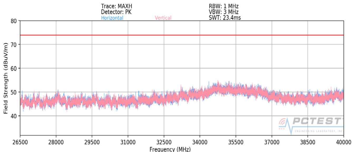
Plot 7-6. Radiated Spurious Plot 26.5GHz - 40GHz SISO ANT1 (802.11a)
