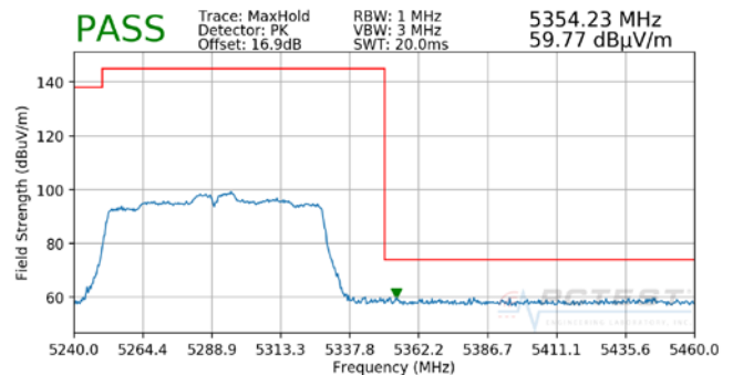
Plot 7-46. Radiated Upper Band Edge Plot (Peak – UNII Band 2A)
