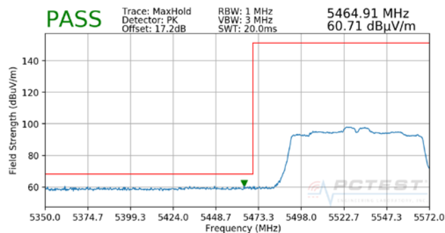
Plot 7-51. Radiated Band Edge Plot (Peak – WCP)
