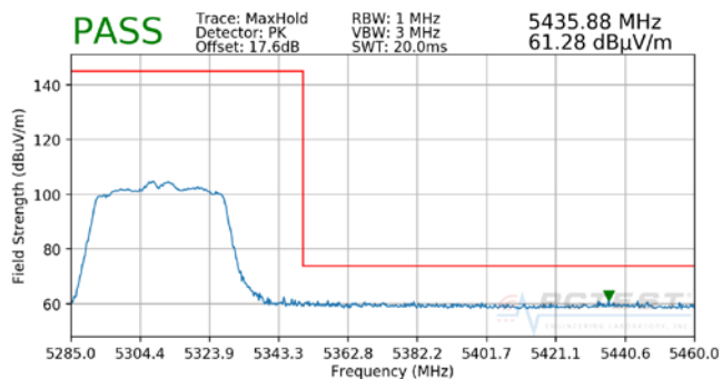
Plot 7-42. Radiated Band Edge Plot (Peak – WCP)
