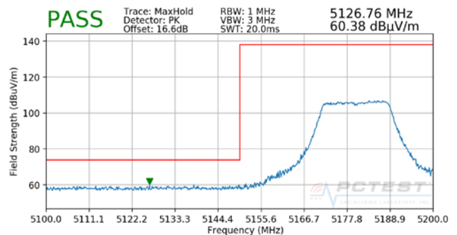
Plot 7-26. Radiated Lower Band Edge Plot (Peak – UNII Band 1)
