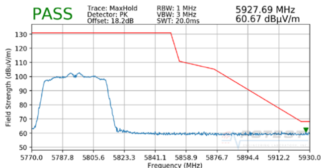
Plot 7-66. Radiated Upper Band Edge Plot SISO ANT2 (Peak - UNII Band 3)
