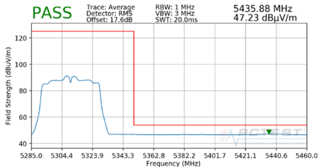
Plot 7-62. Radiated Upper Band Edge Plot SISO ANT2 (Average – UNII Band 2A)
