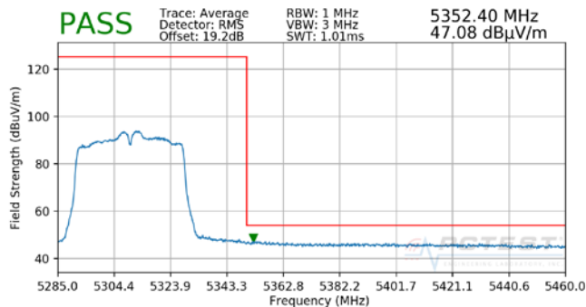
Plot 7-98. Radiated Upper Band Edge Plot MIMO (Average – UNII Band 2A)
