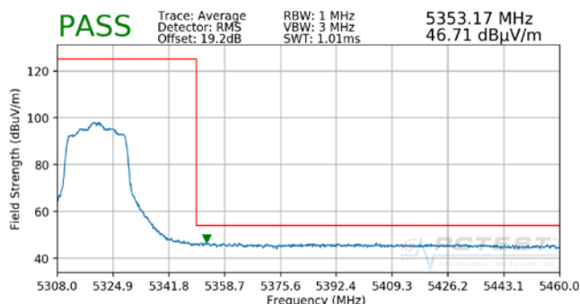
Plot 7-89. Radiated Upper Band Edge Plot MIMO (Average – UNII Band 2A)
