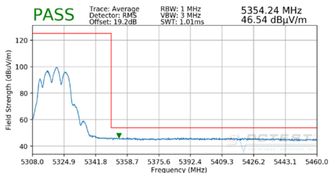
Plot 7-85. Radiated Band Edge Plot MIMO (Average – WCP)
