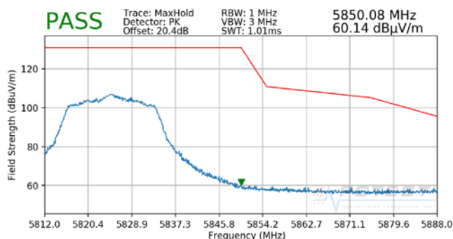
Plot 7-93. Radiated Upper Band Edge Plot MIMO (Peak – UNII Band 3)
