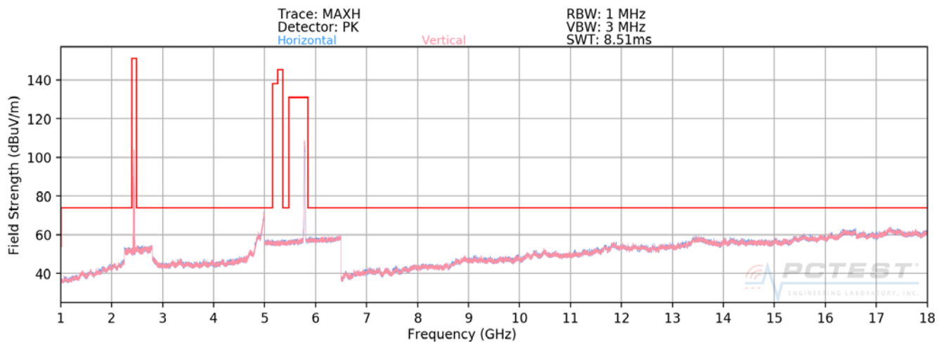
Plot 7-22. Radiated Spurious Plot above 1GHz (2.4GHz – 5GHz)
