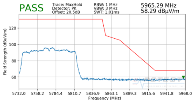
Plot 7-111. Radiated Upper Band Edge Plot MIMO (Peak – UNII Band 3)
