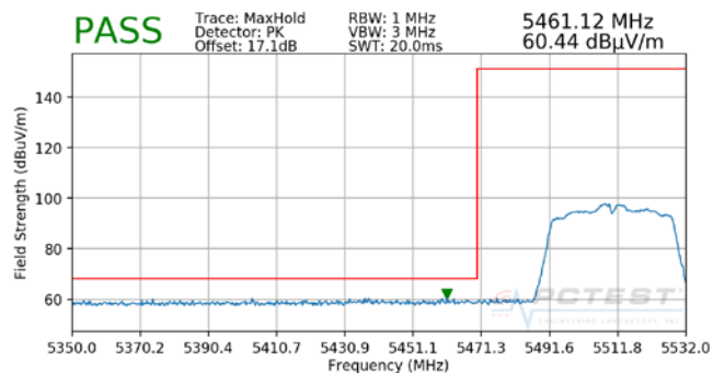
Plot 7-68. Radiated Band Edge Plot SISO ANT2 (Peak – WCP)
