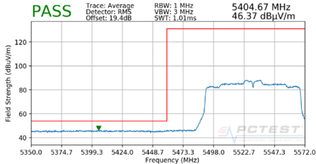
Plot 7-109. Radiated Lower Band Edge Plot MIMO (Average – UNII Band 2C)
