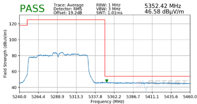
Plot 7-112. Radiated Band Edge Plot ANT (Average – WCP)
