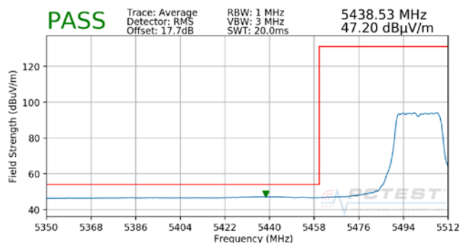
Plot 7-29. Radiated Lower Band Edge Plot (Average – UNII Band 2C)
