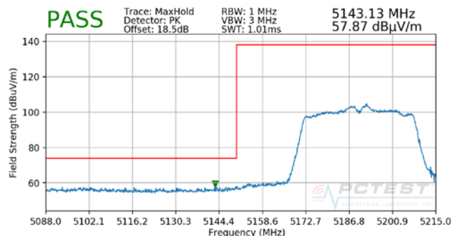
Plot 7-97. Radiated Lower Band Edge Plot MIMO (Peak – UNII Band 1)
