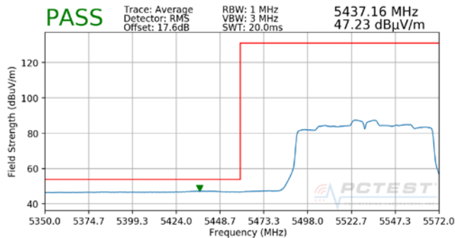
Plot 7-47. Radiated Lower Band Edge Plot (Average – UNII Band 2C)
