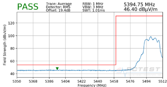
Plot 7-82. Radiated Lower Band Edge Plot MIMO (Average – UNII Band 2C)
