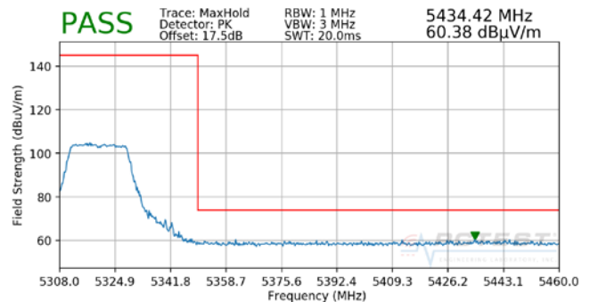
Plot 7-28. Radiated Upper Band Edge Plot (Peak – UNII Band 2A)
