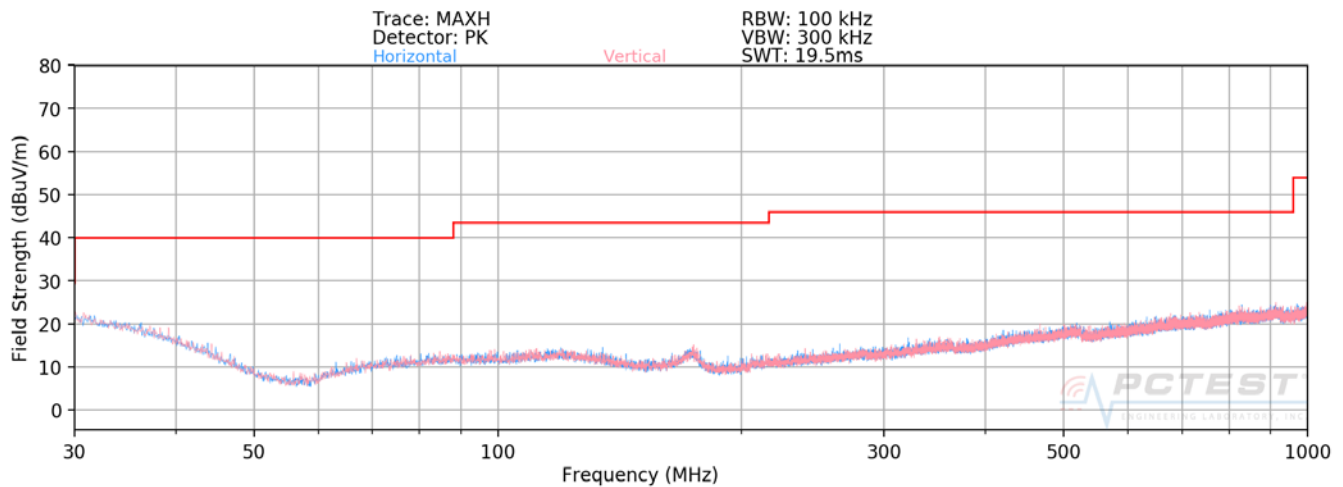
Plot 7-21. Radiated Spurious Plot below 1GHz (2.4GHz – 5GHz)
