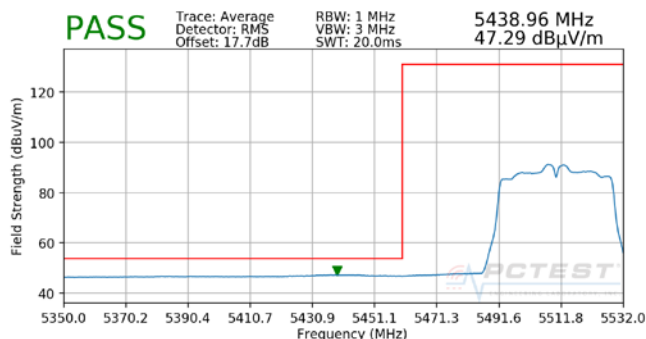
Plot 7-64. Radiated Lower Band Edge Plot SISO ANT2 (Average - UNII Band 2C)
