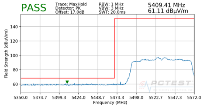
Plot 7-48. Radiated Lower Band Edge Plot (Peak – UNII Band 2C)
