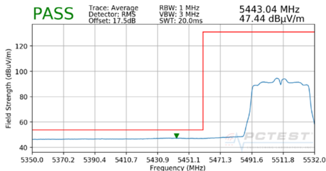
Plot 7-38. Radiated Lower Band Edge Plot (Average – UNII Band 2C)
