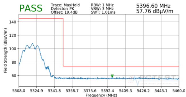
Plot 7-86. Radiated Band Edge Plot MIMO (Peak – WCP)
