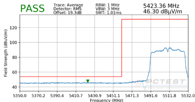
Plot 7-100. Radiated Lower Band Edge Plot MIMO (Average – UNII Band 2C)
