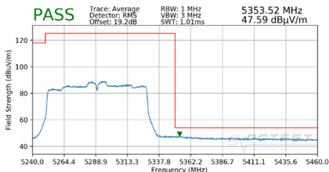
Plot 7-107. Radiated Upper Band Edge Plot MIMO (Average – UNII Band 2A)
