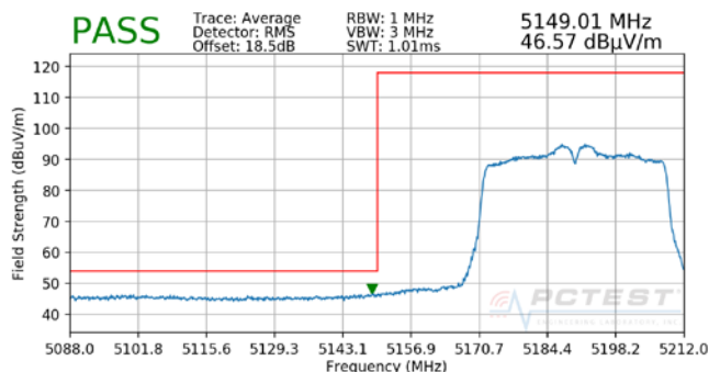
Plot 7-96. Radiated Lower Band Edge Plot MIMO (Average – UNII Band 1)
