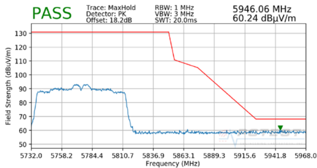
Plot 7-49. Radiated Upper Band Edge Plot (Peak – UNII Band 3)
