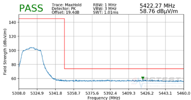
Plot 7-95. Radiated Band Edge Plot MIMO (Peak – WCP)
