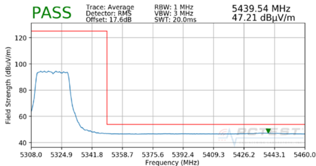
Plot 7-27. Radiated Upper Band Edge Plot (Average – UNII Band 2A)
