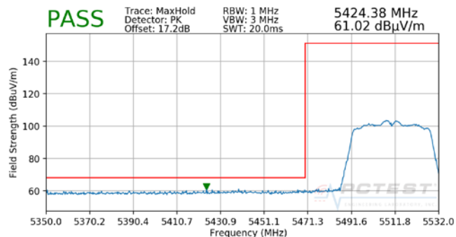
Plot 7-39. Radiated Lower Band Edge Plot (Peak – UNII Band 2C)
