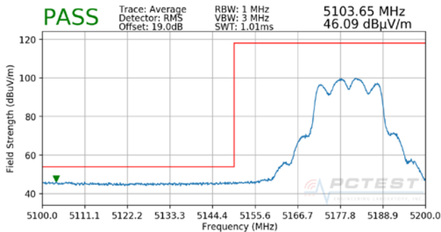
Plot 7-78. Radiated Lower Band Edge Plot MIMO (Average – UNII Band 1)
