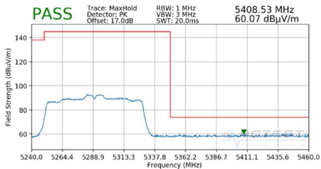
Plot 7-77. Radiated Band Edge Plot SISO ANT2 (Peak – WCP)
