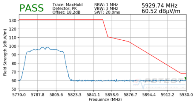
Plot 7-40. Radiated Upper Band Edge Plot (Peak – UNII Band 3)
