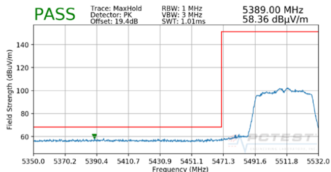
Plot 7-101. Radiated Lower Band Edge Plot MIMO (Peak – UNII Band 2C)
