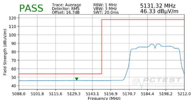
Plot 7-60. Radiated Lower Band Edge Plot SISO ANT2 (Average – UNII Band 1)
