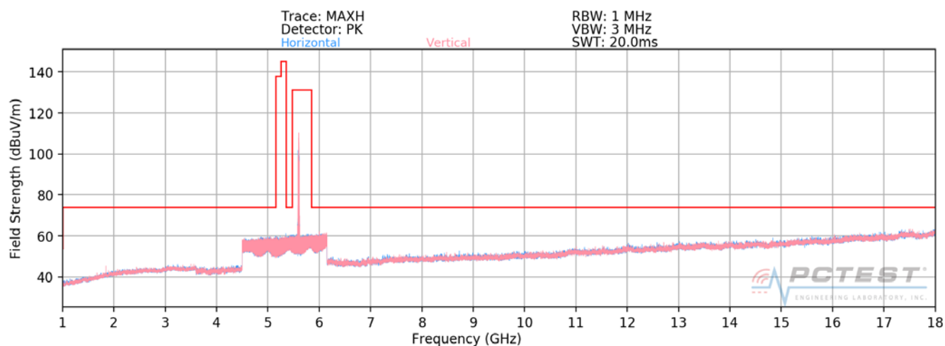
Plot 7-15. Radiated Spurious Plot above 1GHz MIMO/CDD (802.11a – U2C Ch. 120)
