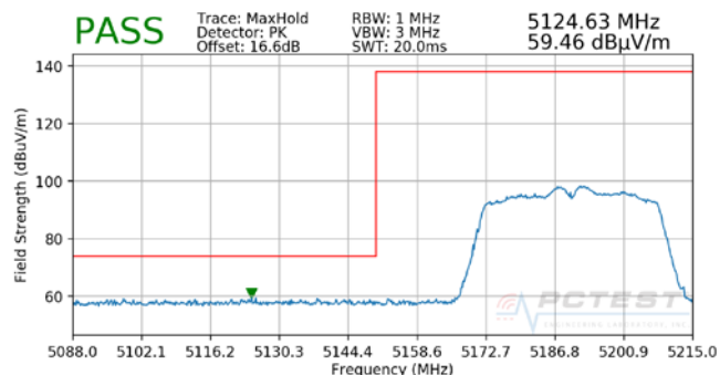
Plot 7-61. Radiated Lower Band Edge Plot SISO ANT2 (Peak – UNII Band 1)
