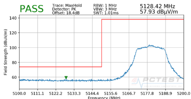
Plot 7-88. Radiated Lower Band Edge Plot MIMO (Peak – UNII Band 1)
