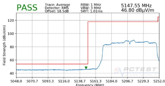
Plot 7-105. Radiated Lower Band Edge Plot MIMO (Average – UNII Band 1)
