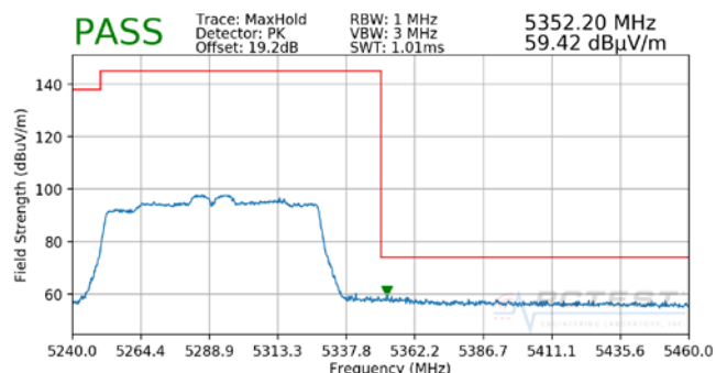
Plot 7-108. Radiated Upper Band Edge Plot MIMO (Peak – UNII Band 2A)
