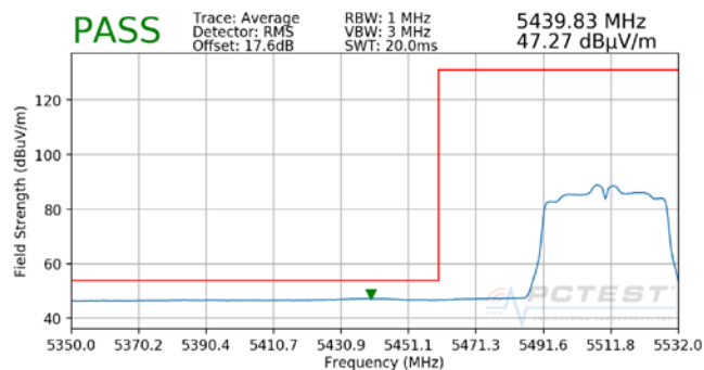
Plot 7-67. Radiated Band Edge Plot SISO ANT2 (Average – WCP)
