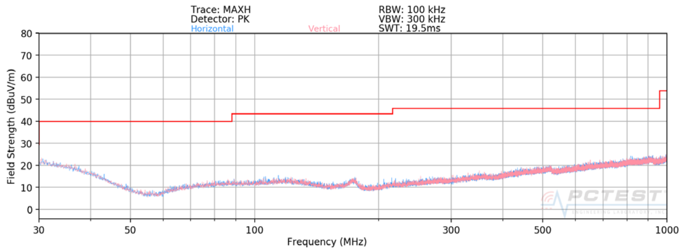
Plot 7-114. Radiated Spurious Plot below 1GHz (802.11a – U3 Ch. 157)
