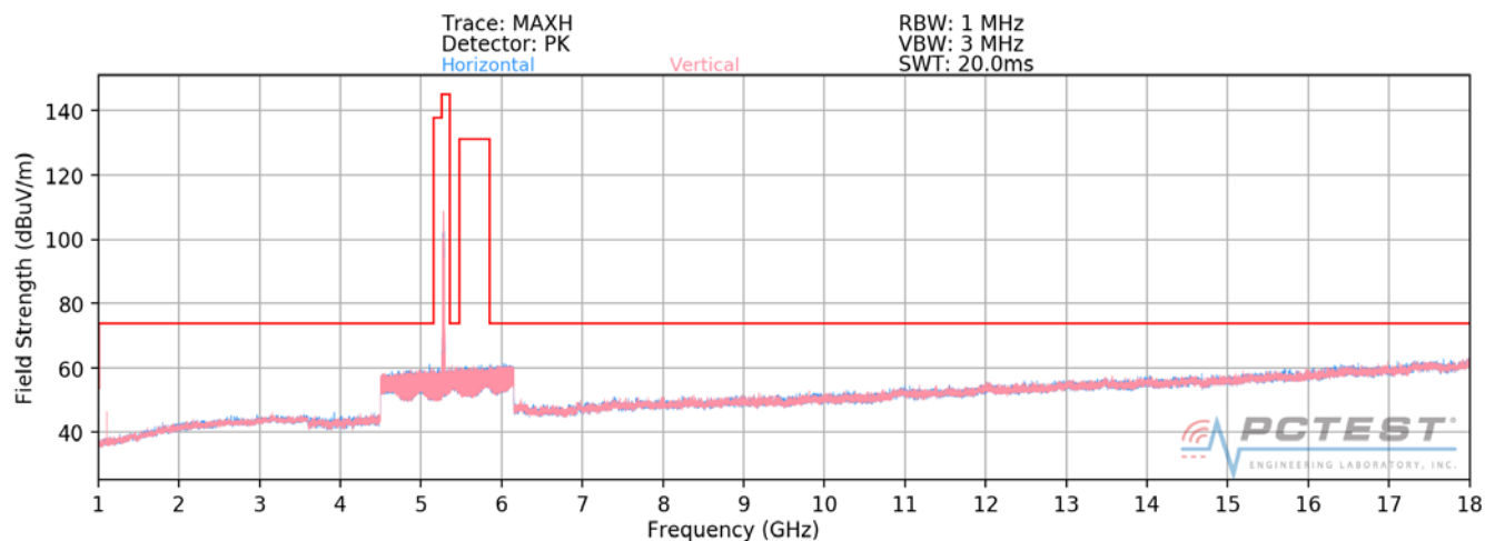
Plot 7-14. Radiated Spurious Plot above 1GHz MIMO/CDD (802.11a – U2A Ch. 56)
