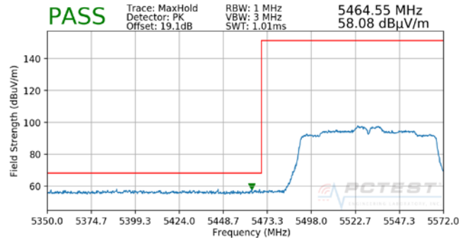
Plot 7-110. Radiated Lower Band Edge Plot MIMO (Peak – UNII Band 2C)
