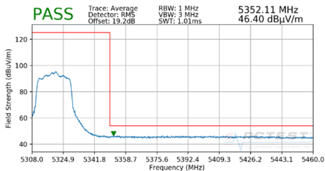
Plot 7-94. Radiated Band Edge Plot MIMO (Average – WCP)
