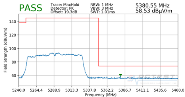
Plot 7-113. Radiated Band Edge Plot ANT (Peak – WCP)
