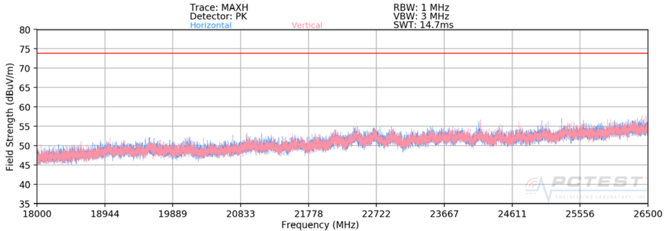
Plot 7-23. Radiated Spurious Plot 18GHz - 26.5GHz (Dual Band Simult. Tx)
