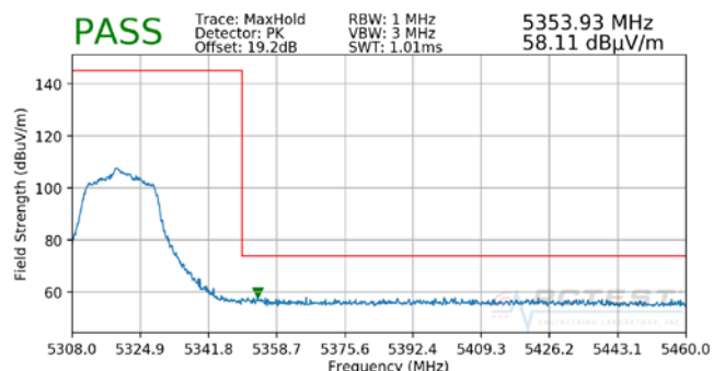
Plot 7-90. Radiated Upper Band Edge Plot MIMO (Peak – UNII Band 2A)
