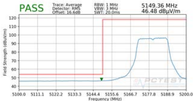
Plot 7-25. Radiated Lower Band Edge Plot (Average – UNII Band 1)
