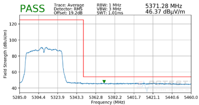
Plot 7-103. Radiated Band Edge Plot ANT (Average – WCP)
