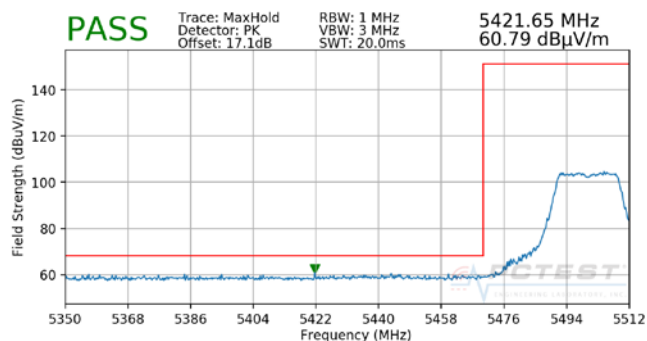
Plot 7-30. Radiated Lower Band Edge Plot (Peak – UNII Band 2C)
