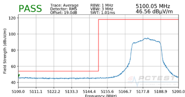
Plot 7-87. Radiated Lower Band Edge Plot MIMO (Average – UNII Band 1)
