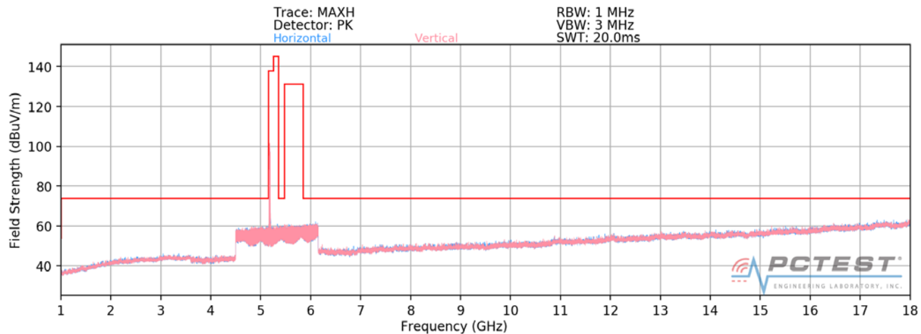
Plot 7-7. Radiated Spurious Plot above 1GHz SISO ANT2 (802.11a – U1 Ch. 40)
