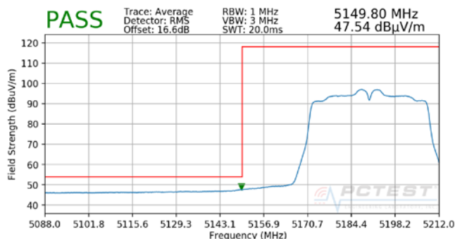
Plot 7-34. Radiated Lower Band Edge Plot (Average – UNII Band 1)
