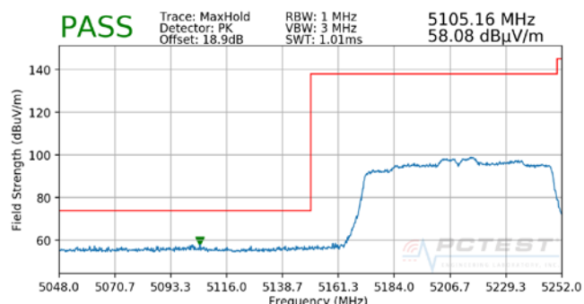
Plot 7-106. Radiated Lower Band Edge Plot MIMO (Peak – UNII Band 1)
