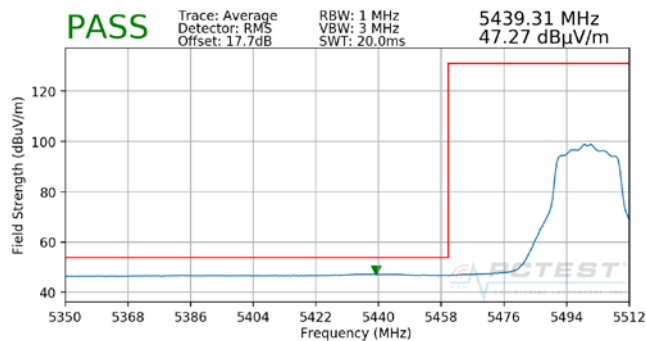
Plot 7-32. Radiated Band Edge Plot (Average – WCP)
