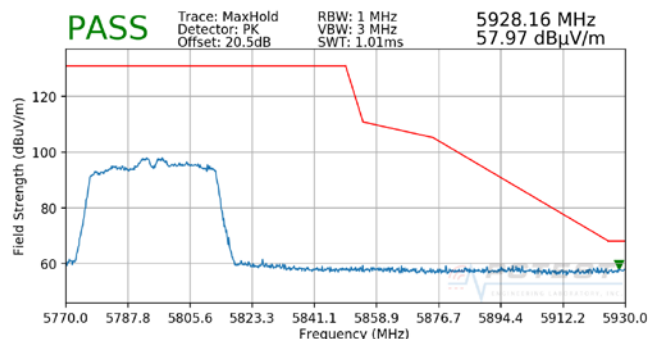
Plot 7-102. Radiated Upper Band Edge Plot MIMO (Peak – UNII Band 3)
