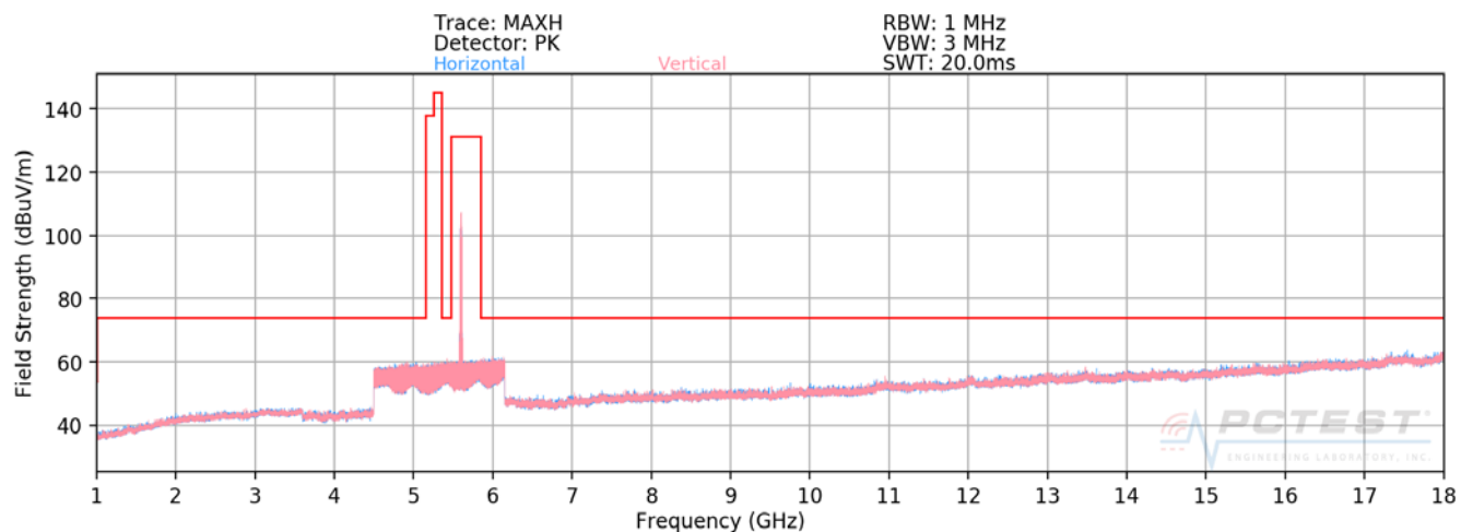
Plot 7-9. Radiated Spurious Plot above 1GHz SISO ANT2 (802.11a – U2C Ch. 120)
