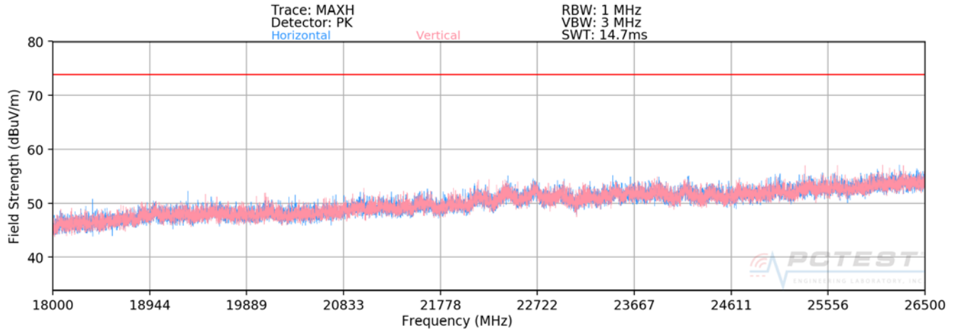
Plot 7-19. Radiated Spurious Plot above 18GHz - 26.5GHz MIMO/CDD (802.11a)
