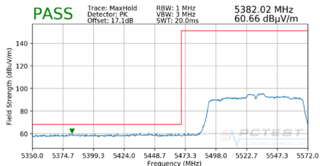
Plot 7-74. Radiated Lower Band Edge Plot SISO ANT2 (Peak – UNII Band 2C)
