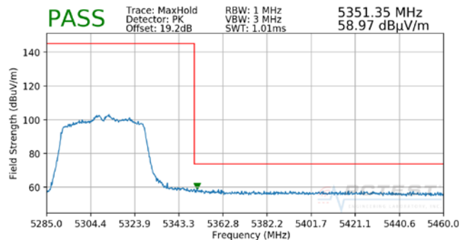
Plot 7-99. Radiated Upper Band Edge Plot MIMO (Peak – UNII Band 2A)
