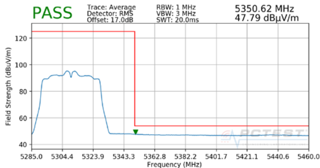
Plot 7-36. Radiated Upper Band Edge Plot (Average – UNII Band 2A)
