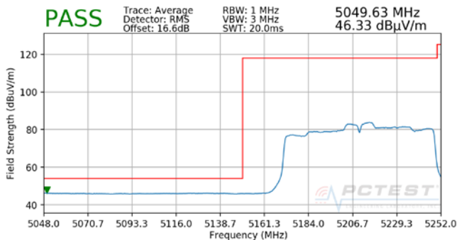
Plot 7-69. Radiated Lower Band Edge Plot SISO ANT2 (Average – UNII Band 1)
