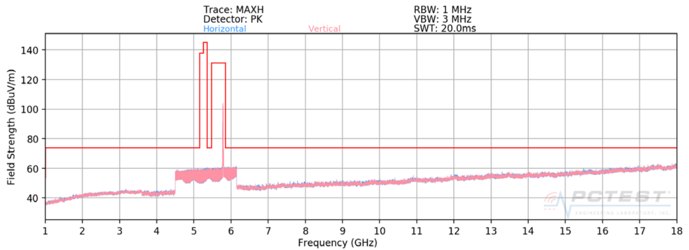
Plot 7-4. Radiated Spurious Plot above 1GHz SISO ANT1 (802.11a – U3 Ch. 157)
