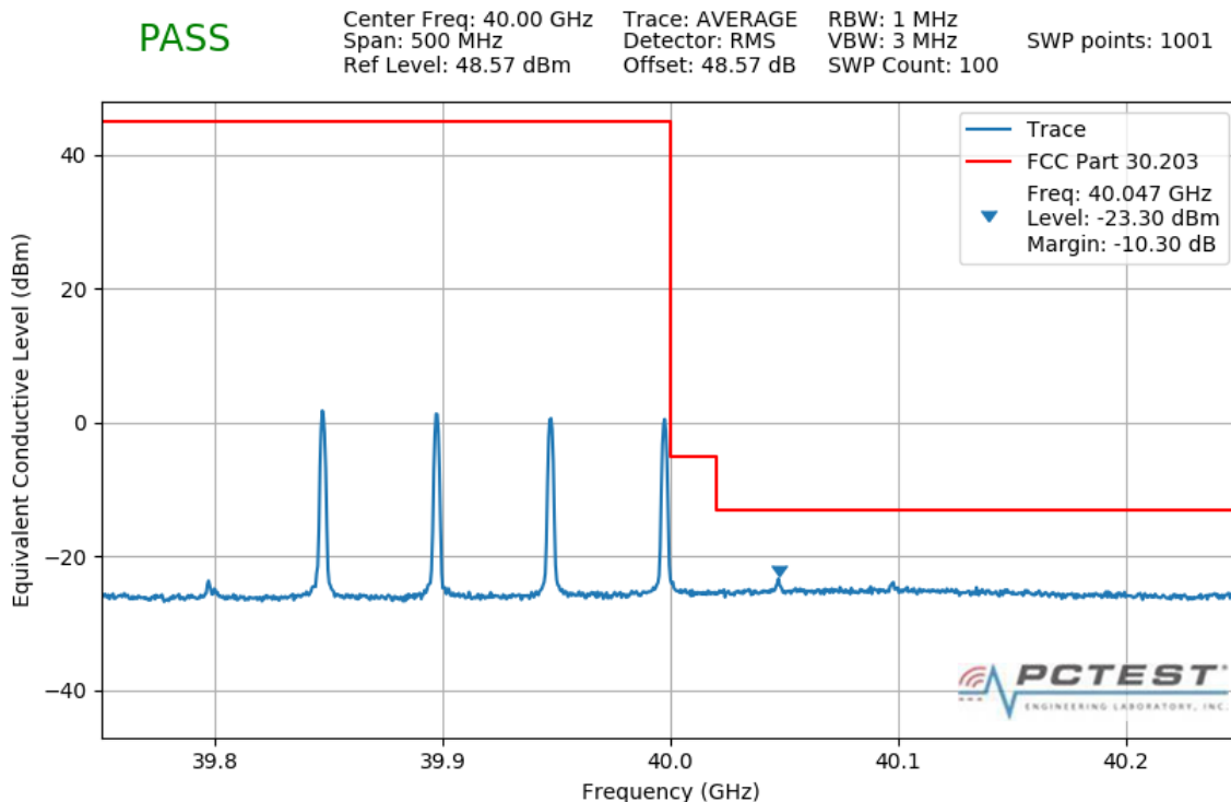
Plot 7-423. Band Edge Plot (4CC 50M QPSK Hi Channel- 1 RB 31 offset)
