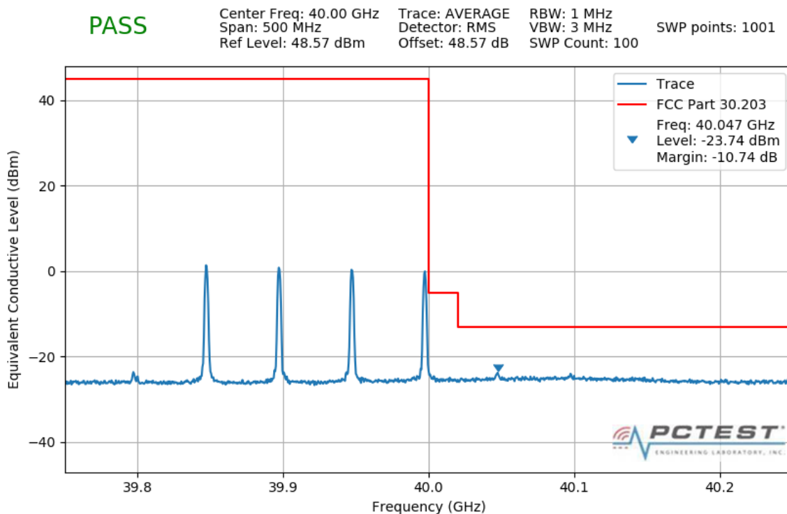
Plot 7-424. Band Edge Plot (4CC 50M 16QAM Hi Channel- 1 RB 31 offset)
