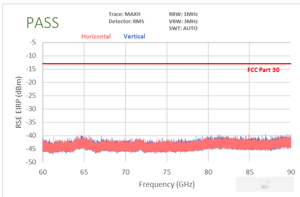
Plot 7-108. Radiated Spurious Plot 60-90 GHz (QTM0 1CC-100MHz Bandwidth QPSK Mid Channel)
