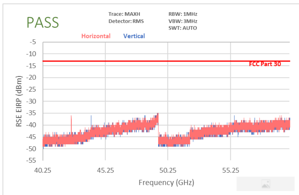
Plot 7-101. Radiated Spurious Plot 40-60 GHz (QTM0 1CC-100MHz Bandwidth QPSK Low Channel)
