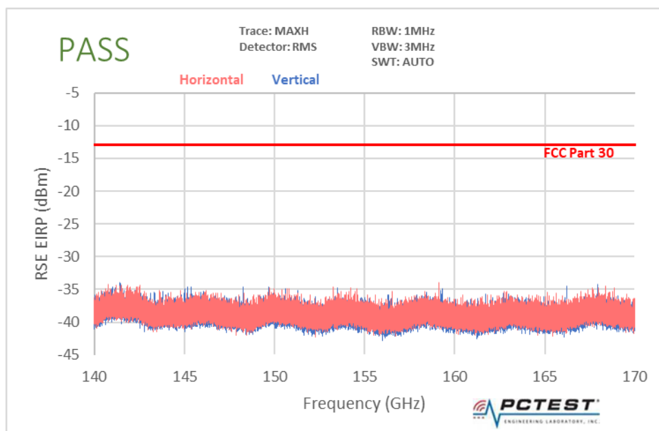
Plot 7-119. Radiated Spurious Plot 140-170 GHz (QTM0 1CC-100MHz Bandwidth QPSK Low Channel)
