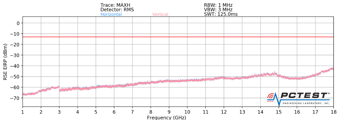
Plot 7-94. Radiated Spurious Plot 1-18 GHz (QTM1 1CC-100MHz Bandwidth QPSK High Channel)
