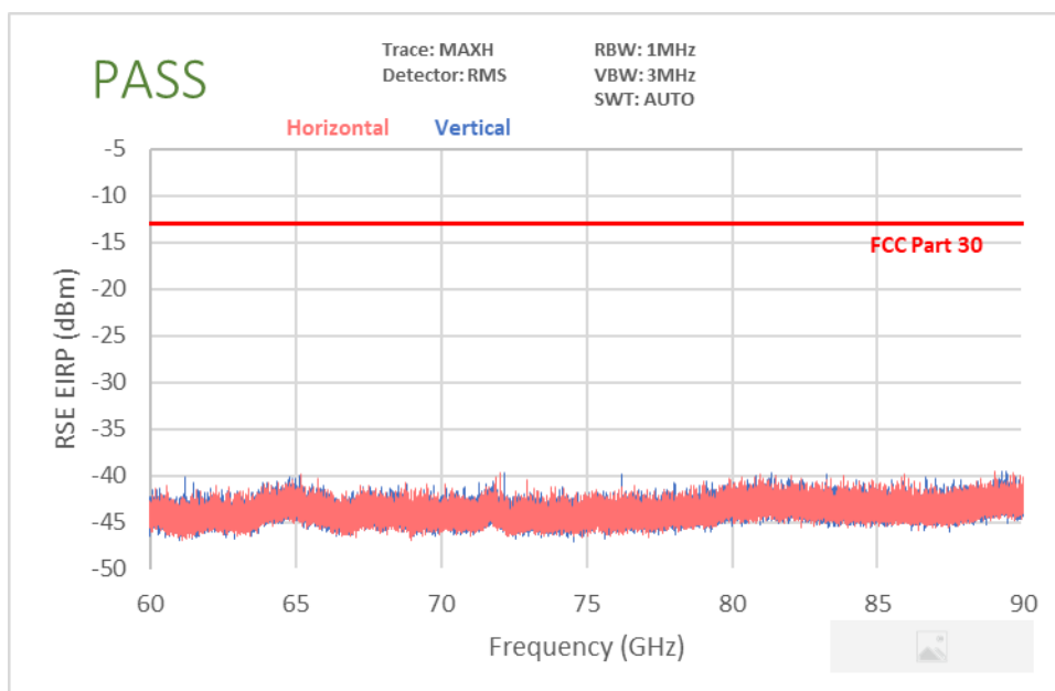
Plot 7-107. Radiated Spurious Plot 60-90 GHz (QTM0 1CC-100MHz Bandwidth QPSK Low Channel)
