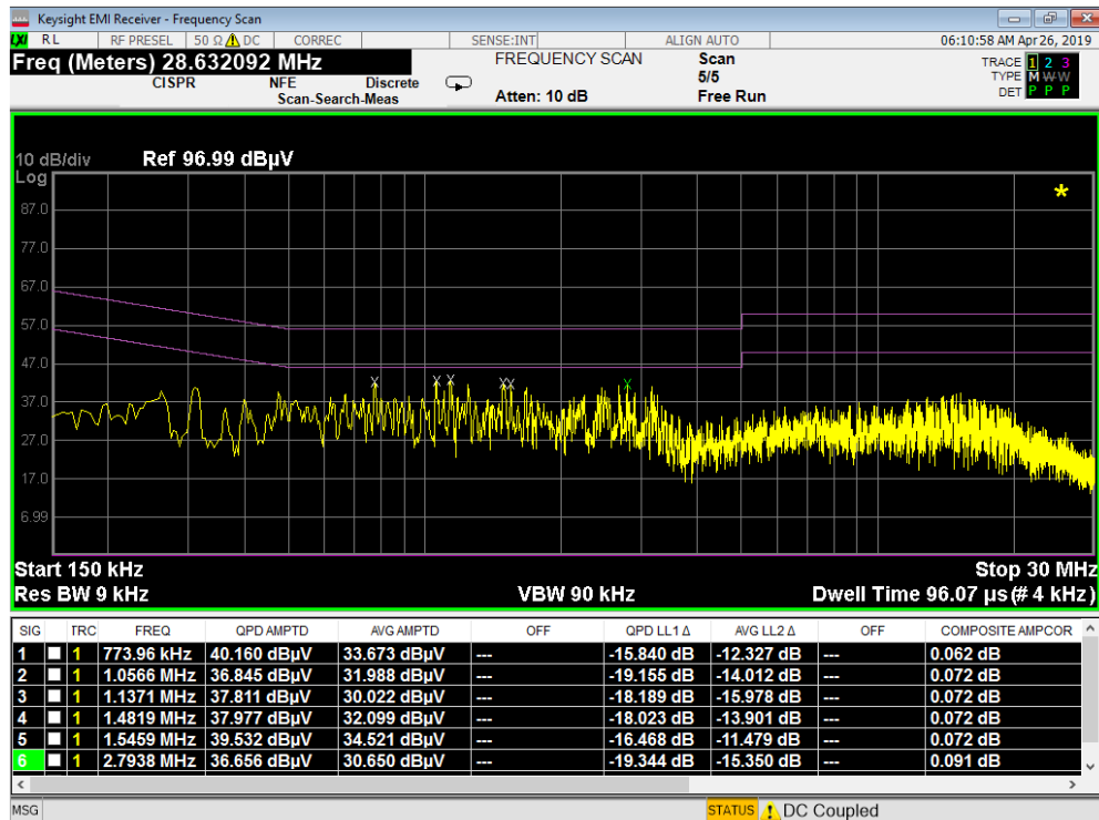
Plot 7-279. Line Conducted Plot with 802.11a UNII Band 3 with WCP (L1)
