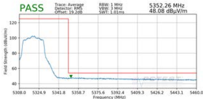
Plot 7-174. Radiated Upper Band Edge Plot SISO ANT1 (Average – UNII Band 2A)
