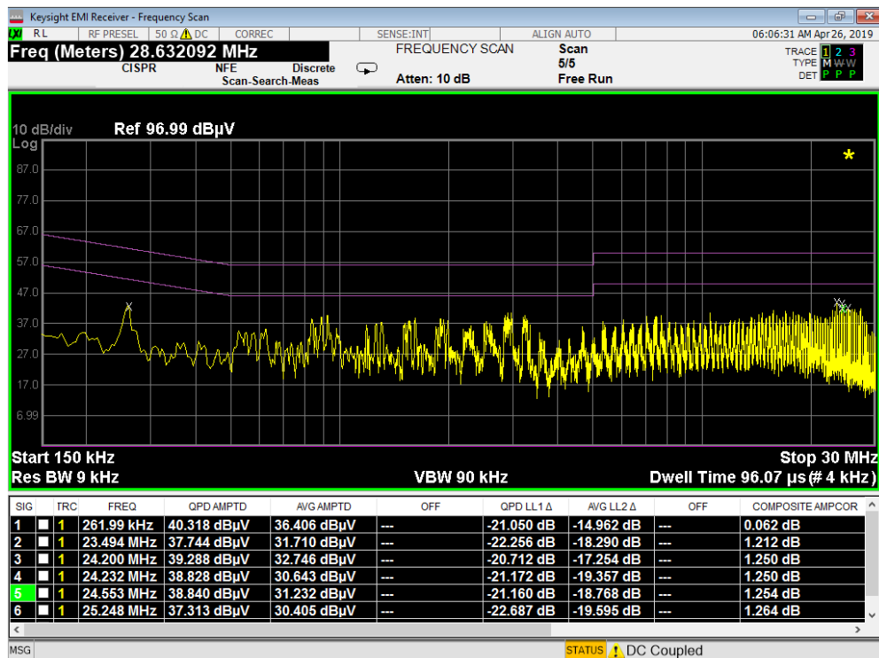
Plot 7-276. Line Conducted Plot with 802.11a UNII Band 2A with WCP (N)
