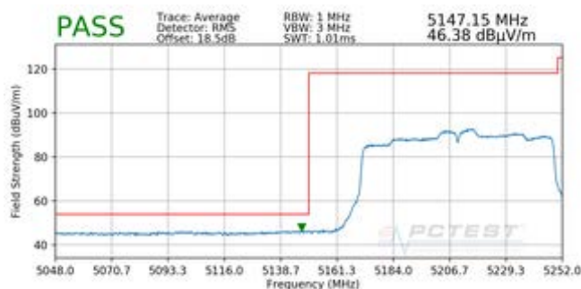
Plot 7-190. Radiated Lower Band Edge Plot SISO ANT1 (Average – UNII Band 1)
