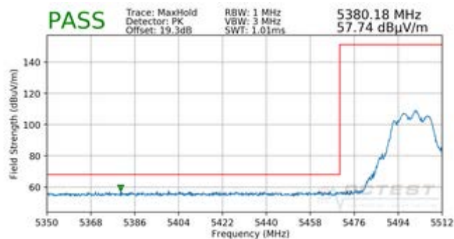
Plot 7-231. Radiated Lower Band Edge Plot CDD (Peak – UNII Band 2C)
