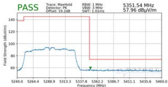
Plot 7-261. Radiated Upper Band Edge Plot MIMO (Peak – WCP)
