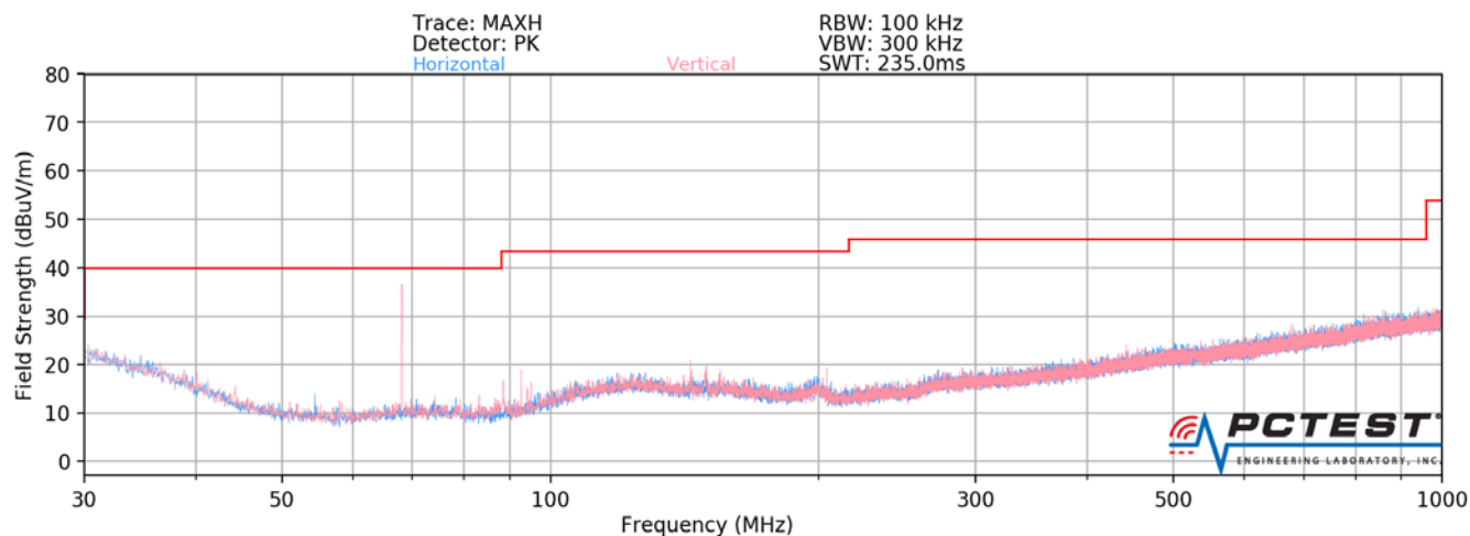
Plot 7-262. Radiated Spurious Plot below 1GHz SISO ANT1 (802.11a – U3 Ch. 157)
