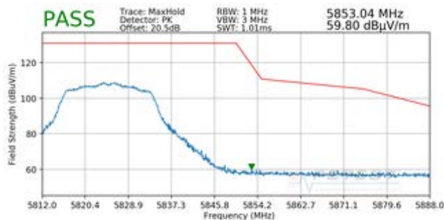
Plot 7-178. Radiated Upper Band Edge Plot SISO ANT1 (Peak – UNII Band 3)
