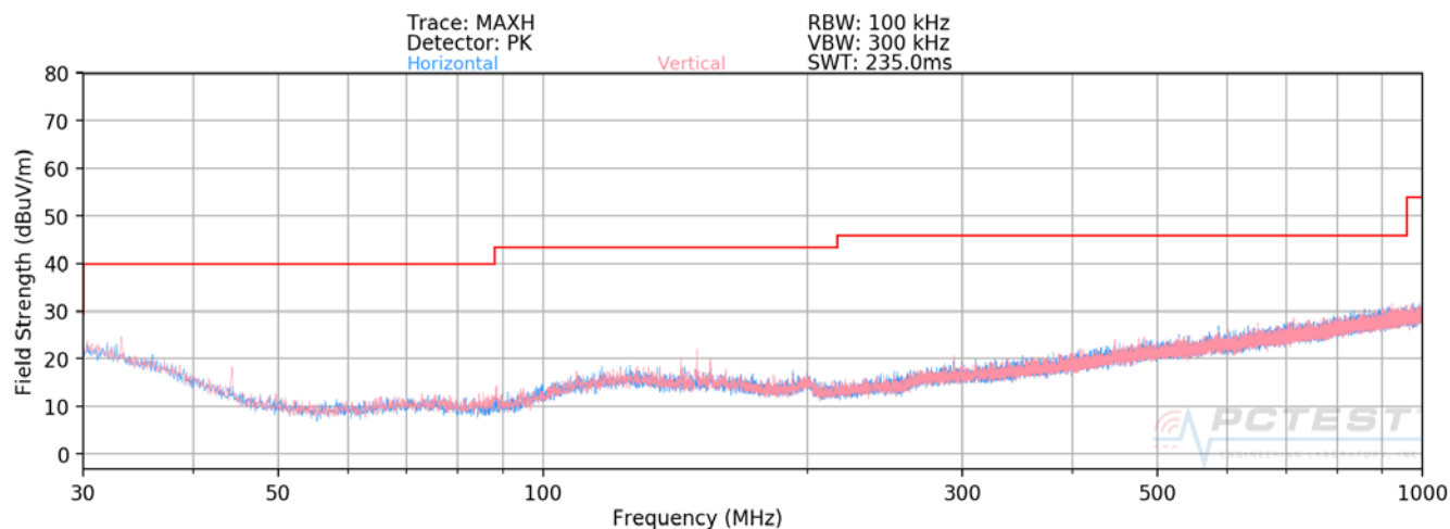
Plot 7-264. Radiated Spurious Plot below 1GHz (2.4GHz – 5GHz)
