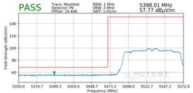
Plot 7-195. Radiated Lower Band Edge Plot SISO ANT1 (Peak – UNII Band 2C)
