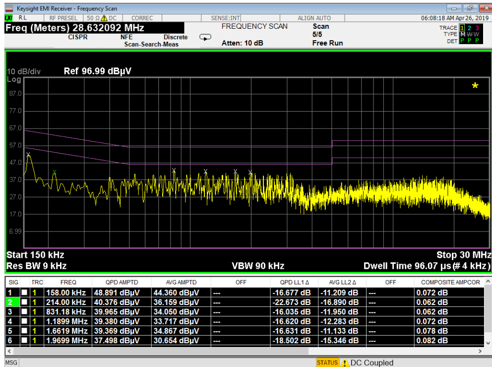
Plot 7-277. Line Conducted Plot with 802.11a UNII Band 2C with WCP (L1)
