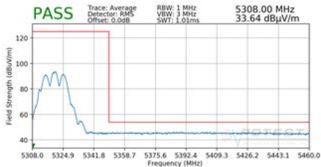
Plot 7-233. Radiated Band Edge Plot CDD (Average – WCP)
