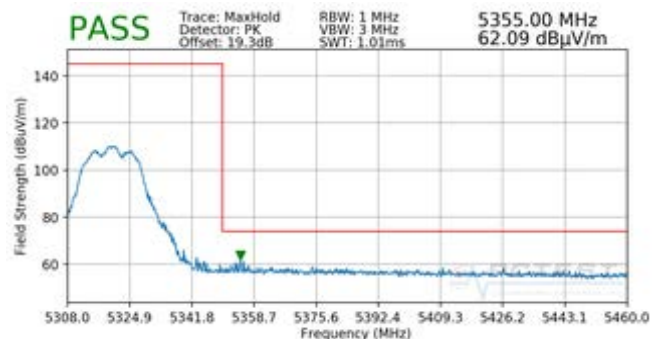
Plot 7-229. Radiated Upper Band Edge Plot CDD (Peak – UNII Band 2A)
