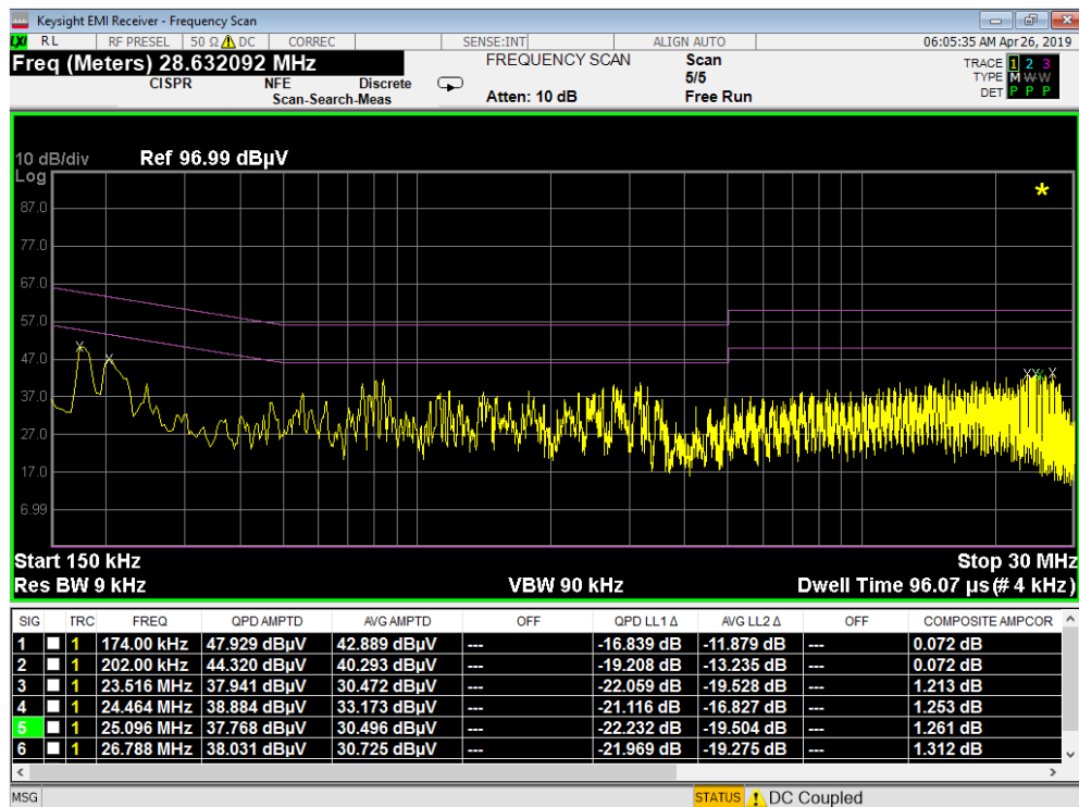
Plot 7-274. Line Conducted Plot with 802.11a UNII Band 1 with WCP (N)
