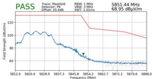
Plot 7-232. Radiated Upper Band Edge Plot CDD (Peak – UNII Band 3)
