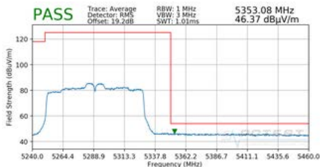
Plot 7-260. Radiated Upper Band Edge Plot MIMO (Average – WCP)
