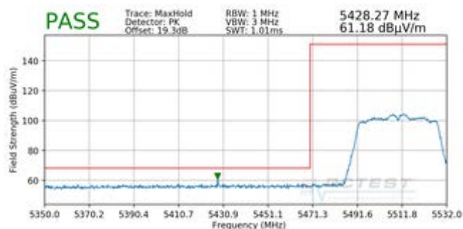
Plot 7-186. Radiated Lower Band Edge Plot SISO ANT1 (Peak – UNII Band 2C)
