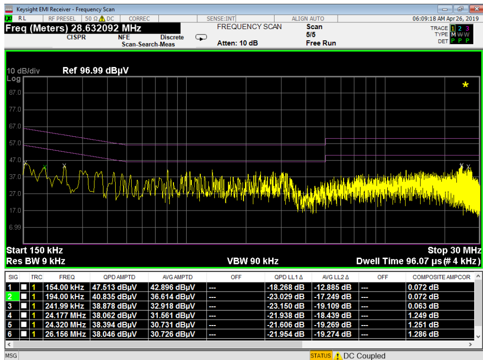
Plot 7-278. Line Conducted Plot with 802.11a UNII Band 2C with WCP (N)
