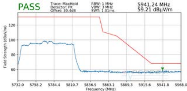
Plot 7-196. Radiated Upper Band Edge Plot SISO ANT1 (Peak – UNII Band 3)
