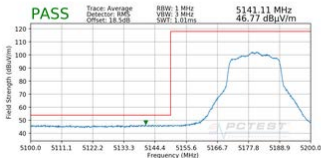
Plot 7-172. Radiated Lower Band Edge Plot SISO ANT1 (Average – UNII Band 1)
