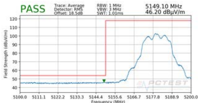
Plot 7-226. Radiated Lower Band Edge Plot CDD (Average – UNII Band 1)
