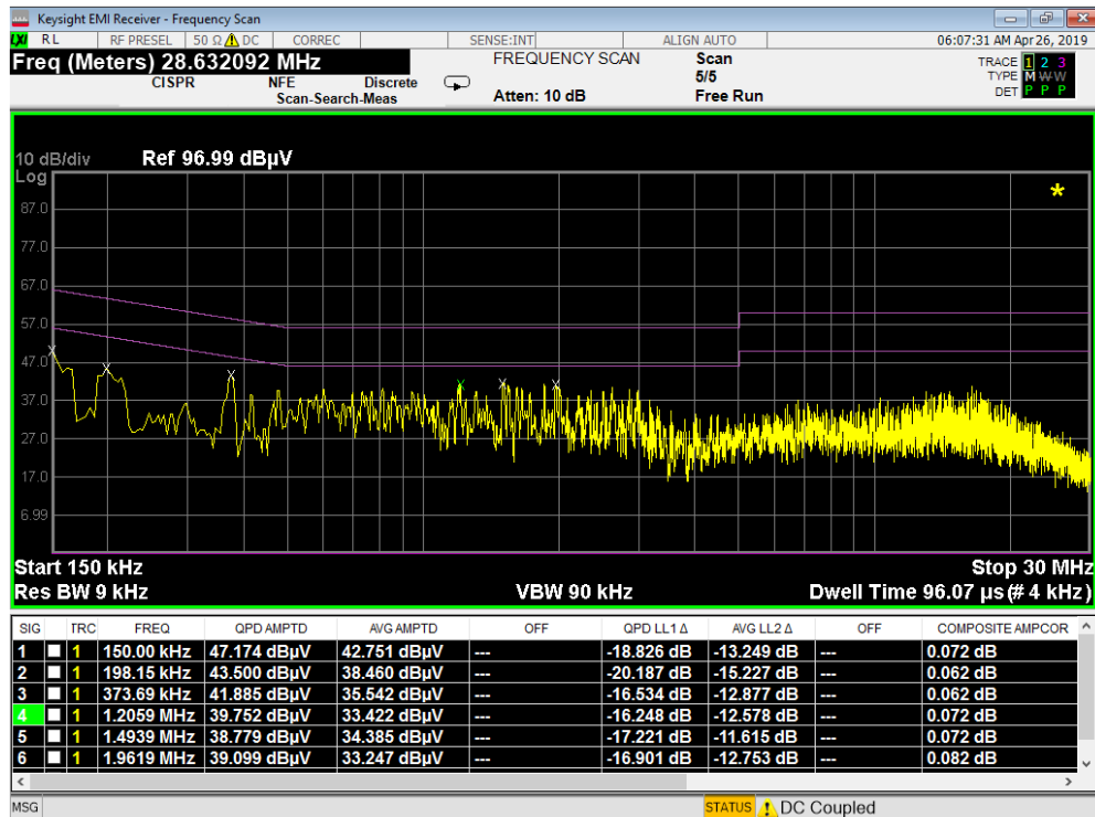
Plot 7-275. Line Conducted Plot with 802.11a UNII Band 2A with WCP (L1)
