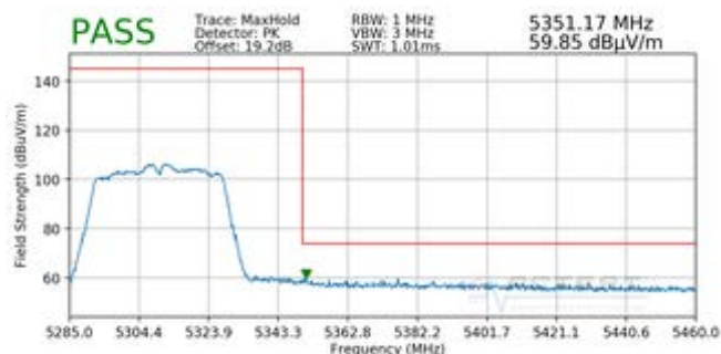
Plot 7-184. Radiated Upper Band Edge Plot SISO ANT1 (Peak – UNII Band 2A)
