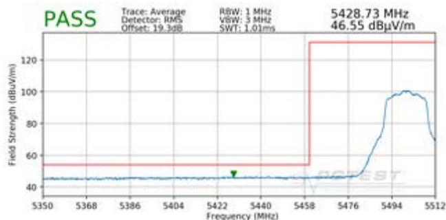
Plot 7-176. Radiated Lower Band Edge Plot SISO ANT1 (Average – UNII Band 2C)
