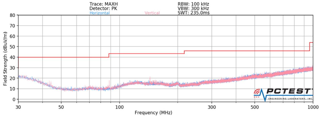
Plot 7-263. Radiated Spurious Plot below 1GHz SISO ANT2 (802.11a – U3 Ch. 157)
