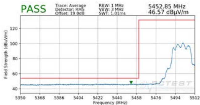
Plot 7-230. Radiated Lower Band Edge Plot CDD (Average – UNII Band 2C)
