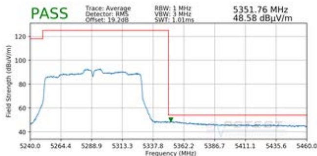
Plot 7-192. Radiated Upper Band Edge Plot SISO ANT1 (Average – UNII Band 2A)
