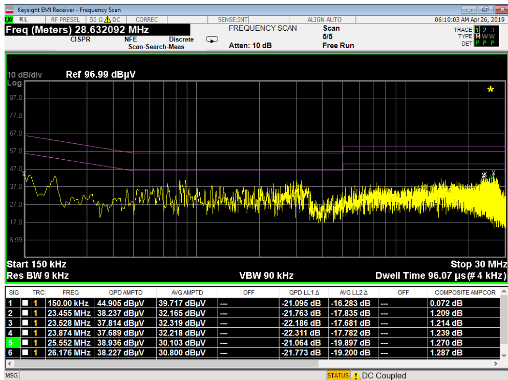
Plot 7-280. Line Conducted Plot with 802.11a UNII Band 3 with WCP (N)
