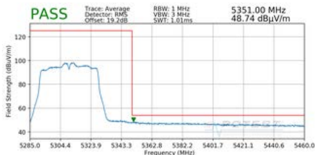
Plot 7-183. Radiated Upper Band Edge Plot SISO ANT1 (Average – UNII Band 2A)
