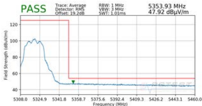
Plot 7-228. Radiated Upper Band Edge Plot CDD (Average – UNII Band 2A)
