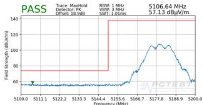
Plot 7-227. Radiated Lower Band Edge Plot CDD (Peak – UNII Band 1)
