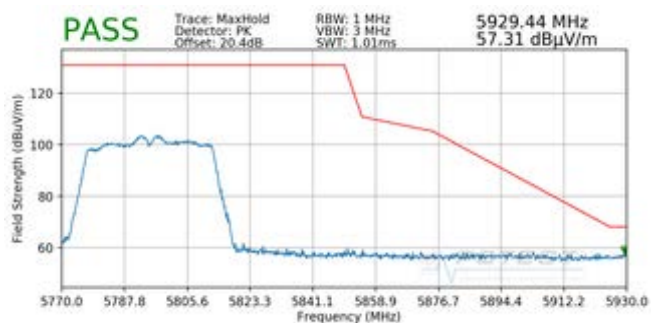
Plot 7-187. Radiated Upper Band Edge Plot SISO ANT1 (Peak – UNII Band 3)
