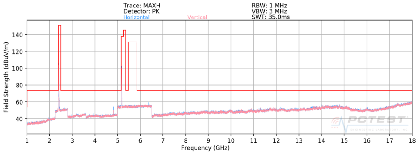
Plot 7-169. Radiated Spurious Plot above 1GHz (2.4GHz – 5GHz)
