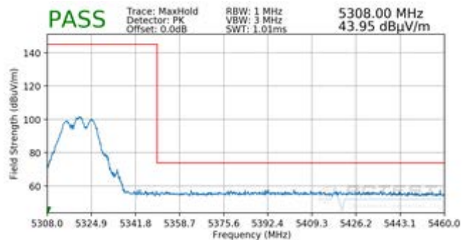
Plot 7-234. Radiated Band Edge Plot CDD (Peak – WCP)
