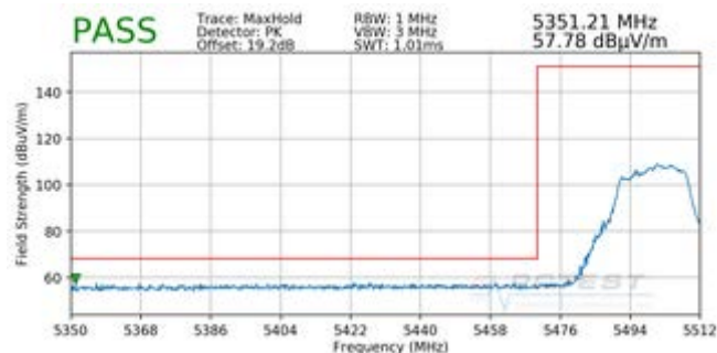
Plot 7-177. Radiated Lower Band Edge Plot SISO ANT1 (Peak – UNII Band 2C)
