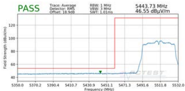
Plot 7-185. Radiated Lower Band Edge Plot SISO ANT1 (Average – UNII Band 2C)
