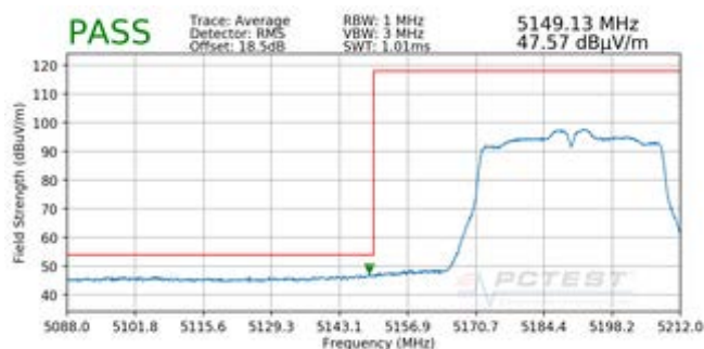
Plot 7-181. Radiated Lower Band Edge Plot SISO ANT1 (Average – UNII Band 1)
