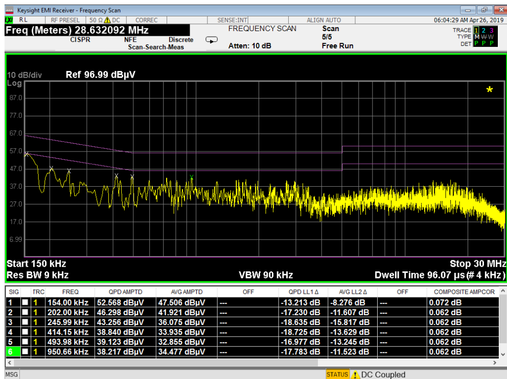
Plot 7-273. Line Conducted Plot with 802.11a UNII Band 1 with WCP (L1)
