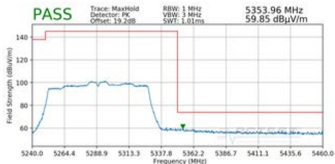
Plot 7-193. Radiated Upper Band Edge Plot SISO ANT1 (Peak – UNII Band 2A)
