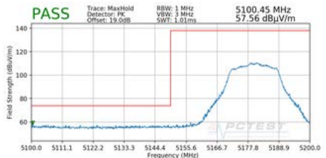
Plot 7-173. Radiated Lower Band Edge Plot SISO ANT1 (Peak – UNII Band 1)
