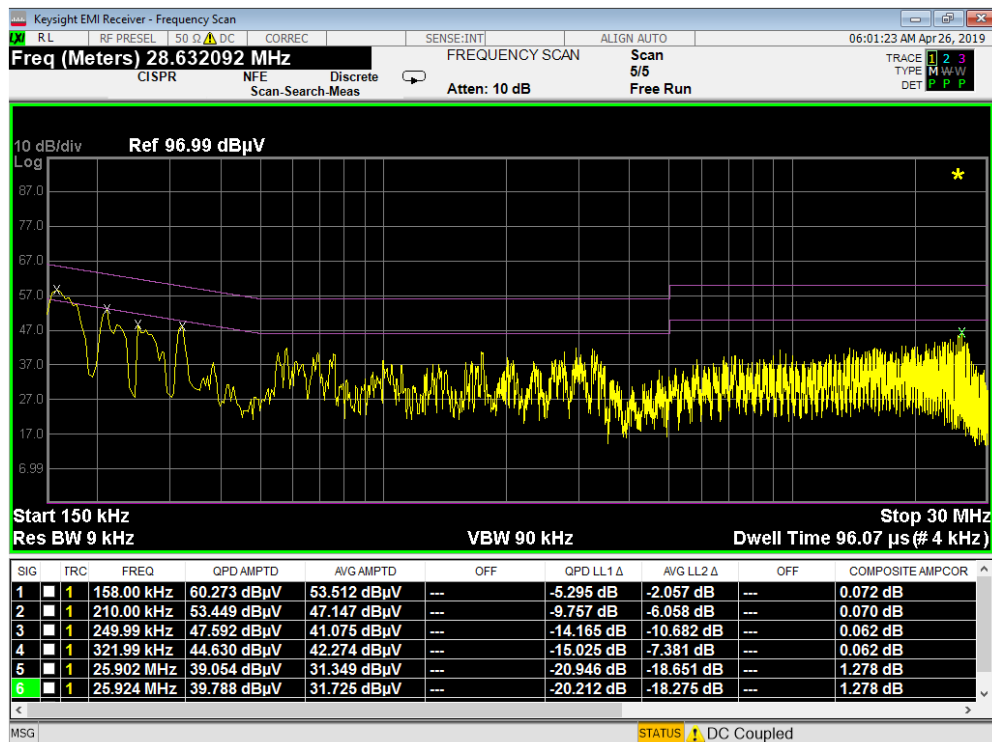
Plot 7-102. Line Conducted Plot with 802.11b with WCP (N)
