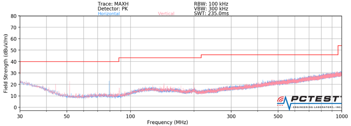
Plot 7-98. Radiated Spurious Plot below 1GHz SISO ANT2
