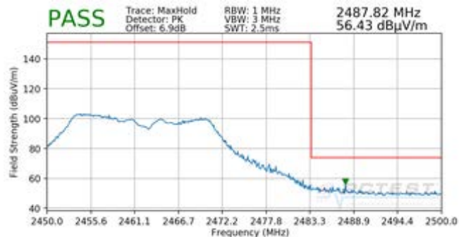
Plot 7-88. Radiated Restricted Upper Band Edge Measurement MIMO (Peak)
