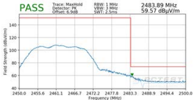
Plot 7-94. Radiated Restricted Upper Band Edge Measurement CDD (Peak)
