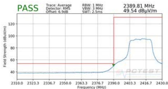
Plot 7-85. Radiated Restricted Lower Band Edge Measurement MIMO (Average)
