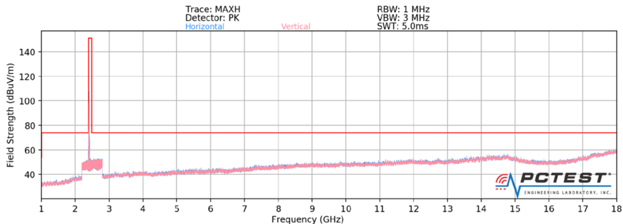
Plot 7-69. Radiated Spurious Plot above 1GHz CDD (802.11g – Ch. 1)
