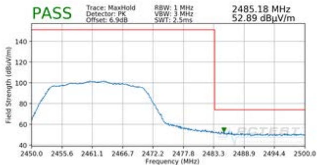
Plot 7-84. Radiated Restricted Band Edge Measurement SISO ANT2 with WCP (Peak)
