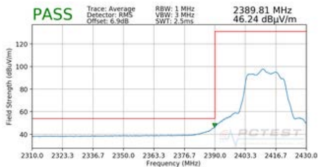
Plot 7-95. Radiated Restricted Band Edge Measurement CDD with WCP (Average)
