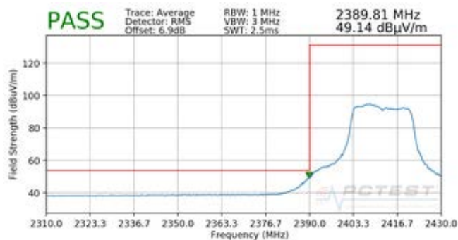
Plot 7-89. Radiated Restricted Band Edge Measurement MIMO with WCP (Average)
