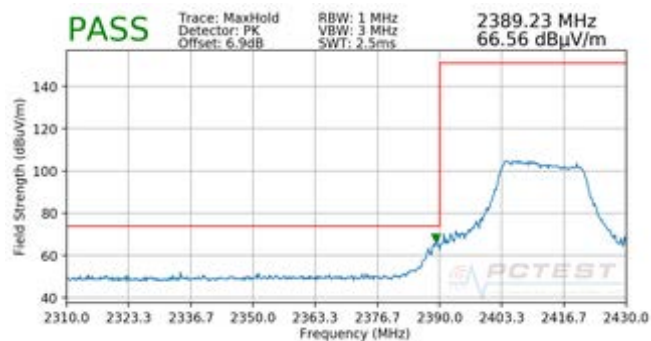
Plot 7-90. Radiated Restricted Band Edge Measurement MIMO with WCP (Peak)
