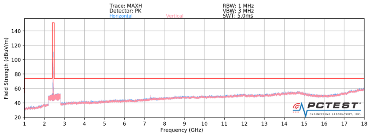
Plot 7-70. Radiated Spurious Plot above 1GHz CDD (802.11g – Ch. 6)
