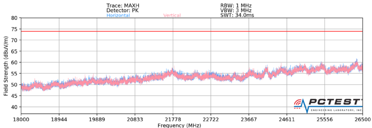
Plot 7-72. Radiated Spurious Plot above 18GHz CDD
