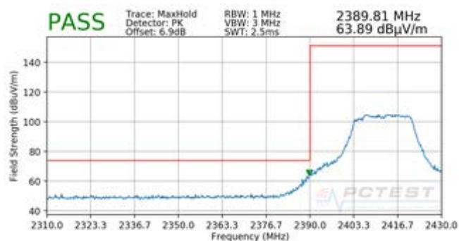
Plot 7-86. Radiated Restricted Lower Band Edge Measurement MIMO (Peak)
