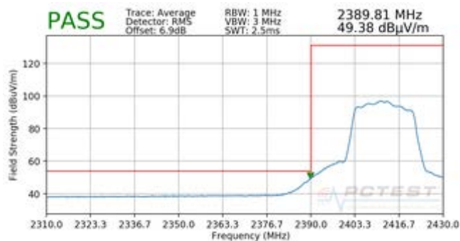
Plot 7-77. Radiated Restricted Band Edge Measurement SISO ANT1 with WCP (Average)
