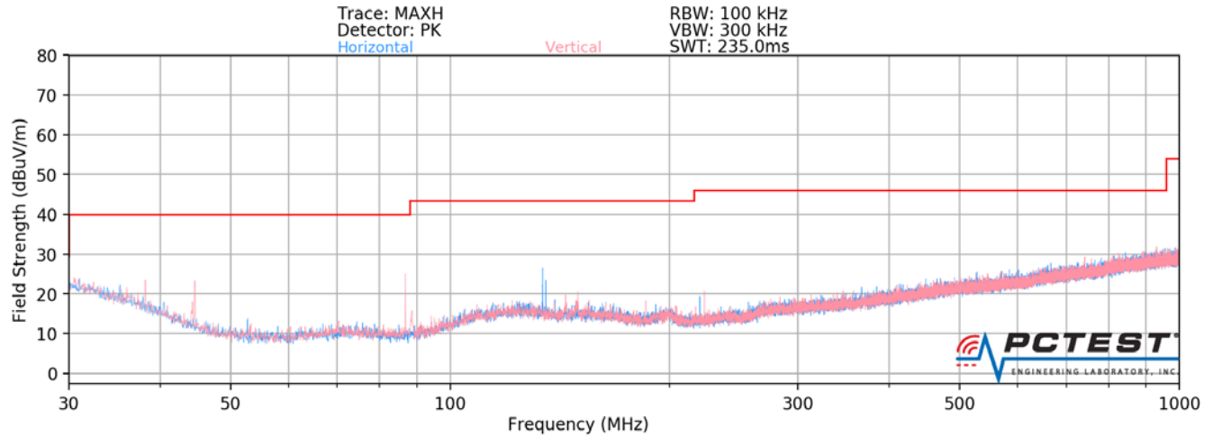
Plot 7-97. Radiated Spurious Plot below 1GHz SISO ANT1
