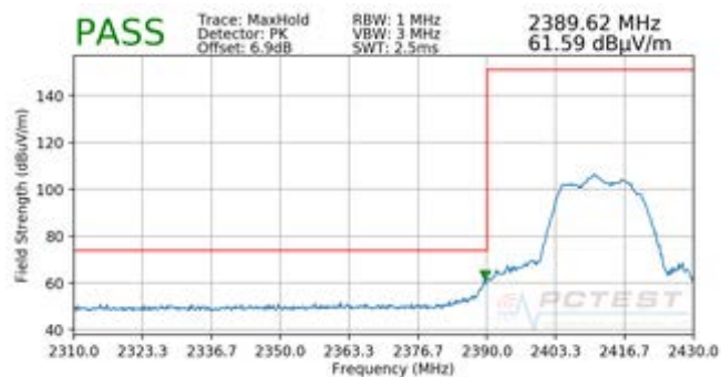
Plot 7-96. Radiated Restricted Band Edge Measurement CDD with WCP (Peak)
