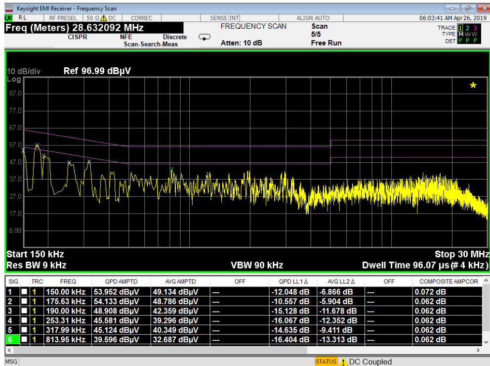
Plot 7-101. Line Conducted Plot with 802.11b with WCP (L1)
