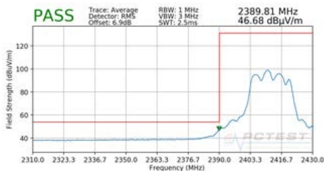
Plot 7-91. Radiated Restricted Lower Band Edge Measurement CDD (Average)
