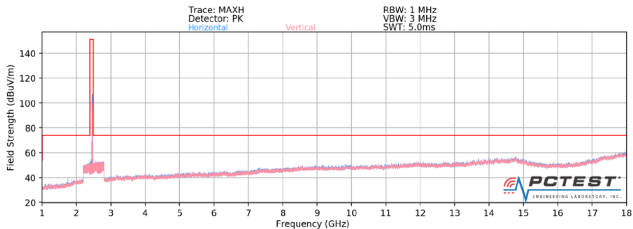
Plot 7-71. Radiated Spurious Plot above 1GHz CDD (802.11g – Ch. 11)
