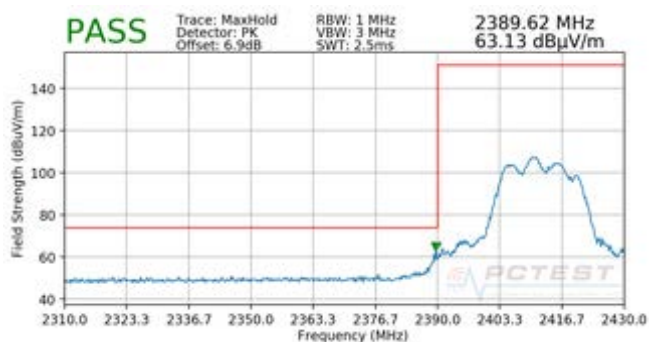
Plot 7-92. Radiated Restricted Lower Band Edge Measurement CDD (Peak)
