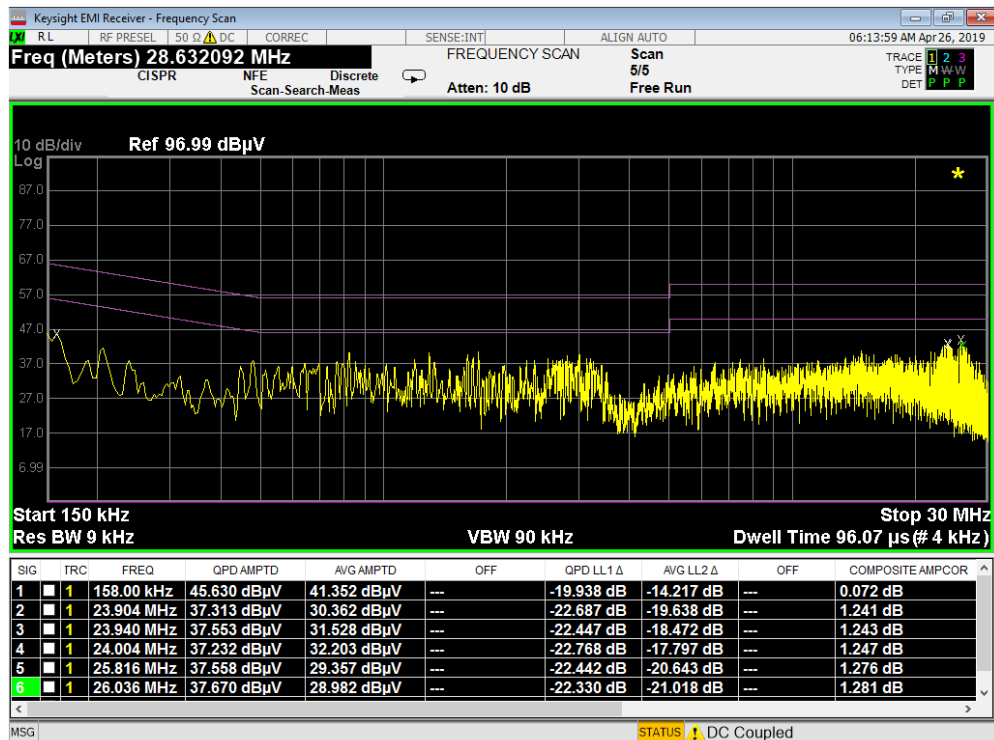
Plot 7-36. Line Conducted Plot with Bluetooth LE with WCP (N)
