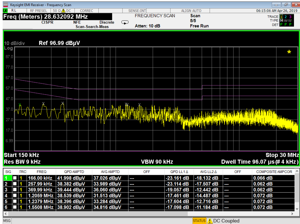
Plot 7-35. Line Conducted Plot with Bluetooth LE with WCP (L1)
