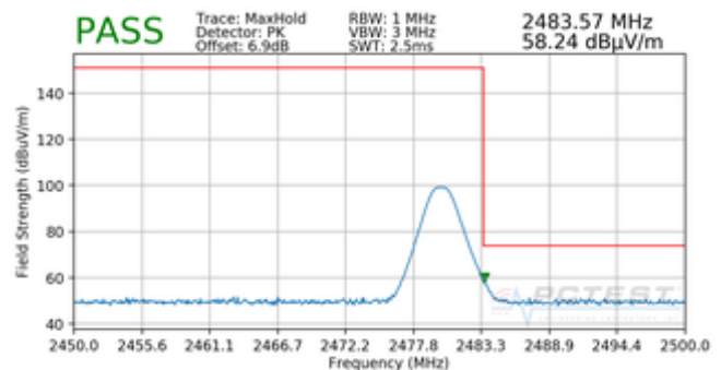
Plot 7-32. Radiated Restricted Upper Band Edge Measurement with WCP (Peak)
