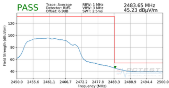
Plot 7-25. Radiated Restricted Band Edge Measurement MIMO with WCP (Average)
