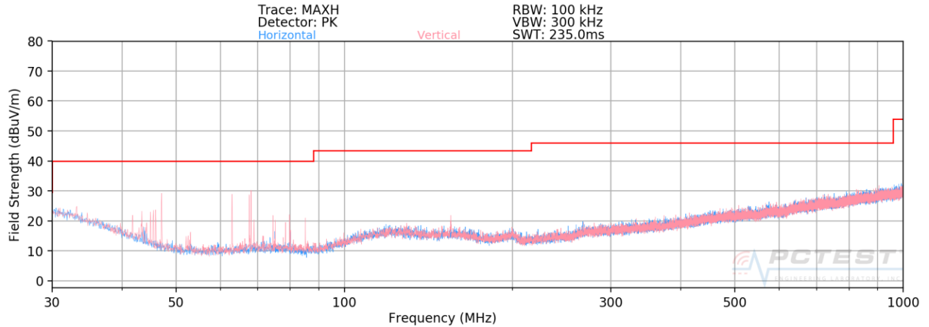
Plot 7-27. Radiated Spurious Plot below 1GHz SISO ANT1
