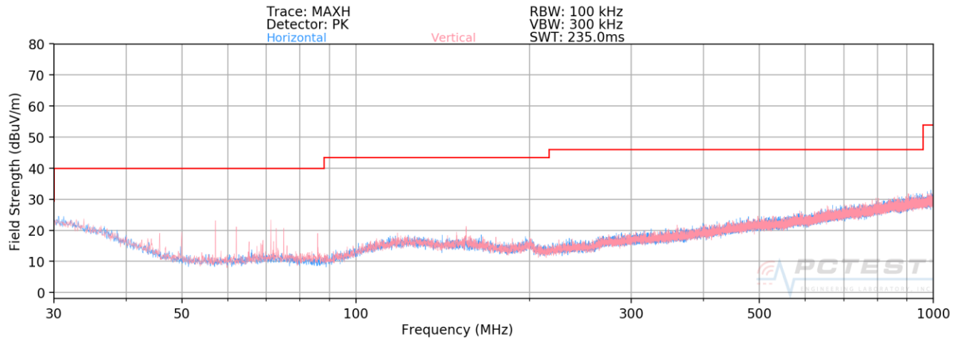
Plot 7-28. Radiated Spurious Plot below 1GHz SISO ANT2
