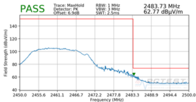
Plot 7-26. Radiated Restricted Band Edge Measurement MIMO with WCP (Peak)
