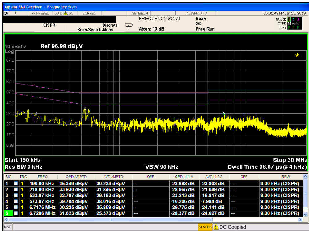
Plot 7-9. Line-Conducted Test Plot with Antenna Terminated at 50 Ohms (N)
