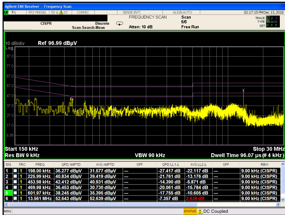
Plot 7-7. Line-Conducted Test Plot with Antenna attached (N)
