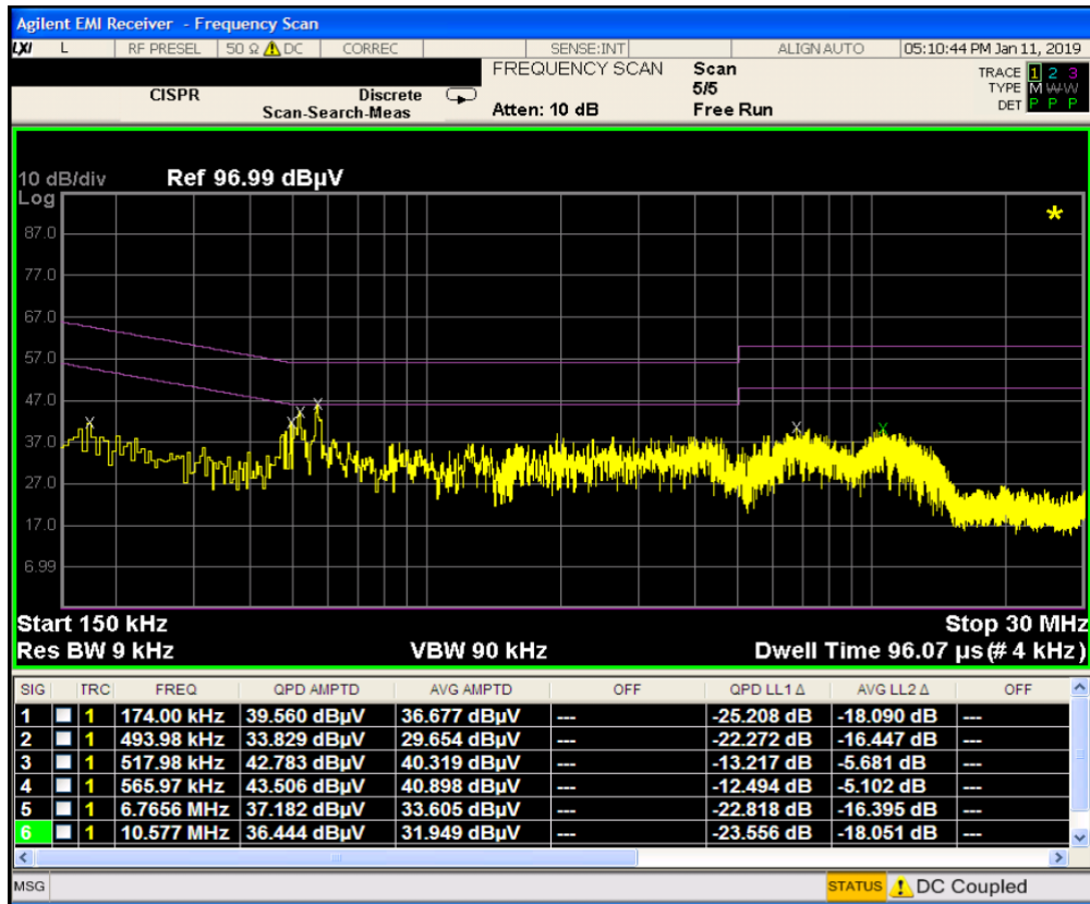
Plot 7-8. Line-Conducted Test Plot with Antenna Terminated at 50 Ohms(L1)
