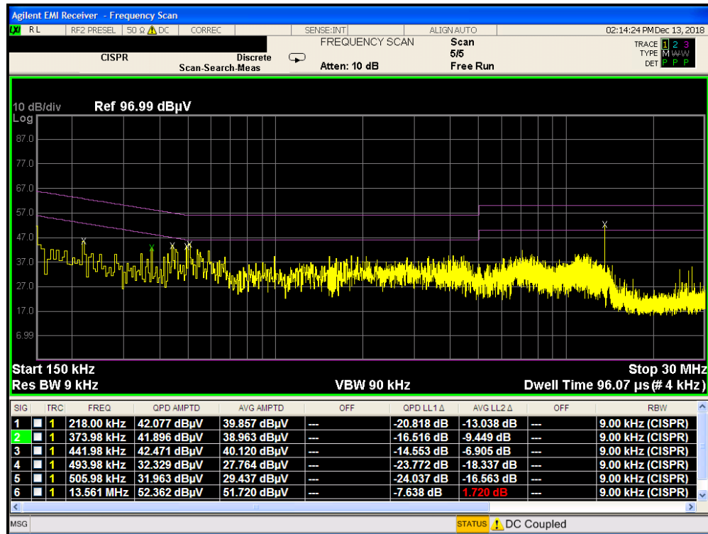
Plot 7-6. Line-Conducted Test Plot with Antenna attached (L1)
