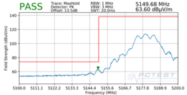
Plot 7-80. Radiated Lower Band Edge Plot MIMO (Peak – UNII Band 1)
