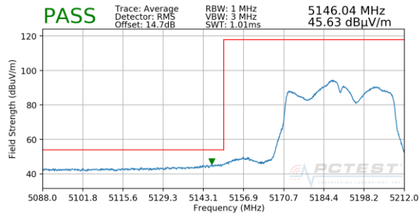
Plot 7-93. Radiated Band Edge Plot ANT (Average – WCP)
