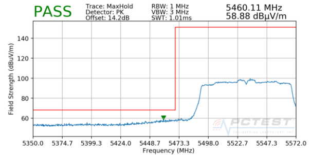
Plot 7-39. Radiated Lower Band Edge Plot SISO ANT1 (Peak – UNII Band 2C)
