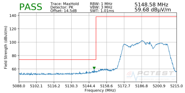
Plot 7-94. Radiated Band Edge Plot ANT (Peak – WCP)
