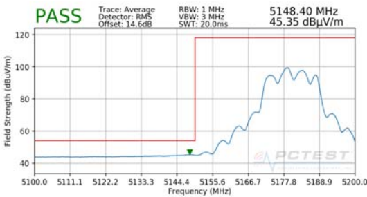
Plot 7-222. Radiated Lower Band Edge Plot (Average – UNII Band 1)
