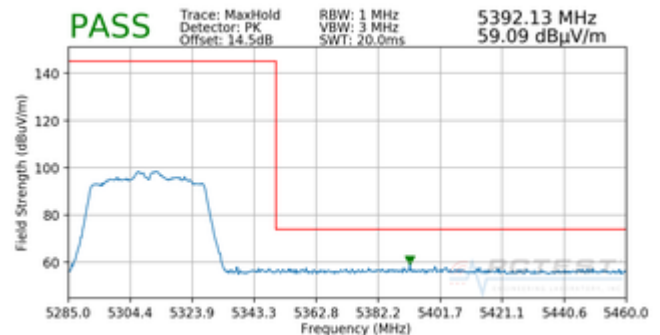
Plot 7-180. Radiated Upper Band Edge Plot (Peak – UNII Band 2A)
