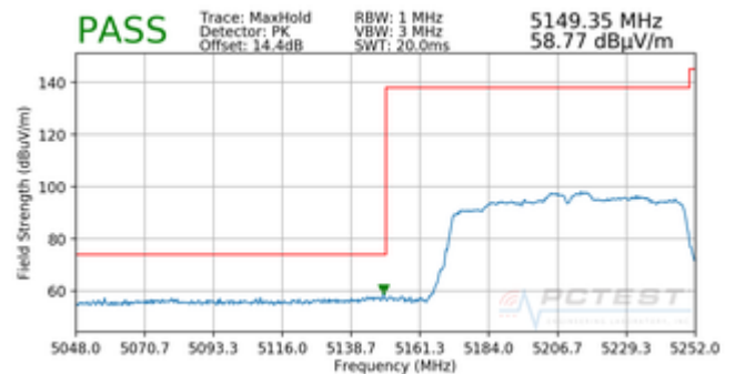
Plot 7-214. Radiated Lower Band Edge Plot (Peak – UNII Band 1)
