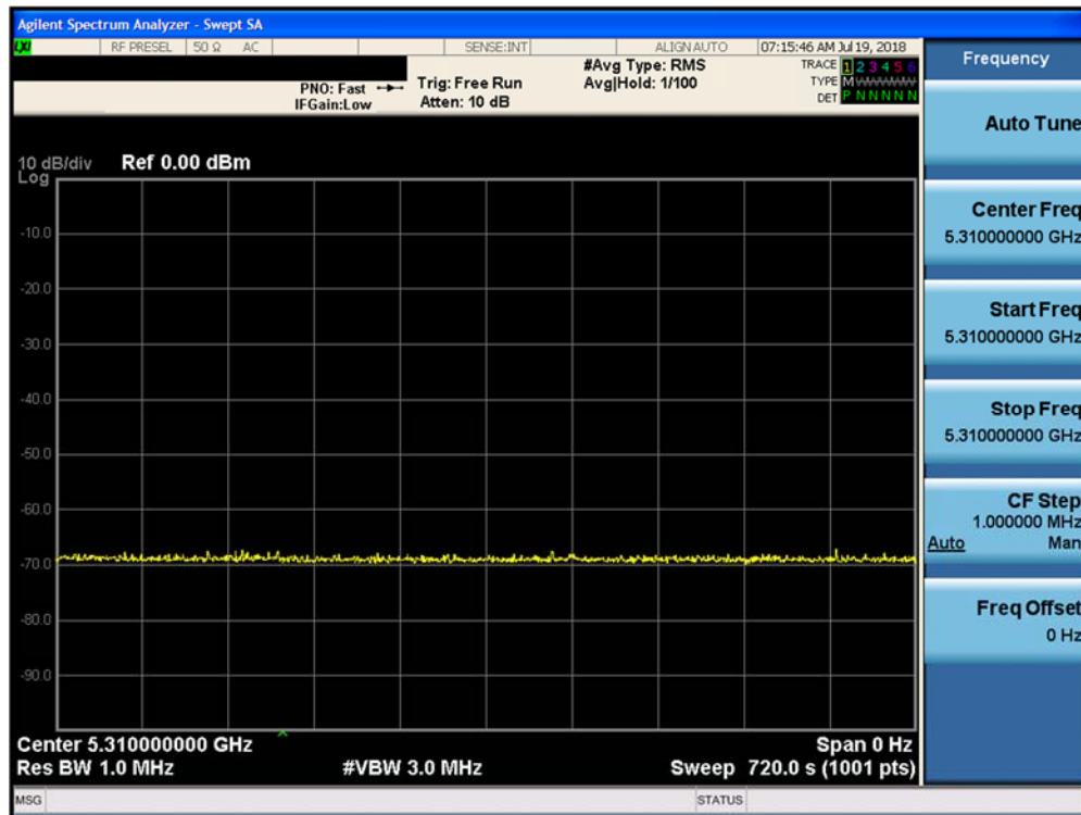
Figure 5-3. Band 2A Client Beacon Test – Monitoring live spectrum – Elapse time 10 minutes
