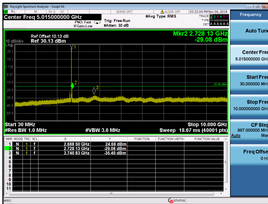
LTE Band 41 / 5MHz / QPSK - RB Size/Offset (12/13) – High Channel
