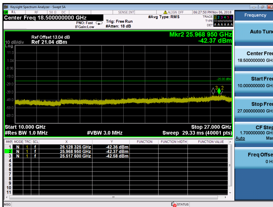
LTE Band 41 / 5MHz / 64QAM - RB Size/Offset (12/6) – Mid Channel
