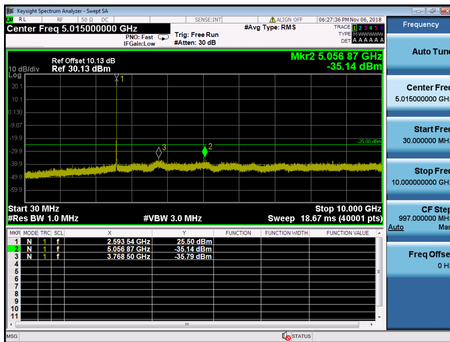
LTE Band 41 / 5MHz / 64QAM - RB Size/Offset (12/6) – Mid Channel
