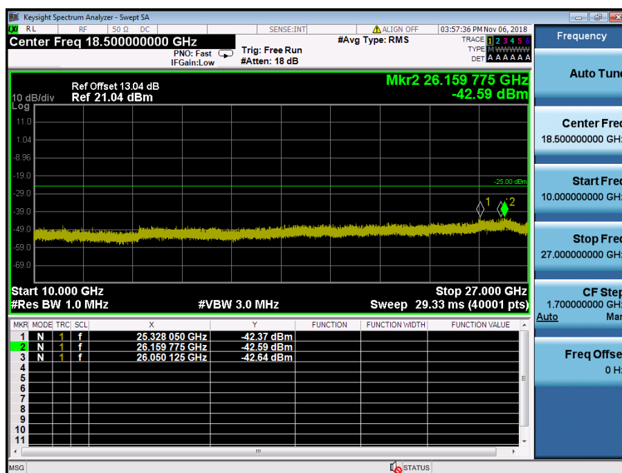
LTE Band 41 / 20MHz / QPSK - RB Size/Offset (100/0) – Low Channel
