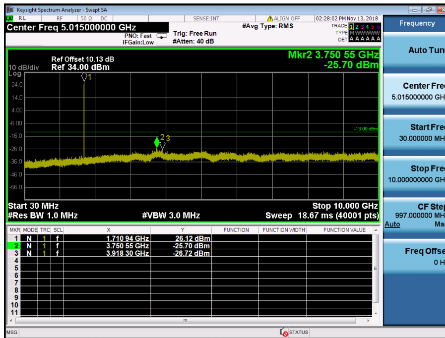
LTE Band 4 / 1.4MHz / 16QAM - RB Size/Offset (6/0) – Low Channel
