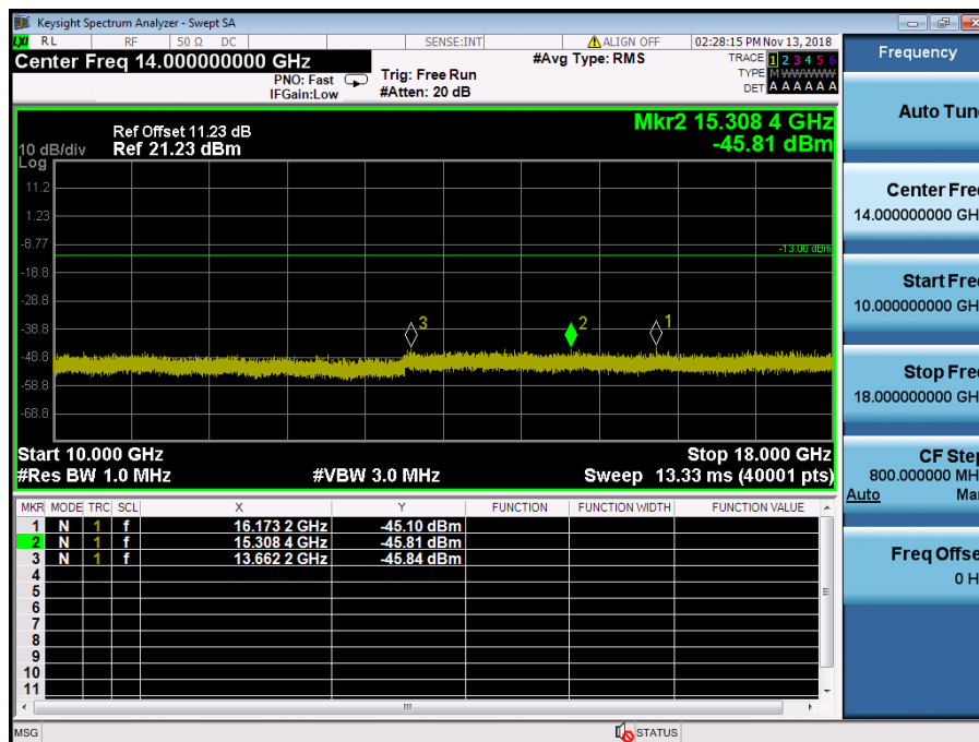
LTE Band 4 / 1.4MHz / 16QAM - RB Size/Offset (6/0) – Low Channel
