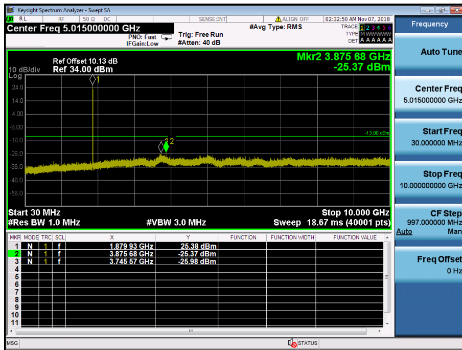
LTE Band 2 / 5MHz / 16QAM - RB Size/Offset (12/6) – Mid Channel
