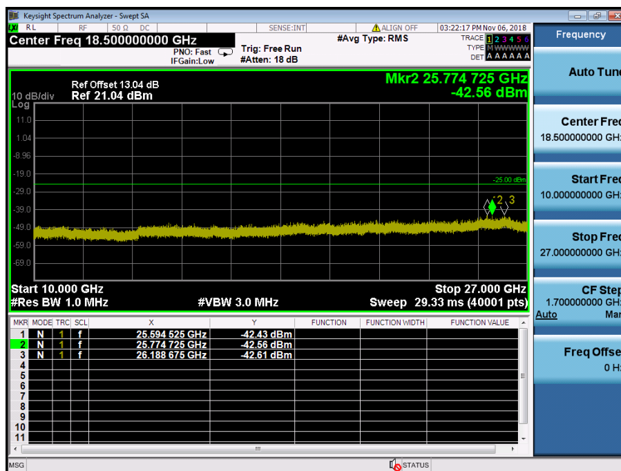
LTE Band 41 / 5MHz / QPSK - RB Size/Offset (12/13) – High Channel
