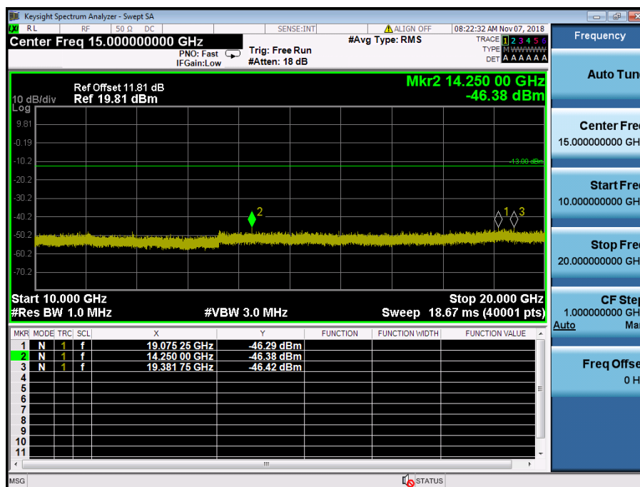
LTE Band 2 / 15MHz / 64QAM - RB Size/Offset (36/39) – Mid Channel
