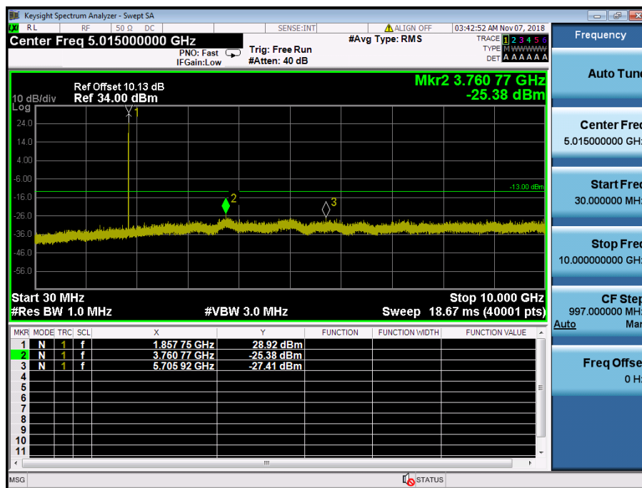
LTE Band 2 / 15MHz / 16QAM - RB Size/Offset (1/36)–Low Channel
