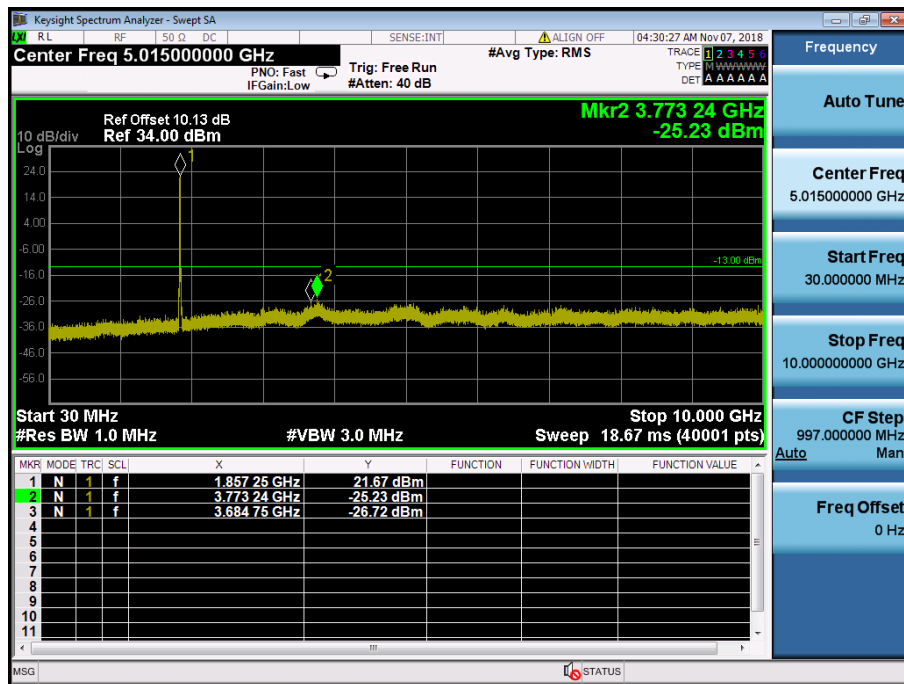
LTE Band 2 / 20MHz / 16QAM - RB Size/Offset (50/0) –Low Channel
