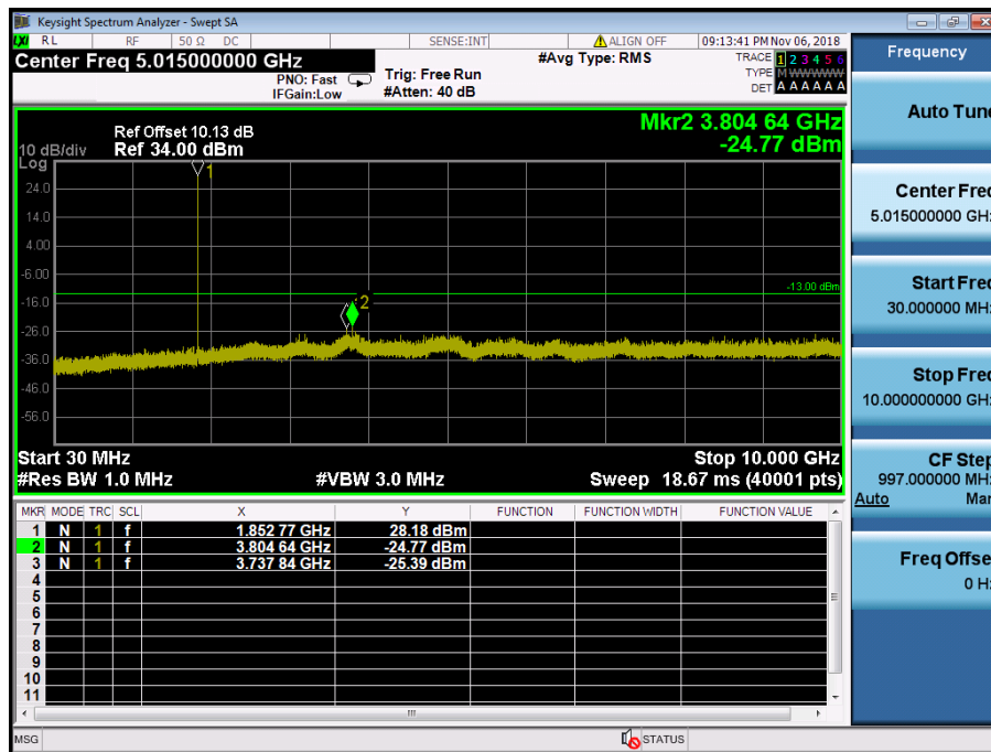
LTE Band 2 / 3MHz / QPSK - RB Size/Offset (1/14) – Low Channel
