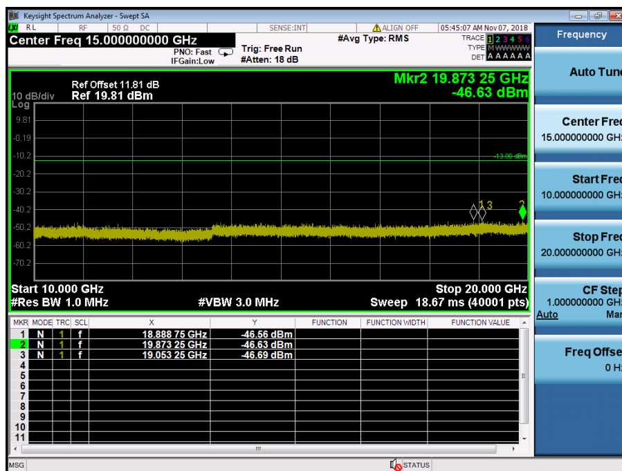
LTE Band 2 / 1.4MHz / 64QAM - RB Size/Offset (3/3) – High Channel
