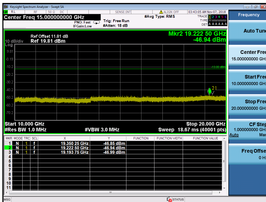
LTE Band 2 / 15MHz / 16QAM - RB Size/Offset (1/36)–Low Channel
