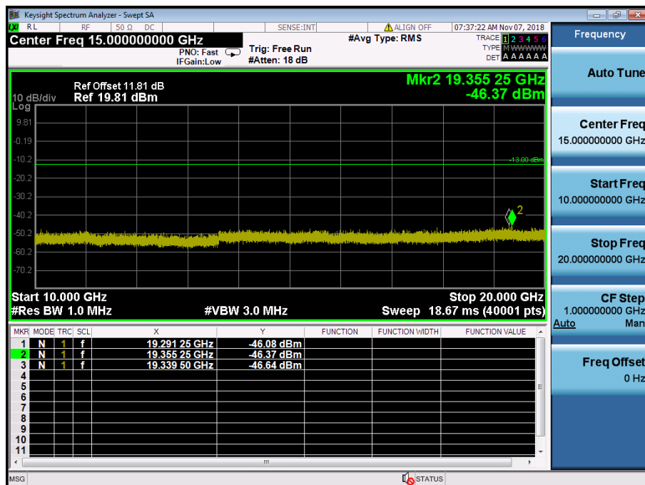
LTE Band 2 / 10MHz / 64QAM - RB Size/Offset (1/49) – Mid Channel
