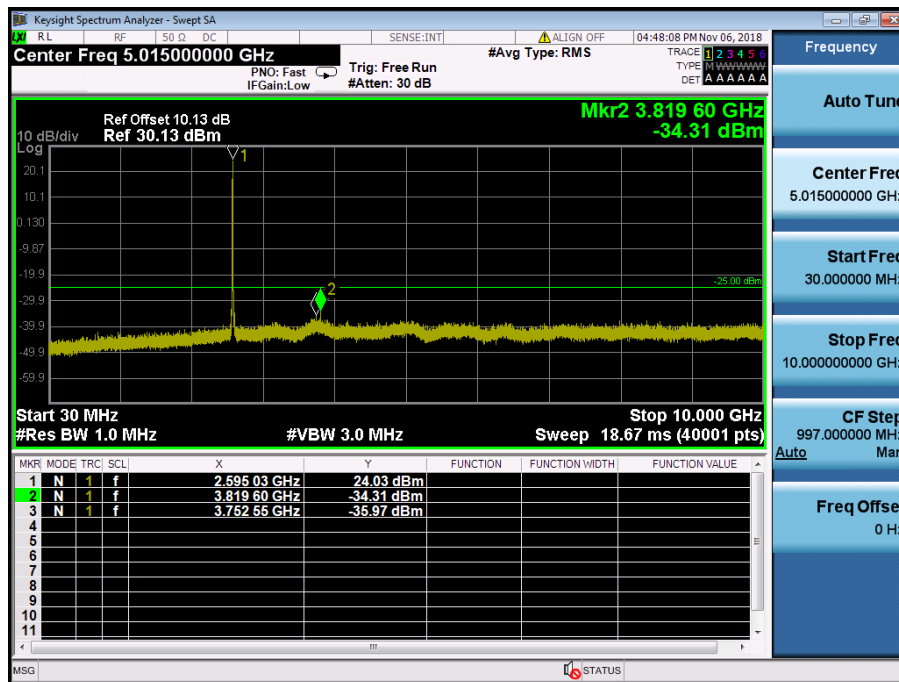
LTE Band 41 / 15MHz / 16QAM - RB Size/Offset (36/18) – Mid Channel
