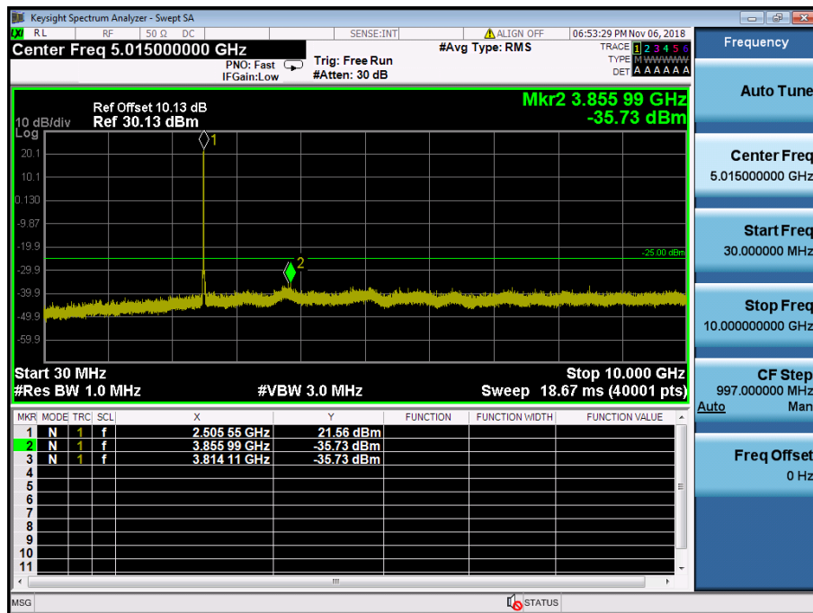
LTE Band 41 / 15MHz / 64QAM - RB Size/Offset (36/18) – Low Channel
