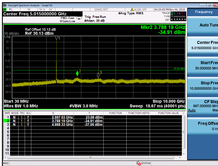
LTE Band 41 / 10MHz / 16QAM - RB Size/Offset (25/25) – Mid Channel
