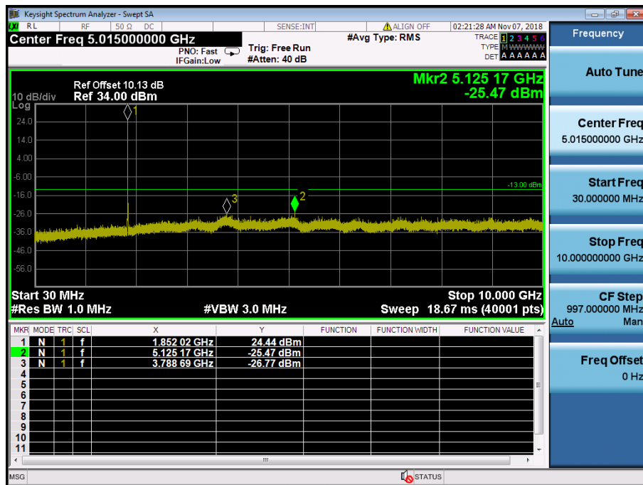
LTE Band 2 / 5MHz / 16QAM - RB Size/Offset (12/0) – Low Channel
