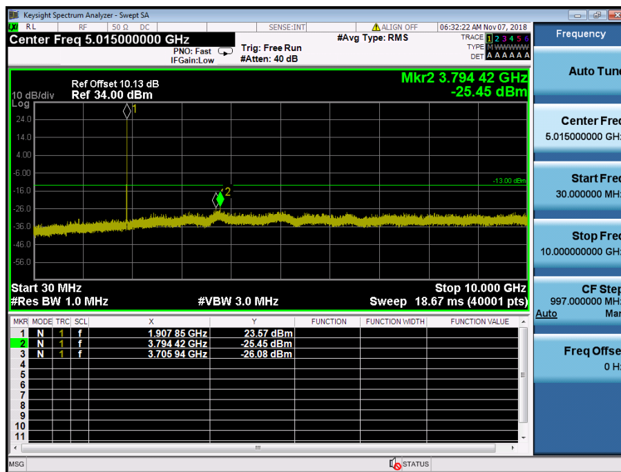
LTE Band 2 / 3MHz / 64QAM - RB Size/Offset (15/0) – High Channel
