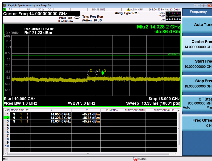
LTE Band 4 / 3MHz / 16QAM - RB Size/Offset (1/14) – High Channel
