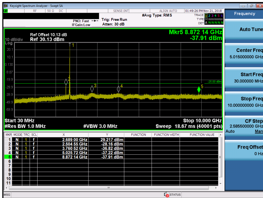
LTE Band 41 / 20MHz / QPSK - RB Size/Offset (1/99) – High Channel
