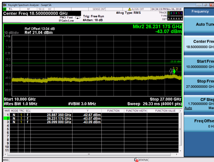
LTE Band 41 / 10MHz / 16QAM - RB Size/Offset (25/25) – Mid Channel
