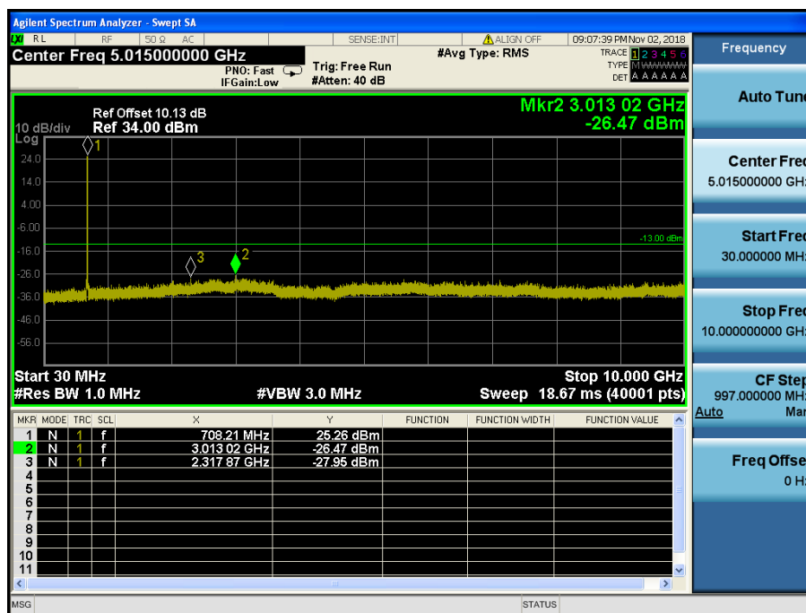
LTE Band 12,17 / 5MHz / 64QAM - RB Size/Offset (25/0) – Mid Channel
