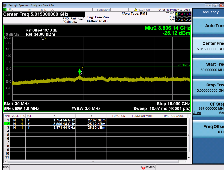
LTE Band 4 / 5MHz / 16QAM - RB Size/Offset (1/24) – High Channel
