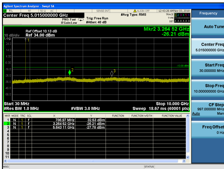
LTE Band 13 / 5MHz / 64QAM - RB Size/Offset (1/24) – High Channel
