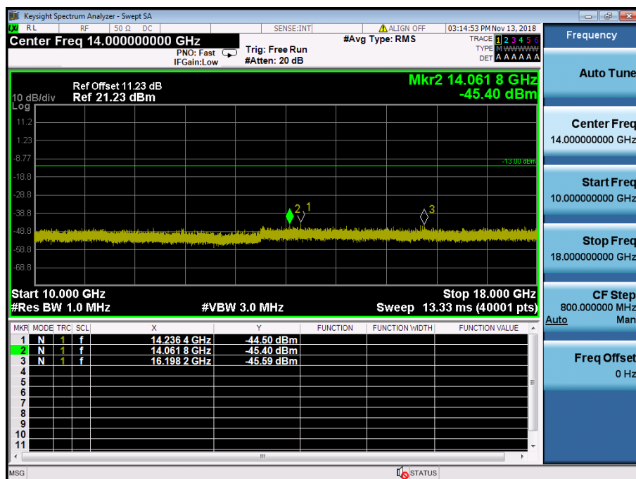
LTE Band 4 / 3MHz / 16QAM - RB Size/Offset (8/0) – Mid Channel
