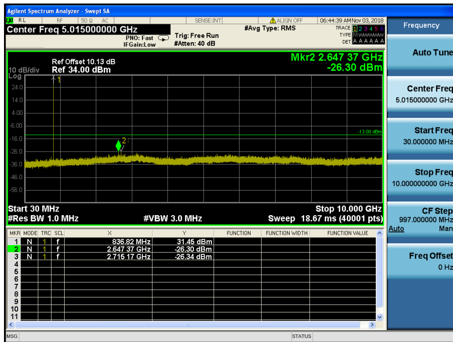
LTE Band 5 / 1.4MHz / 64QAM - RB Size/Offset (1/2) – Mid Channel
