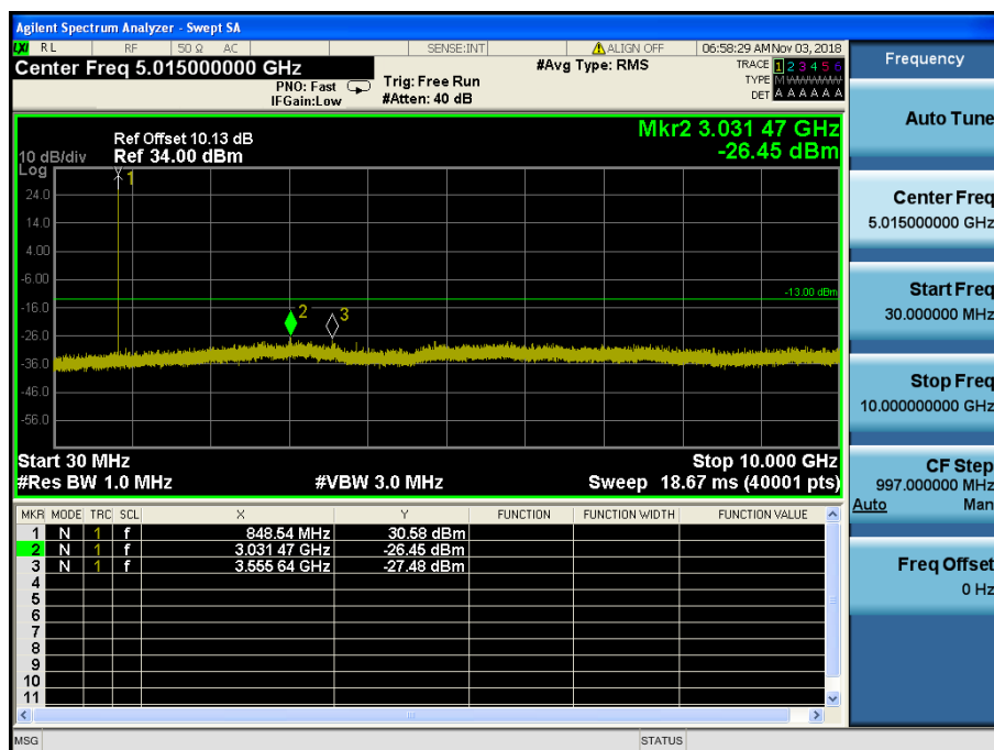
LTE Band 5 / 1.4MHz / 64QAM - RB Size/Offset (3/2) – High Channel
