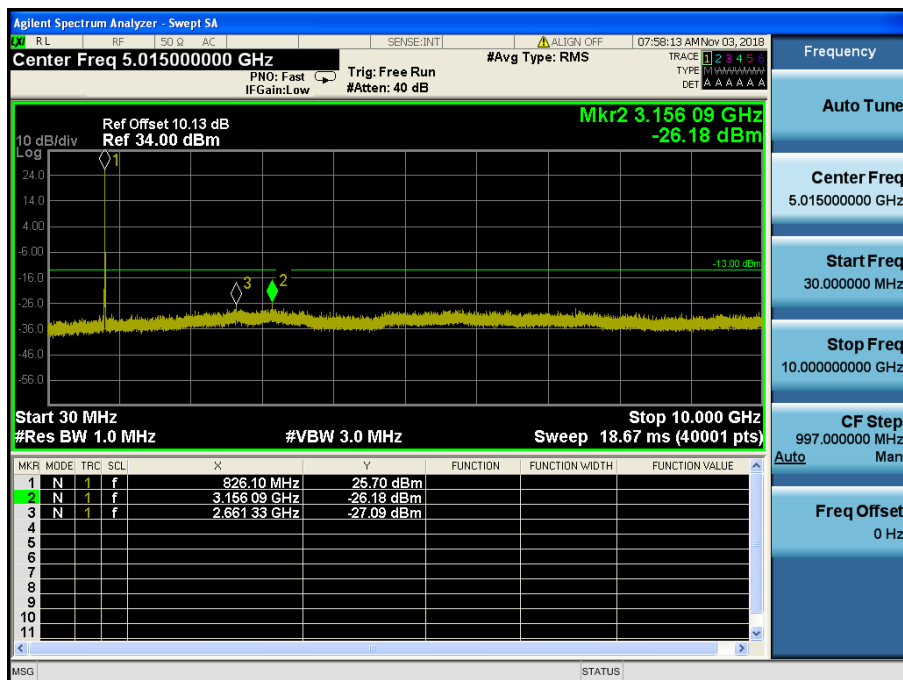
LTE Band 5 / 5MHz / 64QAM - RB Size/Offset (25/0) – Low Channel
