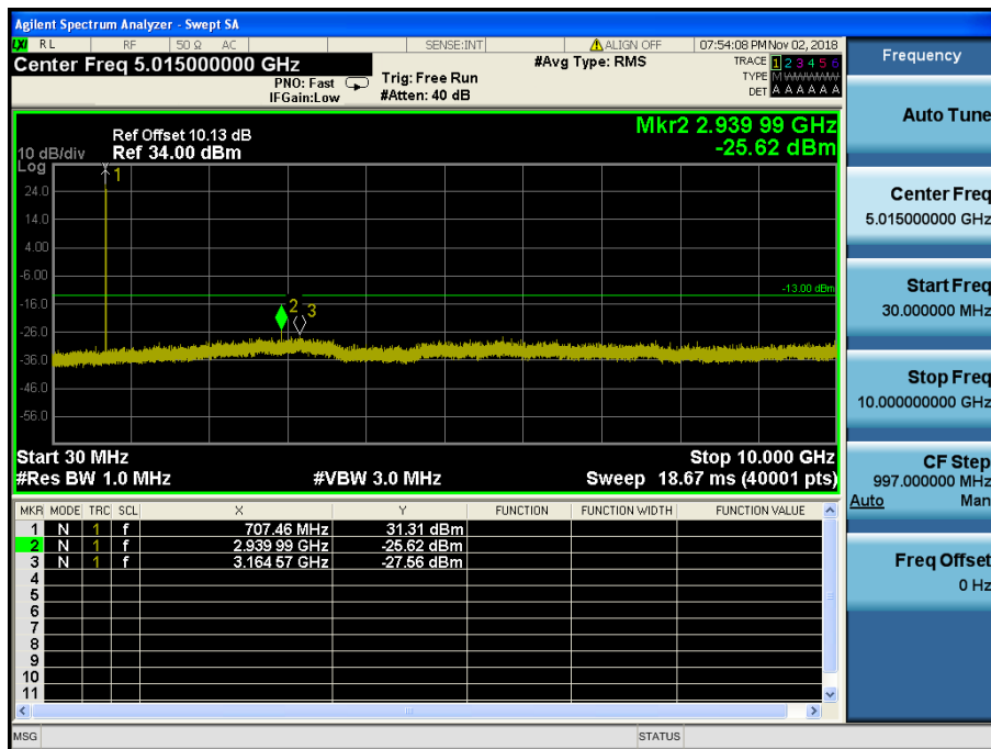
LTE Band 12 / 1.4MHz / 64QAM - RB Size/Offset (3/0) – Mid Channel
