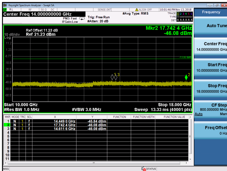
LTE Band 4 / 15MHz / 64QAM - RB Size/Offset (75/0) – Mid Channel
