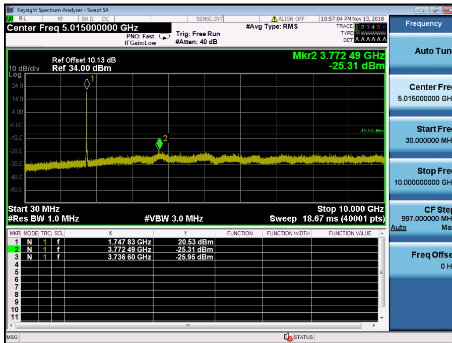
LTE Band 4 / 20MHz / 64QAM - RB Size/Offset (50/25) – High Channel
