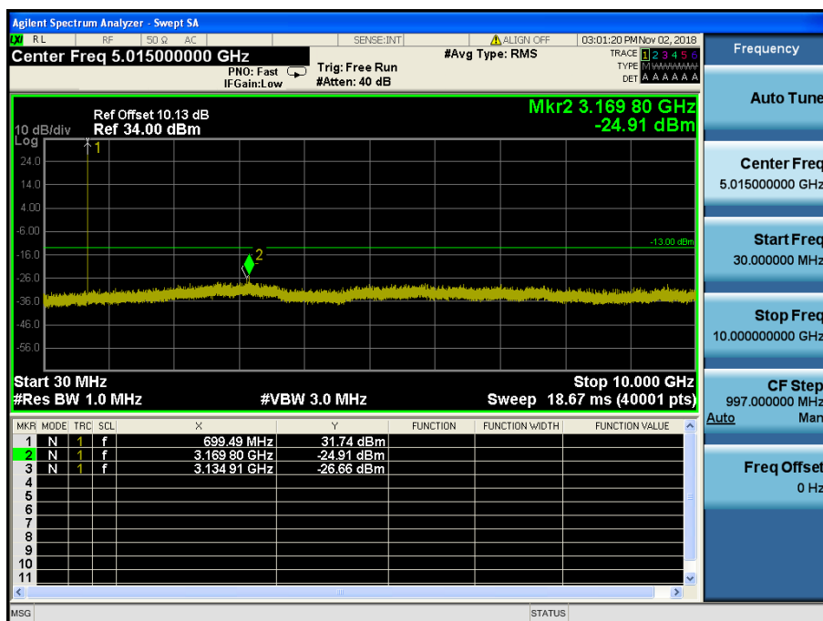
LTE Band 12 / 1.4MHz / QPSK - RB Size/Offset (1/0) – Low Channel
