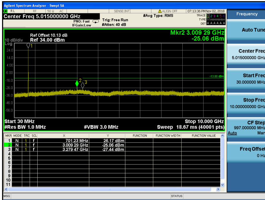
LTE Band 12,17 / 10MHz / 16QAM - RB Size/Offset (25/0) – Low Channel
