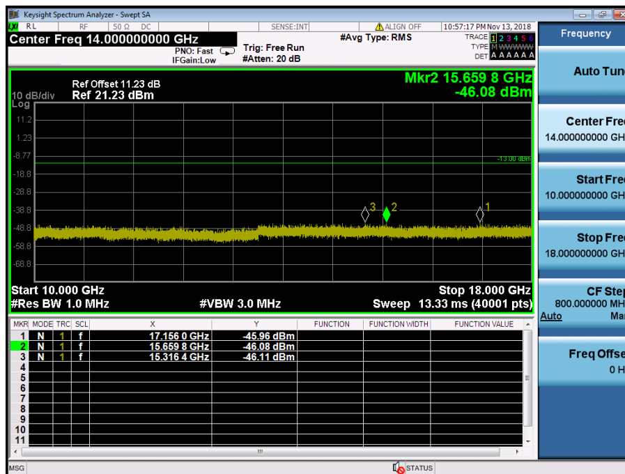
LTE Band 4 / 20MHz / 64QAM - RB Size/Offset (50/25) – High Channel
