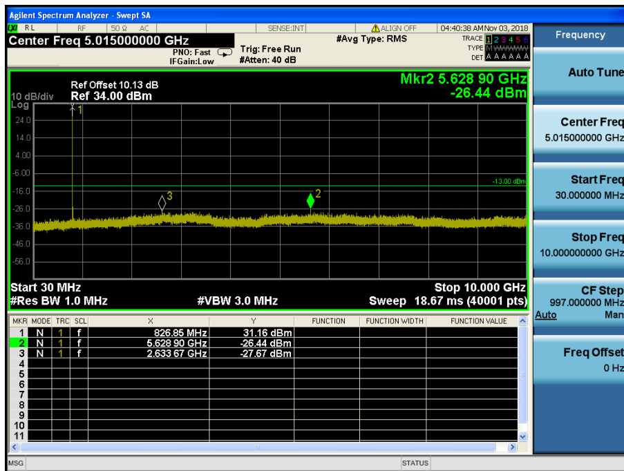
LTE Band 5 / 3MHz / 16QAM - RB Size/Offset (1/14) – Low Channel
