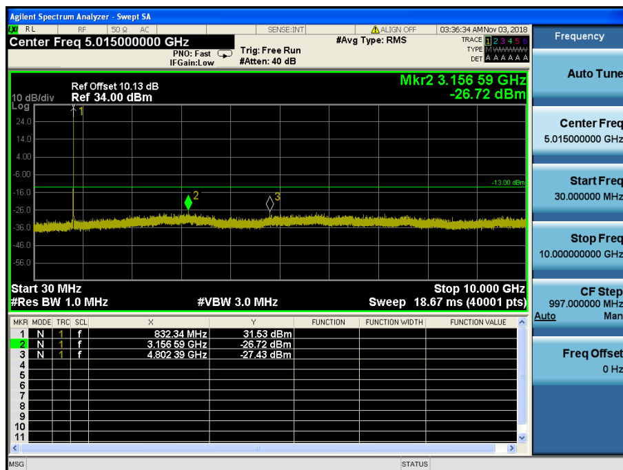
LTE Band 5 / 10MHz / QPSK - RB Size/Offset (1/0) – Mid Channel
