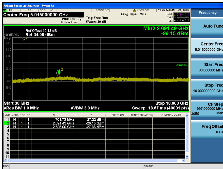
LTE Band 12 / 3MHz / QPSK - RB Size/Offset (15/0) – Low Channel
