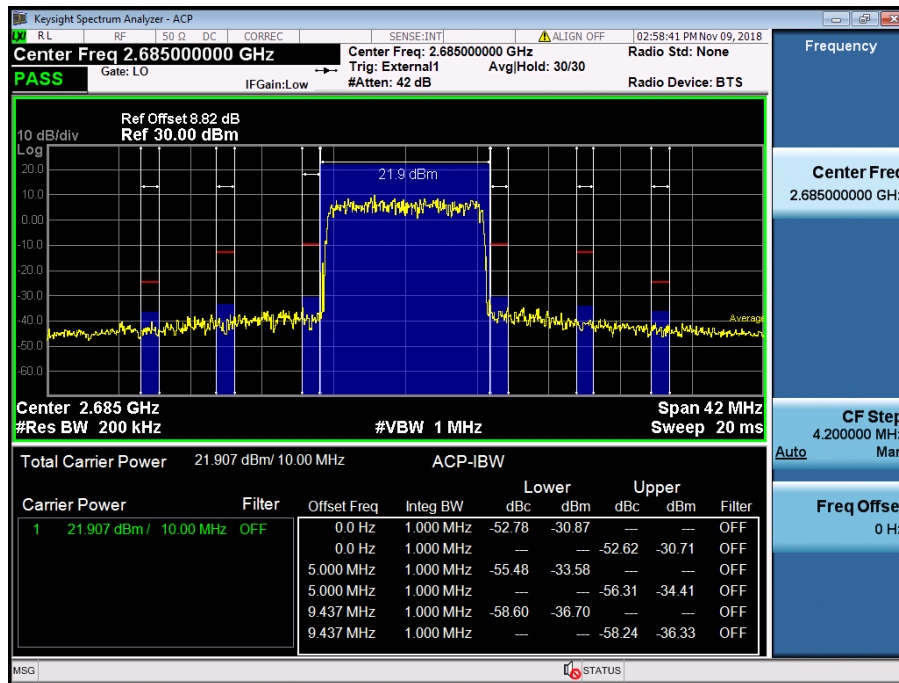
LTE Band 41 / 10MHz / 64QAM - RB Size/Offset (50/0)
