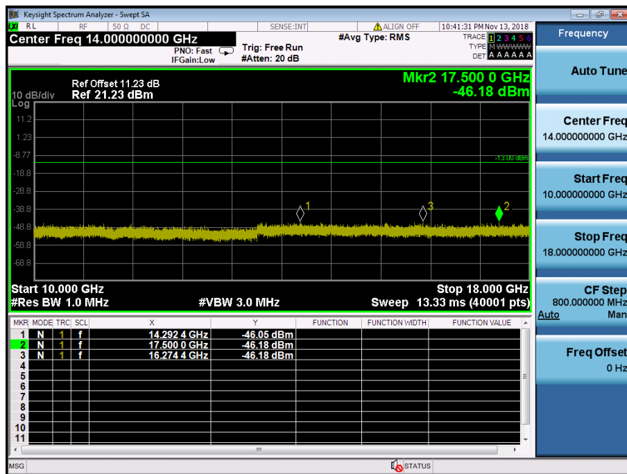
LTE Band 4 / 20MHz / QPSK - RB Size/Offset (1/99)–Mid Channel
