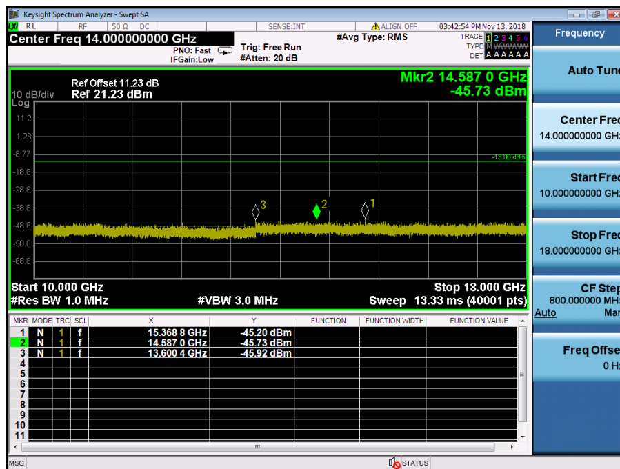
LTE Band 4 / 5MHz / 16QAM - RB Size/Offset (1/12) – Low Channel
