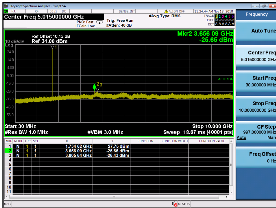
LTE Band 4 / 5MHz / QPSK - RB Size/Offset (1/24) – Mid Channel
