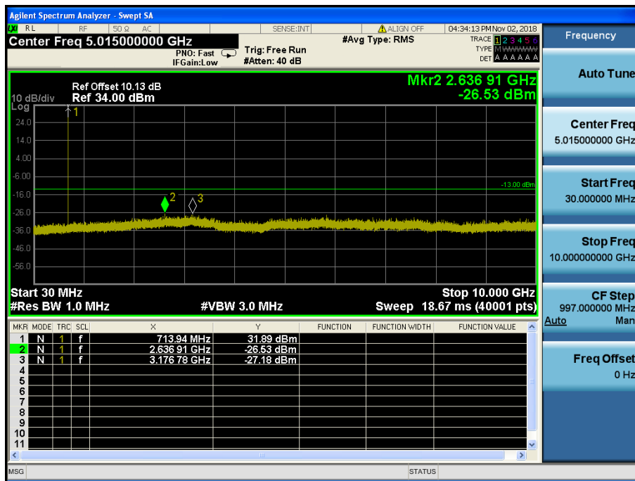
LTE Band 12,17 / 5MHz / QPSK - RB Size/Offset (1/12) – High Channel
