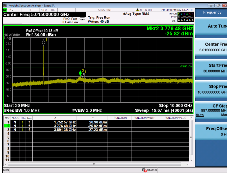
LTE Band 4 / 10MHz / 64QAM - RB Size/Offset (25/25) – High Channel
