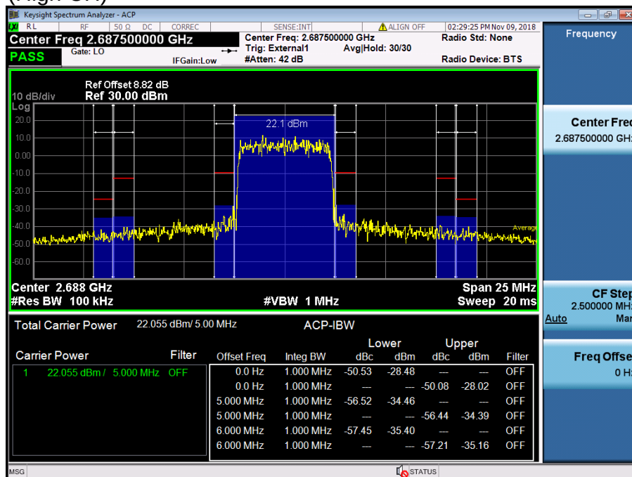
LTE Band 41 / 5MHz / 64QAM - RB Size/Offset (15/0)
