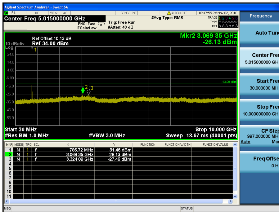
LTE Band 13 / 10MHz / QPSK - RB Size/Offset (1/49) – Low Channel
