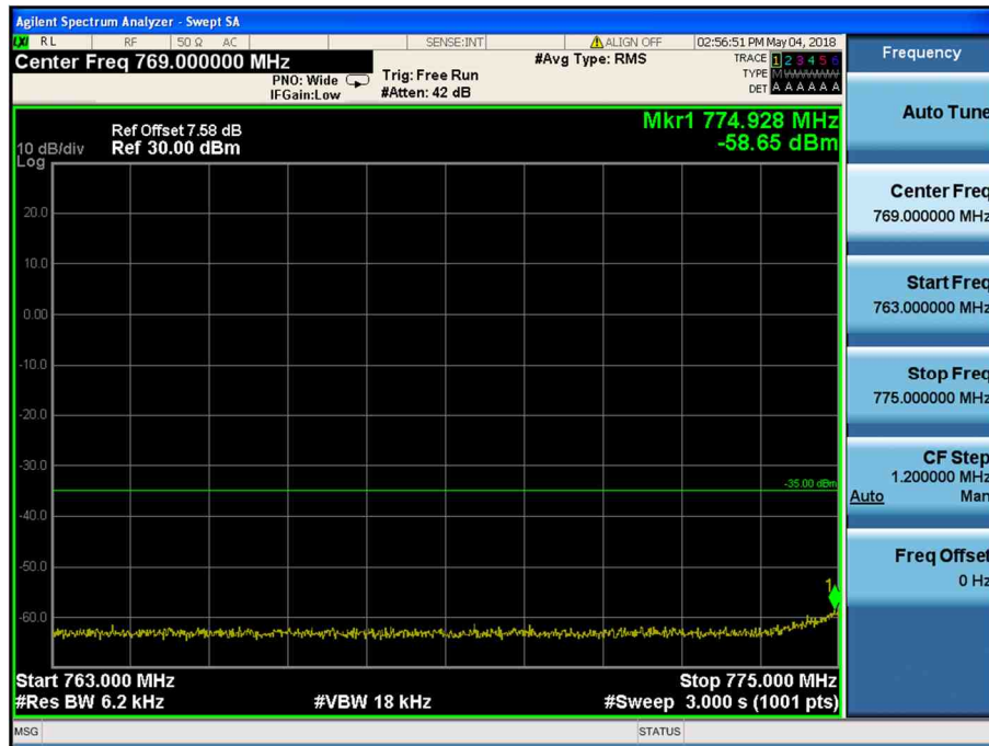
LTE Band 13 / 10MHz / 16QAM - RB Size/Offset (25/0)
