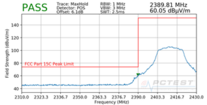
Plot 7-20. Radiated Restricted Band Edge Measurement SISO ANT2 with WCP (Peak)
