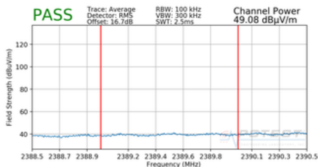
Plot 7-27. Radiated Restricted Lower Band Edge Measurement CDD (Average)
