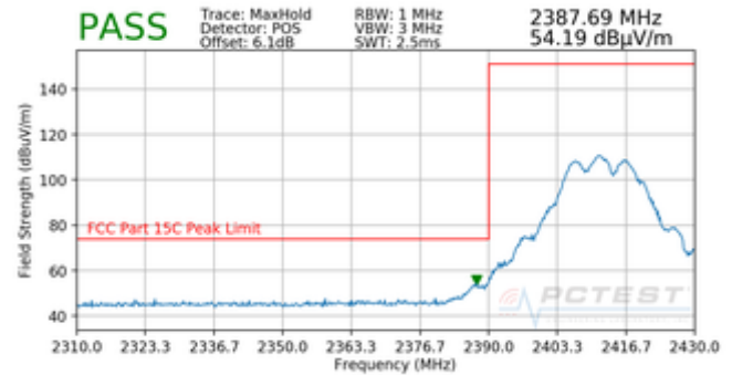
Plot 7-32. Radiated Restricted Band Edge Measurement CDD with WCP (Peak)
