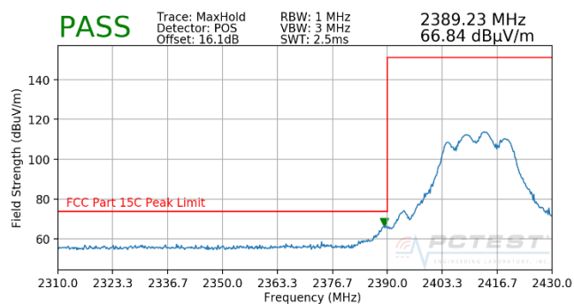
Plot 7-28. Radiated Restricted Lower Band Edge Measurement CDD (Peak)
