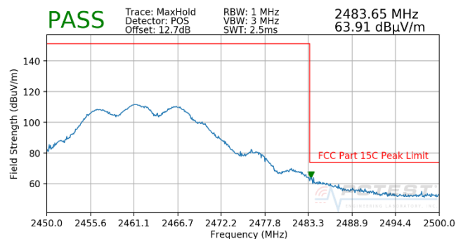
Plot 7-30. Radiated Restricted Upper Band Edge Measurement CDD (Peak)
