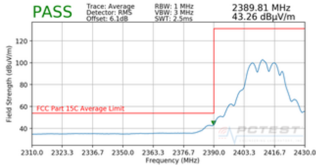
Plot 7-31. Radiated Restricted Band Edge Measurement CDD with WCP (Average)
