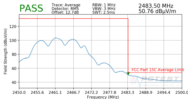
Plot 7-29. Radiated Restricted Upper Band Edge Measurement CDD (Average)
