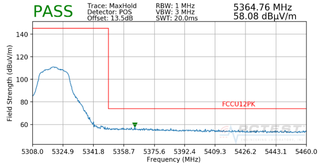
Plot 7-46. Radiated Upper Band Edge Plot SISO ANT2 (Peak – UNII Band 2A)
