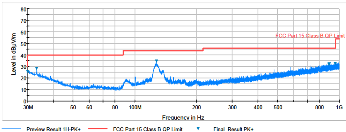
Plot 7-95. Radiated Spurious Plot below 1GHz (2.4GHz – 5GHz, Ant. Pol. V)
