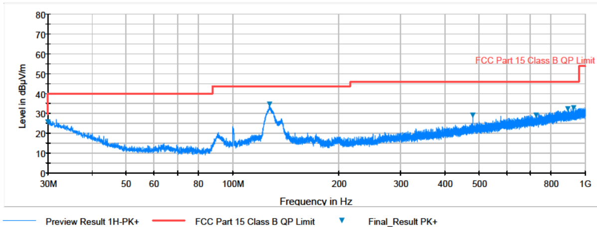
Plot 7-94. Radiated Spurious Plot below 1GHz (2.4GHz – 5GHz, Ant. Pol. H)
