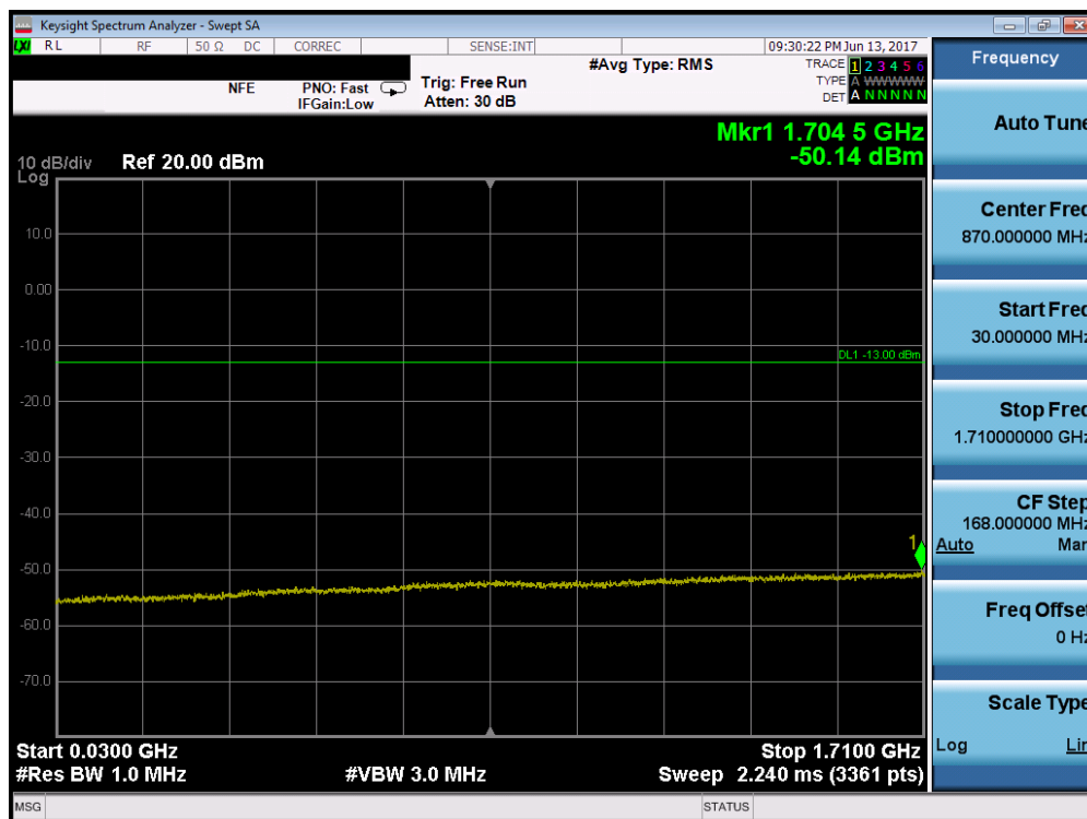
Plot 7-124. Conducted Spurious Plot (Band 4/66 – 5.0MHz QPSK – RB Size 1, RB Offset 0 – High Channel)
