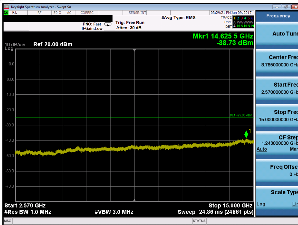
Plot 7-149. Conducted Spurious Plot (Band 7 – 10.0MHz QPSK – RB Size 1, RB Offset 0 – Mid Channel)
