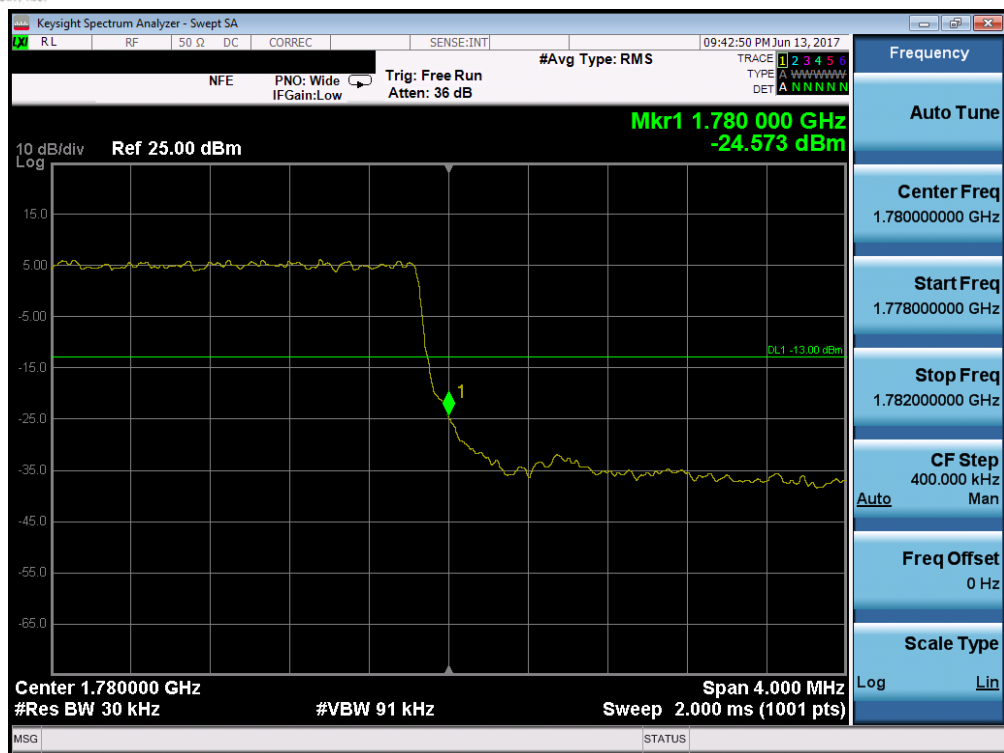
Plot 7-197. Upper Band Edge Plot (Band 66 – 3.0MHz QPSK – RB Size 15)
