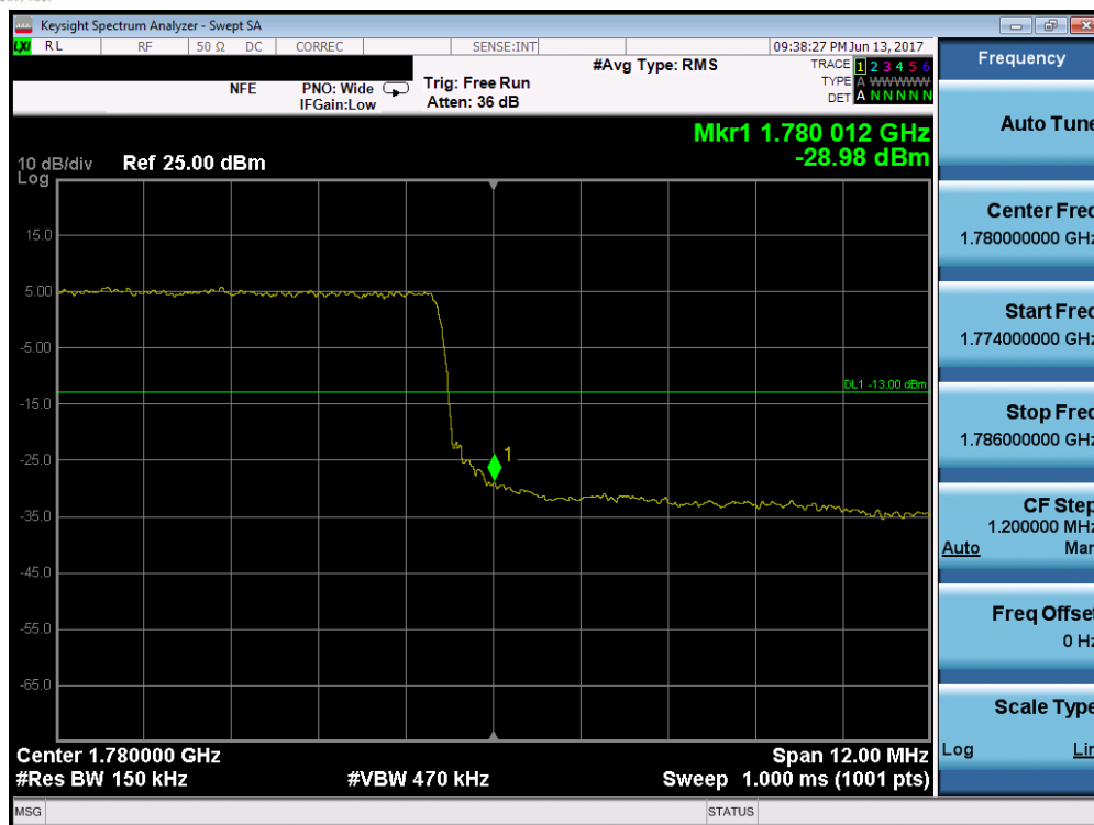
Plot 7-215. Upper Band Edge Plot (Band 66 – 15.0MHz QPSK – RB Size 75)
