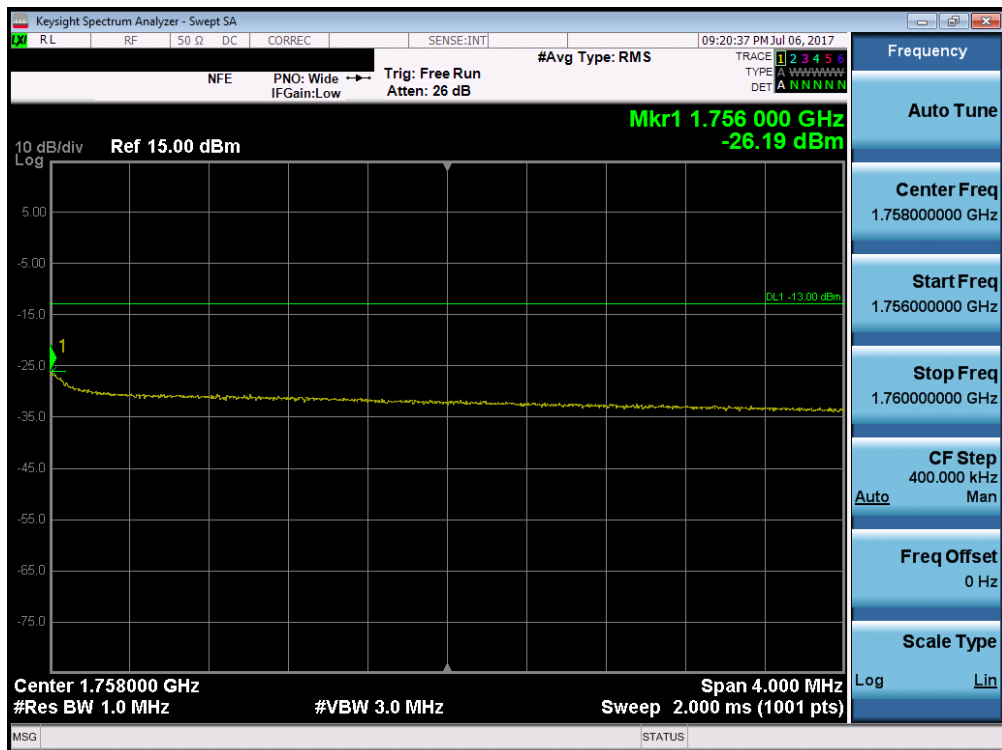
Plot 7-212. Upper Extended Band Edge Plot (Band 4 – 10.0MHz QPSK – RB Size 50)
