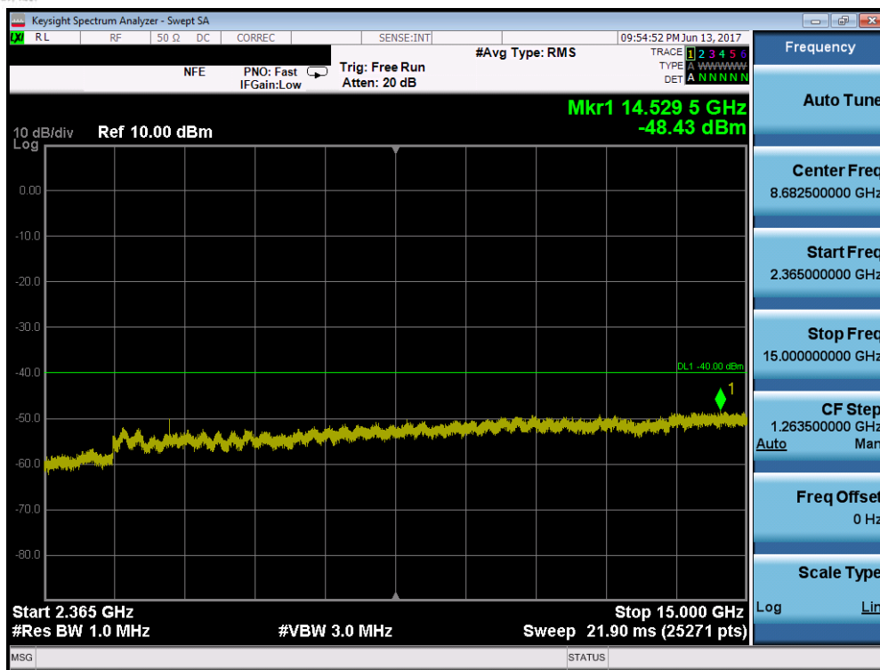
Plot 7-137. Conducted Spurious Plot (Band 30 – 5.0MHz QPSK – RB Size 1, RB Offset 0 – Low Channel)
