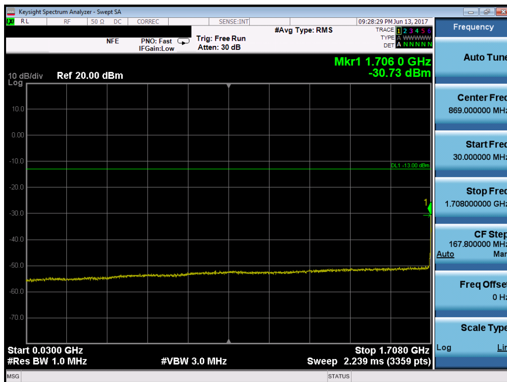
Plot 7-118. Conducted Spurious Plot (Band 4/66 – 5.0MHz QPSK – RB Size 1, RB Offset 0 – Low Channel)
