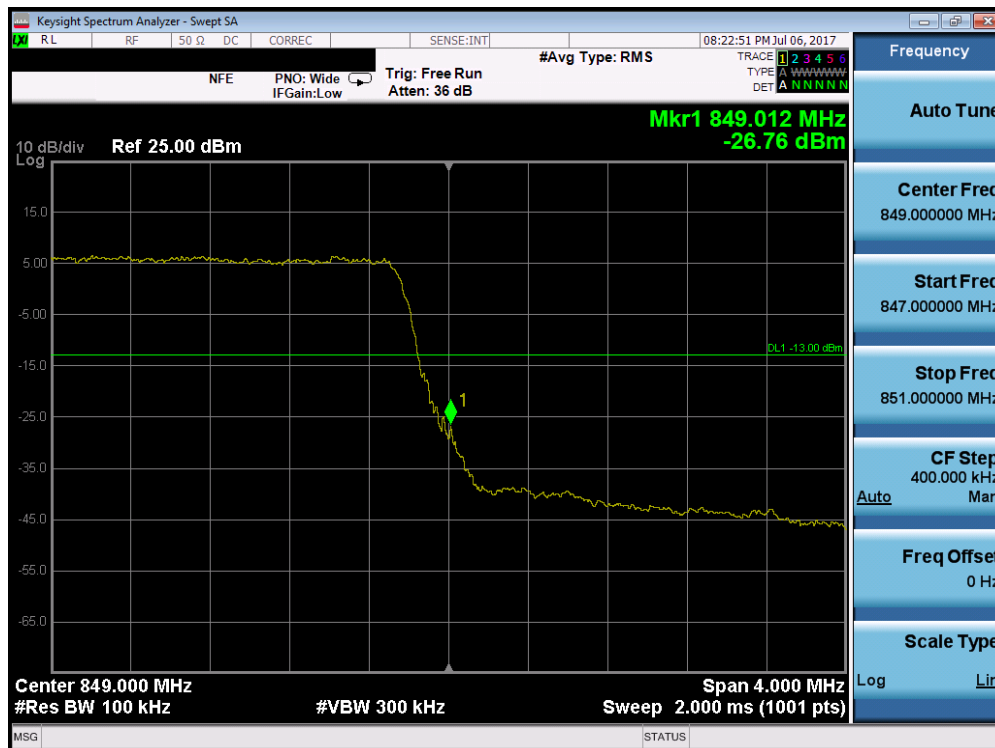
Plot 7-186. Upper Band Edge Plot (Band 5 - 5.0MHz QPSK - RB Size 25)
