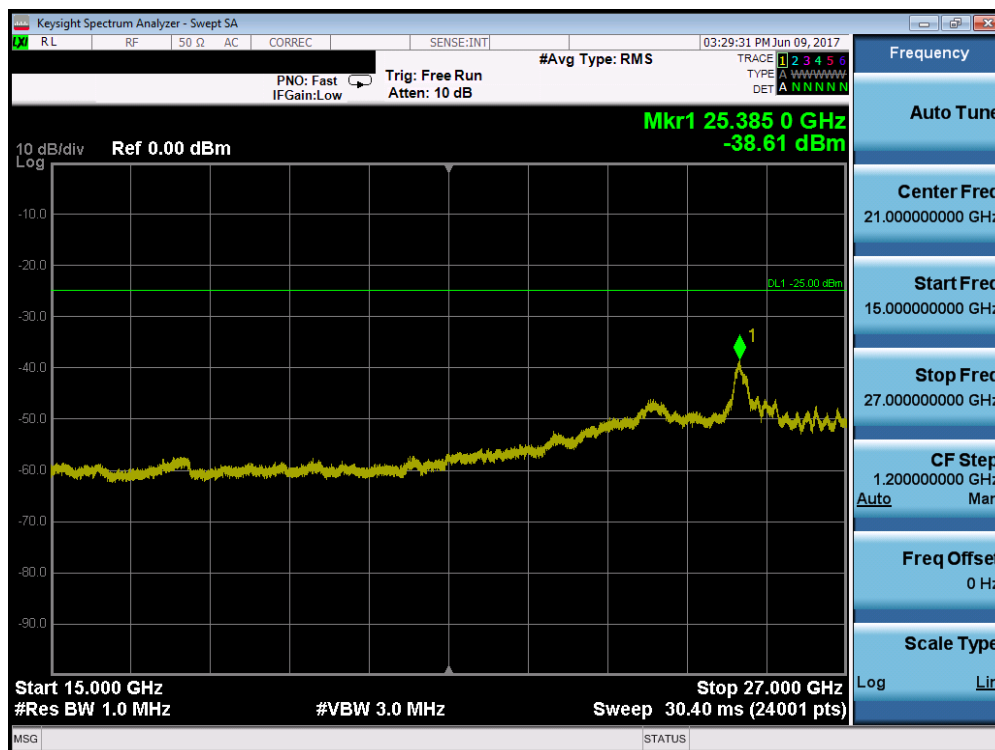
Plot 7-150. Conducted Spurious Plot (Band 7 – 10.0MHz QPSK – RB Size 1, RB Offset 0 – Mid Channel)
