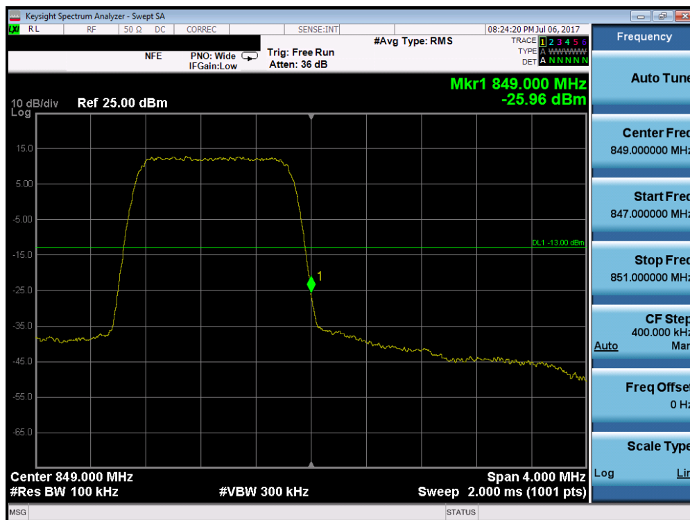
Plot 7-182. Upper Band Edge Plot (Band 5 – 1.4MHz QPSK – RB Size 6)
