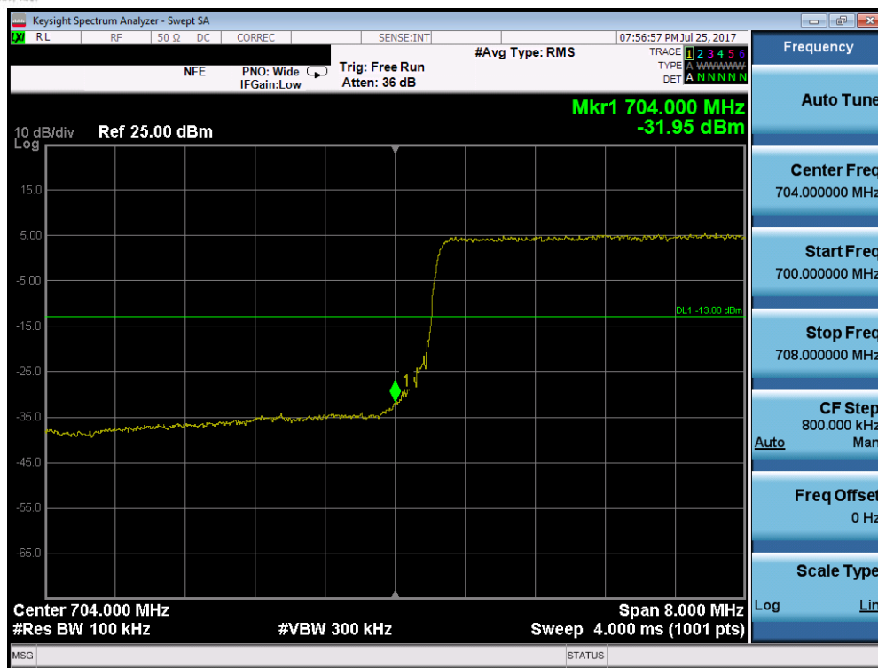
Plot 7-171. Lower Band Edge Plot (Band 17 – 10.0MHz QPSK – RB Size 50)
