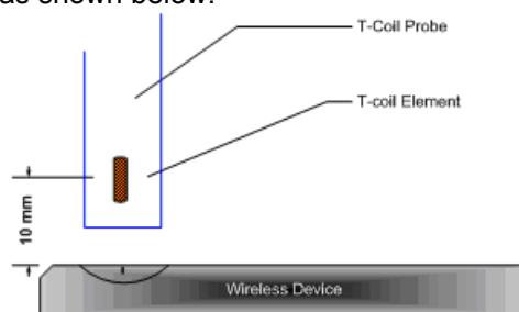
Figure 4-11 Measurement Distance
