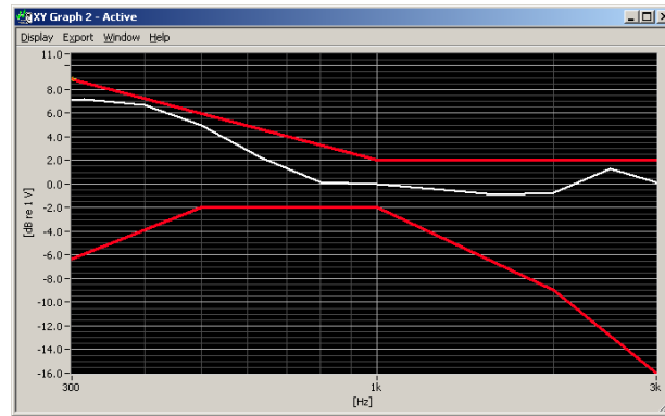
Figure 6-1 Axial Frequency Response
