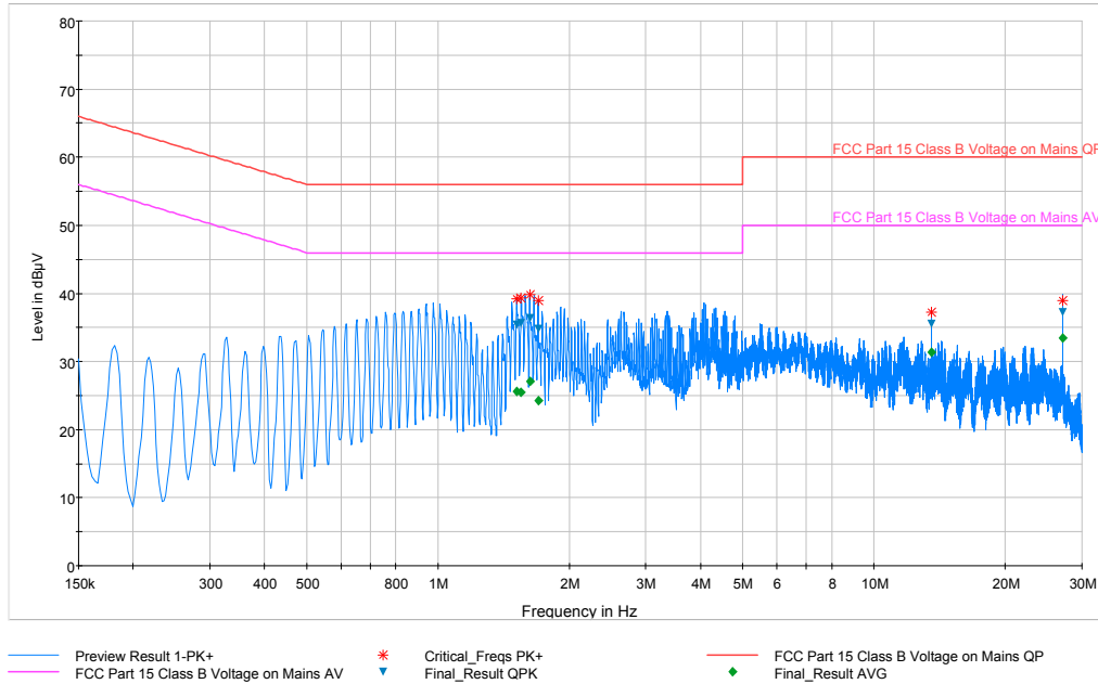
Plot 8-1. Line-Conducted Test Plot (L1)
