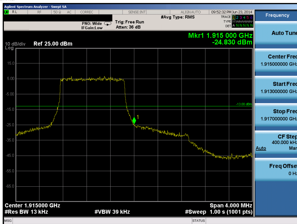
Plot 6-219. Upper Band Edge Plot (Band 25 – 1.4MHz QPSK – RB Size 6)
