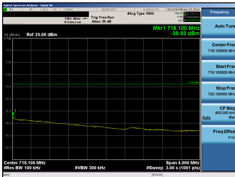
Plot 6-168. Upper Extended Band Edge Plot (Band 12 – 3.0MHz QPSK – RB Size 15)
