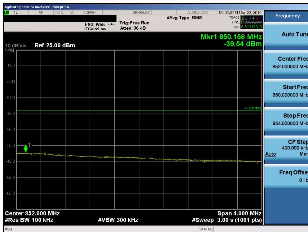
Plot 6-192. Upper Extended Band Edge Plot (Band 5 – 10.0MHz QPSK – RB Size 50)
