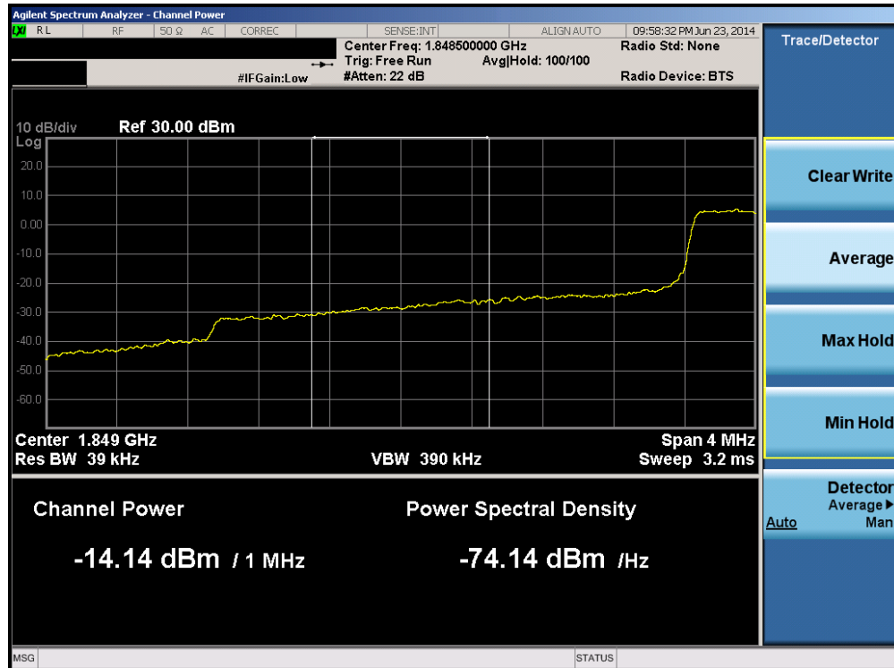
Plot 6-222. Lower Extended Band Edge Plot (Band 25 – 3.0MHz QPSK – RB Size 15)
