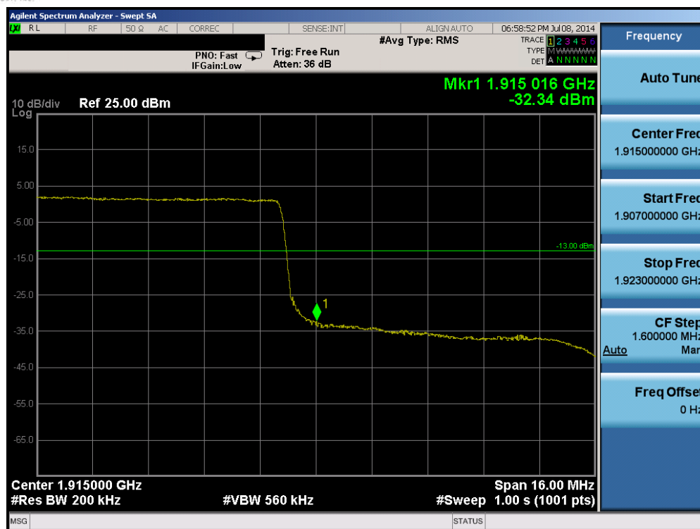
Plot 6-239. Upper Band Edge Plot (Band 25 - 20.0MHz QPSK - RB Size 100)
