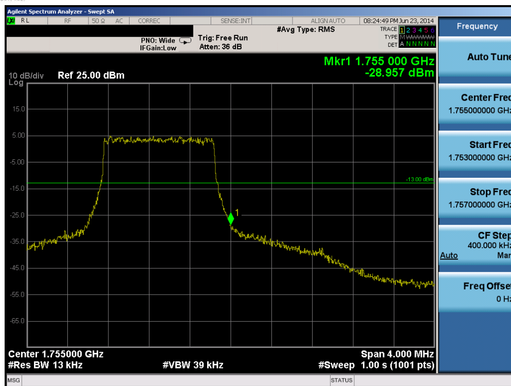
Plot 6-195. Upper Band Edge Plot (Band 4 – 1.4MHz QPSK – RB Size 6)
