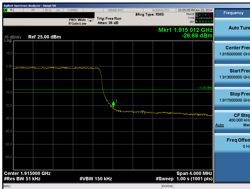
Plot 6-227. Upper Band Edge Plot (Band 25 – 5.0MHz QPSK – RB Size 25)
