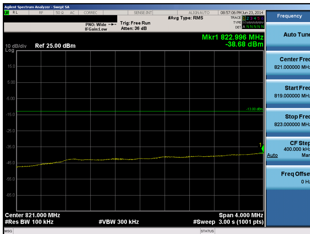
Plot 6-186. Lower Extended Band Edge Plot (Band 5 – 5.0MHz QPSK – RB Size 25)
