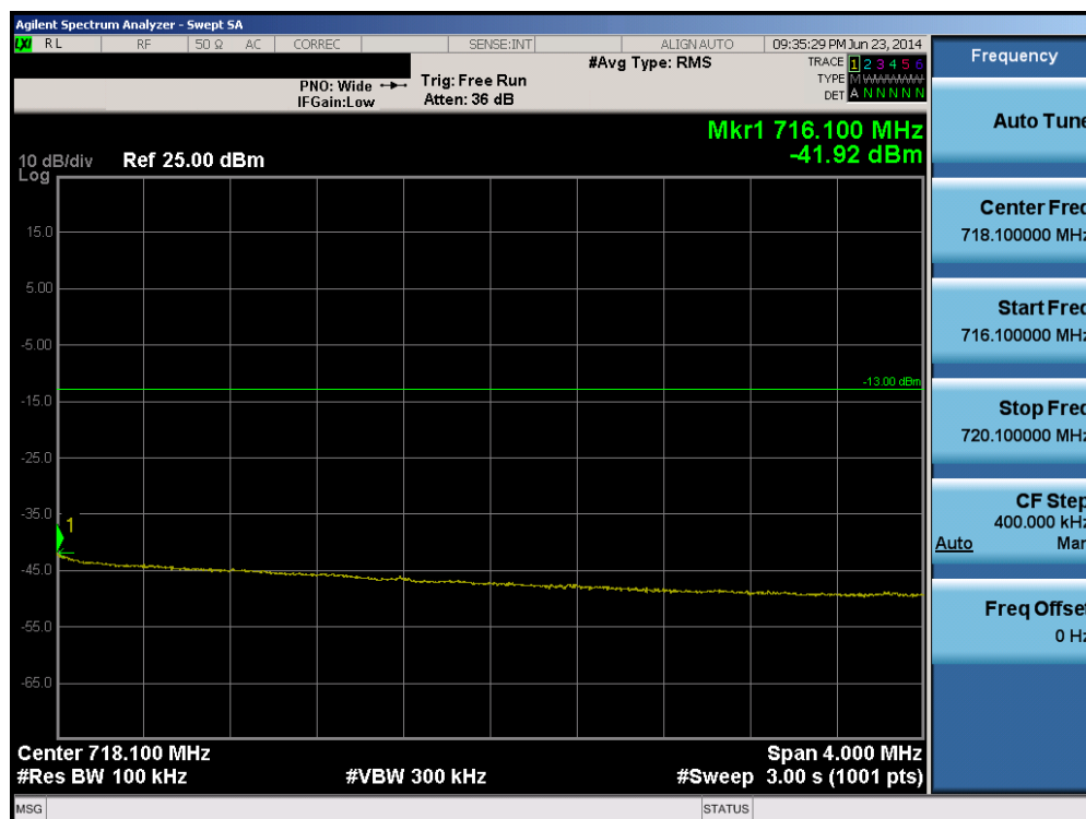
Plot 6-176. Upper Extended Band Edge Plot (Band 12 – 10.0MHz QPSK – RB Size 50)
