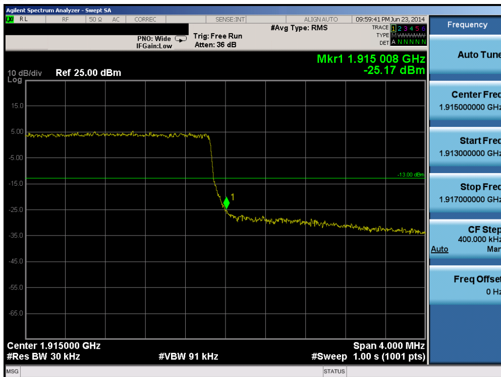
Plot 6-223. Upper Band Edge Plot (Band 25 – 3.0MHz QPSK – RB Size 15)
