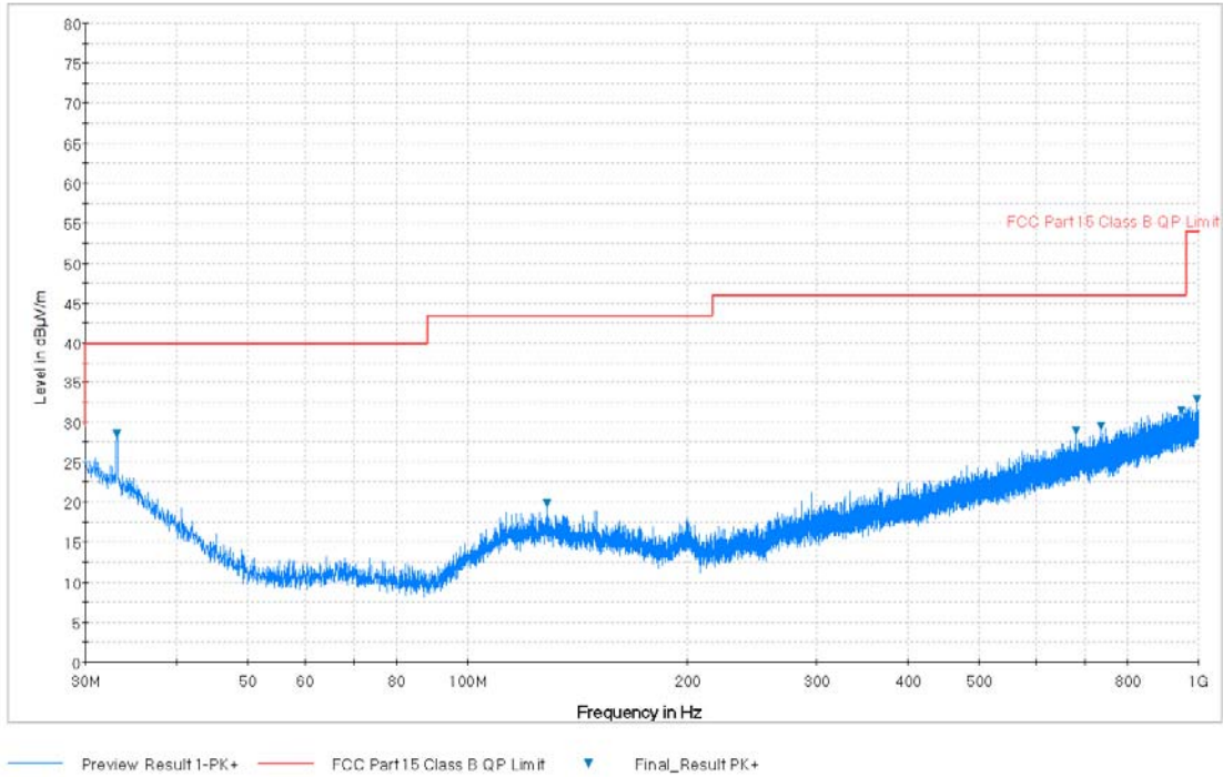
Plot 7-44. Radiated Spurious Plot below 1GHz (Pol. H)
