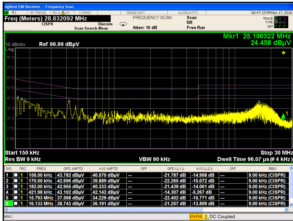
Plot 7-47. Line Conducted Plot with 802.11b (N)
