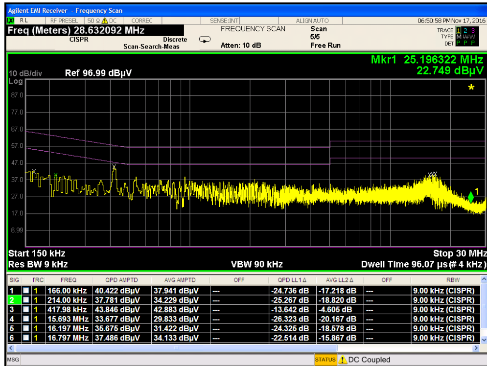
Plot 7-46. Line Conducted Plot with 802.11b (L1)
