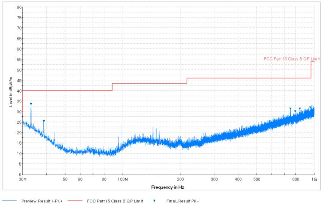
Plot 7-45. Radiated Spurious Plot below 1GHz (Pol. V)
