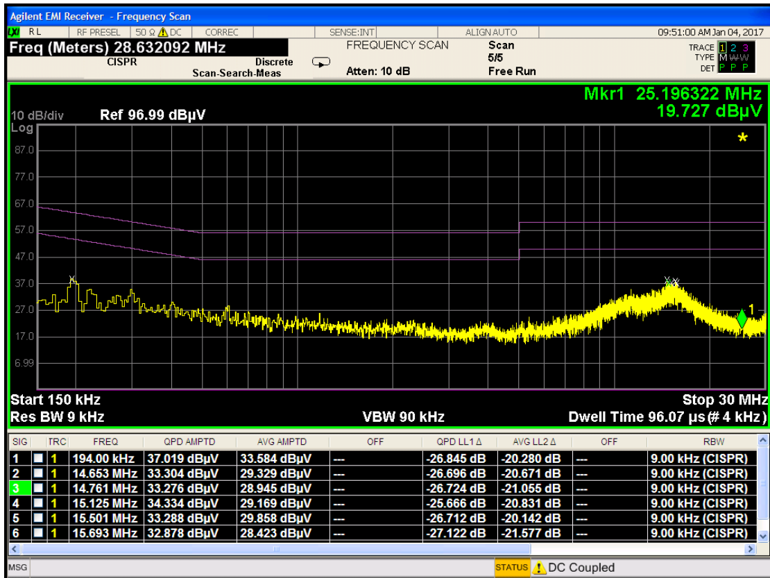
Plot 7-55. Line-Conducted Test Plot (N)
