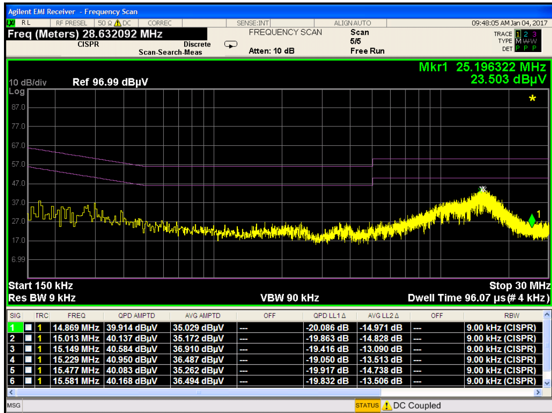
Plot 7-54. Line-Conducted Test Plot (L1)
