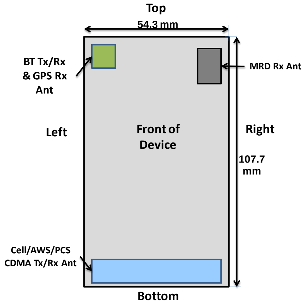
Figure 1-1 DUT Antenna Locations
