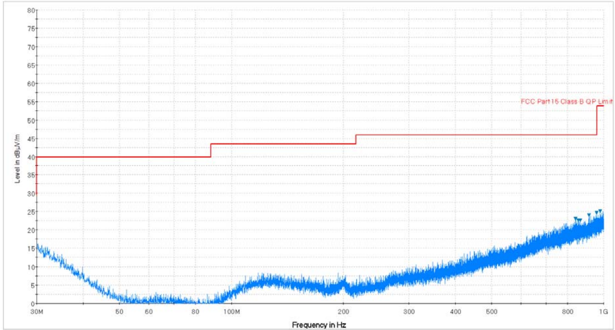
Plot 7-45. Radiated Spurious Plot below 1GHz (Pol. H)
