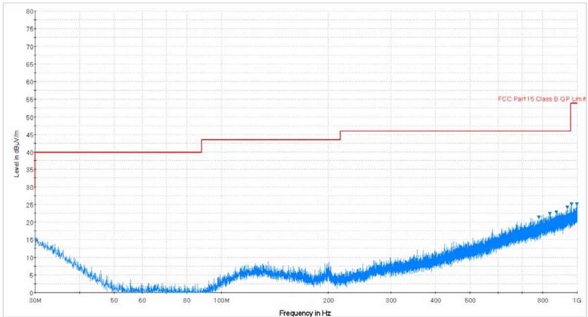
Plot 7-46. Radiated Spurious Plot below 1GHz (Pol. V)
