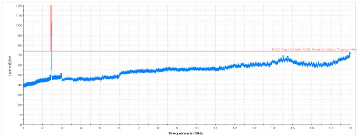
Plot 7-36. Radiated Spurious Plot above 1GHz (802.11b – Ch. 11, Ant. Pol. V)
