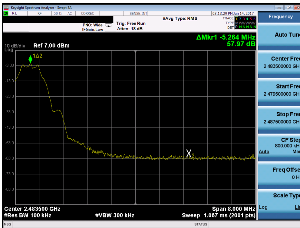
Plot 7-11. Band Edge Plot (Bluetooth (LE), 1Mbps – Ch. 39)
