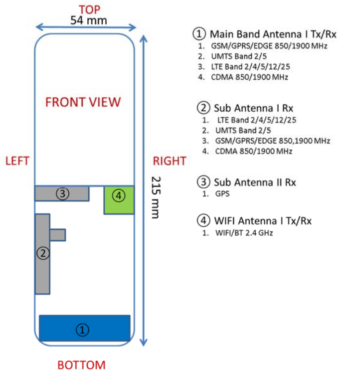
Figure F-2 DUT Antenna Location Open
