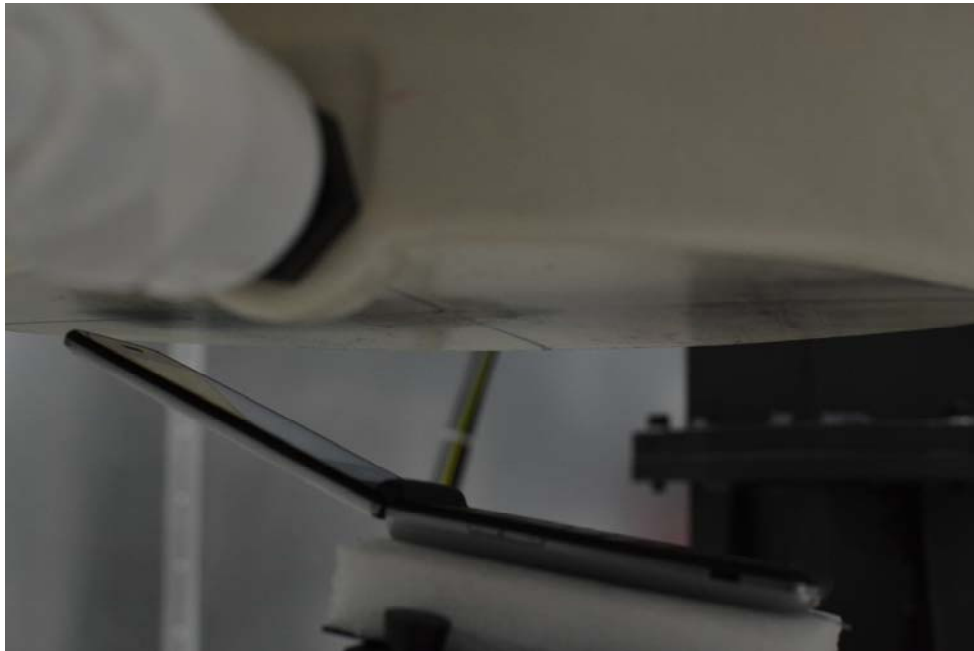
SAR Test Setup Photo 6 Mouth-Jaw Replacing Left Cheek UMTS 1900
