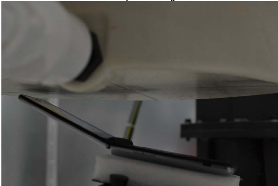
SAR Test Setup Photo 2 Mouth-Jaw Replacing Right Cheek
