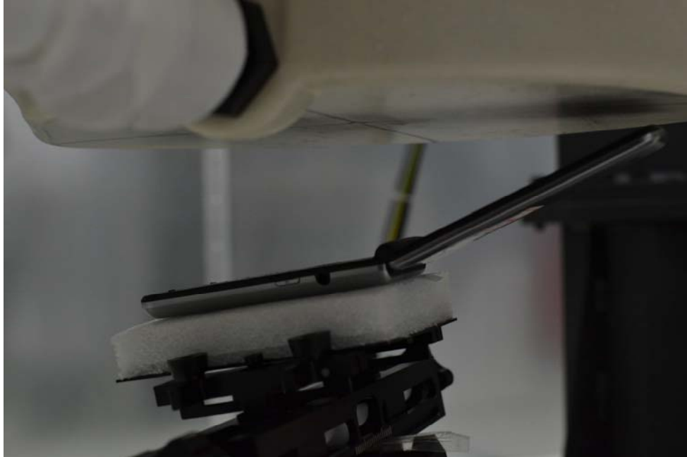
SAR Test Setup Photo 5 Mouth-Jaw Replacing Left Cheek
