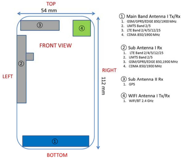
Figure F-1 DUT Antenna Location Closed
