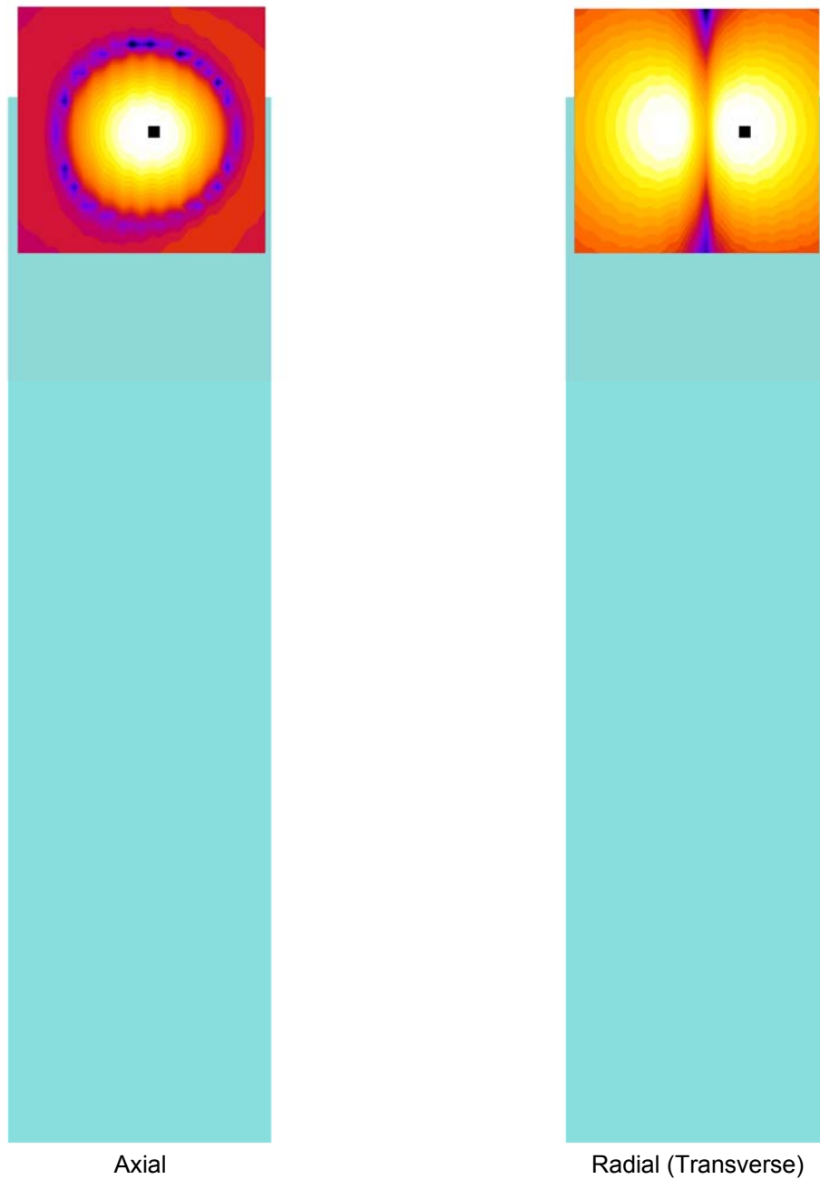
Figure 6-1 T-Coil Scan Overlay Magnetic Field Distributions
