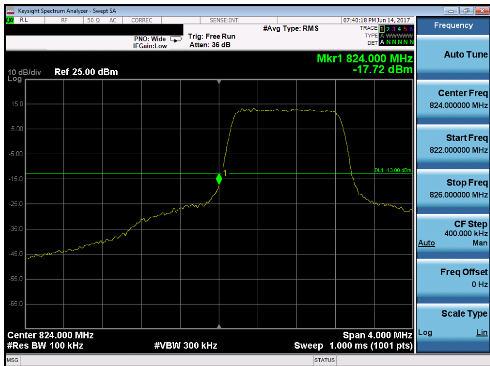
Plot 7-86. Lower Band Edge Plot (Band 5 - 1.4MHz QPSK - RB Size 6)
