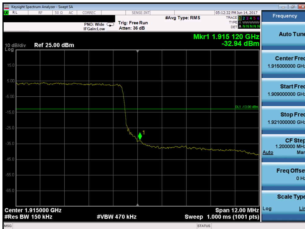
Plot 7-136. Upper Band Edge Plot (Band 25/2 – 15.0MHz QPSK – RB Size 75)
