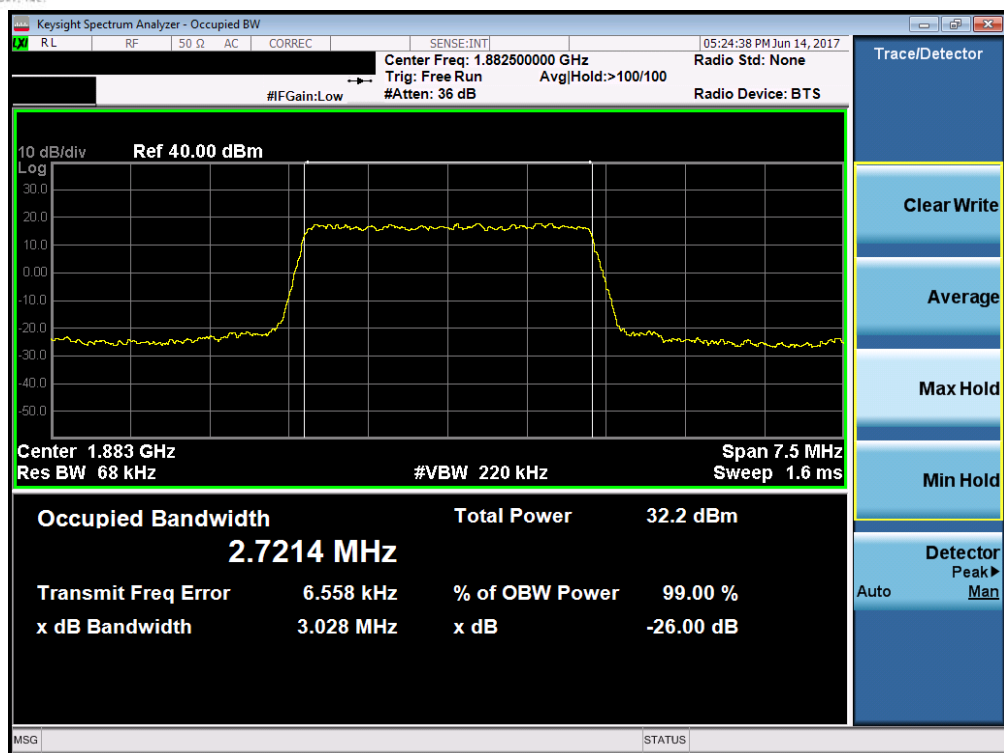
Plot 7-31. Occupied Bandwidth Plot (Band 25/2 – 3.0MHz QPSK – RB Size 15)
