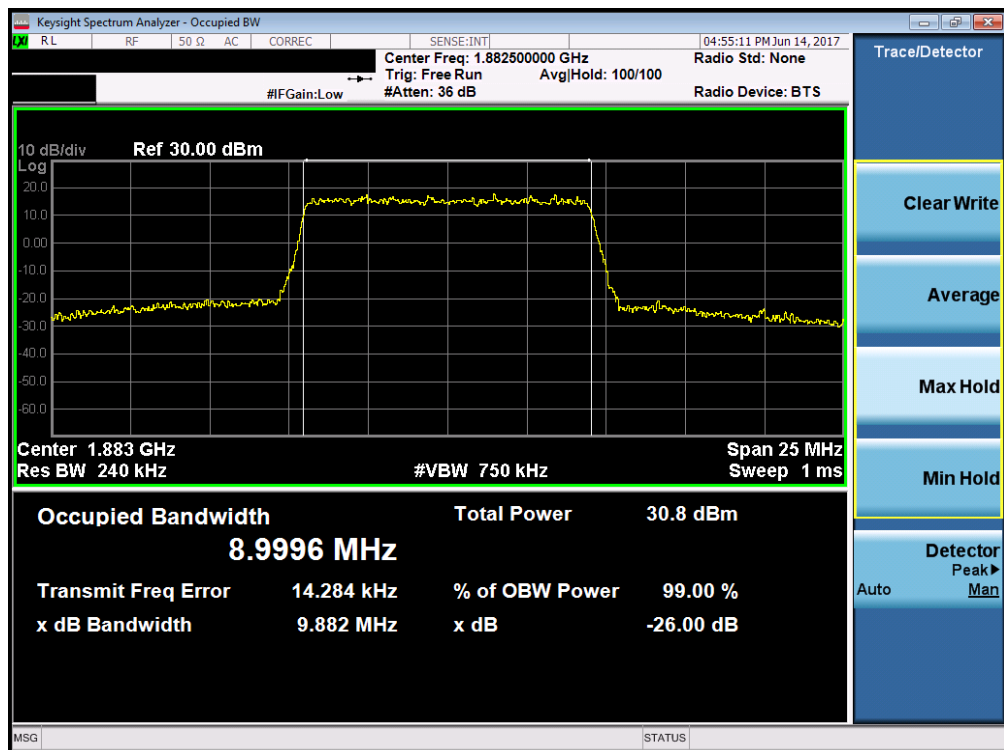
Plot 7-36. Occupied Bandwidth Plot (Band 25/2 – 10.0MHz 16-QAM – RB Size 50)
