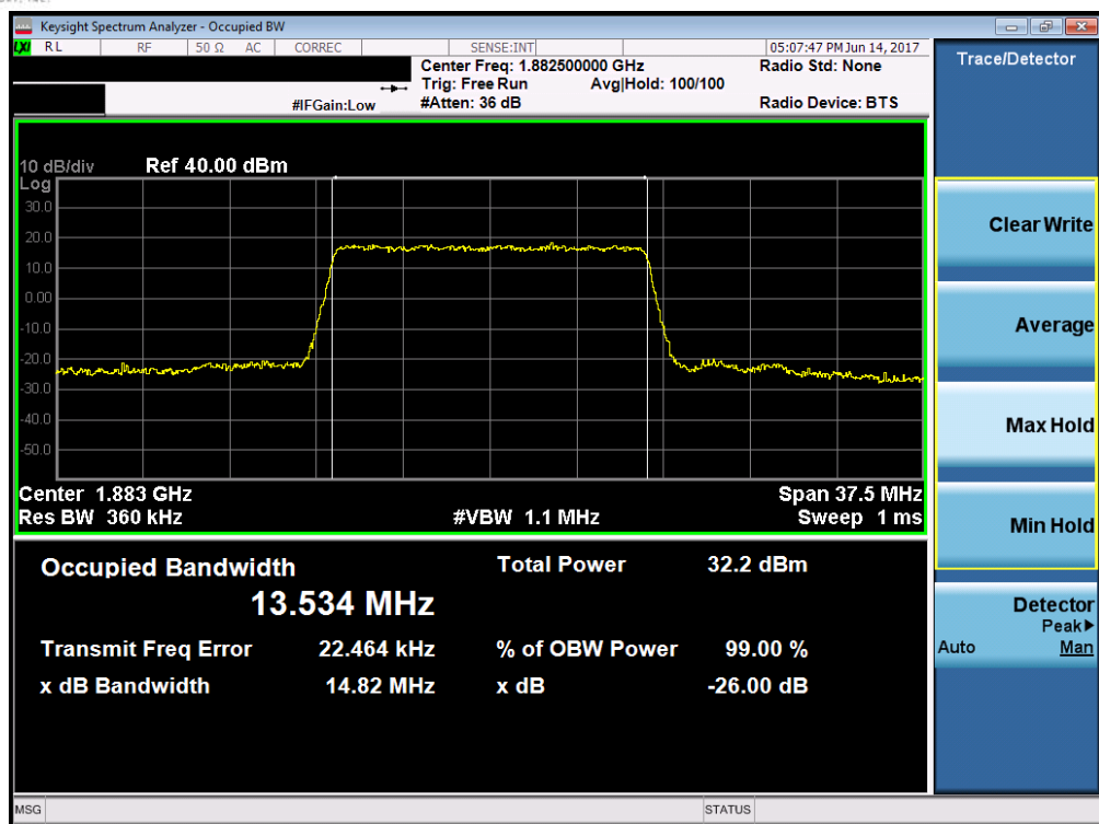
Plot 7-37. Occupied Bandwidth Plot (Band 25/2 – 15.0MHz QPSK – RB Size 75)
