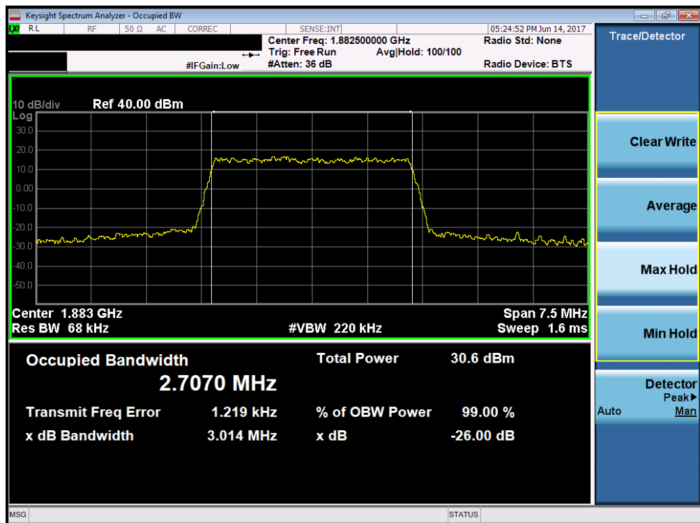
Plot 7-32. Occupied Bandwidth Plot (Band 25/2 – 3.0MHz 16-QAM – RB Size 15)
