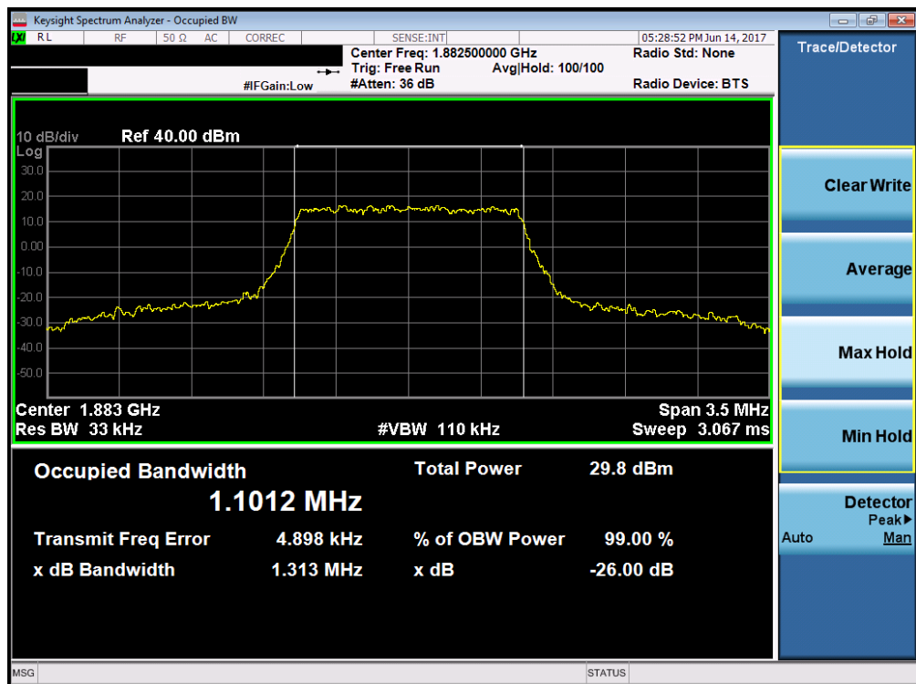
Plot 7-30. Occupied Bandwidth Plot (Band 25/2 – 1.4MHz 16-QAM – RB Size 6)
