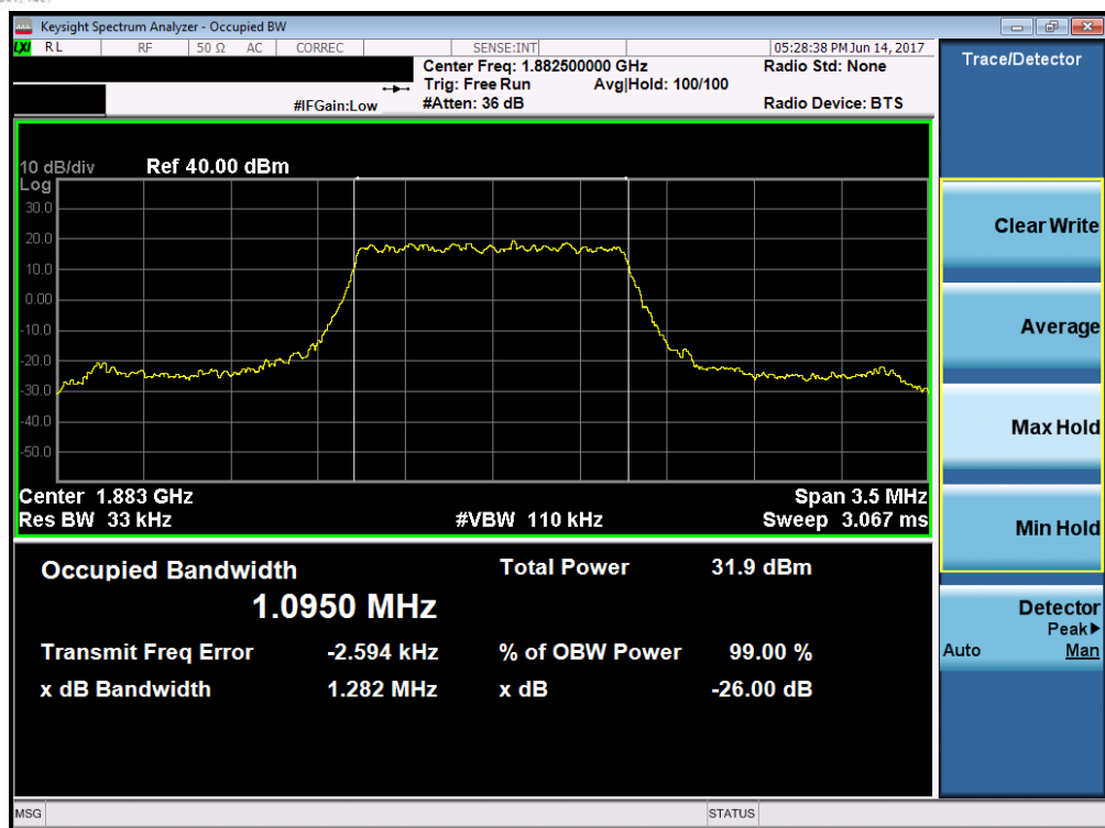
Plot 7-29. Occupied Bandwidth Plot (Band 25/2 – 1.4MHz QPSK – RB Size 6)
