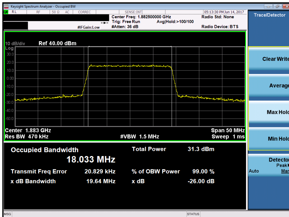
Plot 7-40. Occupied Bandwidth Plot (Band 25/2 – 20.0MHz 16-QAM – RB Size 100)
