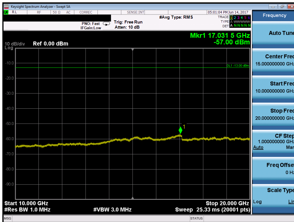
Plot 7-70. Conducted Spurious Plot (Band 25/2 – 10.0MHz QPSK – RB Size 1, RB Offset 0 – Low Channel)
