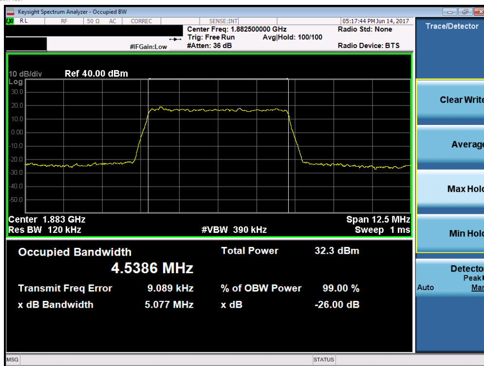
Plot 7-33. Occupied Bandwidth Plot (Band 25/2 – 5.0MHz QPSK – RB Size 25)
