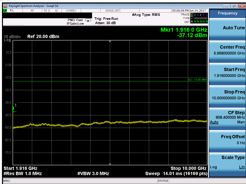
Plot 7-75. Conducted Spurious Plot (Band 25/2 – 10.0MHz QPSK – RB Size 1, RB Offset 0 – High Channel)
