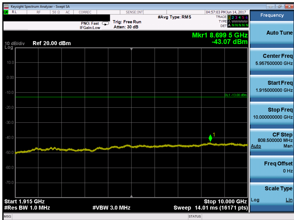
Plot 7-72. Conducted Spurious Plot (Band 25/2 – 10.0MHz QPSK – RB Size 1, RB Offset 0 – Mid Channel)
