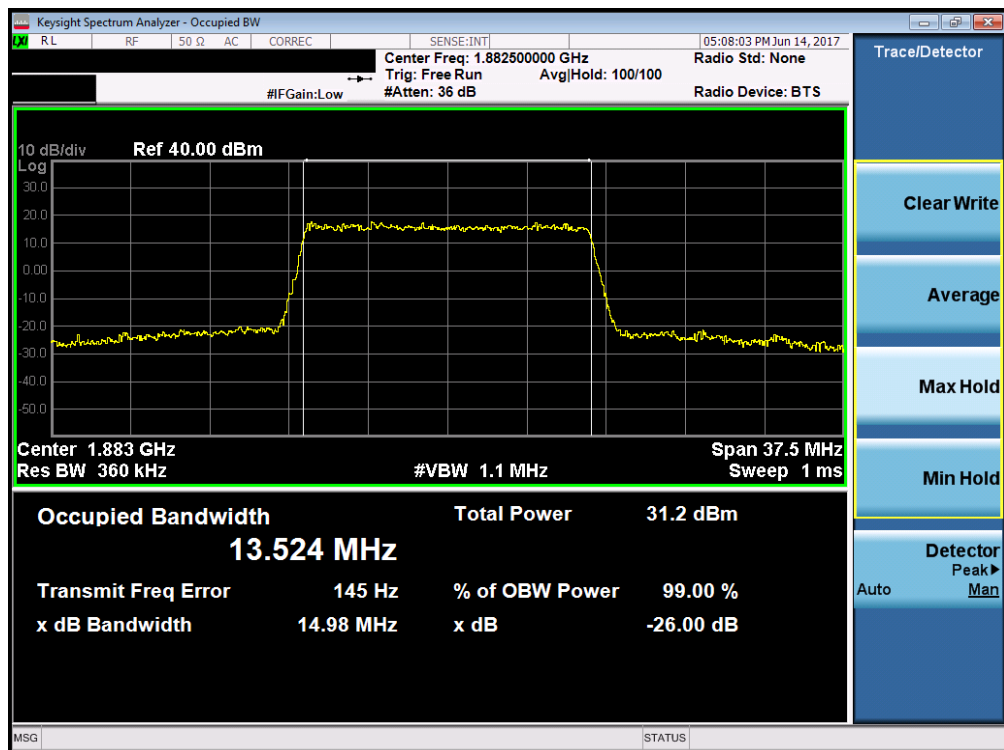
Plot 7-38. Occupied Bandwidth Plot (Band 25/2 – 15.0MHz 16-QAM – RB Size 75)
