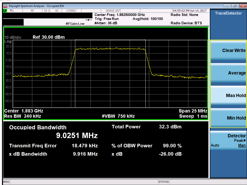
Plot 7-35. Occupied Bandwidth Plot (Band 25/2 – 10.0MHz QPSK – RB Size 50)
