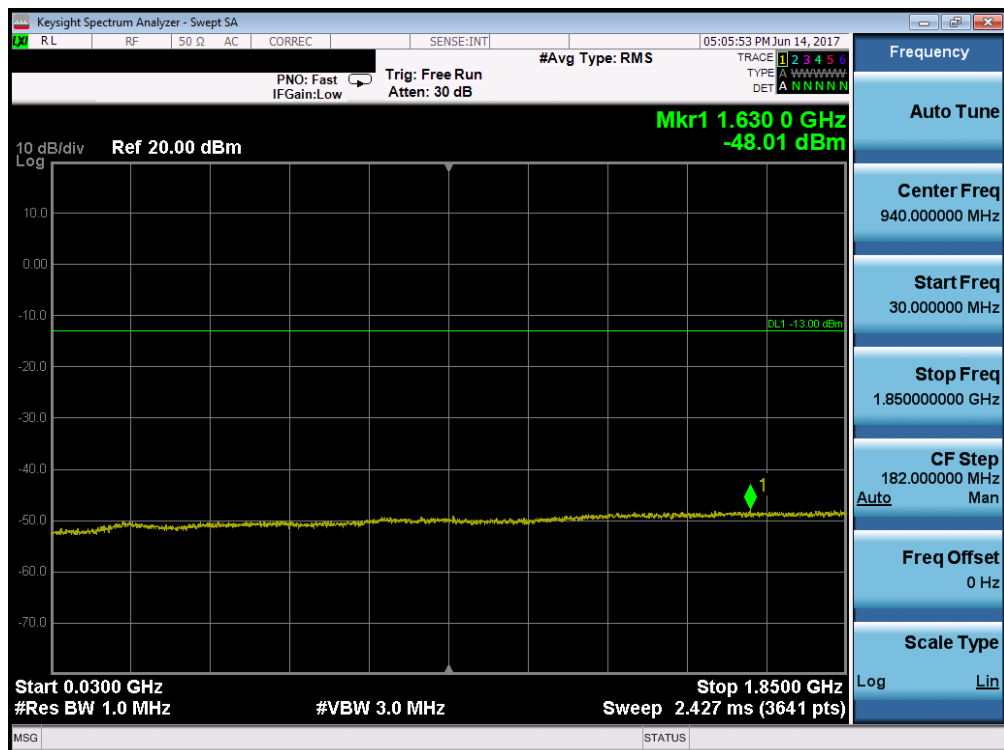
Plot 7-74. Conducted Spurious Plot (Band 25/2 – 10.0MHz QPSK – RB Size 1, RB Offset 0 – High Channel)
