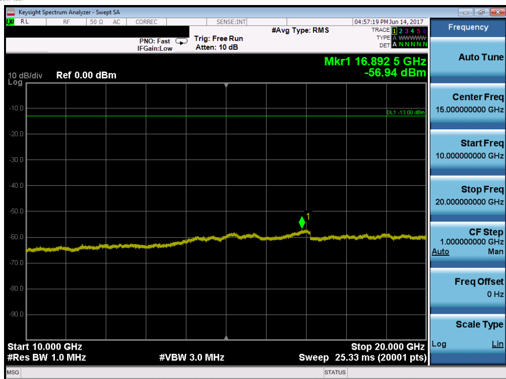
Plot 7-73. Conducted Spurious Plot (Band 25/2 – 10.0MHz QPSK – RB Size 1, RB Offset 0 – Mid Channel)
