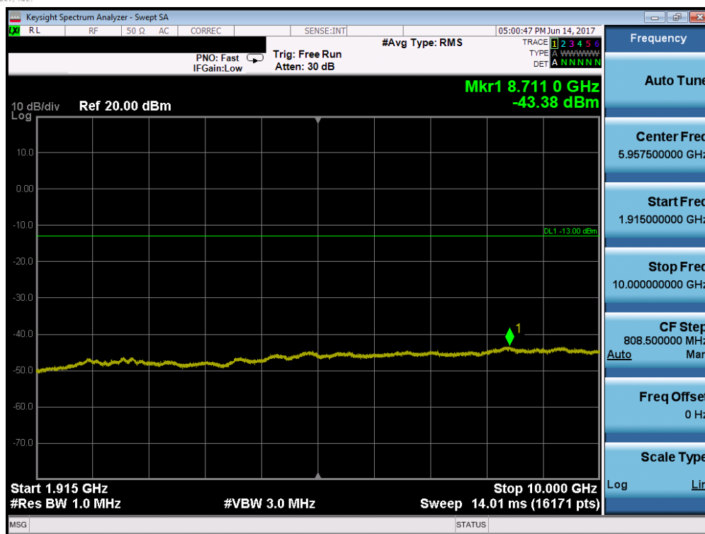
Plot 7-69. Conducted Spurious Plot (Band 25/2 – 10.0MHz QPSK – RB Size 1, RB Offset 0 – Low Channel)
