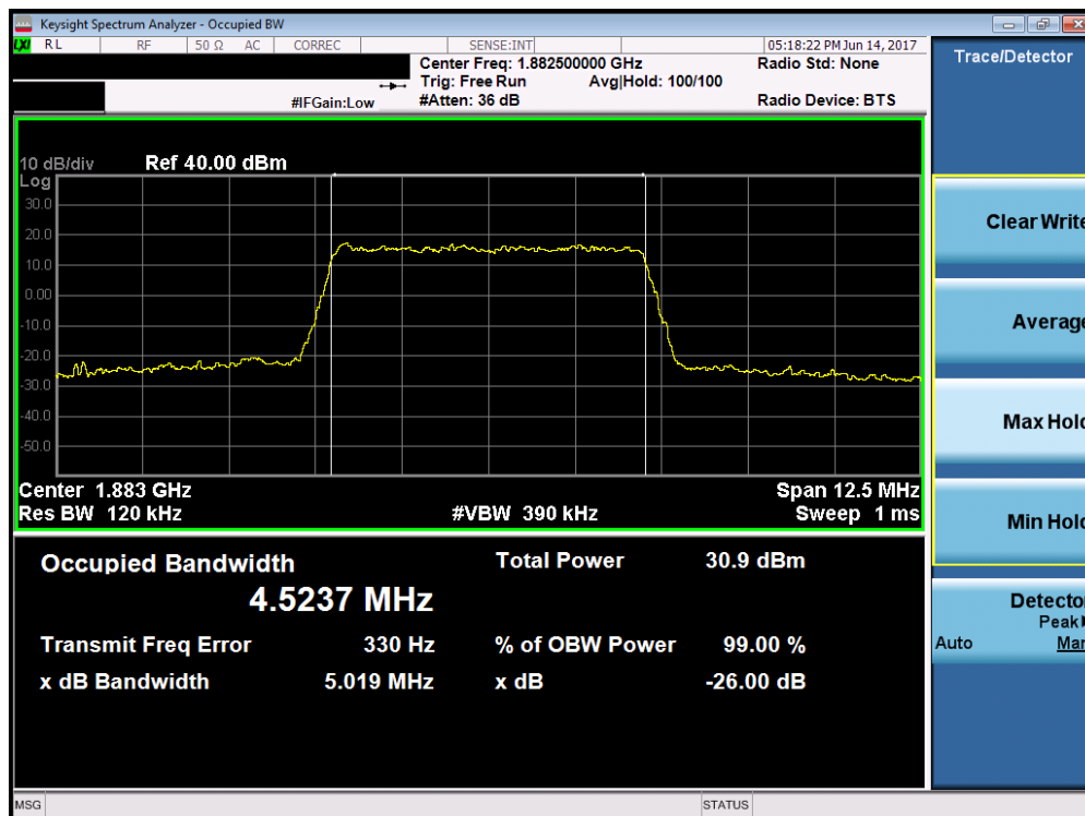
Plot 7-34. Occupied Bandwidth Plot (Band 25/2 – 5.0MHz 16-QAM – RB Size 25)
