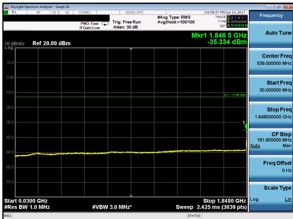
Plot 7-68. Conducted Spurious Plot (Band 25/2 – 10.0MHz QPSK – RB Size 1, RB Offset 0– Low Channel)
