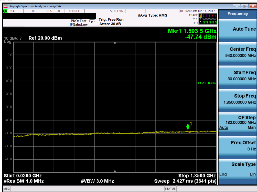
Plot 7-71. Conducted Spurious Plot (Band 25/2 – 10.0MHz QPSK – RB Size 1, RB Offset 0 – Mid Channel)
