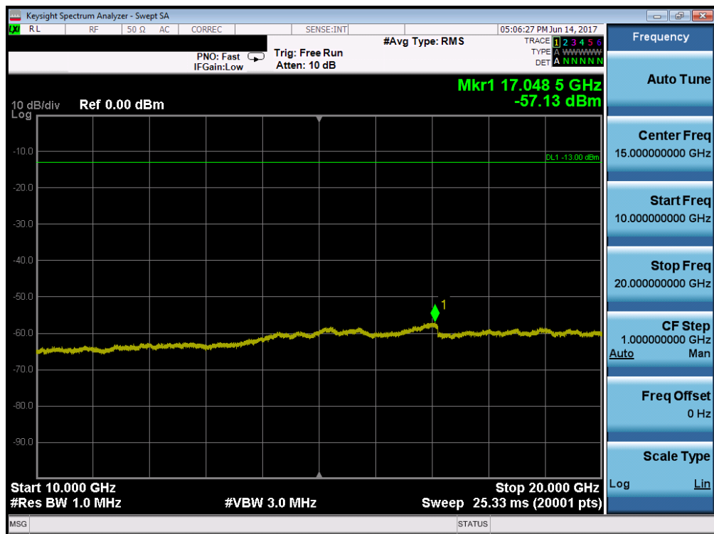
Plot 7-76. Conducted Spurious Plot (Band 25/2 – 10.0MHz QPSK – RB Size 1, RB Offset 0 – High Channel)
