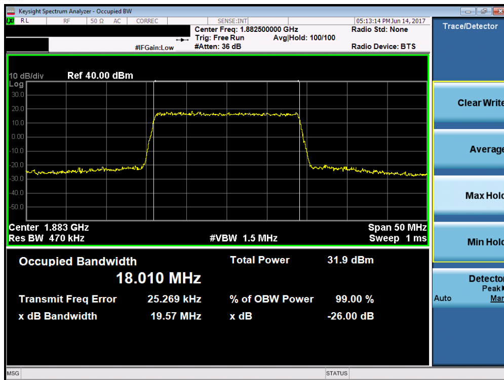
Plot 7-39. Occupied Bandwidth Plot (Band 25/2 – 20.0MHz QPSK – RB Size 100)
