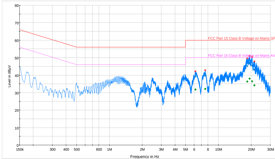
Plot 6-98. Line Conducted Plot with 802.11a UNII Band 3 (N)
