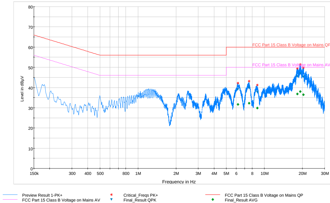
Plot 6-96. Line Conducted Plot with 802.11a UNII Band 2C (N)
