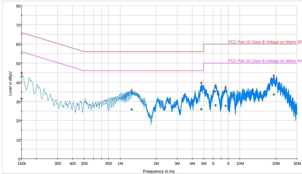
Plot 6-93. Line Conducted Plot with 802.11a UNII Band 2A (L1)
