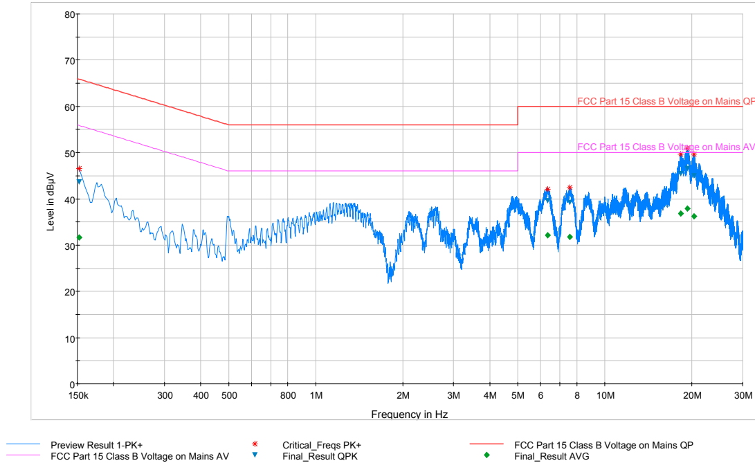
Plot 6-44. Line Conducted Plot with 802.11b (N)
