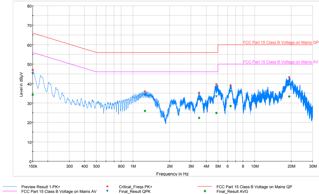
Plot 6-43. Line Conducted Plot with 802.11b (L1)
