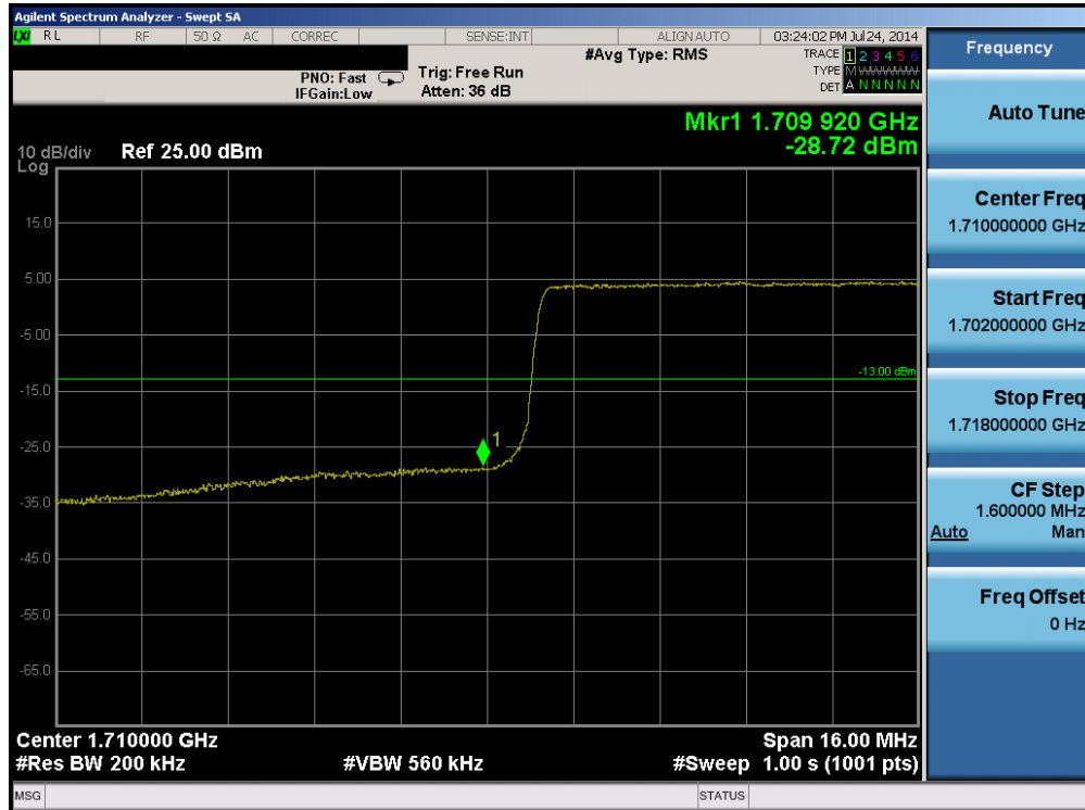
Plot 6-75. Lower Band Edge Plot (Band 4 – 20.0MHz QPSK – RB Size 100)
