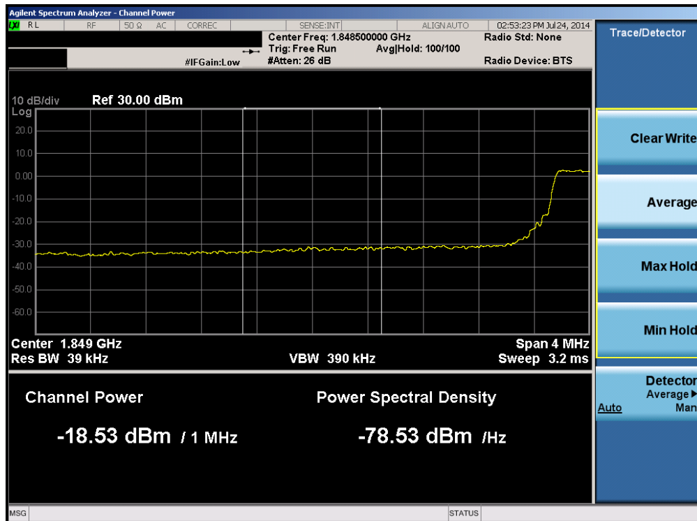
Plot 6-80. Lower Extended Band Edge Plot (Band 2 – 5.0MHz QPSK – RB Size 25)
