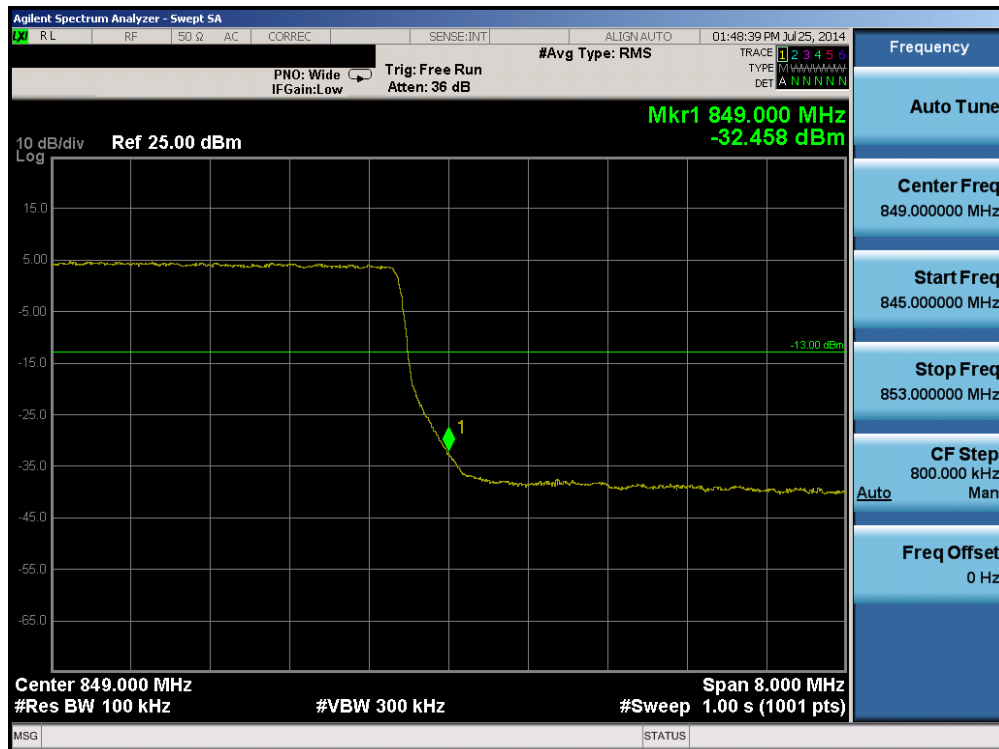
Plot 6-62. Upper Band Edge Plot (Band 5 – 10.0MHz QPSK – RB Size 50)
