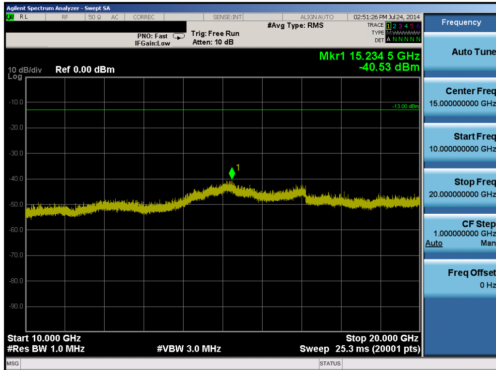
Plot 6-42. Conducted Spurious Plot (Band 2 – 5.0MHz QPSK – RB Size 1, RB Offset 0 – Mid Channel)
