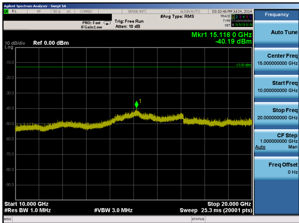
Plot 6-36. Conducted Spurious Plot (Band 4 – 5.0MHz QPSK – RB Size 1, RB Offset 0 – Mid Channel)
