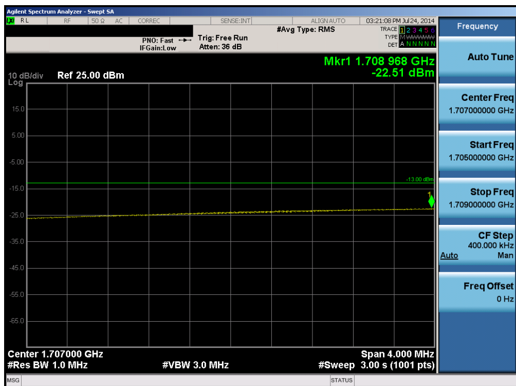
Plot 6-72. Lower Extended Band Edge Plot (Band 4 – 15.0MHz QPSK – RB Size 75)
