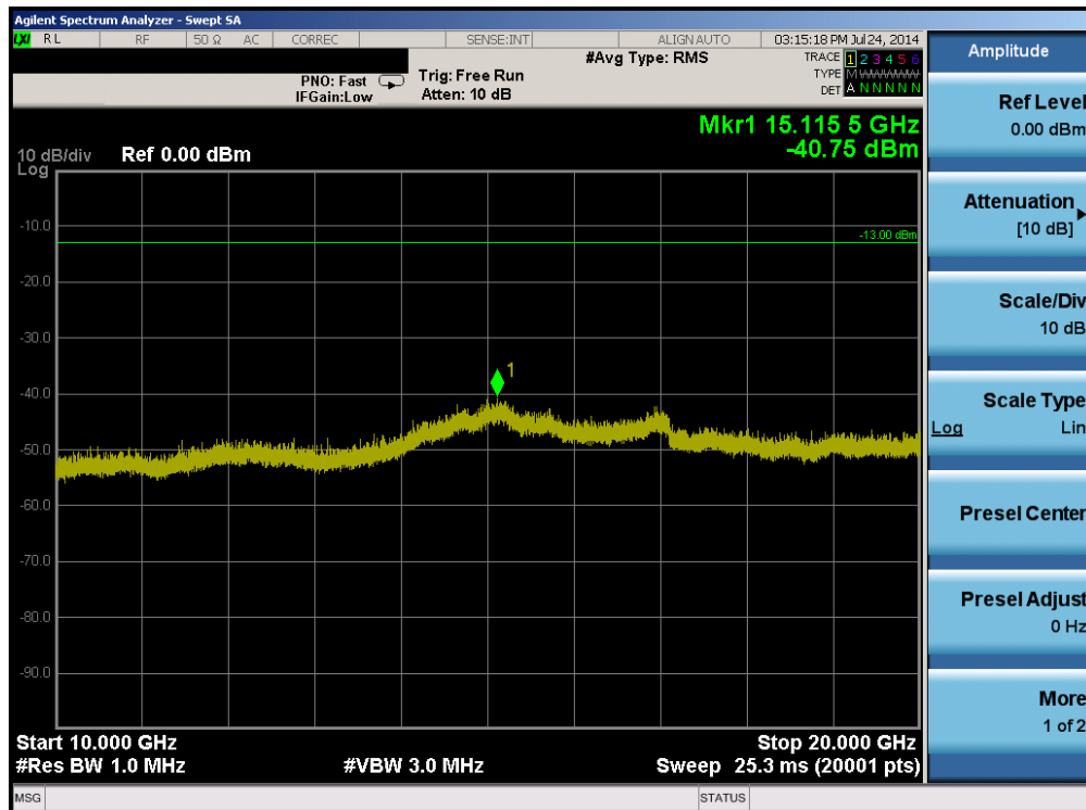
Plot 6-38. Conducted Spurious Plot (Band 4 – 5.0MHz QPSK – RB Size 1, RB Offset 0 – High Channel)
