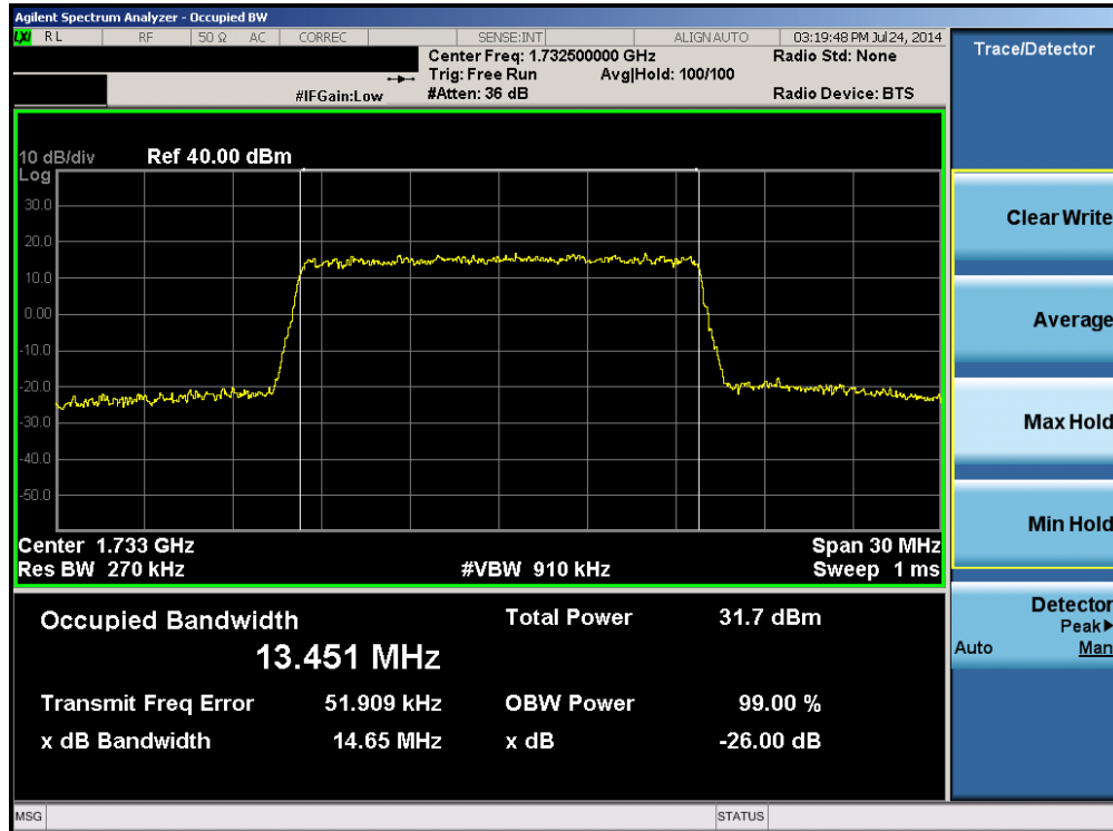
Plot 6-15. Occupied Bandwidth Plot (Band 4 – 15.0MHz QPSK – RB Size 75)
