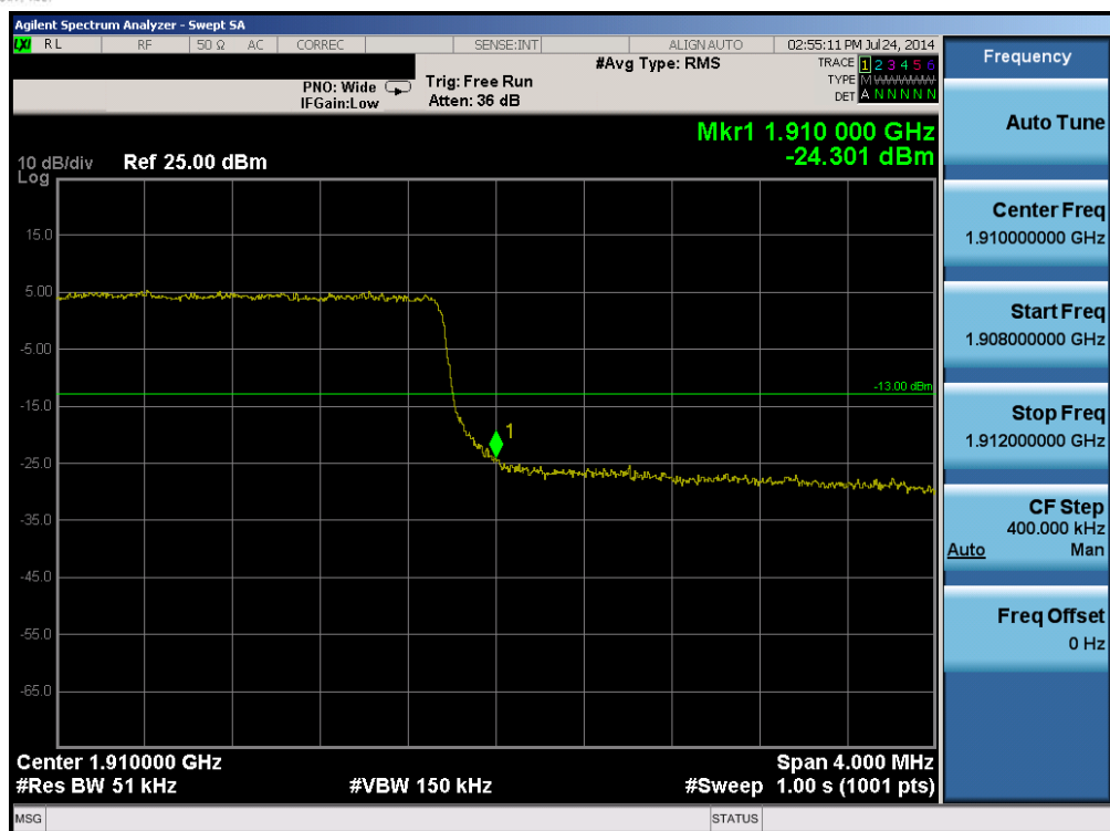
Plot 6-81. Upper Band Edge Plot (Band 2 – 5.0MHz QPSK – RB Size 25)
