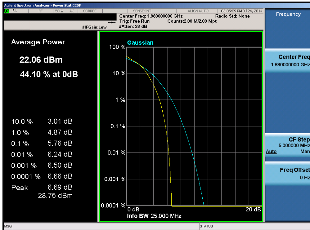
Plot 6-102. PAR Plot (Band 2 – 20.0MHz 16-QAM – RB Size 100)
