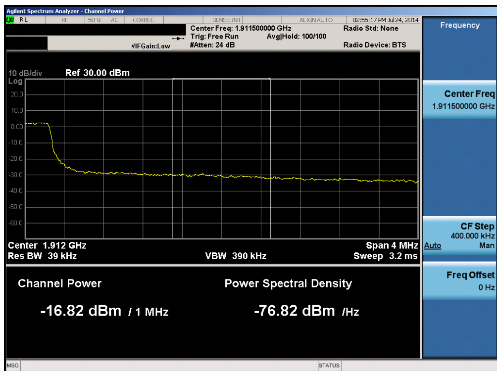
Plot 6-82. Upper Extended Band Edge Plot (Band 2 – 5.0MHz QPSK – RB Size 25)
