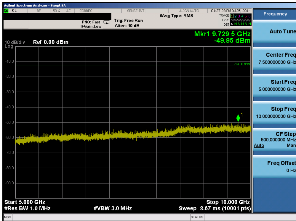
Plot 6-28. Conducted Spurious Plot (Band 5 – 5.0MHz QPSK – RB Size 1, RB Offset 0 – Low Channel)
