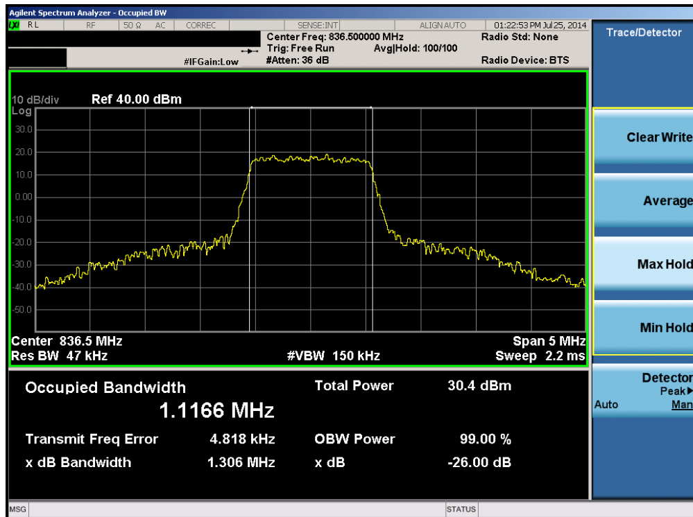
Plot 6-4. Occupied Bandwidth Plot (Band 5 – 1.4MHz 16-QAM – RB Size 6)
