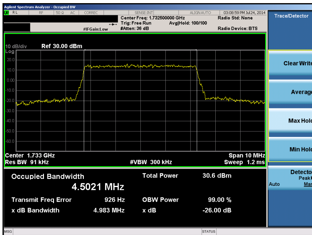
Plot 6-12. Occupied Bandwidth Plot (Band 4 – 5.0MHz 16-QAM – RB Size 25)
