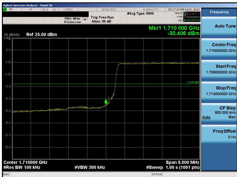
Plot 6-67. Lower Band Edge Plot (Band 4 – 10.0MHz QPSK – RB Size 50)
