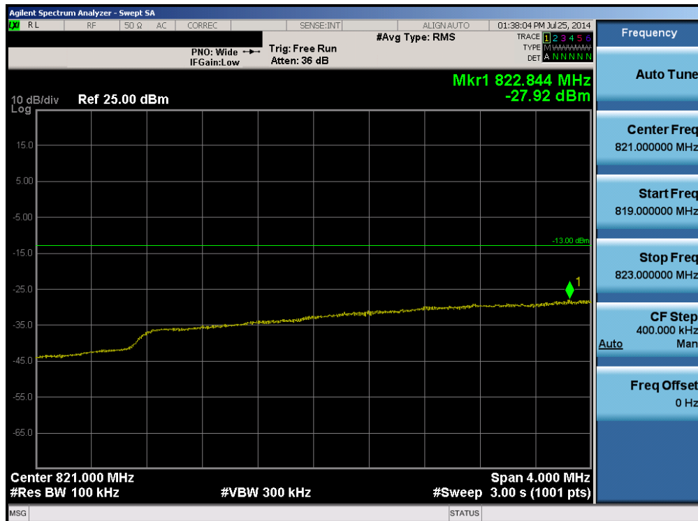
Plot 6-58. Lower Extended Band Edge Plot (Band 5 - 5.0MHz QPSK - RB Size 25)
