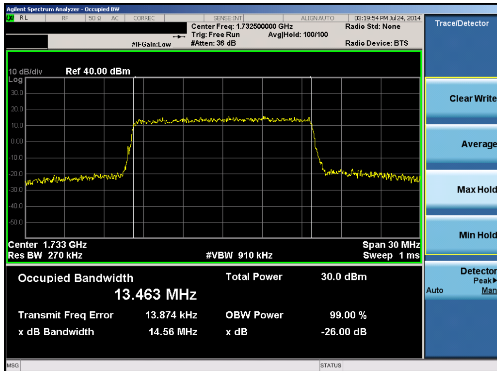
Plot 6-16. Occupied Bandwidth Plot (Band 4 – 15.0MHz 16-QAM – RB Size 75)
