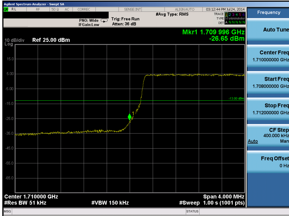
Plot 6-63. Lower Band Edge Plot (Band 4 – 5.0MHz QPSK – RB Size 25)
