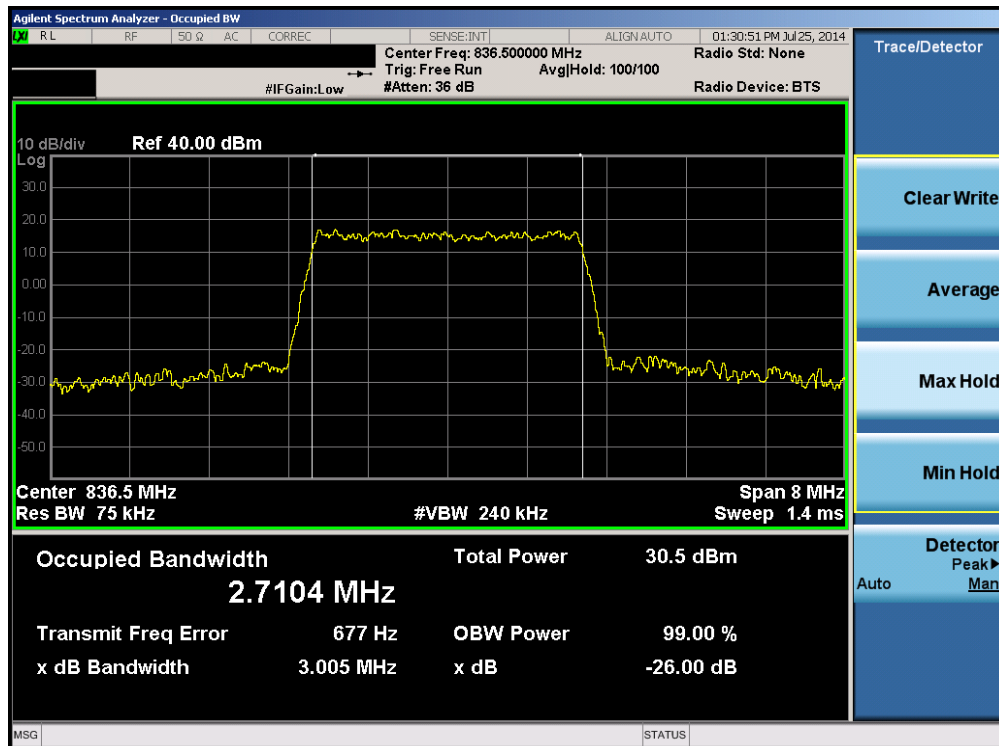
Plot 6-6. Occupied Bandwidth Plot (Band 5 – 3.0MHz 16-QAM – RB Size 15)
