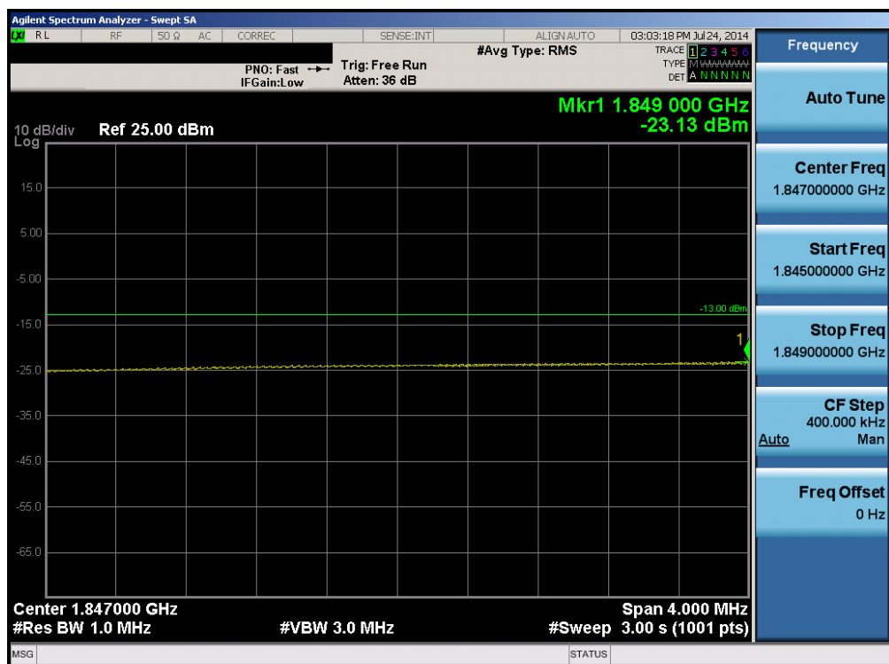
Plot 6-88. Lower Extended Band Edge Plot (Band 2 – 15.0MHz QPSK – RB Size 75)
