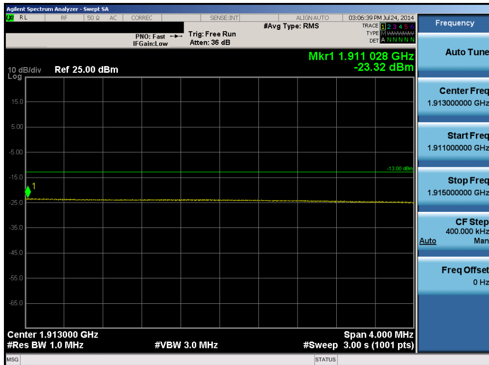
Plot 6-94. Upper Extended Band Edge Plot (Band 2 – 20.0MHz QPSK – RB Size 100)
