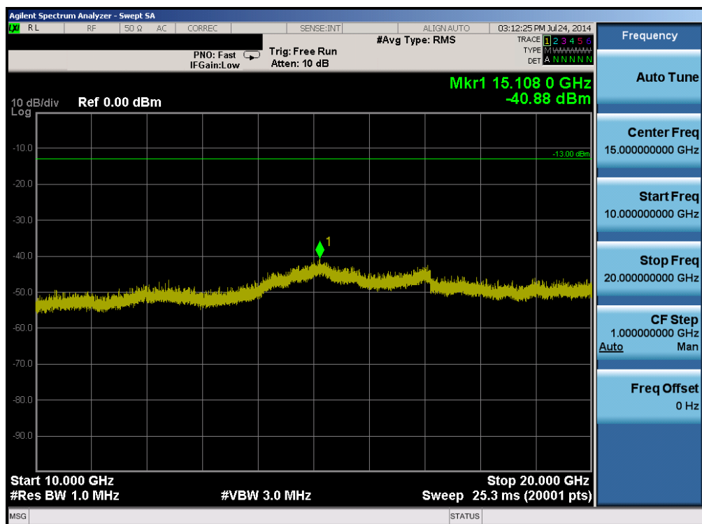
Plot 6-34. Conducted Spurious Plot (Band 4 – 5.0MHz QPSK – RB Size 1, RB Offset 0 – Low Channel)
