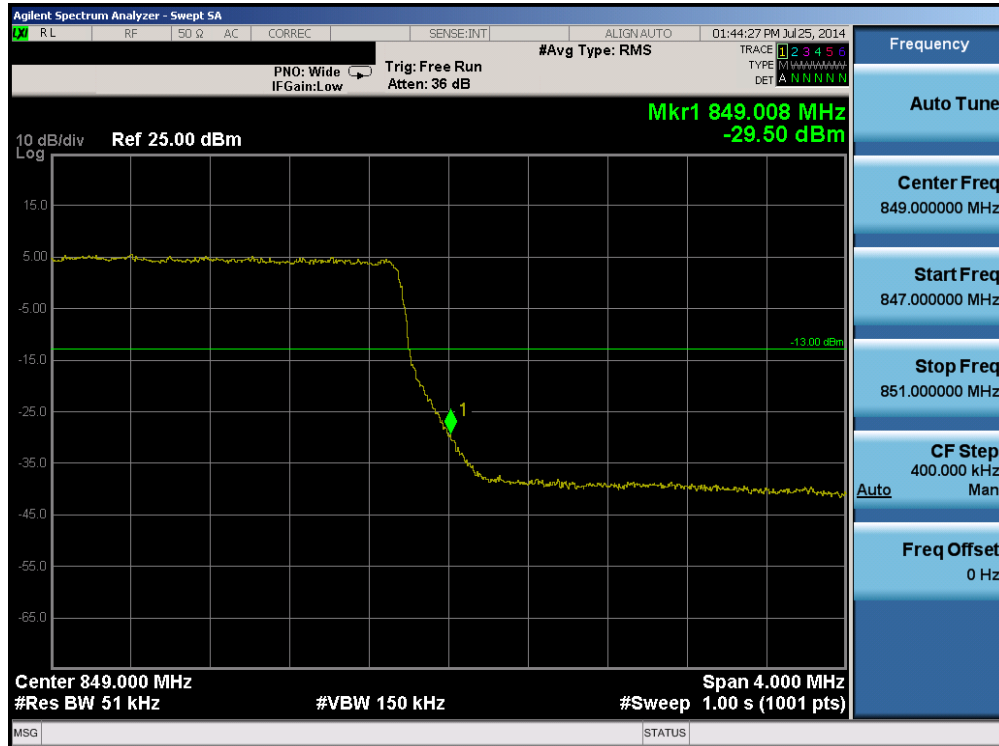
Plot 6-59. Upper Band Edge Plot (Band 5 – 5.0MHz QPSK – RB Size 25)
