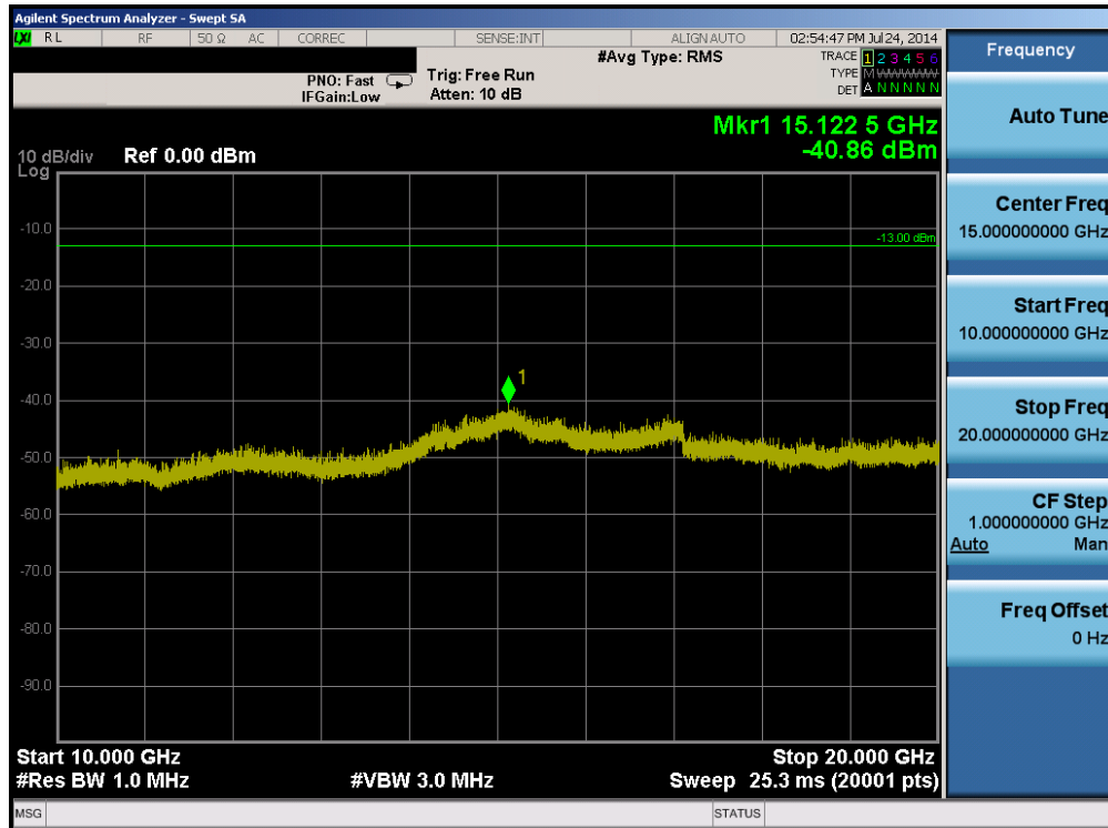
Plot 6-44. Conducted Spurious Plot (Band 2 – 5.0MHz QPSK – RB Size 1, RB Offset 0 – High Channel)
