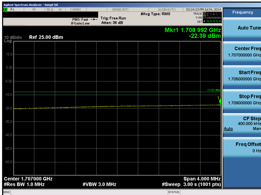
Plot 6-76. Lower Extended Band Edge Plot (Band 4 – 20.0MHz QPSK – RB Size 100)
