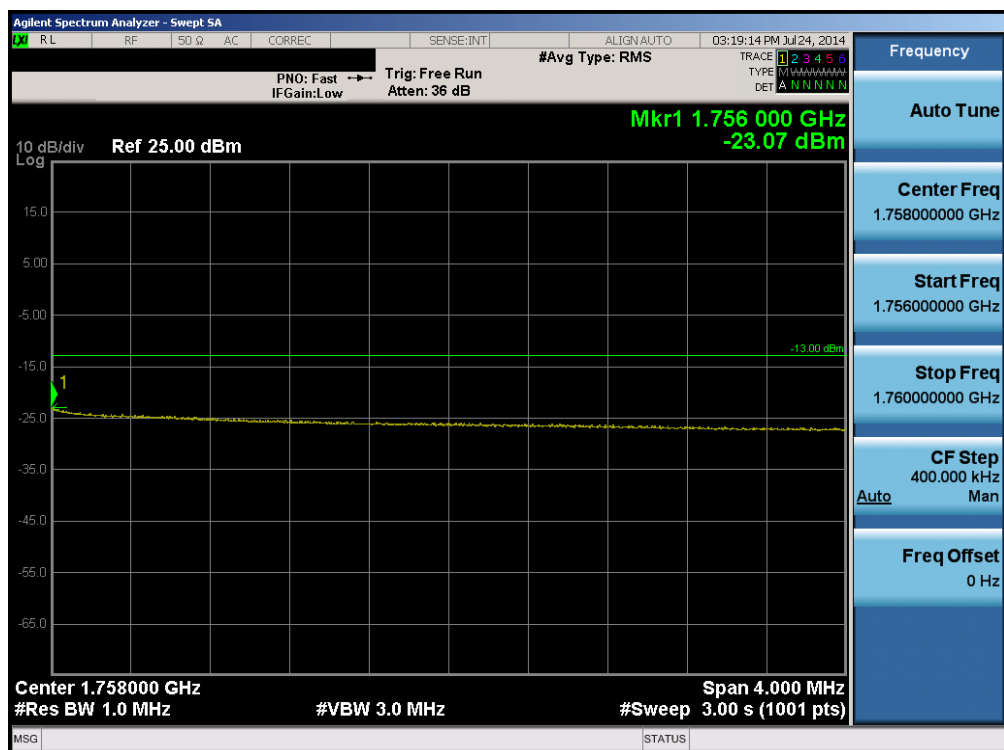
Plot 6-70. Upper Extended Band Edge Plot (Band 4 – 10.0MHz QPSK – RB Size 50)
