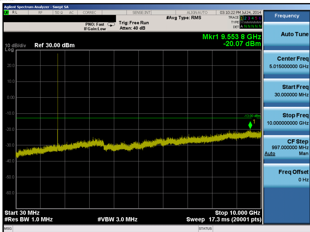
Plot 6-35. Conducted Spurious Plot (Band 4 – 5.0MHz QPSK – RB Size 1, RB Offset 0 – Mid Channel)
