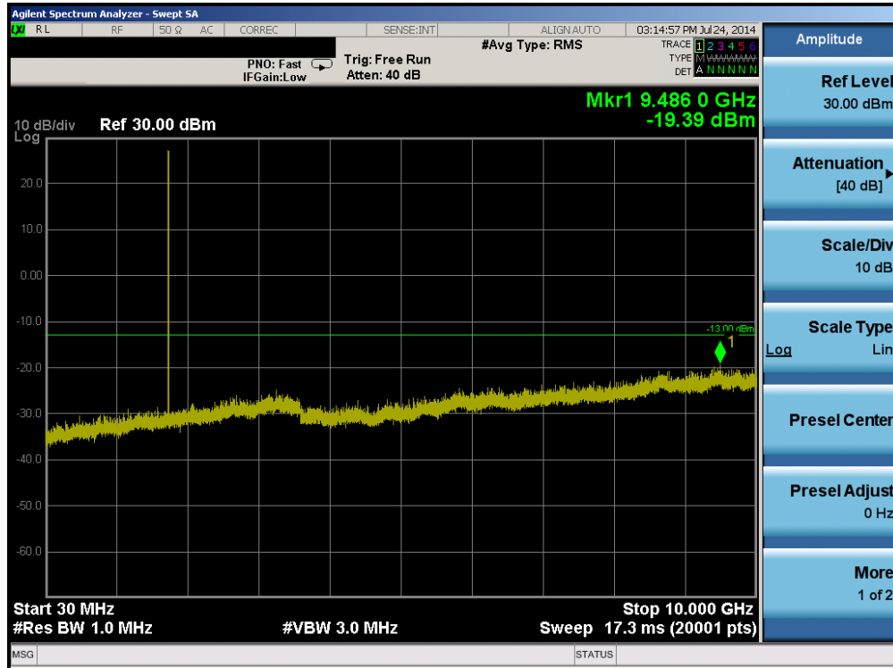
Plot 6-37. Conducted Spurious Plot (Band 4 – 5.0MHz QPSK – RB Size 1, RB Offset 0 – High Channel)
