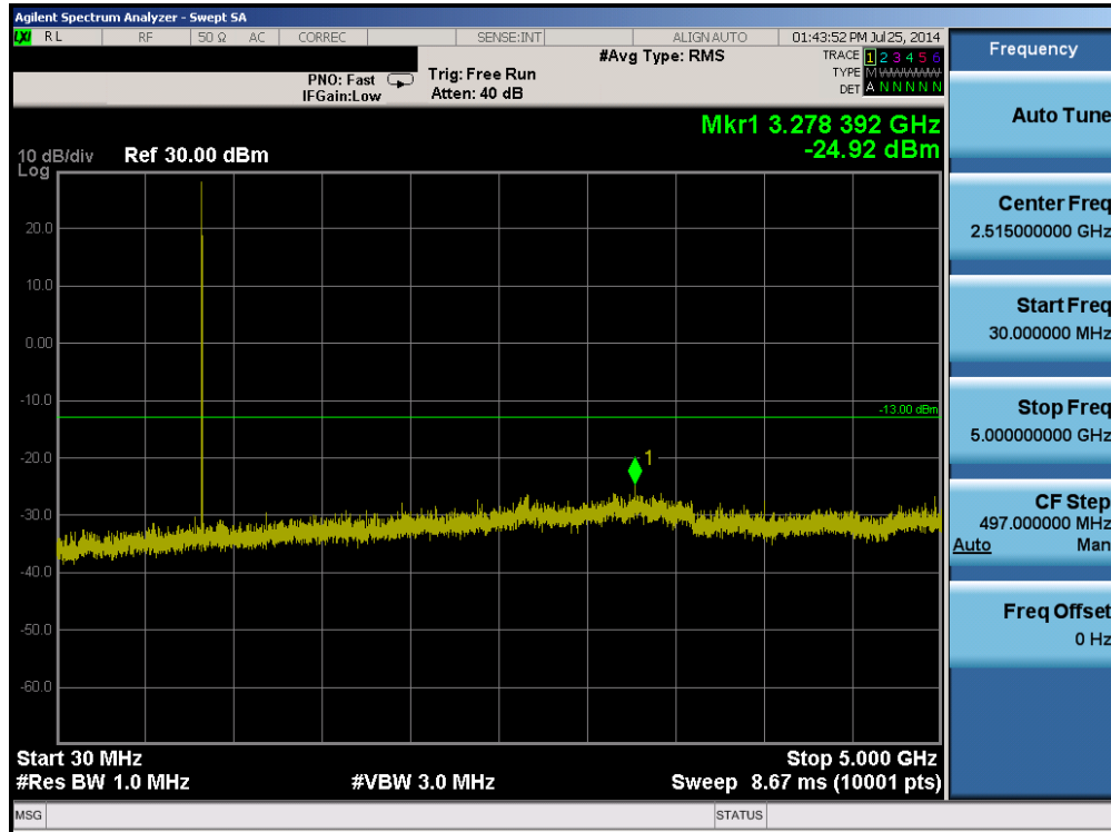
Plot 6-31. Conducted Spurious Plot (Band 5 – 5.0MHz QPSK – RB Size 1, RB Offset 0 – High Channel)
