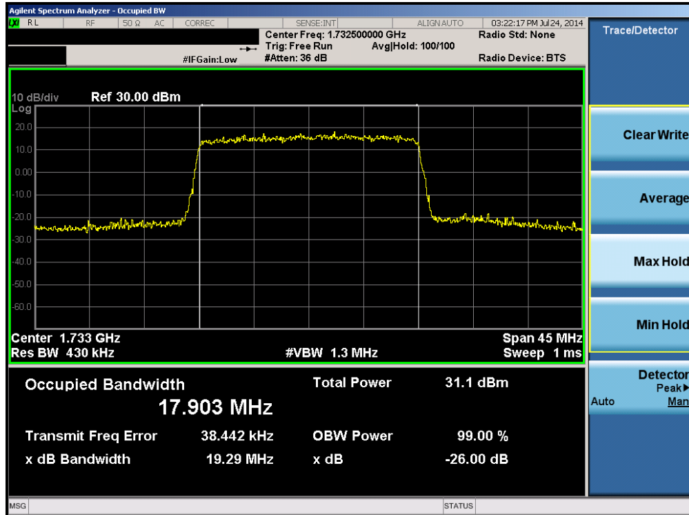
Plot 6-17. Occupied Bandwidth Plot (Band 4 – 20.0MHz QPSK – RB Size 100)
