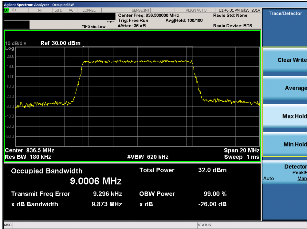
Plot 6-9. Occupied Bandwidth Plot (Band 5 – 10.0MHz QPSK – RB Size 50)
