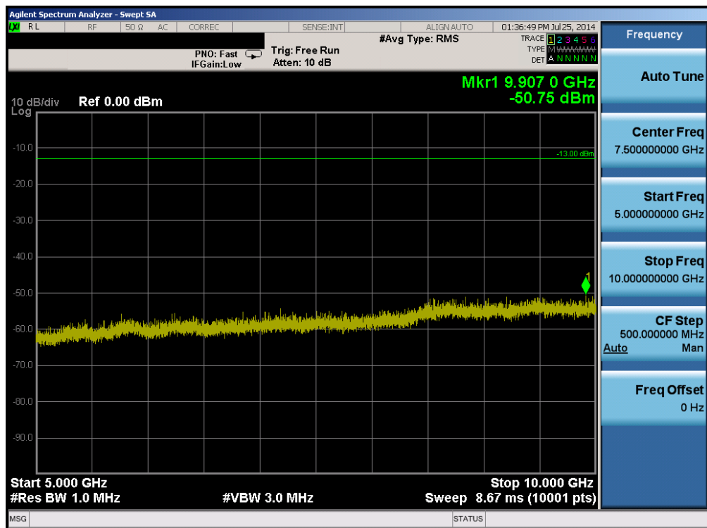
Plot 6-30. Conducted Spurious Plot (Band 5 – 5.0MHz QPSK – RB Size 1, RB Offset 0 – Mid Channel)
