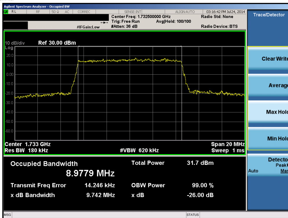
Plot 6-13. Occupied Bandwidth Plot (Band 4 – 10.0MHz QPSK – RB Size 50)
