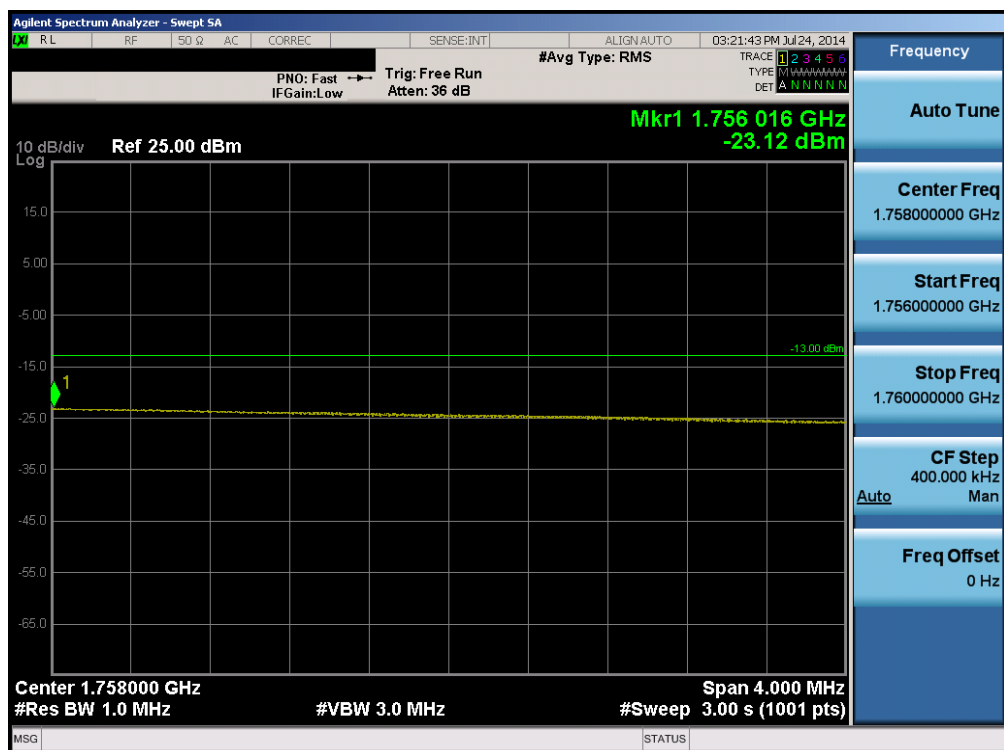
Plot 6-74. Upper Extended Band Edge Plot (Band 4 – 15.0MHz QPSK – RB Size 75)
