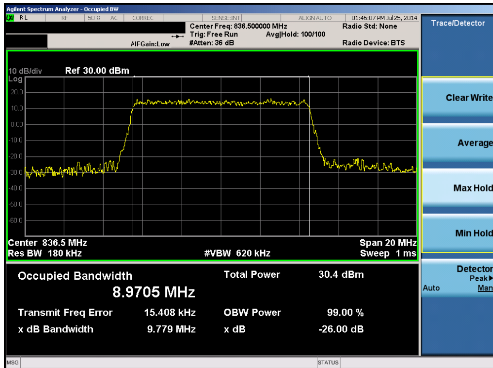
Plot 6-10. Occupied Bandwidth Plot (Band 5 – 10.0MHz 16-QAM – RB Size 50)
