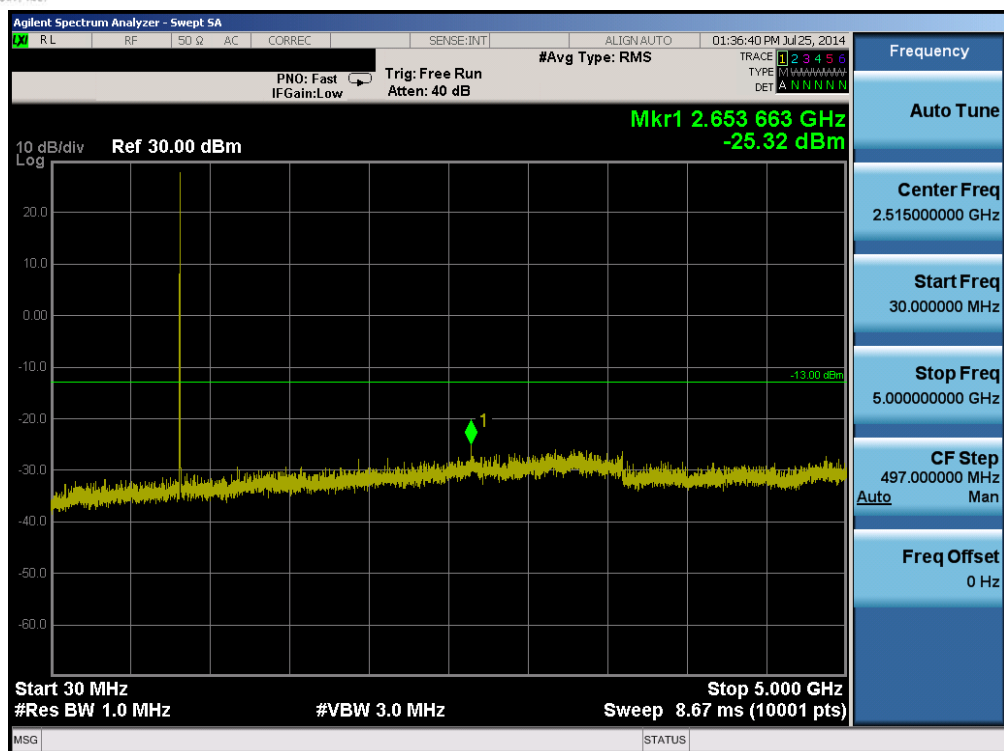
Plot 6-29. Conducted Spurious Plot (Band 5 – 5.0MHz QPSK – RB Size 1, RB Offset 0 – Mid Channel)
