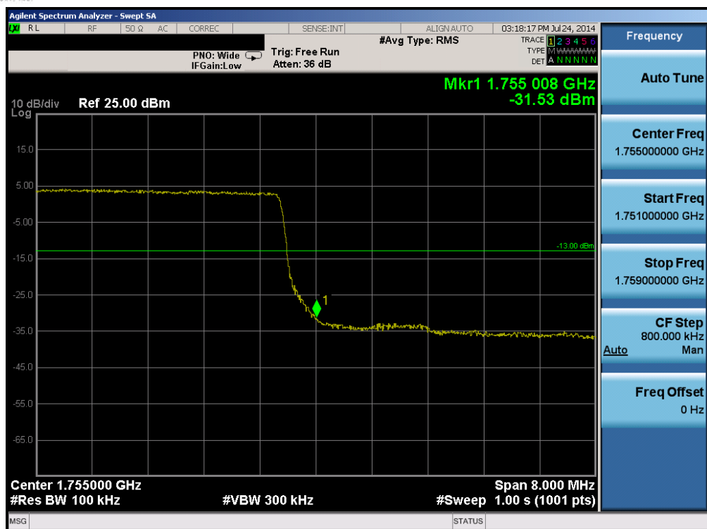
Plot 6-69. Upper Band Edge Plot (Band 4 – 10.0MHz QPSK – RB Size 50)
