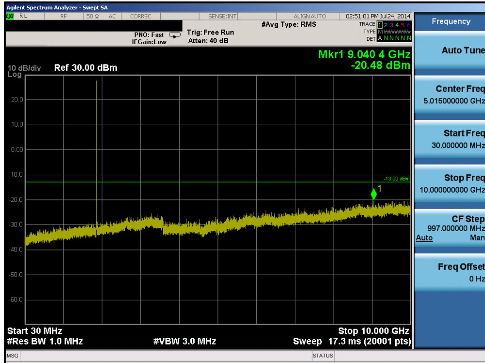
Plot 6-41. Conducted Spurious Plot (Band 2 – 5.0MHz QPSK – RB Size 1, RB Offset 0 – Mid Channel)
