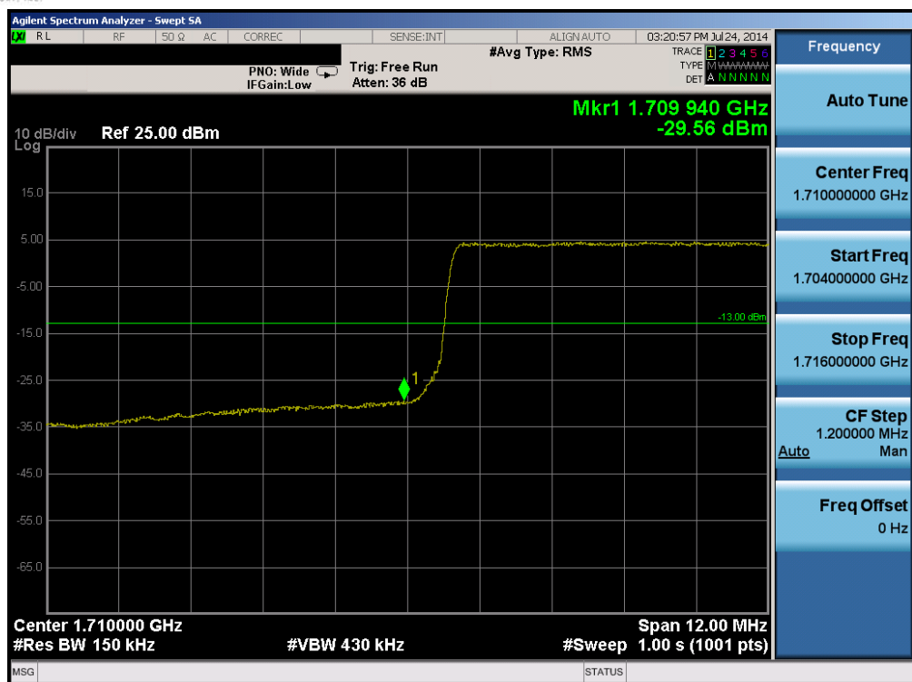
Plot 6-71. Lower Band Edge Plot (Band 4 – 15.0MHz QPSK – RB Size 75)
