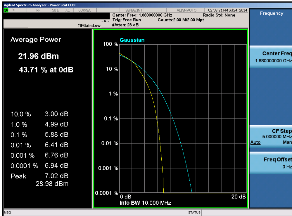
Plot 6-98. PAR Plot (Band 2 – 10.0MHz 16-QAM – RB Size 50)
