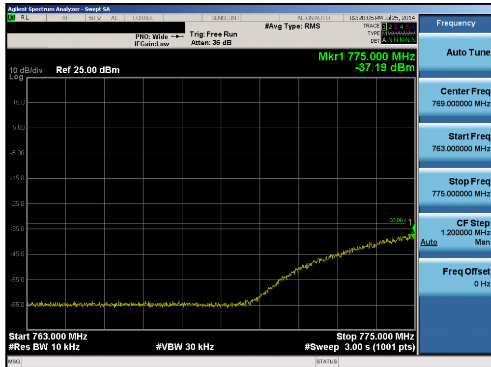
Plot 6-46. Lower Emission Mask Plot (Band 13 – 10.0MHz QPSK – RB Size 50)
