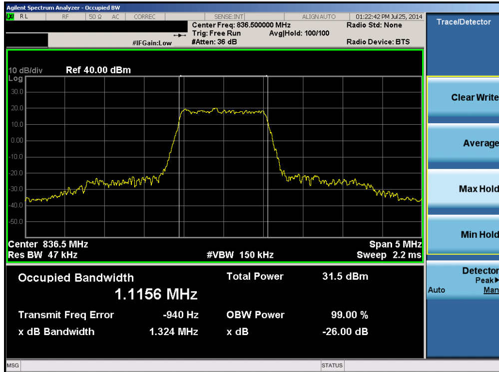
Plot 6-3. Occupied Bandwidth Plot (Band 5 – 1.4MHz QPSK – RB Size 6)
