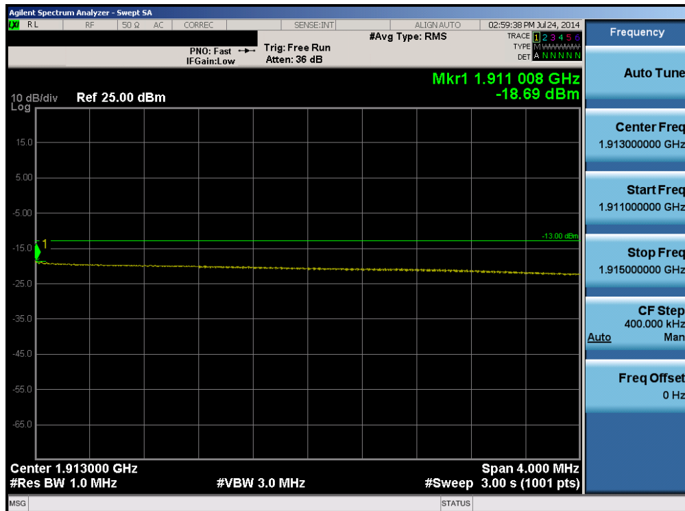
Plot 6-86. Upper Extended Band Edge Plot (Band 2 – 10.0MHz QPSK – RB Size 50)
