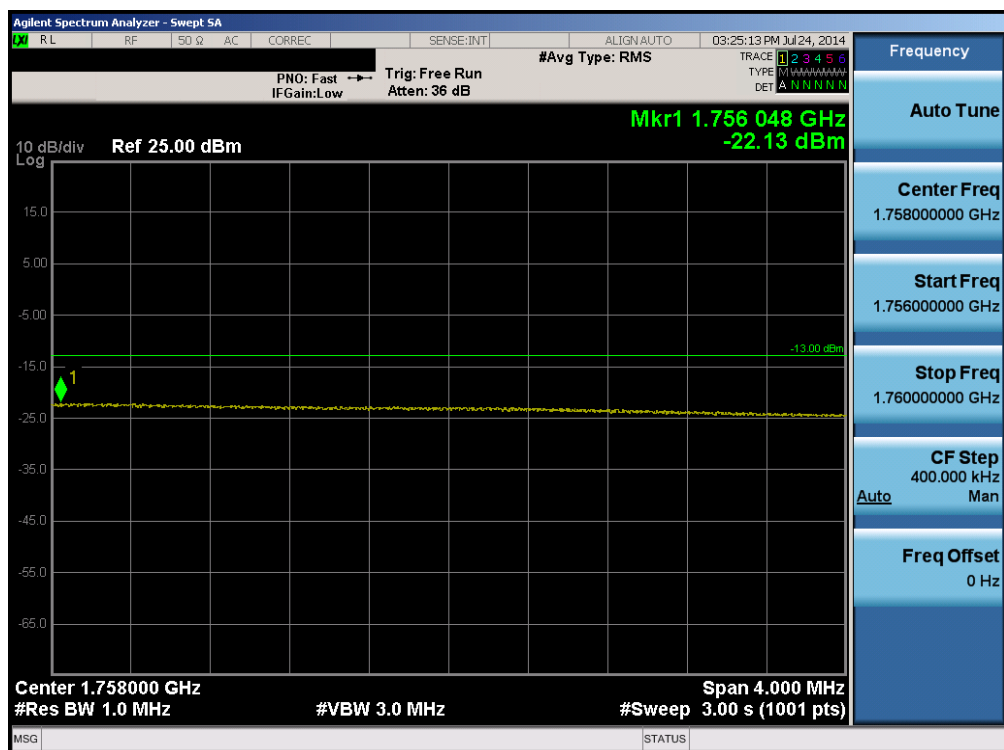
Plot 6-78. Upper Extended Band Edge Plot (Band 4 – 20.0MHz QPSK – RB Size 100)
