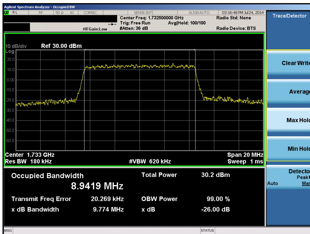
Plot 6-14. Occupied Bandwidth Plot (Band 4 – 10.0MHz 16-QAM – RB Size 50)
