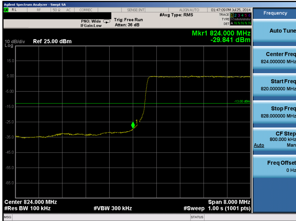
Plot 6-61. Lower Band Edge Plot (Band 5 – 10.0MHz QPSK – RB Size 50)
