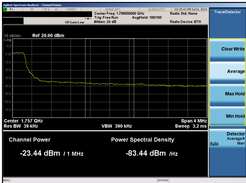
Plot 6-66. Upper Extended Band Edge Plot (Band 4 – 5.0MHz QPSK – RB Size 25)
