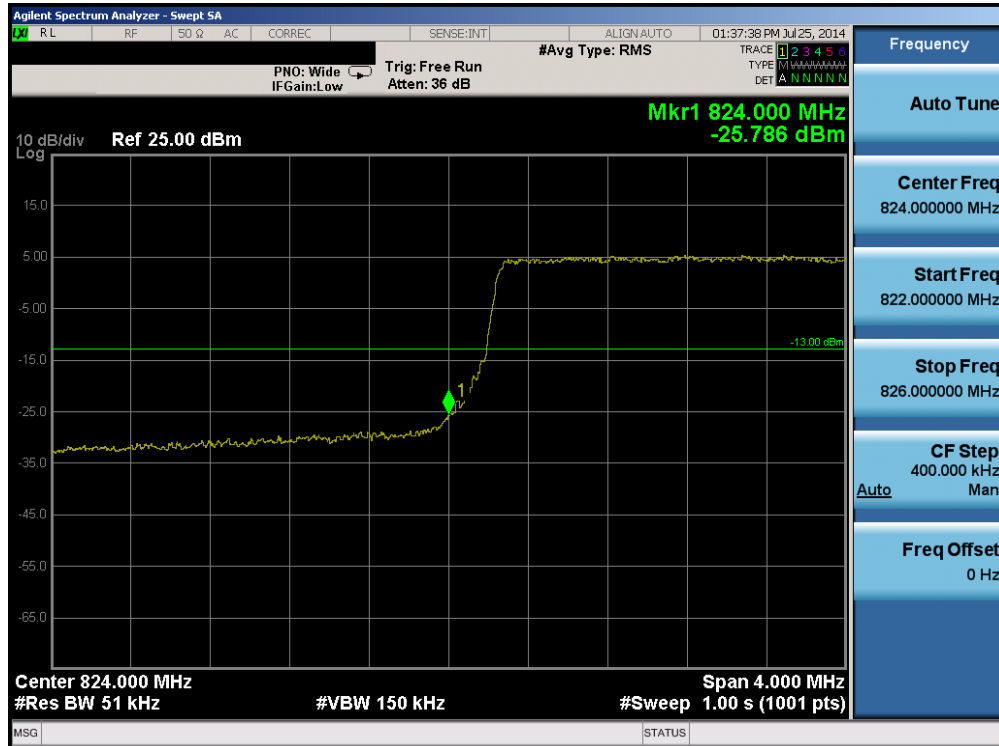
Plot 6-57. Lower Band Edge Plot (Band 5 - 5.0MHz QPSK - RB Size 25)
