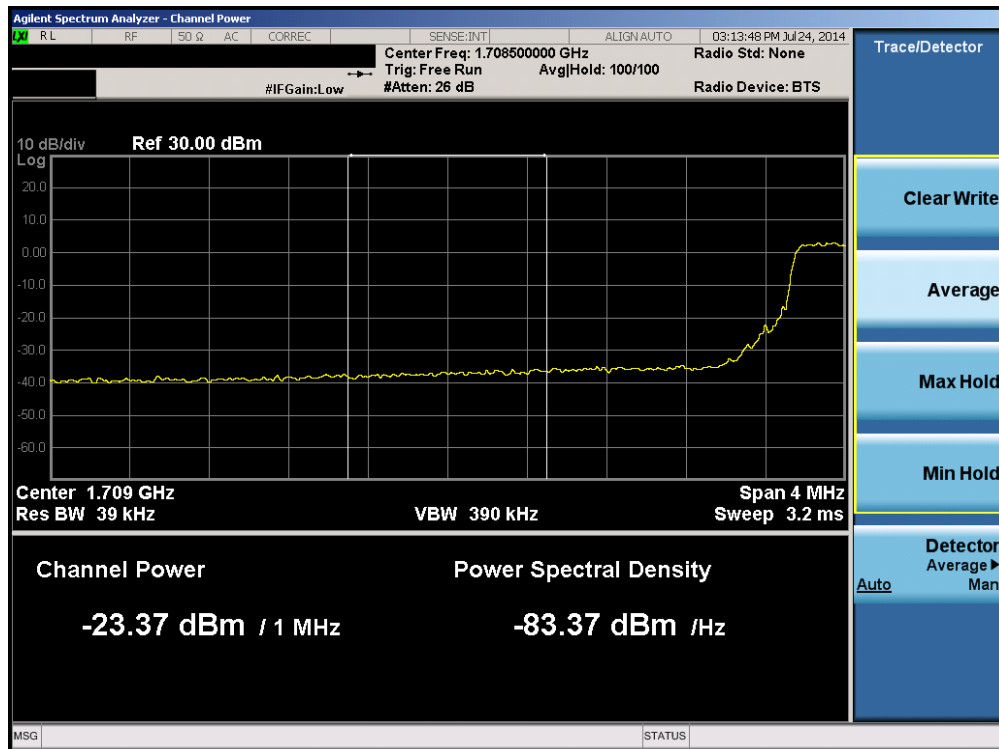
Plot 6-64. Lower Extended Band Edge Plot (Band 4 – 5.0MHz QPSK – RB Size 25)
