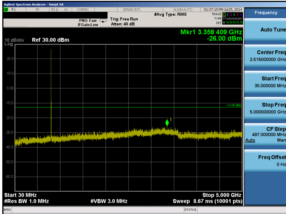
Plot 6-27. Conducted Spurious Plot (Band 5 – 5.0MHz QPSK – RB Size 1, RB Offset 0 – Low Channel)
