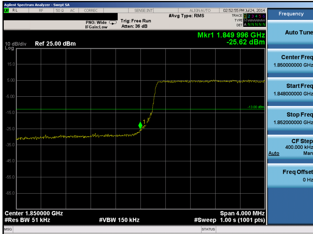
Plot 6-79. Lower Band Edge Plot (Band 2 – 5.0MHz QPSK – RB Size 25)
