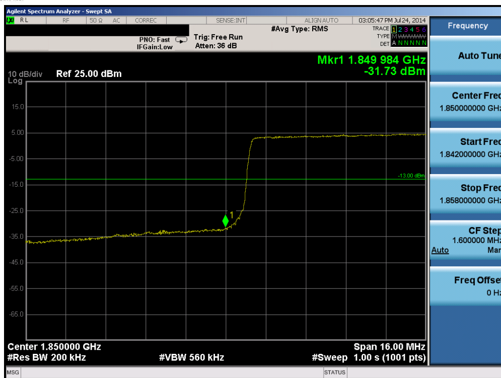
Plot 6-91. Lower Band Edge Plot (Band 2 – 20.0MHz QPSK – RB Size 100)
