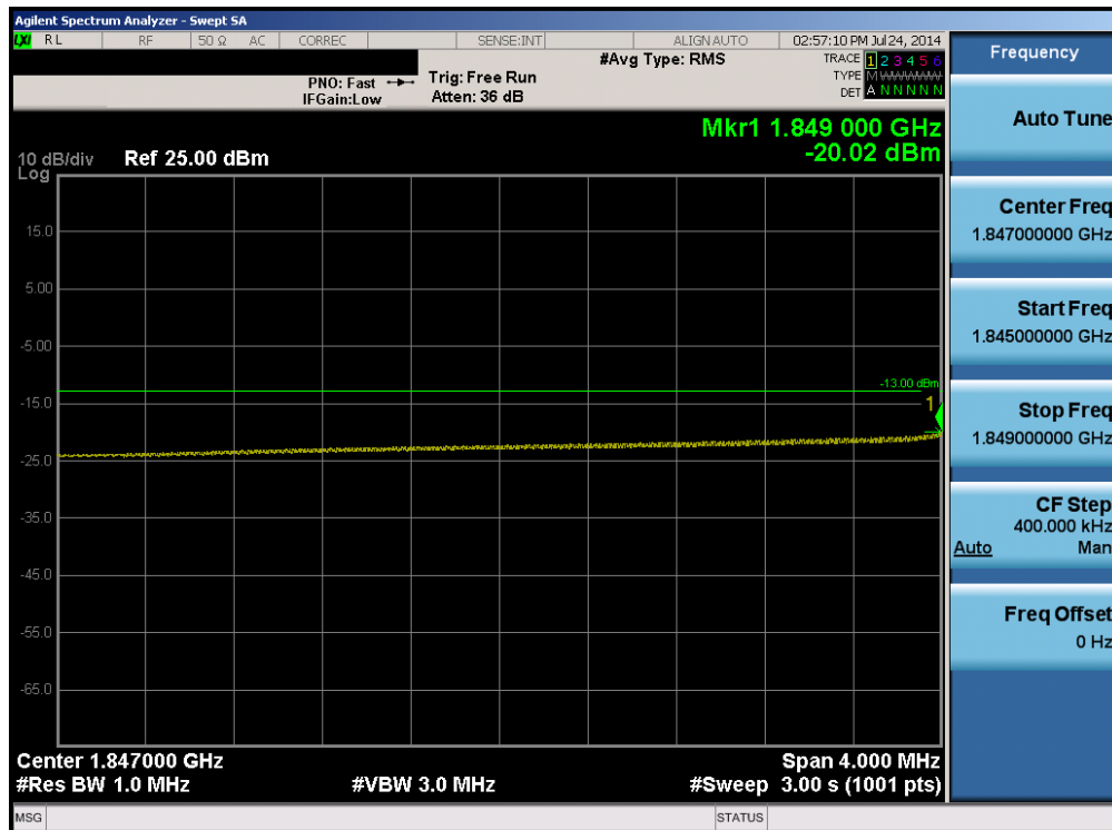
Plot 6-84. Lower Extended Band Edge Plot (Band 2 - 10.0MHz QPSK - RB Size 50)
