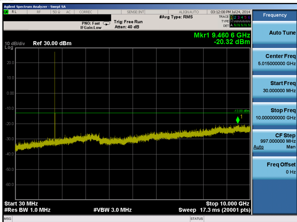
Plot 6-33. Conducted Spurious Plot (Band 4 – 5.0MHz QPSK – RB Size 1, RB Offset 0 – Low Channel)
