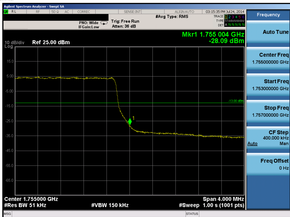
Plot 6-65. Upper Band Edge Plot (Band 4 – 5.0MHz QPSK – RB Size 25)
