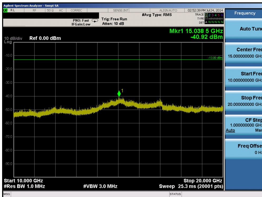
Plot 6-40. Conducted Spurious Plot (Band 2 – 5.0MHz QPSK – RB Size 1, RB Offset 0 – Low Channel)
