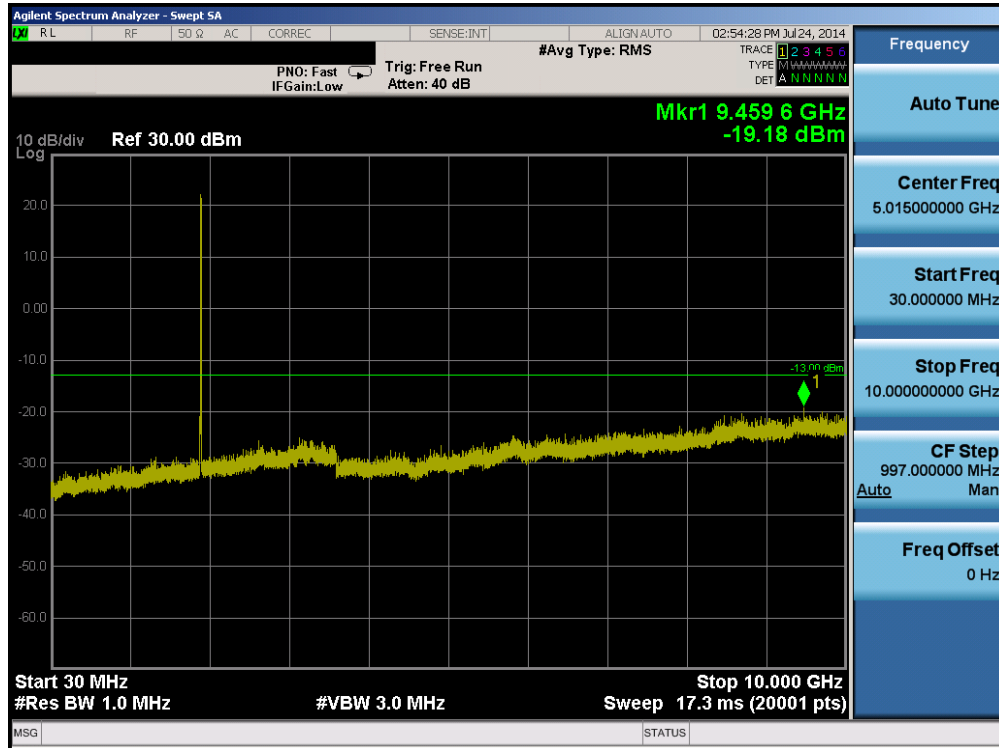
Plot 6-43. Conducted Spurious Plot (Band 2 – 5.0MHz QPSK – RB Size 1, RB Offset 0 – High Channel)
