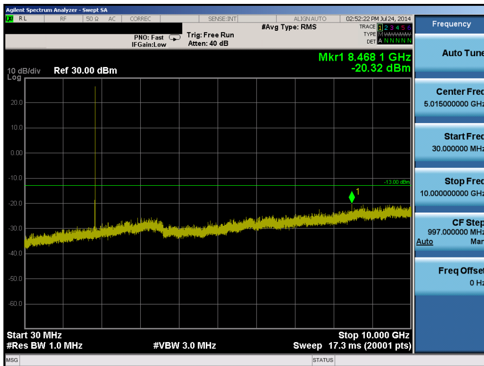
Plot 6-39. Conducted Spurious Plot (Band 2 – 5.0MHz QPSK – RB Size 1, RB Offset 0 – Low Channel)
