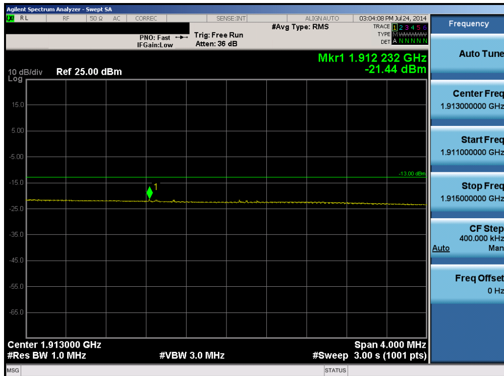
Plot 6-90. Upper Extended Band Edge Plot (Band 2 – 15.0MHz QPSK – RB Size 75)
