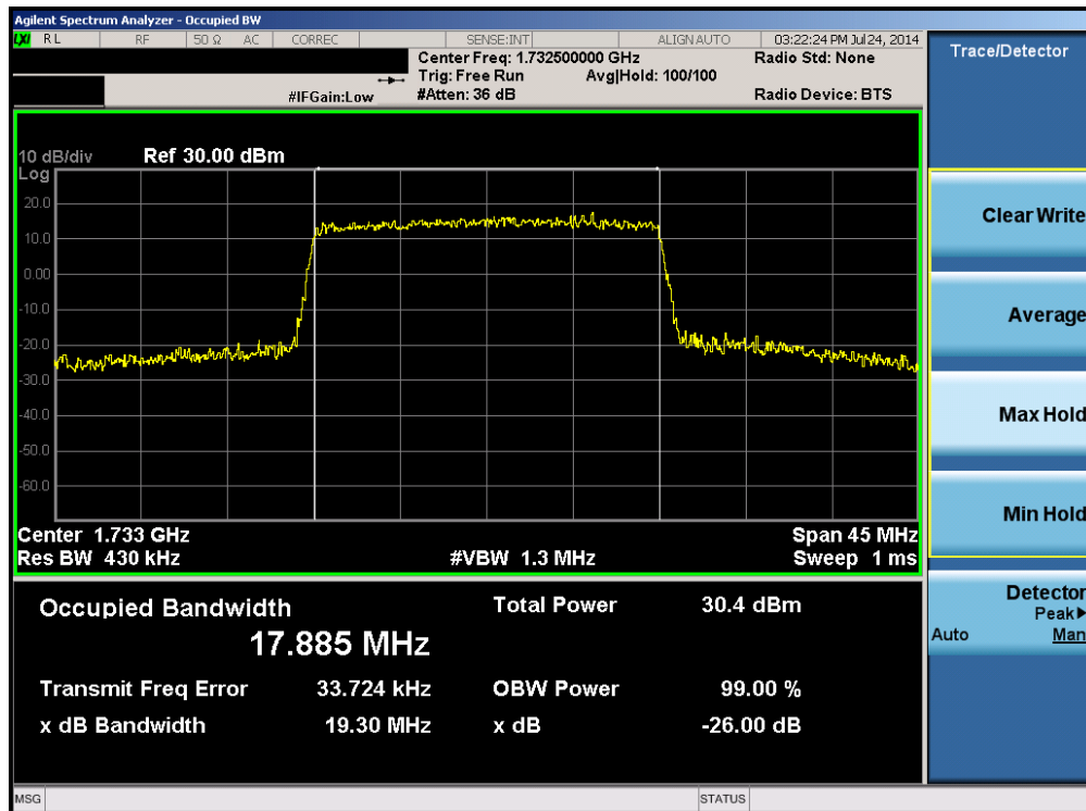
Plot 6-18. Occupied Bandwidth Plot (Band 4 – 20.0MHz 16-QAM – RB Size 100)
