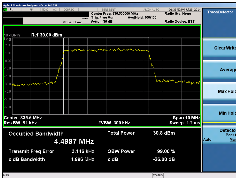
Plot 6-8. Occupied Bandwidth Plot (Band 5 – 5.0MHz 16-QAM – RB Size 25)
