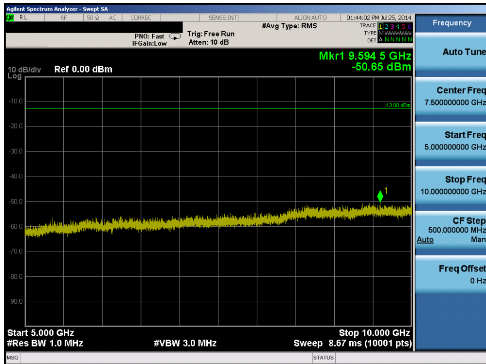
Plot 6-32. Conducted Spurious Plot (Band 5 – 5.0MHz QPSK – RB Size 1, RB Offset 0 – High Channel)
