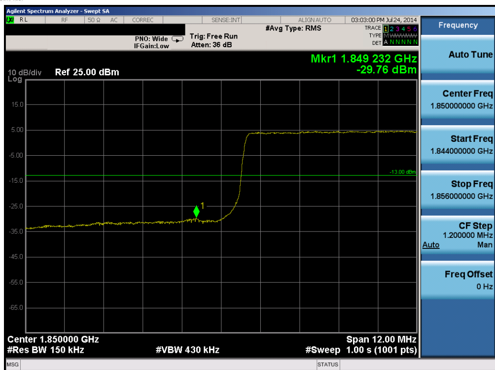
Plot 6-87. Lower Band Edge Plot (Band 2 – 15.0MHz QPSK – RB Size 75)
