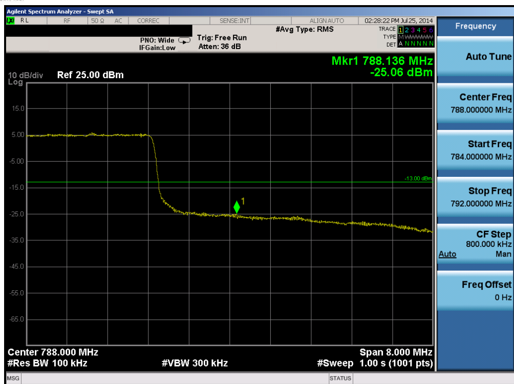
Plot 6-47. Upper Band Edge Plot (Band 13 – 10.0MHz QPSK – RB Size 50)
