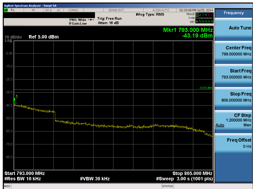
Plot 6-48. Upper Emission Mask Plot (Band 13 – 10.0MHz QPSK – RB Size 50)
