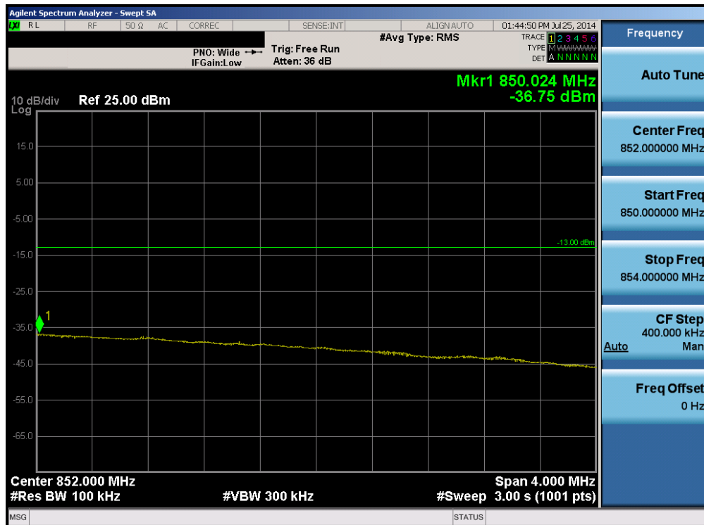
Plot 6-60. Upper Extended Band Edge Plot (Band 5 – 5.0MHz QPSK – RB Size 25)
