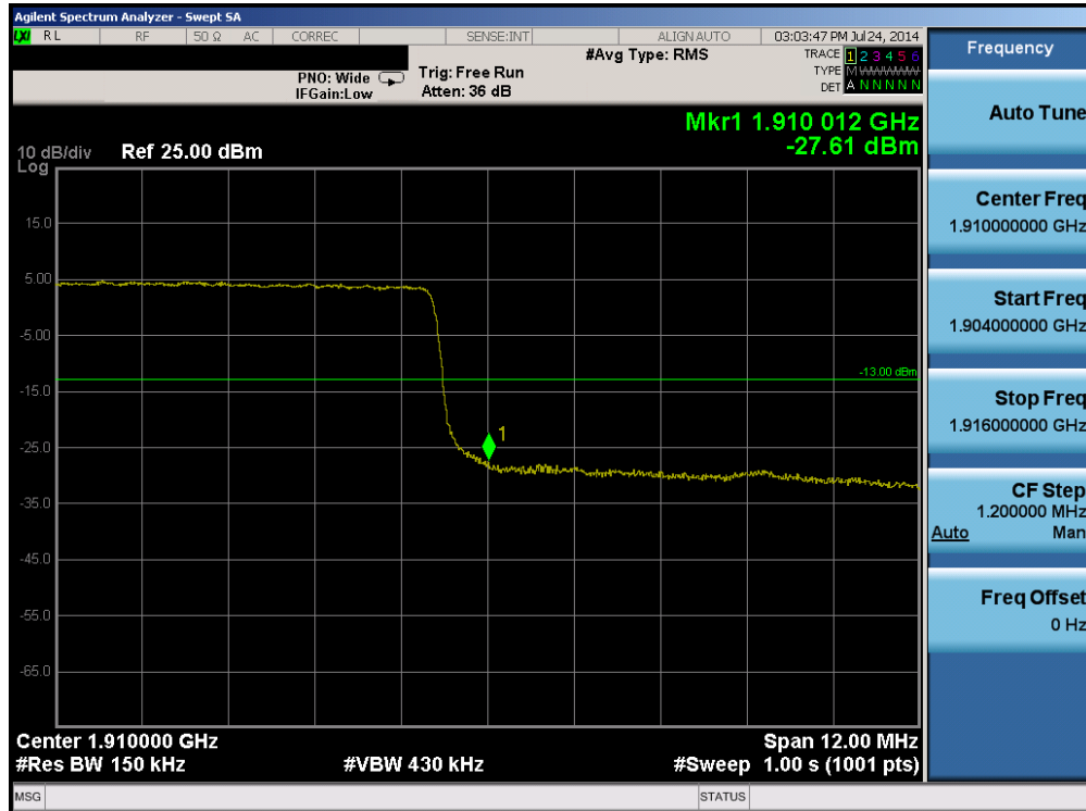
Plot 6-89. Upper Band Edge Plot (Band 2 – 15.0MHz QPSK – RB Size 75)
