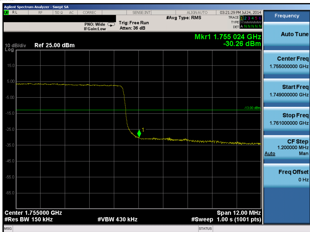
Plot 6-73. Upper Band Edge Plot (Band 4 – 15.0MHz QPSK – RB Size 75)
