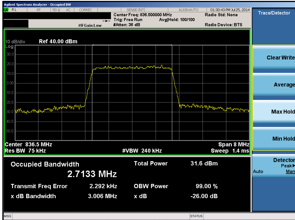
Plot 6-5. Occupied Bandwidth Plot (Band 5 – 3.0MHz QPSK – RB Size 15)
