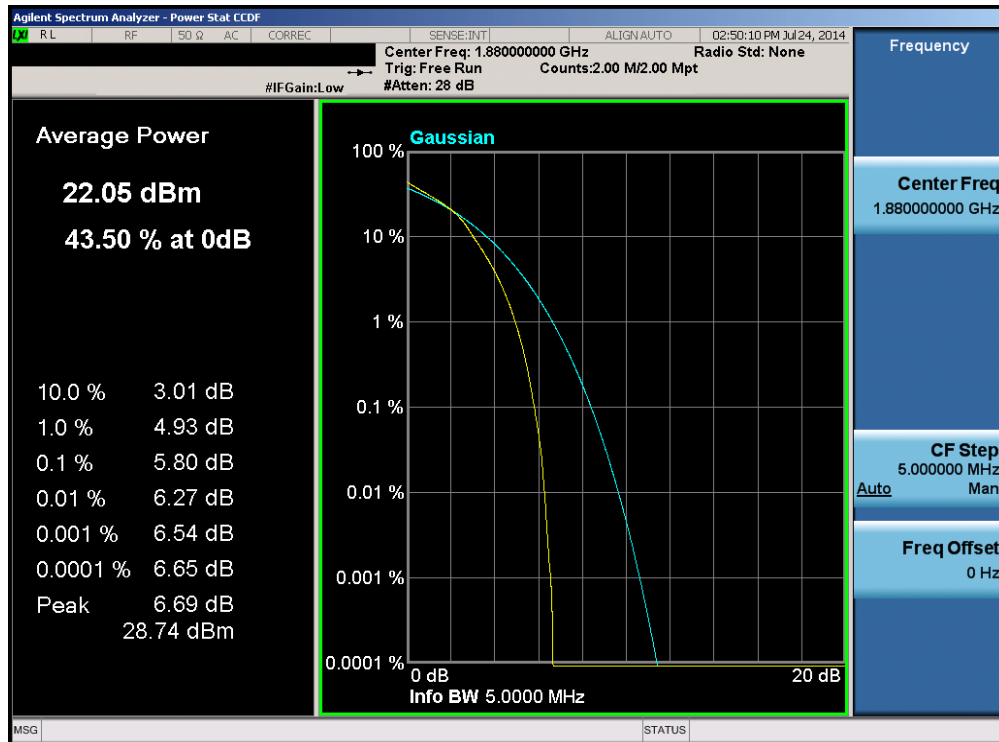
Plot 6-96. PAR Plot (Band 2 – 5.0MHz 16-QAM – RB Size 25)
