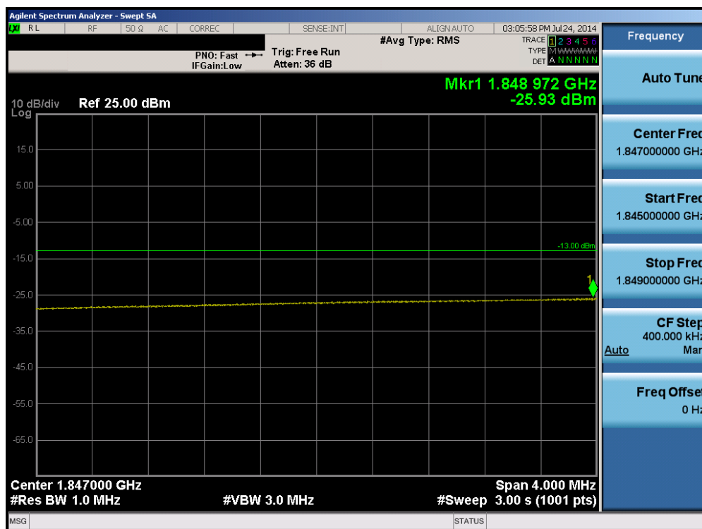
Plot 6-92. Lower Extended Band Edge Plot (Band 2 – 20.0MHz QPSK – RB Size 100)
