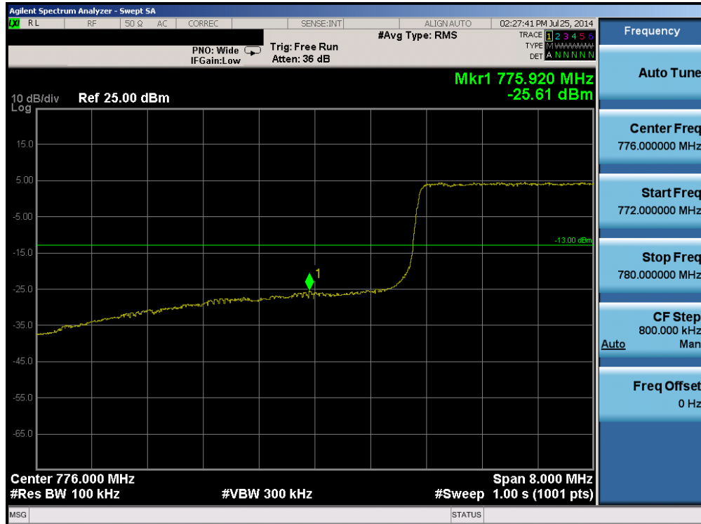
Plot 6-45. Lower Band Edge Plot (Band 13 – 10.0MHz QPSK – RB Size 50)
