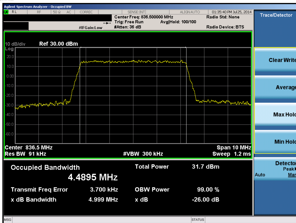
Plot 6-7. Occupied Bandwidth Plot (Band 5 – 5.0MHz QPSK – RB Size 25)
