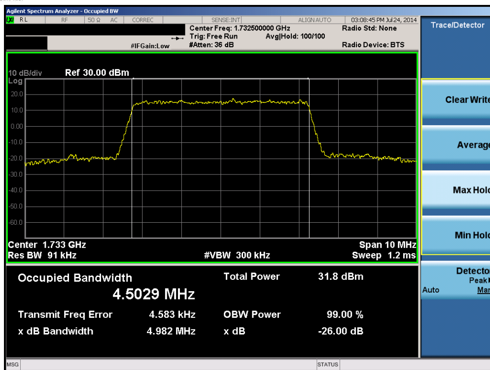
Plot 6-11. Occupied Bandwidth Plot (Band 4 – 5.0MHz QPSK – RB Size 25)
