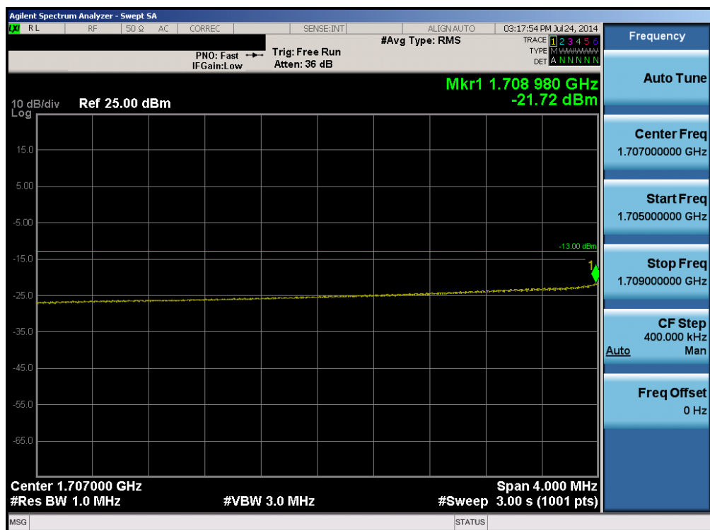
Plot 6-68. Lower Extended Band Edge Plot (Band 4 – 10.0MHz QPSK – RB Size 50)
