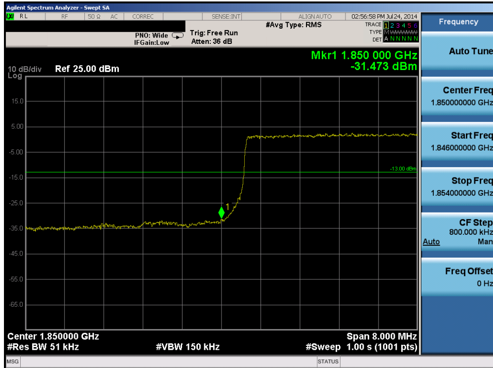
Plot 6-83. Lower Band Edge Plot (Band 2 - 10.0MHz QPSK - RB Size 50)
