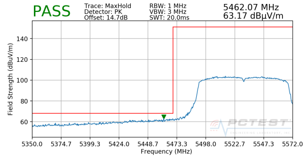
Plot 7-236. Radiated Lower Band Edge Plot MIMO (Peak – UNII Band 2C)
