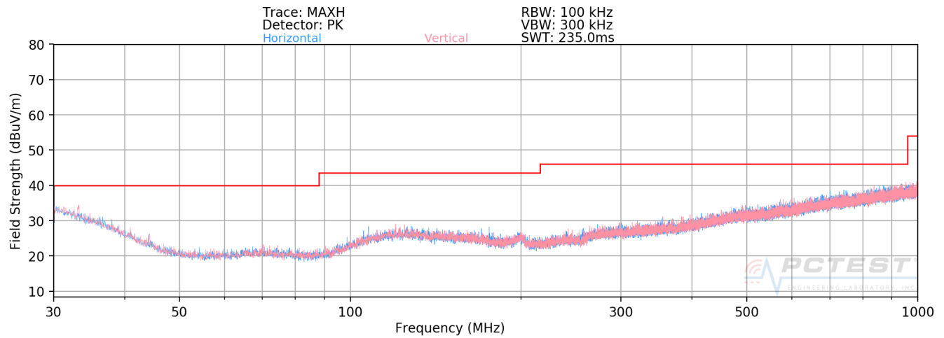
Plot 7-239. Radiated Spurious Plot below 1GHz SISO ANT2 (802.11a – U3 Ch. 157)
