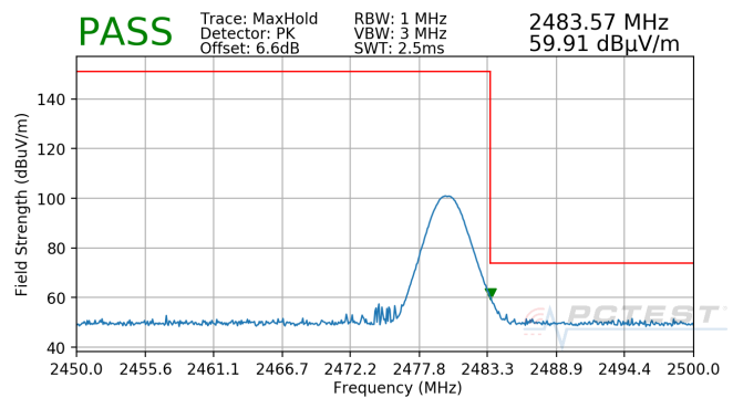
Plot 7-47. Radiated Restricted Upper Band Edge Measurement (Peak)
