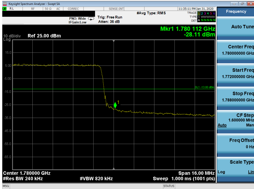
Plot 7-219. Upper Band Edge Plot (Band 66 - 20.0MHz QPSK - Full RB Configuration)
