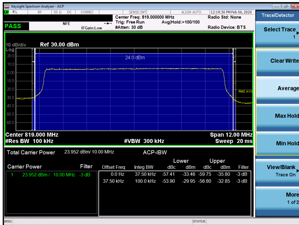
Plot 7-20. Channel Edge Plot (LTE Band 26 - 10MHz QPSK)
