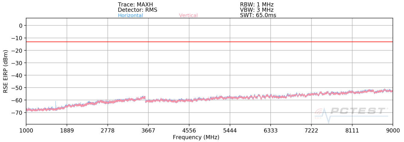
Plot 7-28. Radiated Spurious Plot (Band 26)
