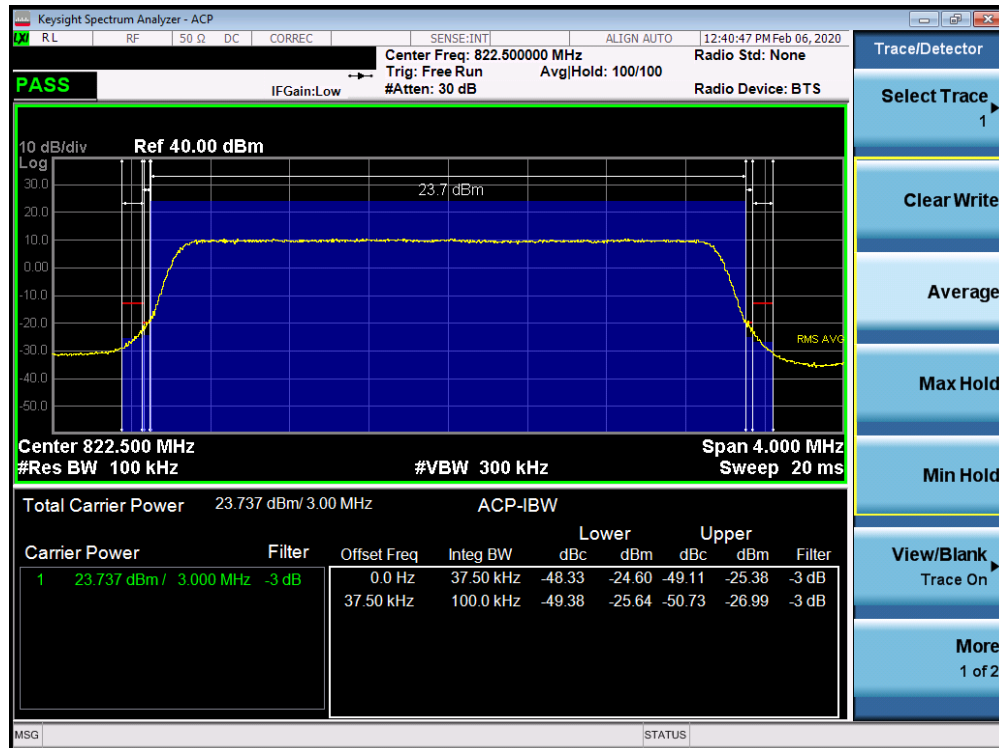
Plot 7-24. Channel Edge Plot (LTE Band 26 - 3MHz QPSK - High Channel)
