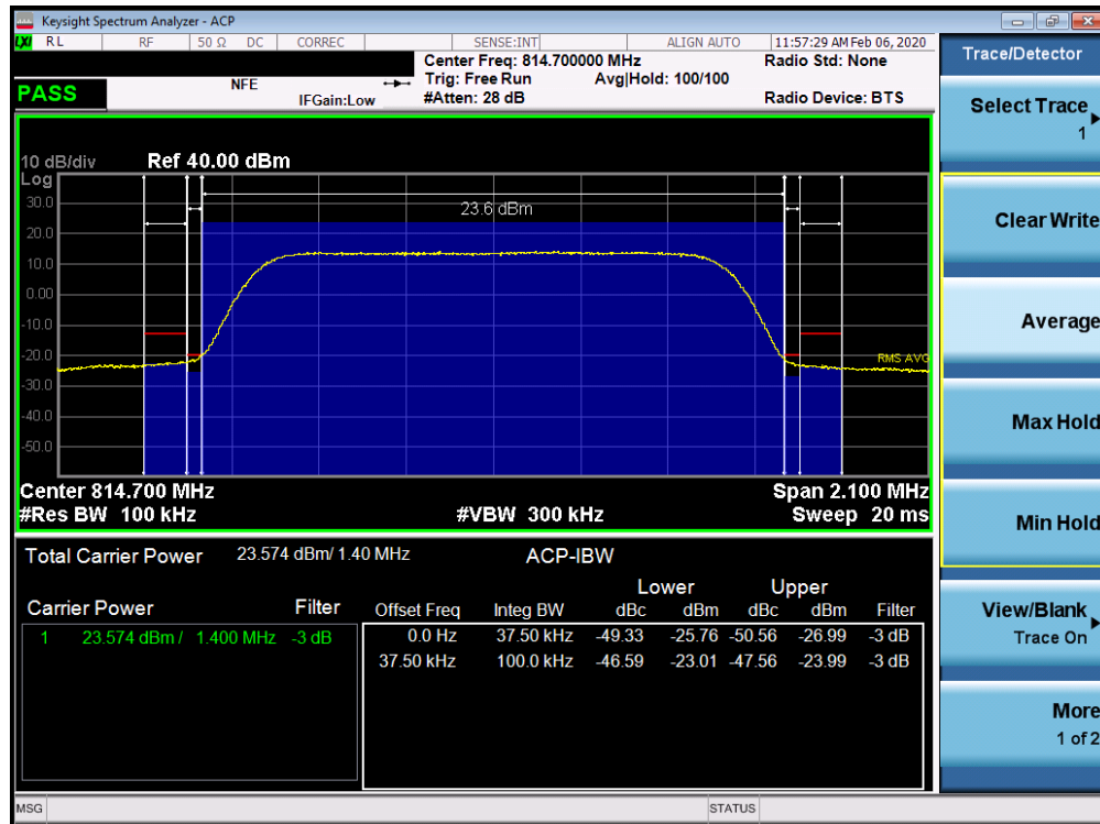
Plot 7-25. Channel Edge Plot (LTE Band 26 - 1.4MHz QPSK - Low Channel)
