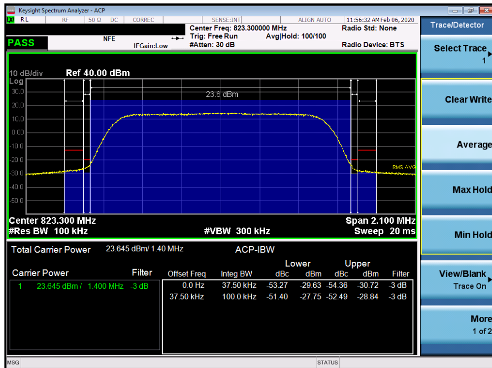
Plot 7-26. Channel Edge Plot (LTE Band 26 - 1.4MHz QPSK - High Channel)
