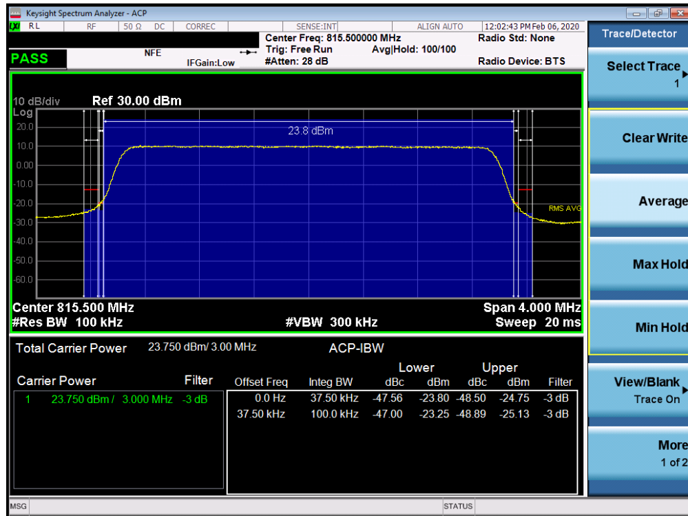
Plot 7-23. Channel Edge Plot (LTE Band 26 - 3MHz QPSK - Low Channel)
