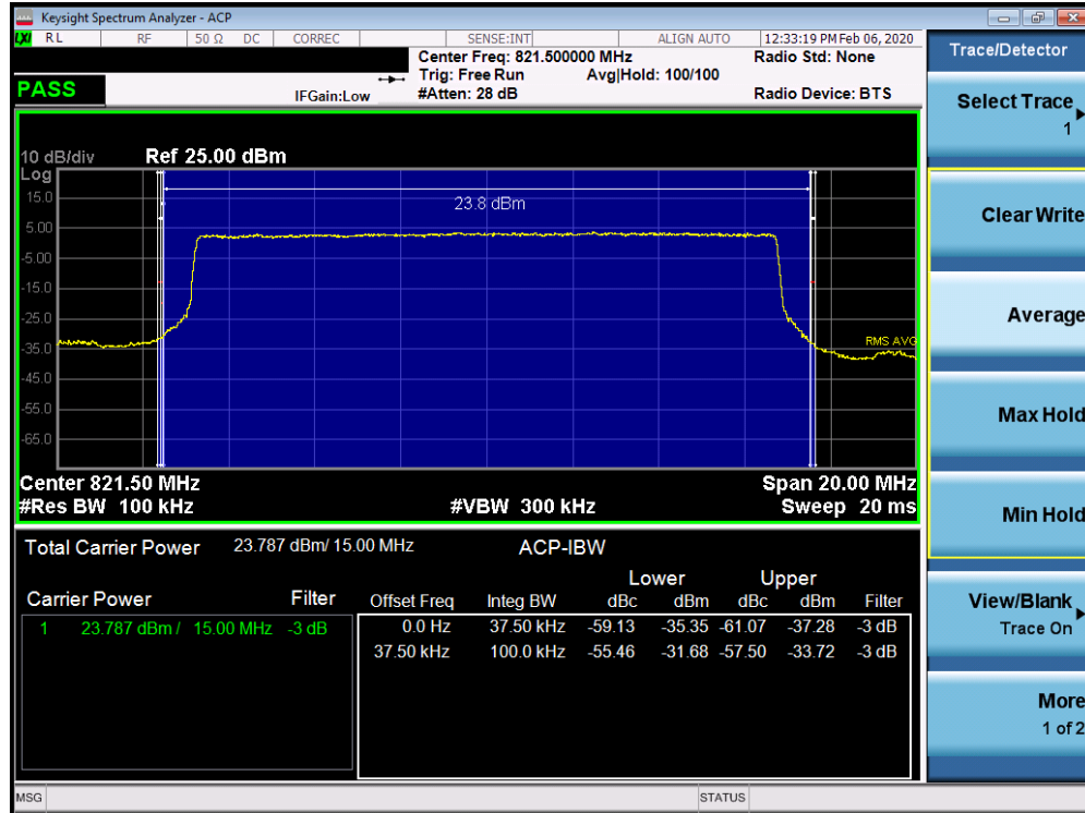
Plot 7-19. Channel Edge Plot (LTE Band 26 - 15MHz QPSK)
