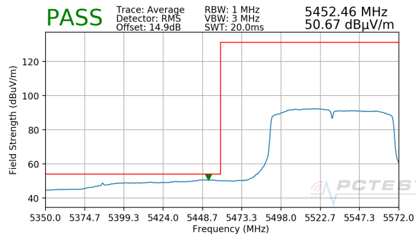
Plot 7-233. Radiated Lower Band Edge Plot MIMO (Average – UNII Band 2C)
