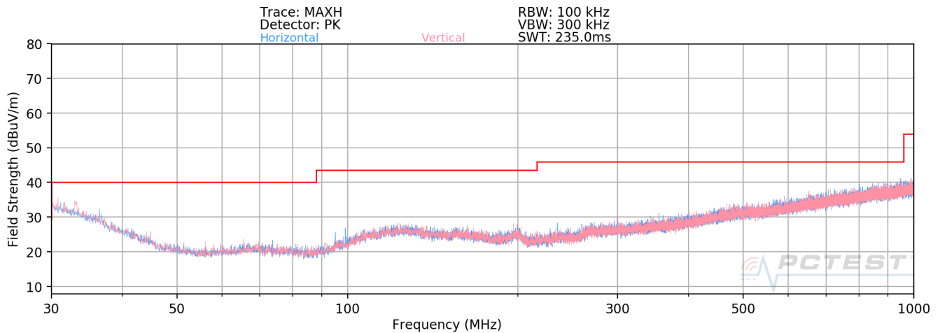
Plot 7-237. Radiated Spurious Plot below 1GHz SISO ANT2 (802.11a – U3 Ch. 157)
