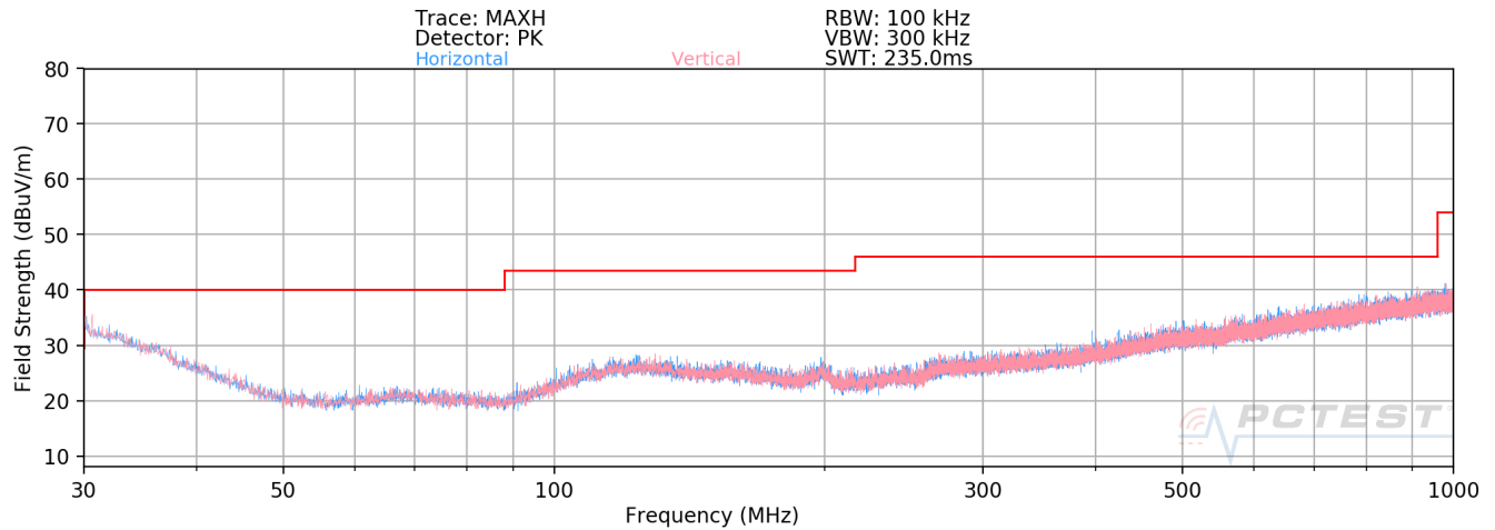
Plot 7-238. Radiated Spurious Plot below 1GHz MIMO (802.11a – U3 Ch. 157)
