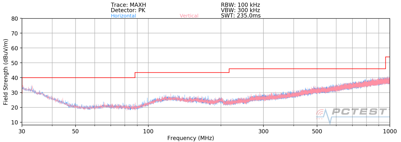
Plot 7-236. Radiated Spurious Plot below 1GHz SISO ANT1 (802.11a – U3 Ch. 157)
