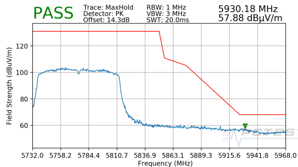
Plot 7-235. Radiated Upper Band Edge Plot MIMO (Peak – UNII Band 3)
