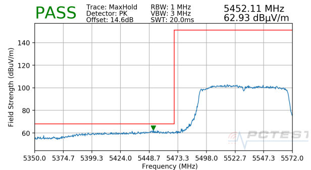
Plot 7-234. Radiated Lower Band Edge Plot MIMO (Peak – UNII Band 2C)
