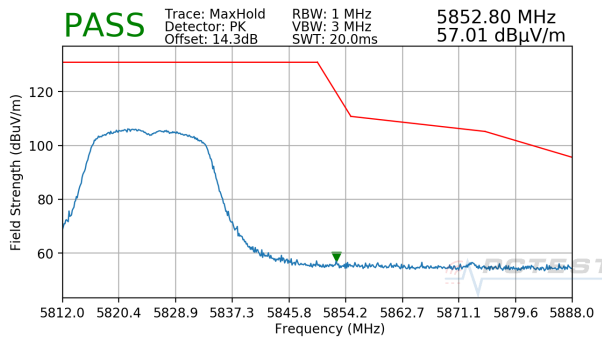
Plot 7-200. Radiated Upper Band Edge Plot SISO ANT2 (Peak – UNII Band 3)
