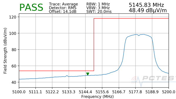
Plot 7-215. Radiated Lower Band Edge Plot MIMO (Average – UNII Band 1)
