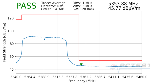
Plot 7-210. Radiated Upper Band Edge Plot SISO ANT2 (Average – UNII Band 2A)
