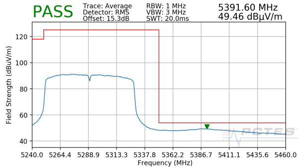
Plot 7-231. Radiated Upper Band Edge Plot MIMO (Average – UNII Band 2A)
