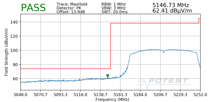
Plot 7-188. Radiated Lower Band Edge Plot SISO ANT1 (Peak - UNII Band 1)
