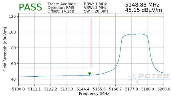
Plot 7-194. Radiated Lower Band Edge Plot SISO ANT2 (Average – UNII Band 1)
