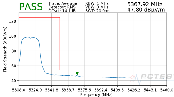
Plot 7-217. Radiated Upper Band Edge Plot MIMO (Average – UNII Band 2A)
