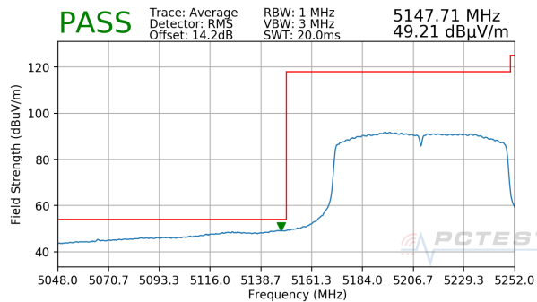
Plot 7-229. Radiated Lower Band Edge Plot MIMO (Average – UNII Band 1)
