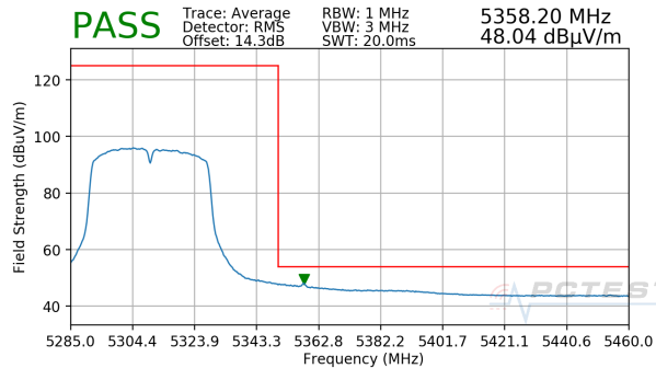
Plot 7-224. Radiated Upper Band Edge Plot MIMO (Average – UNII Band 2A)
