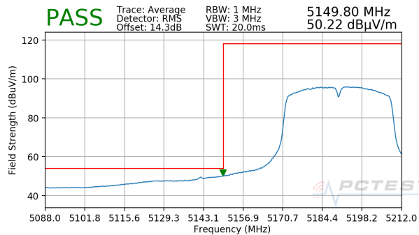
Plot 7-222. Radiated Lower Band Edge Plot MIMO (Average – UNII Band 1)
