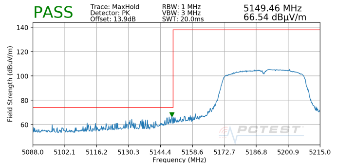
Plot 7-181. Radiated Lower Band Edge Plot SISO ANT1 (Peak – UNII Band 1)
