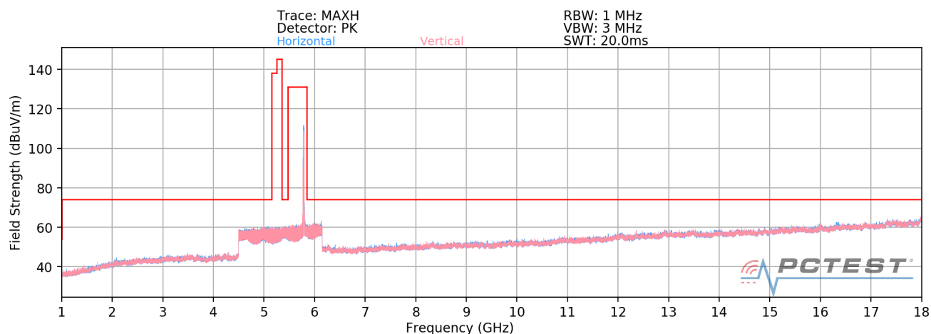
Plot 7-172. Radiated Spurious Plot above 1GHz MIMO (802.11a – U3 Ch. 157)
