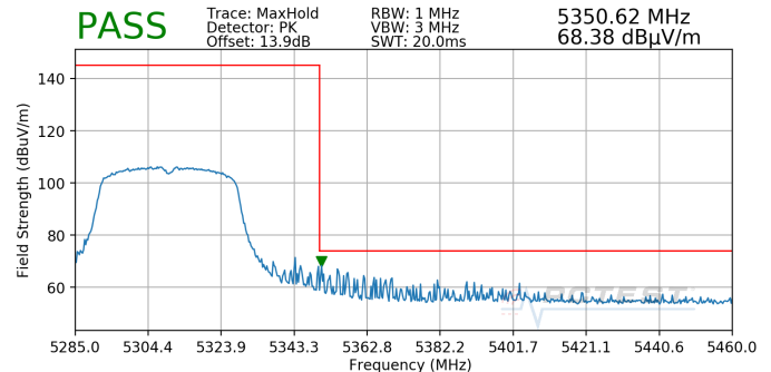
Plot 7-183. Radiated Upper Band Edge Plot SISO ANT1 (Peak – UNII Band 2A)
